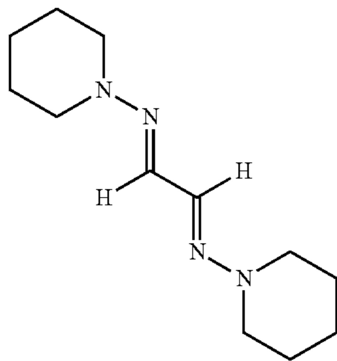
Bis-Hydrazone B
