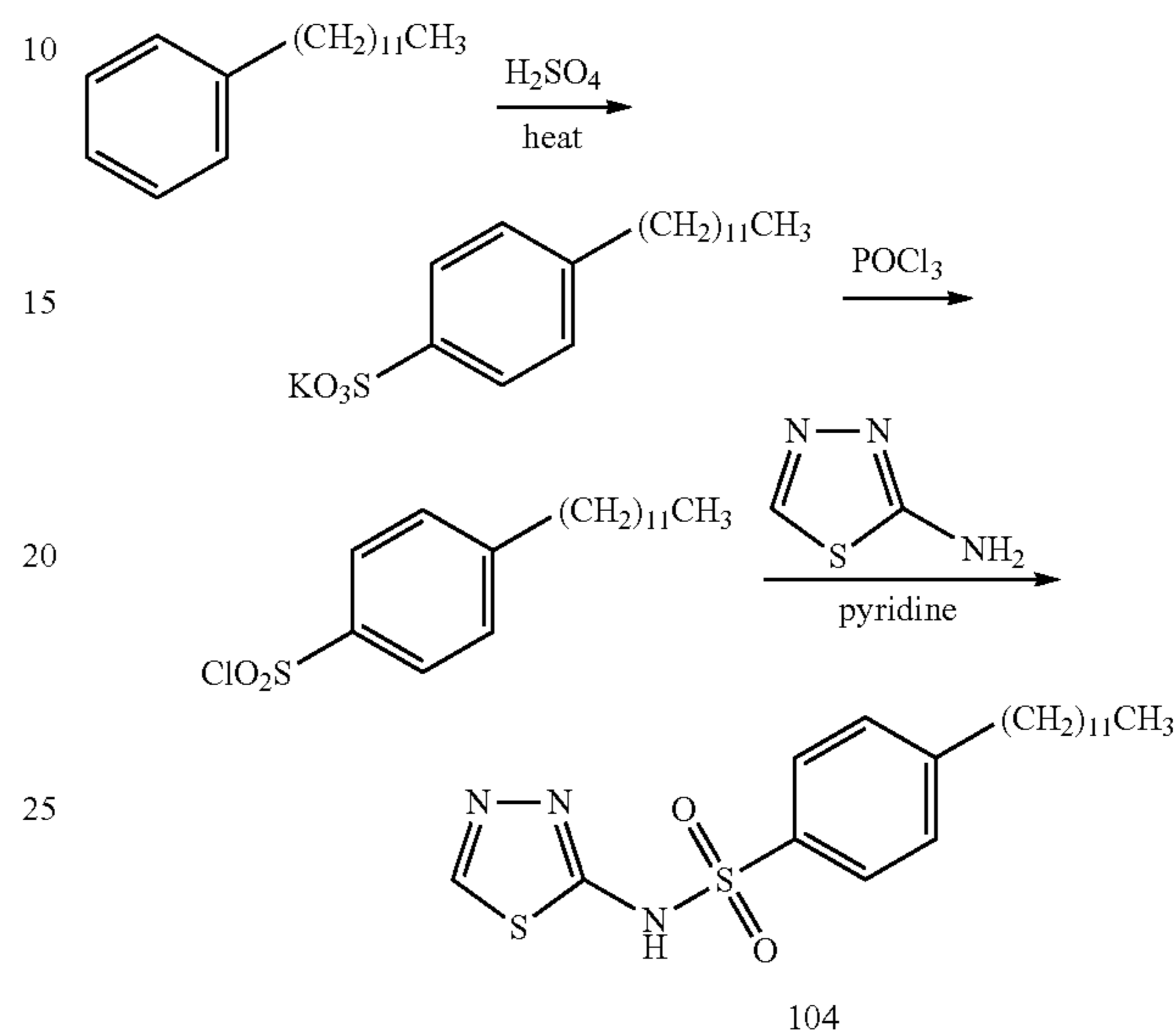
Scheme 2. Synthesis of compound 104.
