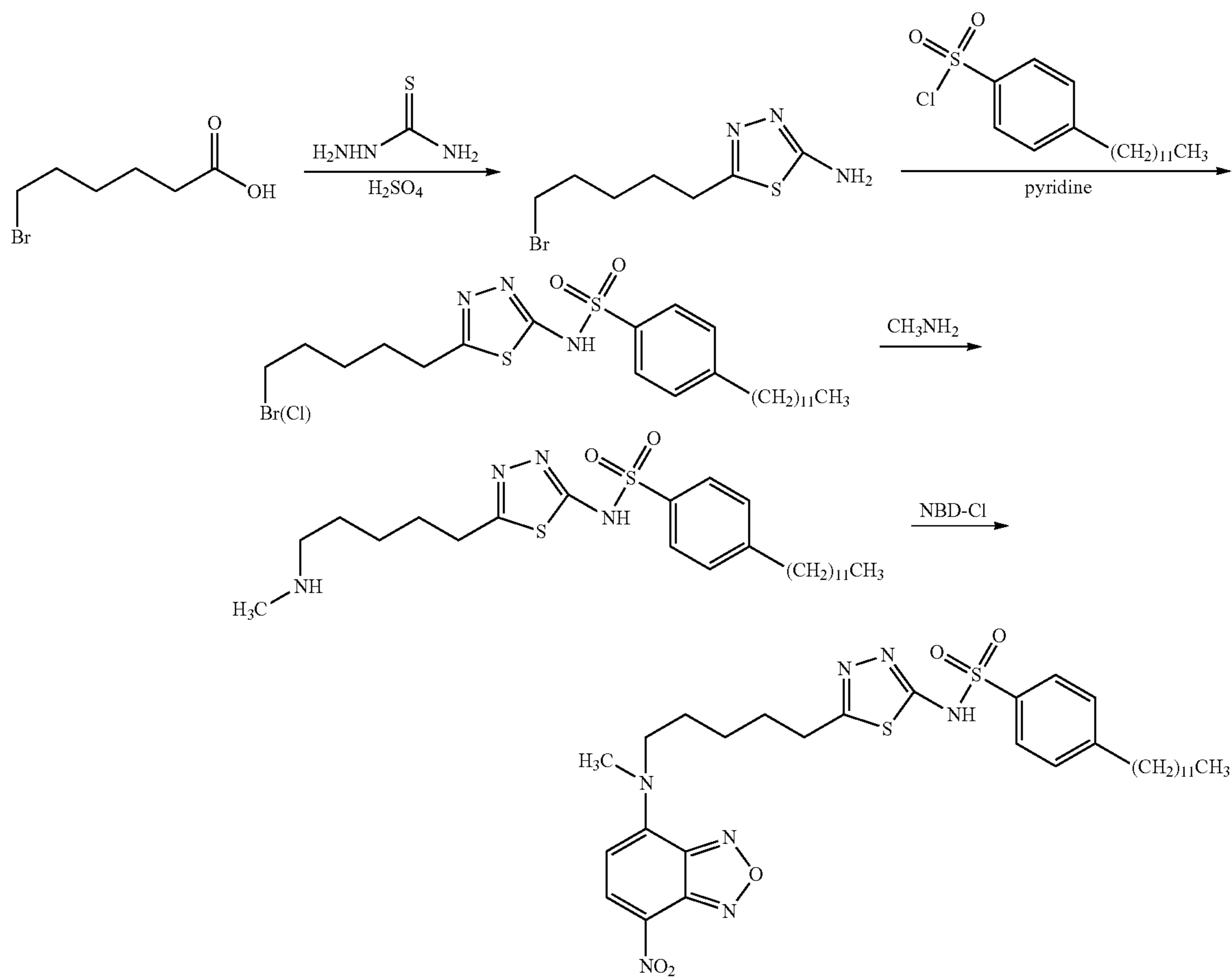
Scheme 3. Synthesis of compound 137.
