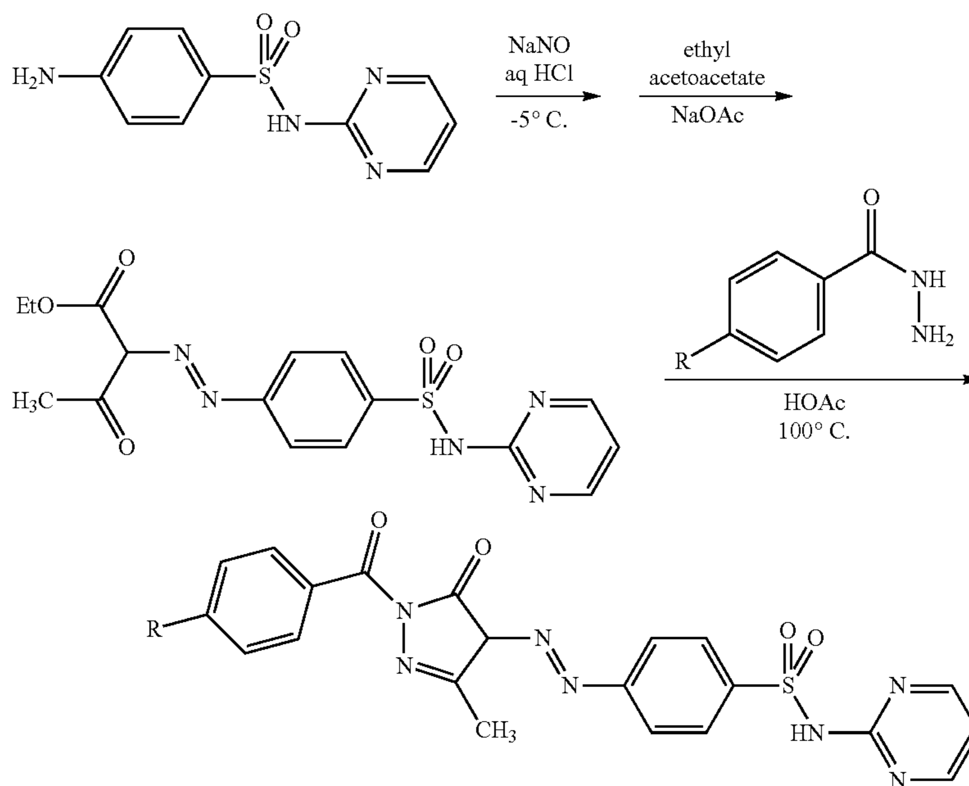
Scheme 4: Synthesis of compounds 316, 331-333, and 360
