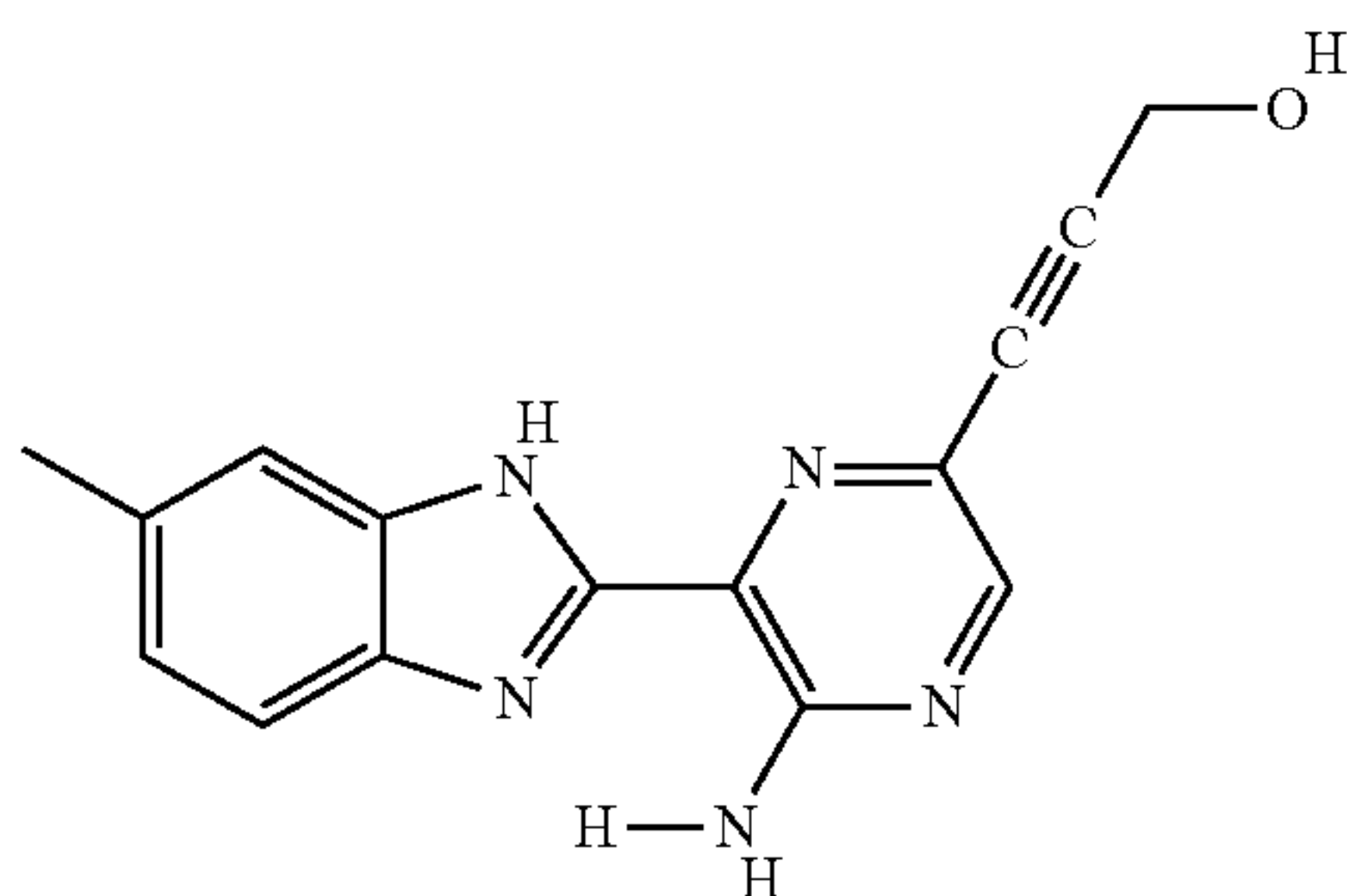
II-82
