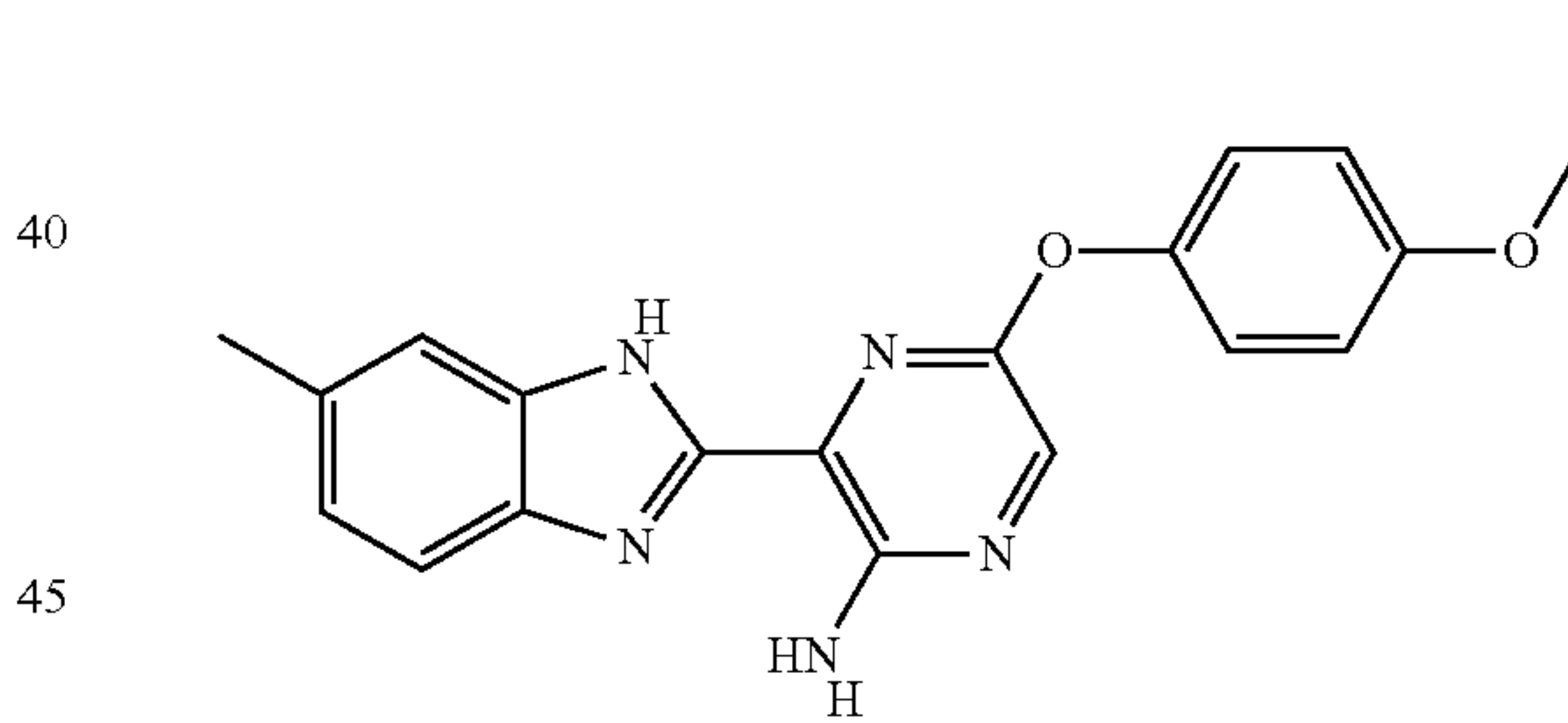
II-19
