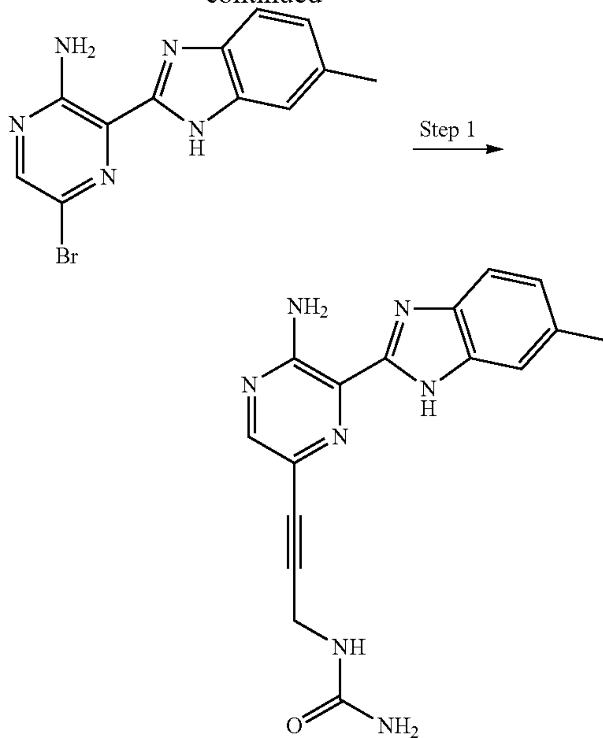
Compound II-86
