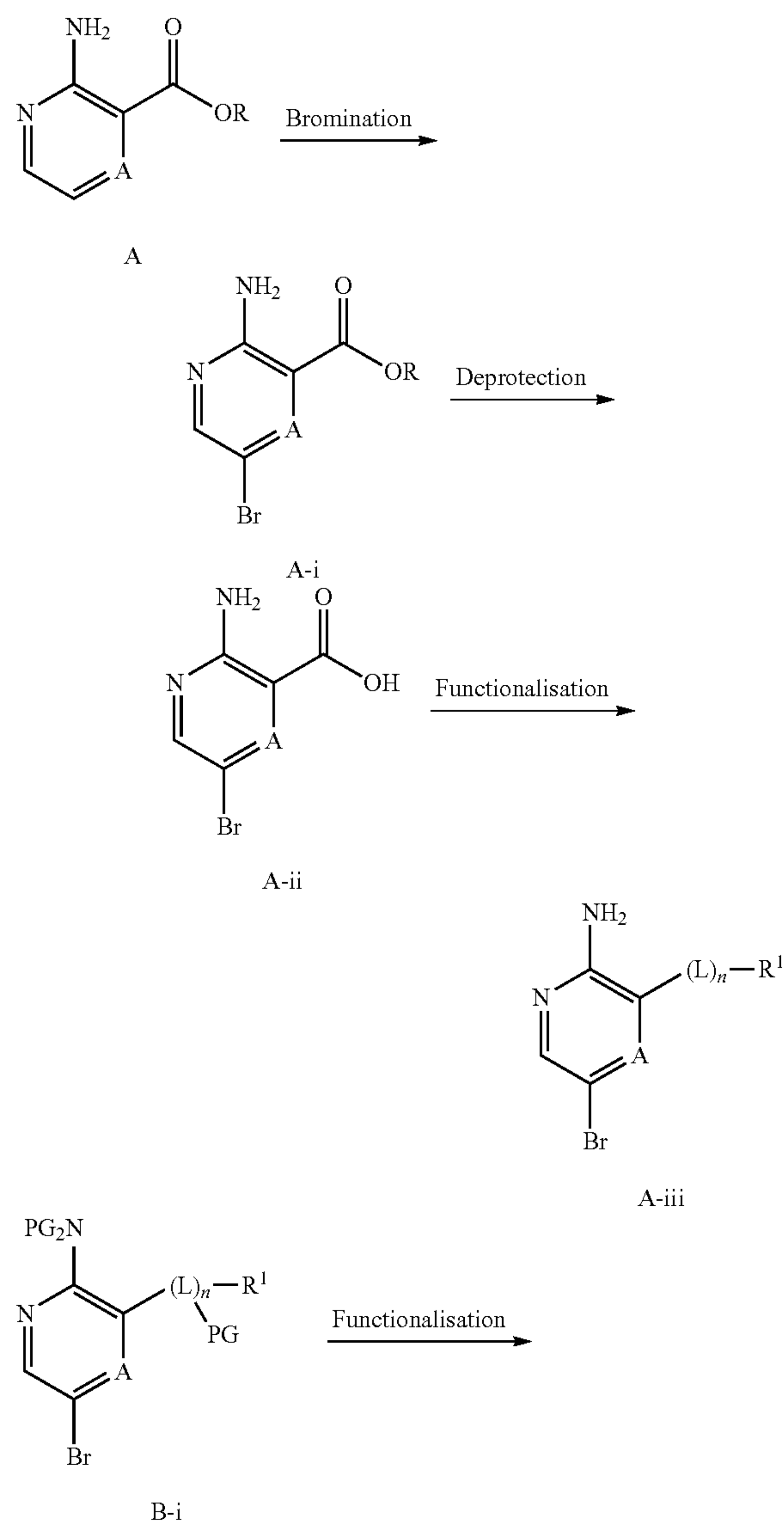
Scheme B
