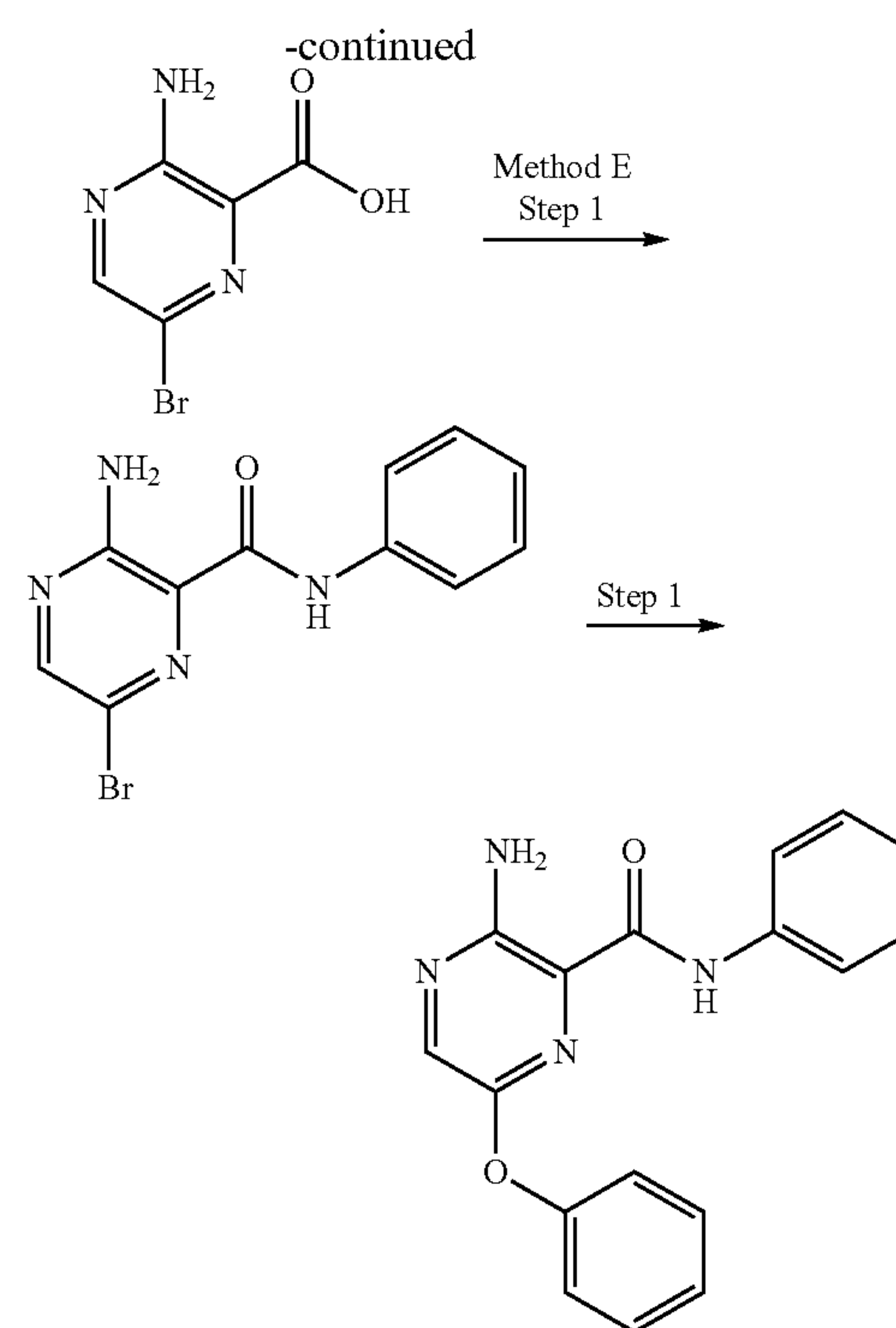
Compound II-17
