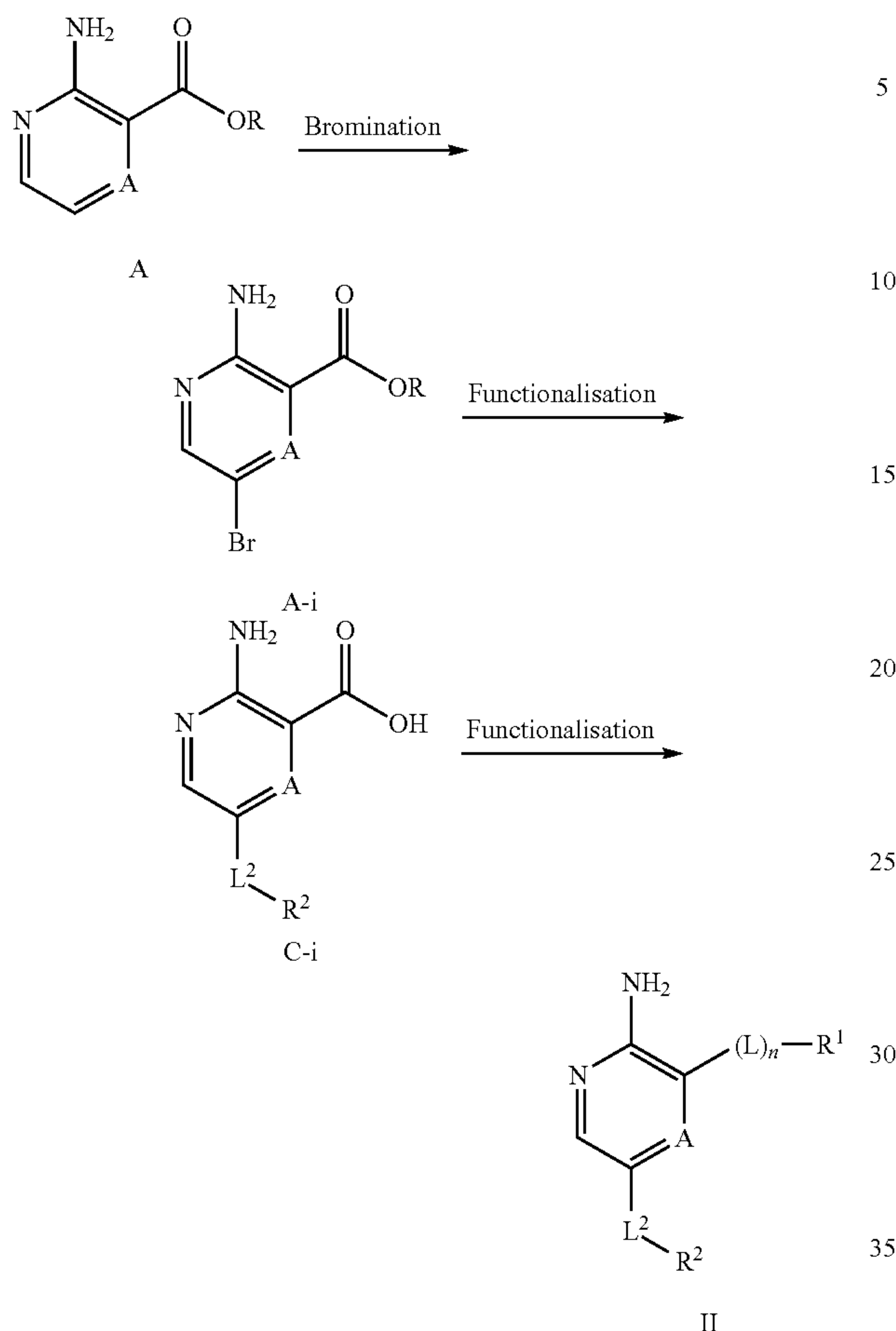
Scheme C
