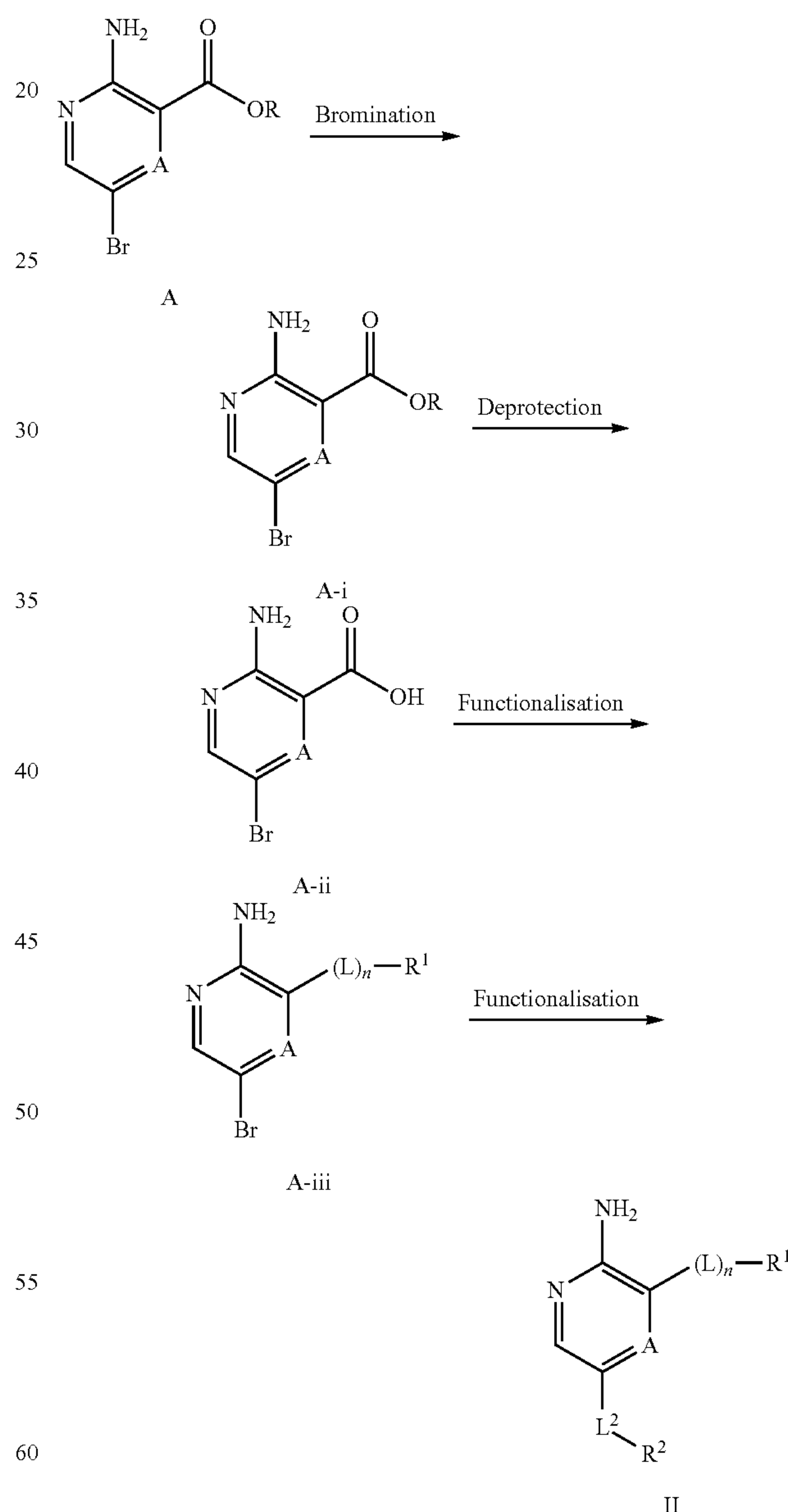
Scheme A
