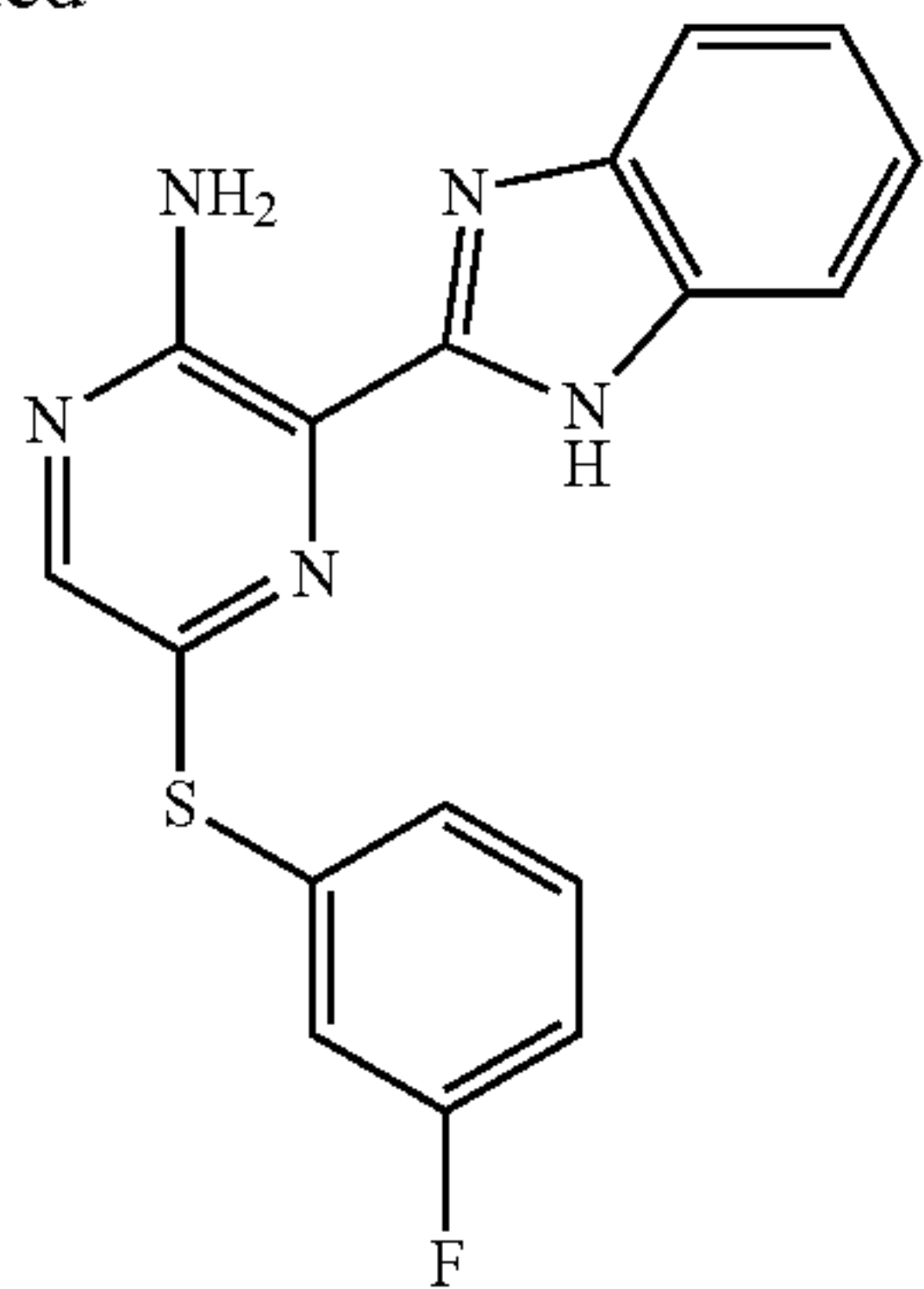
Compound II-40
