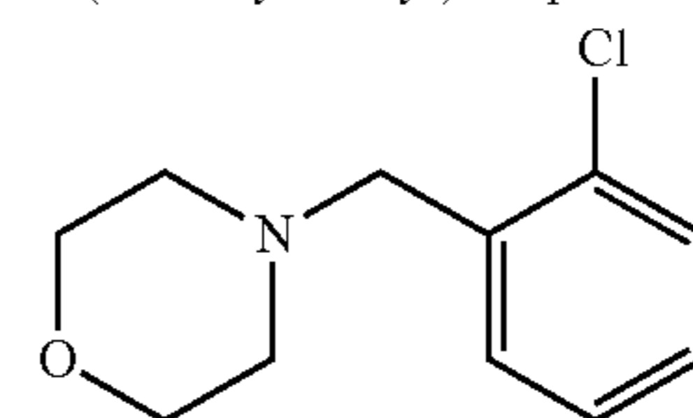
4-(2-chlorobenzyl)morpholine
