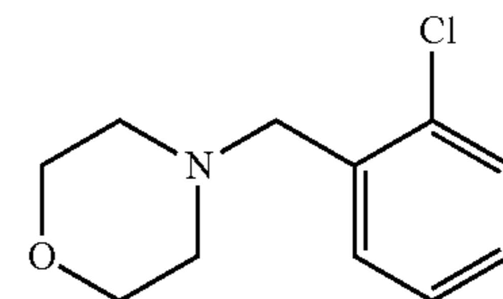
4-(2-chlorobenzyl)morpholine
