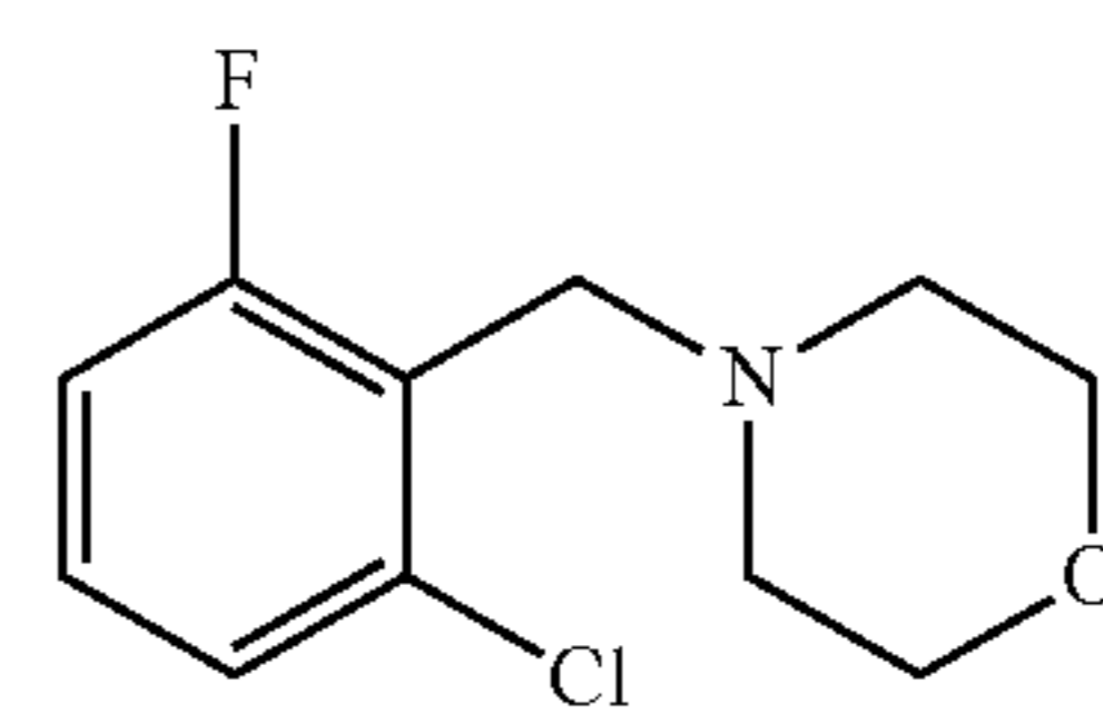
4-(2-chloro-6-fluorobenzyl)morpholine
