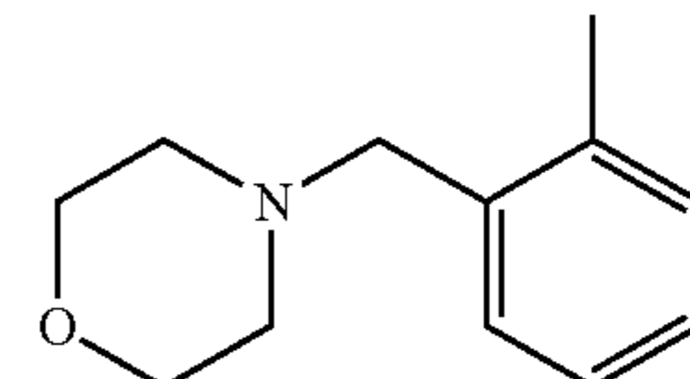
4-(2-methylbenzyl)morpholine
