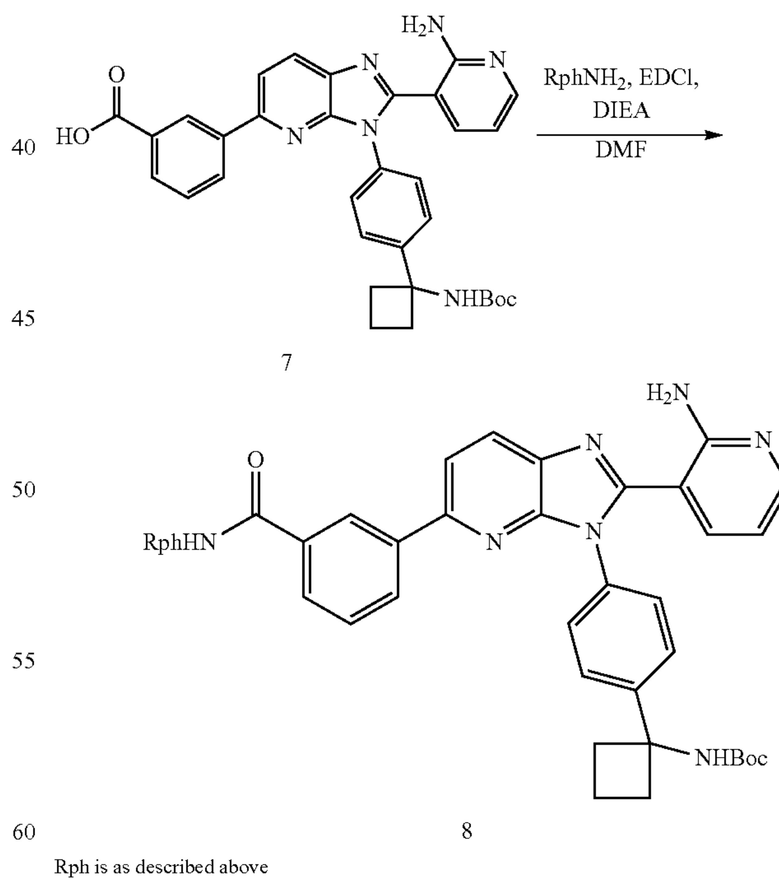
Scheme 3: Amide formation
