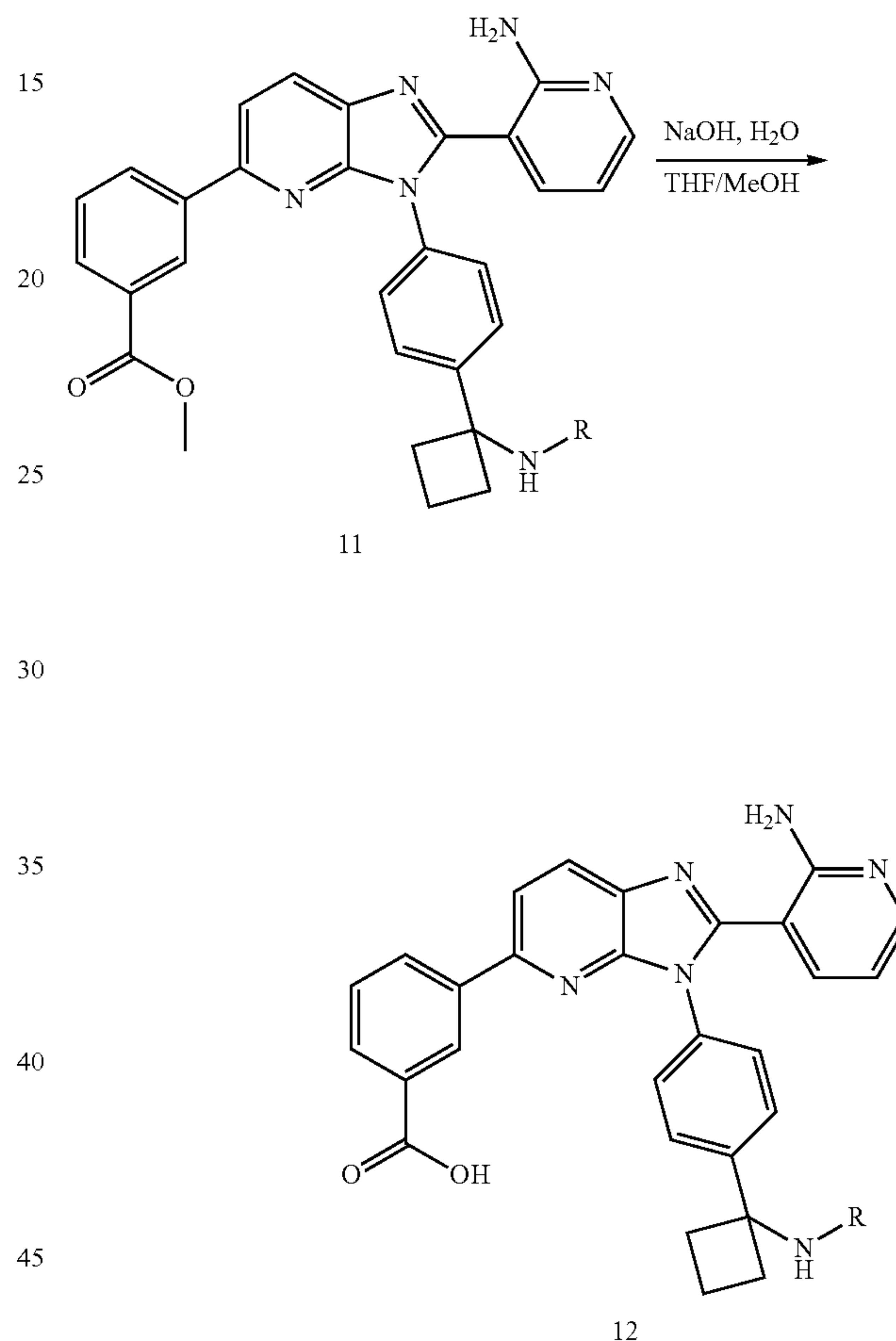
Scheme 5: Saponification
