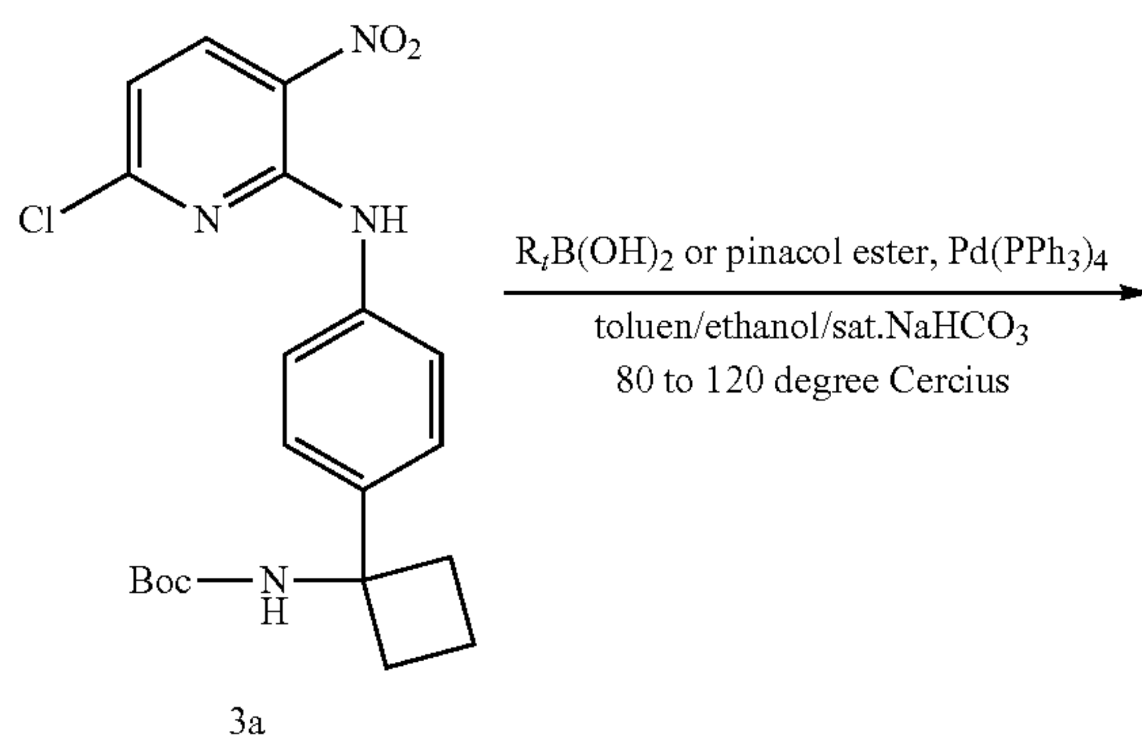
Scheme 6: Suzuki coupling 1
