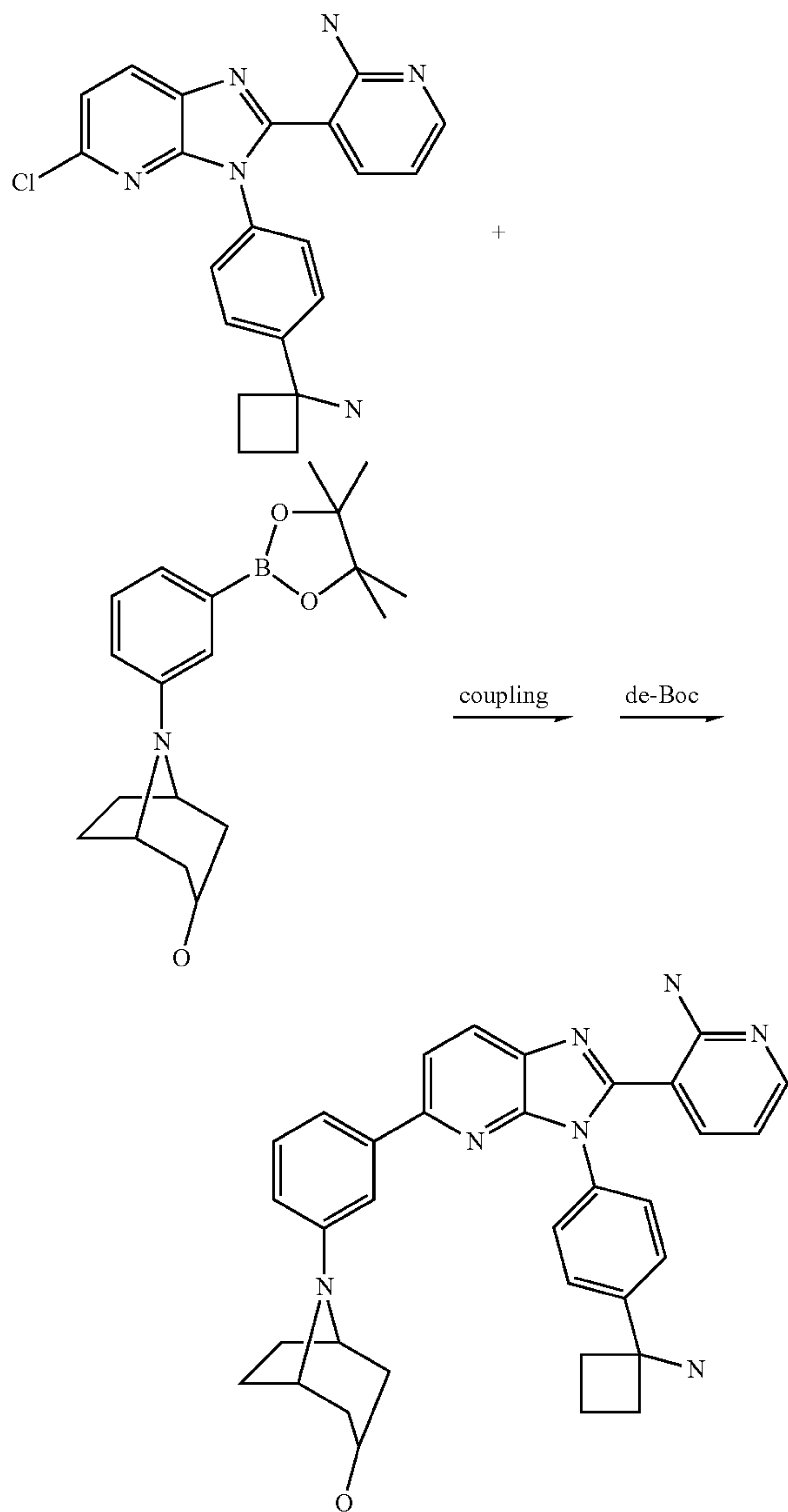
Step 2: Coupling
