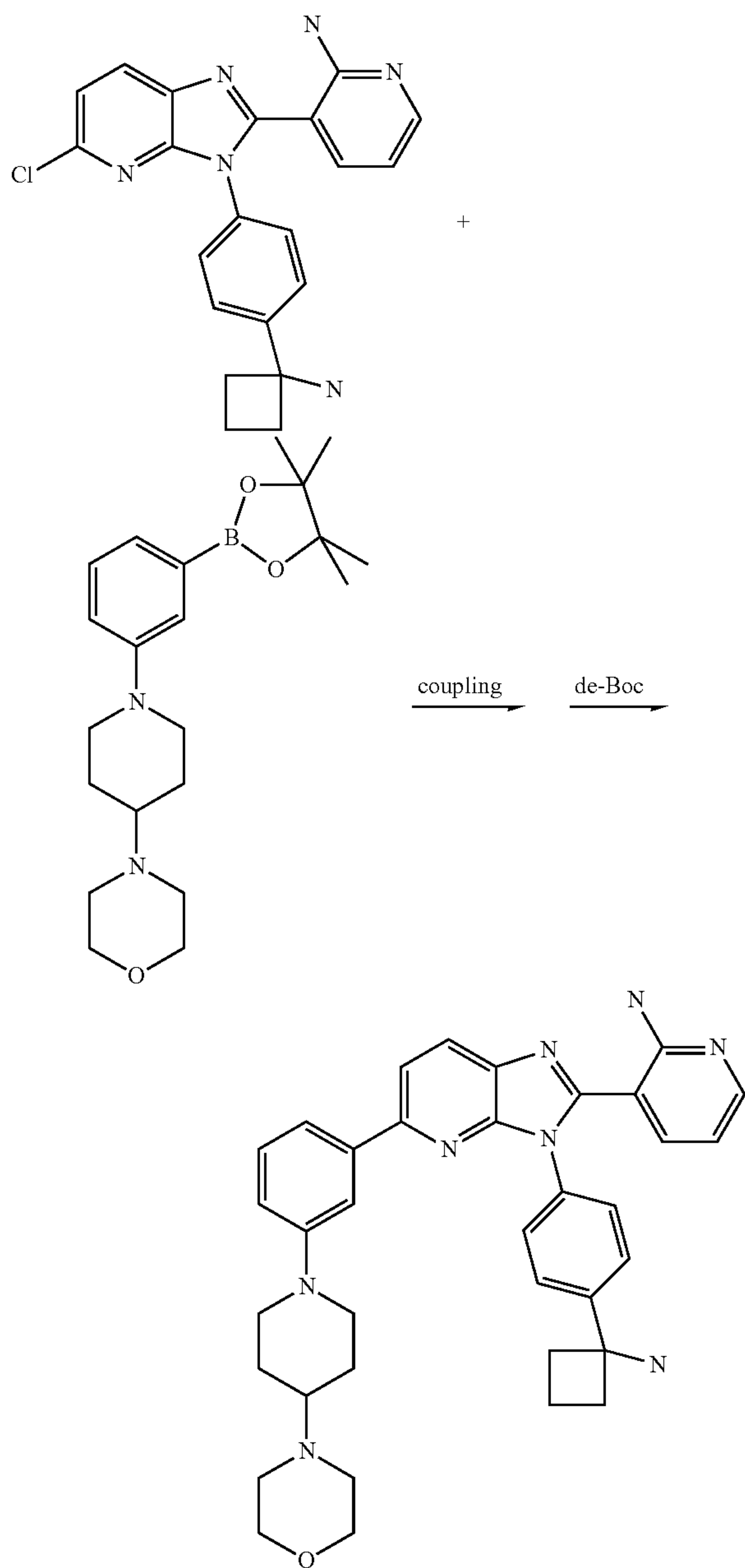
Step 2: Coupling
