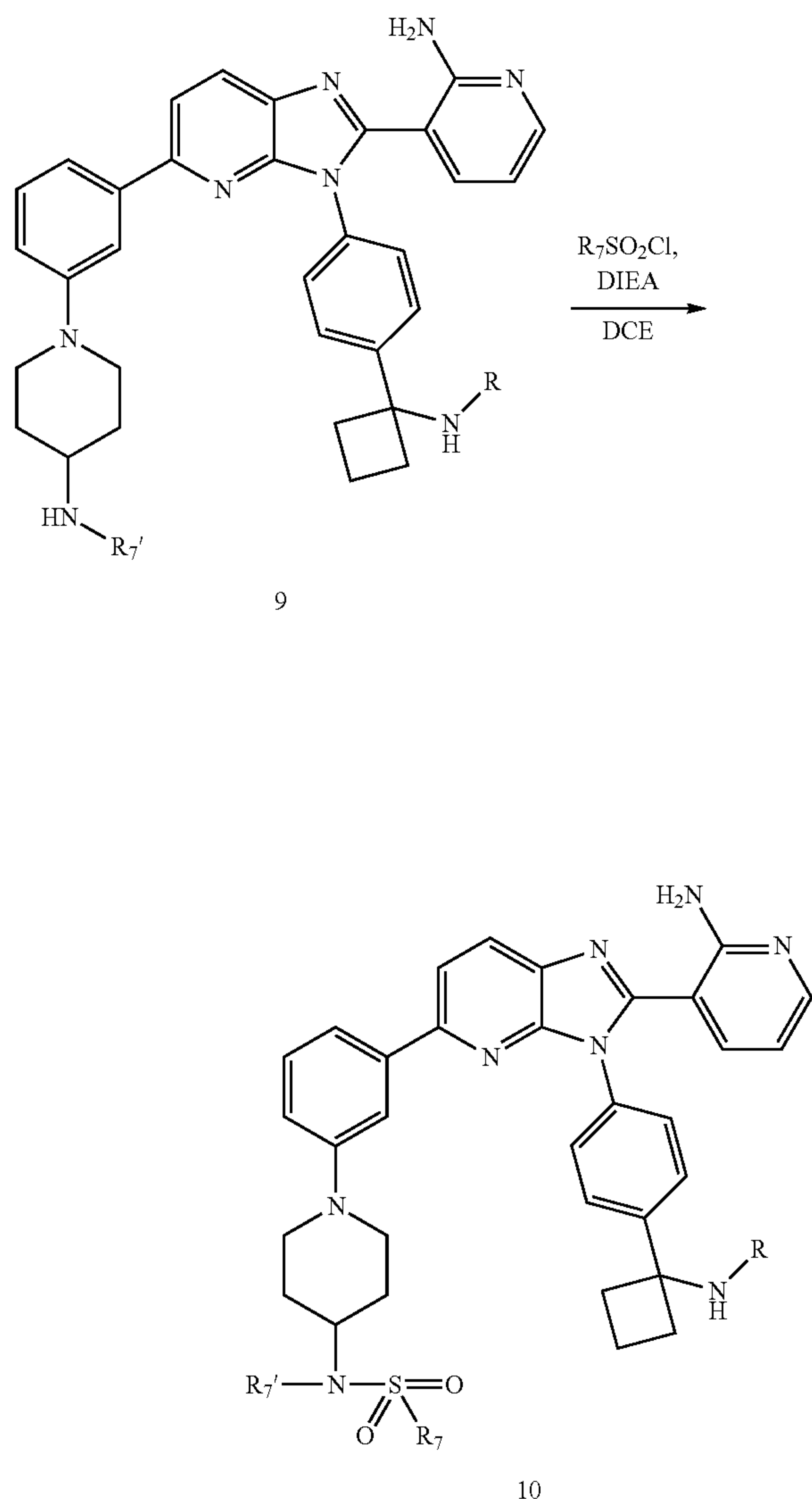
Scheme 4: Sulfonamide formation
