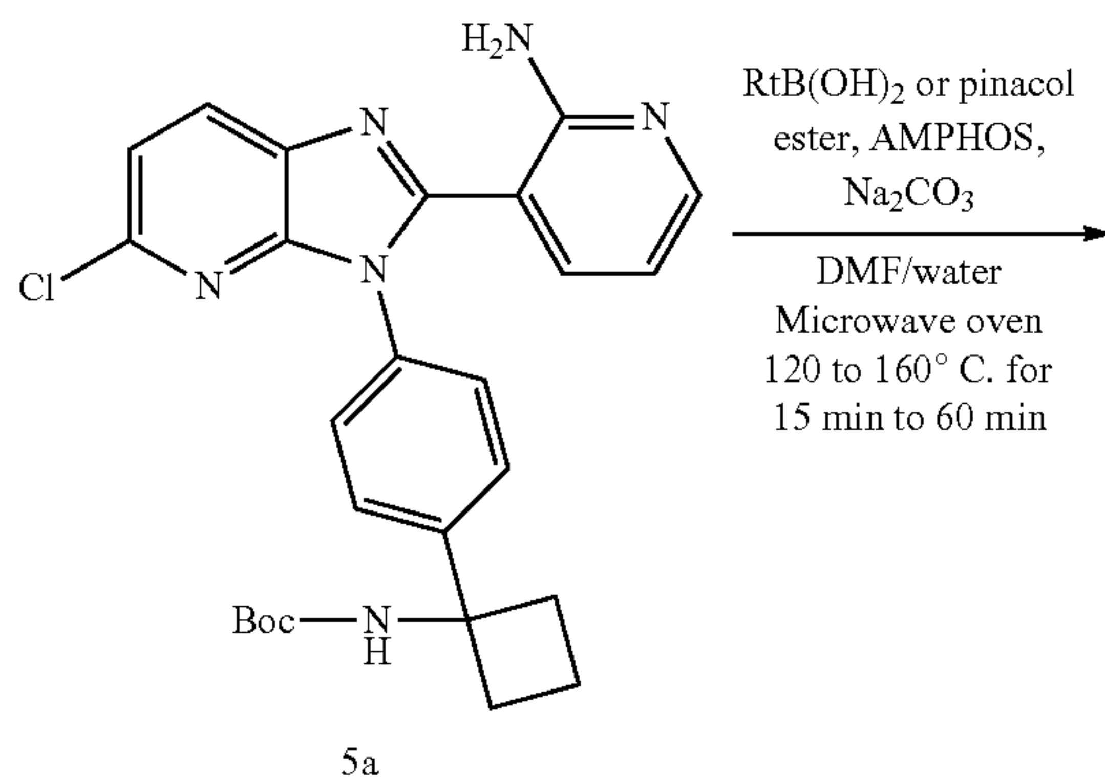
Scheme 7: Suzuki coupling 2
