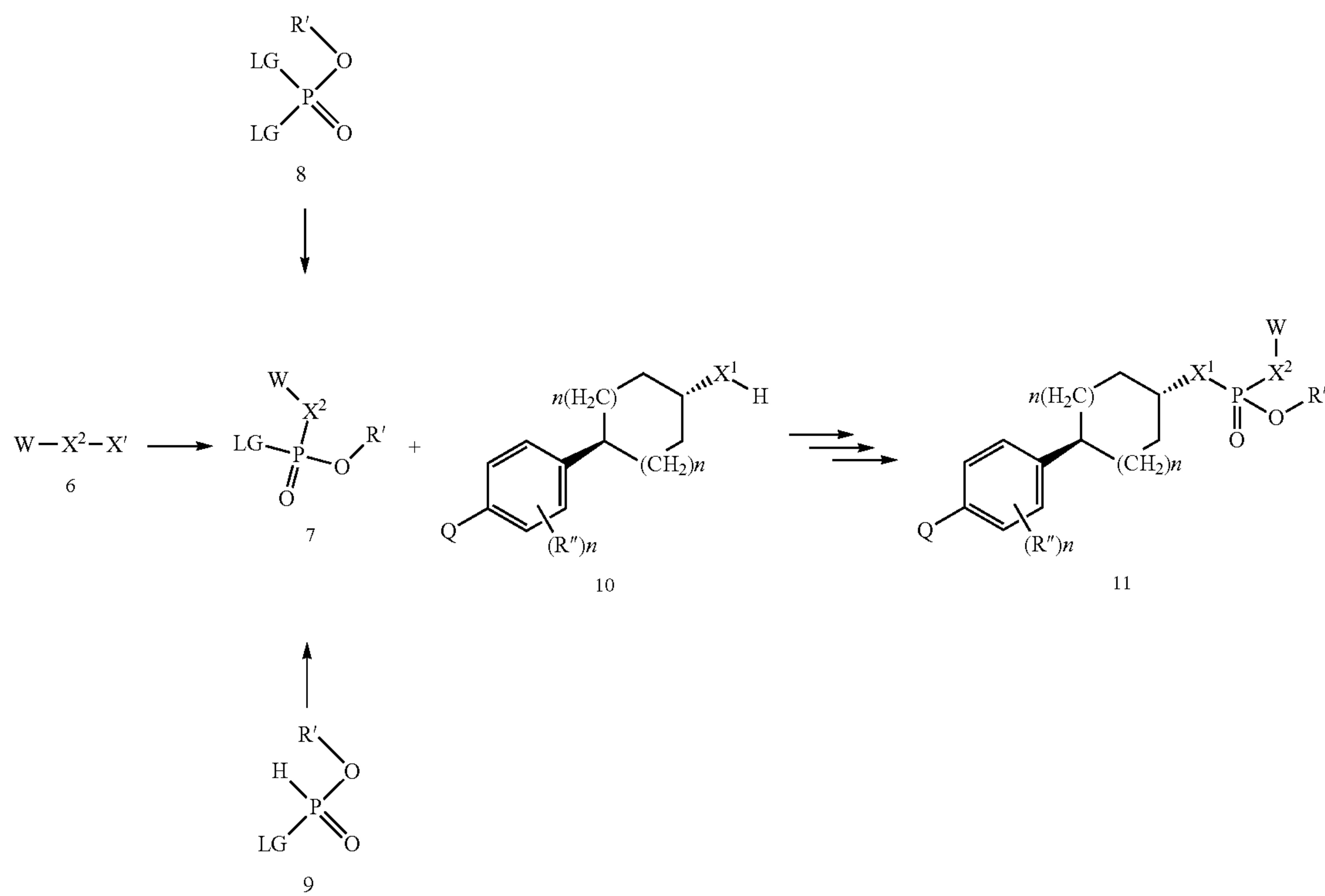
Scheme 2
