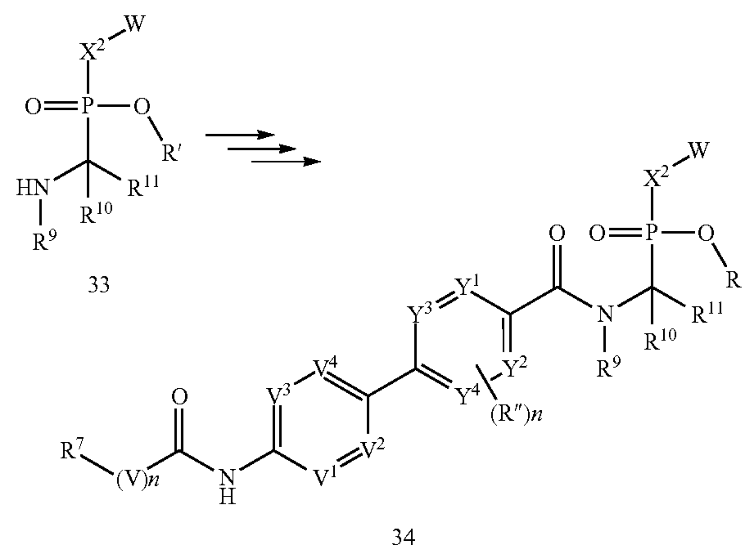
Scheme 8
