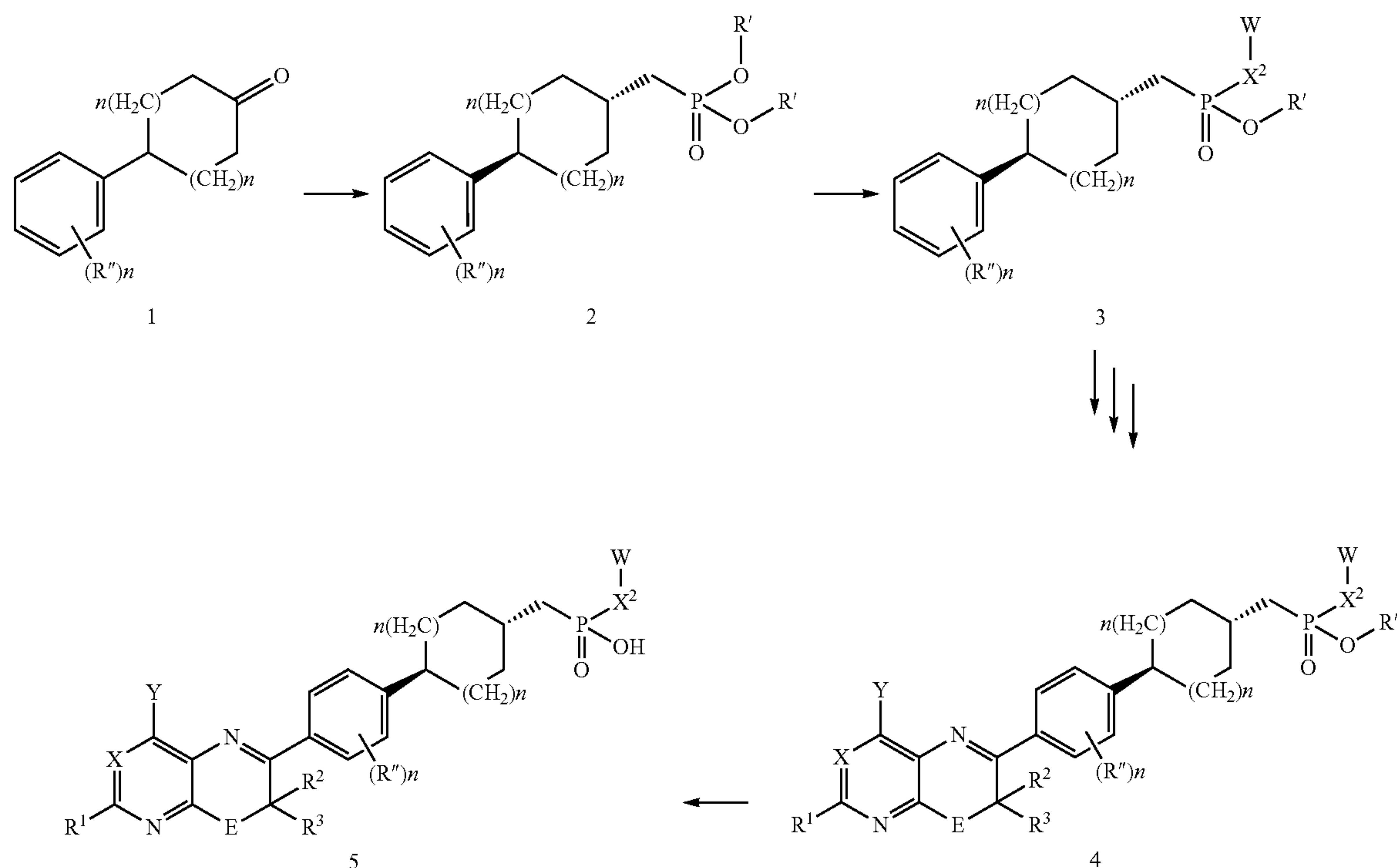
Scheme 1
