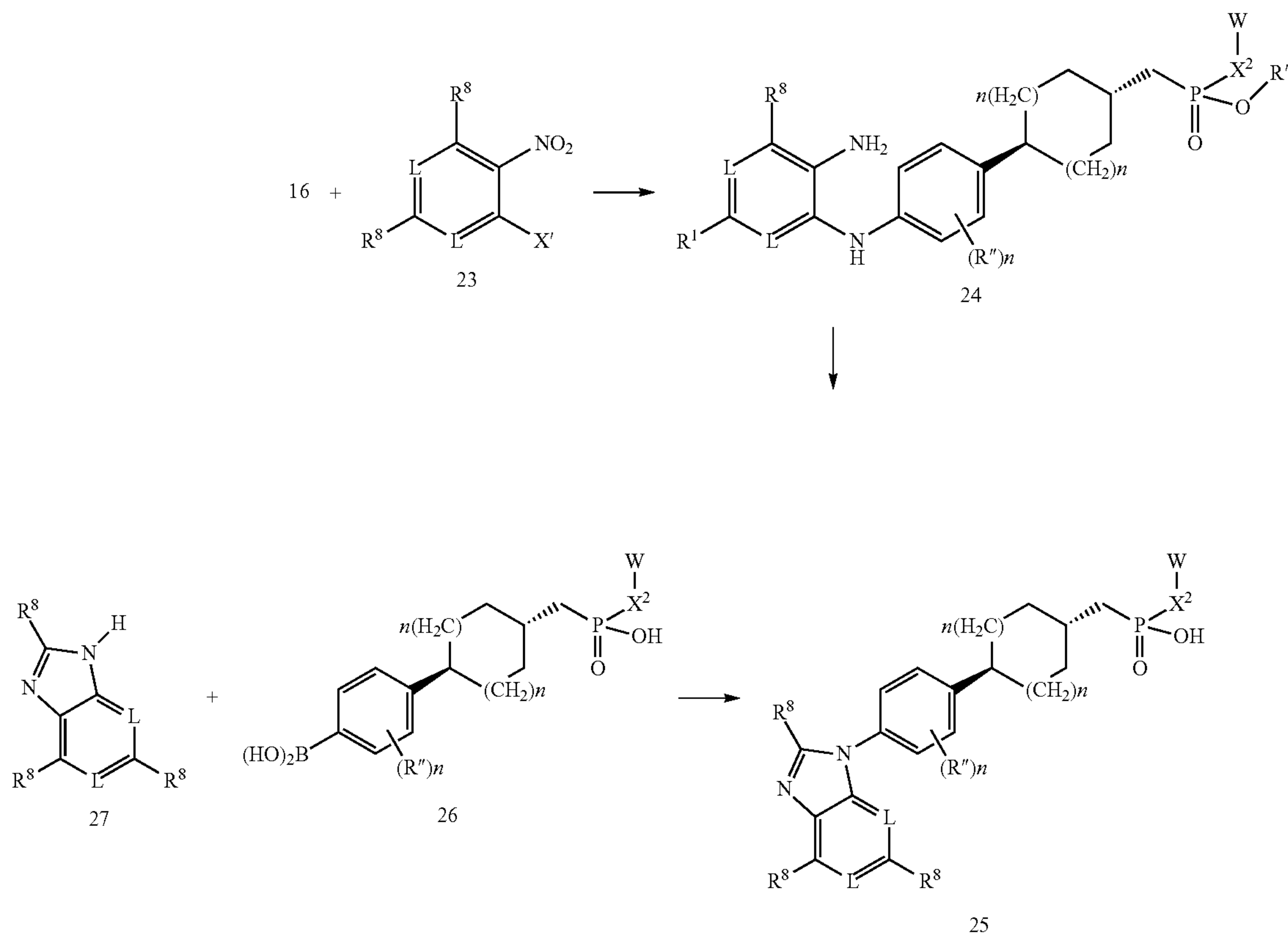
Scheme 6
