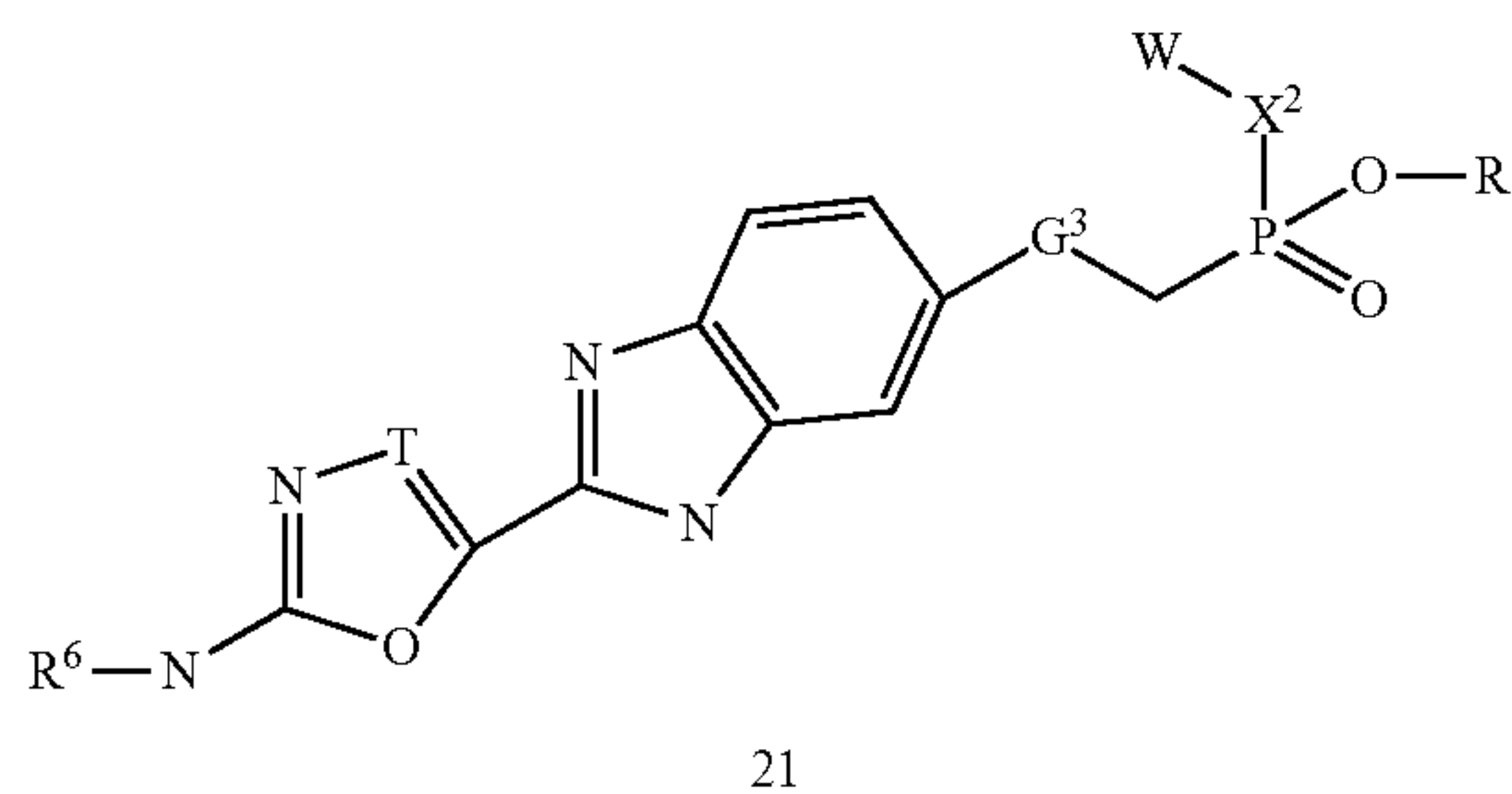
Scheme 5
