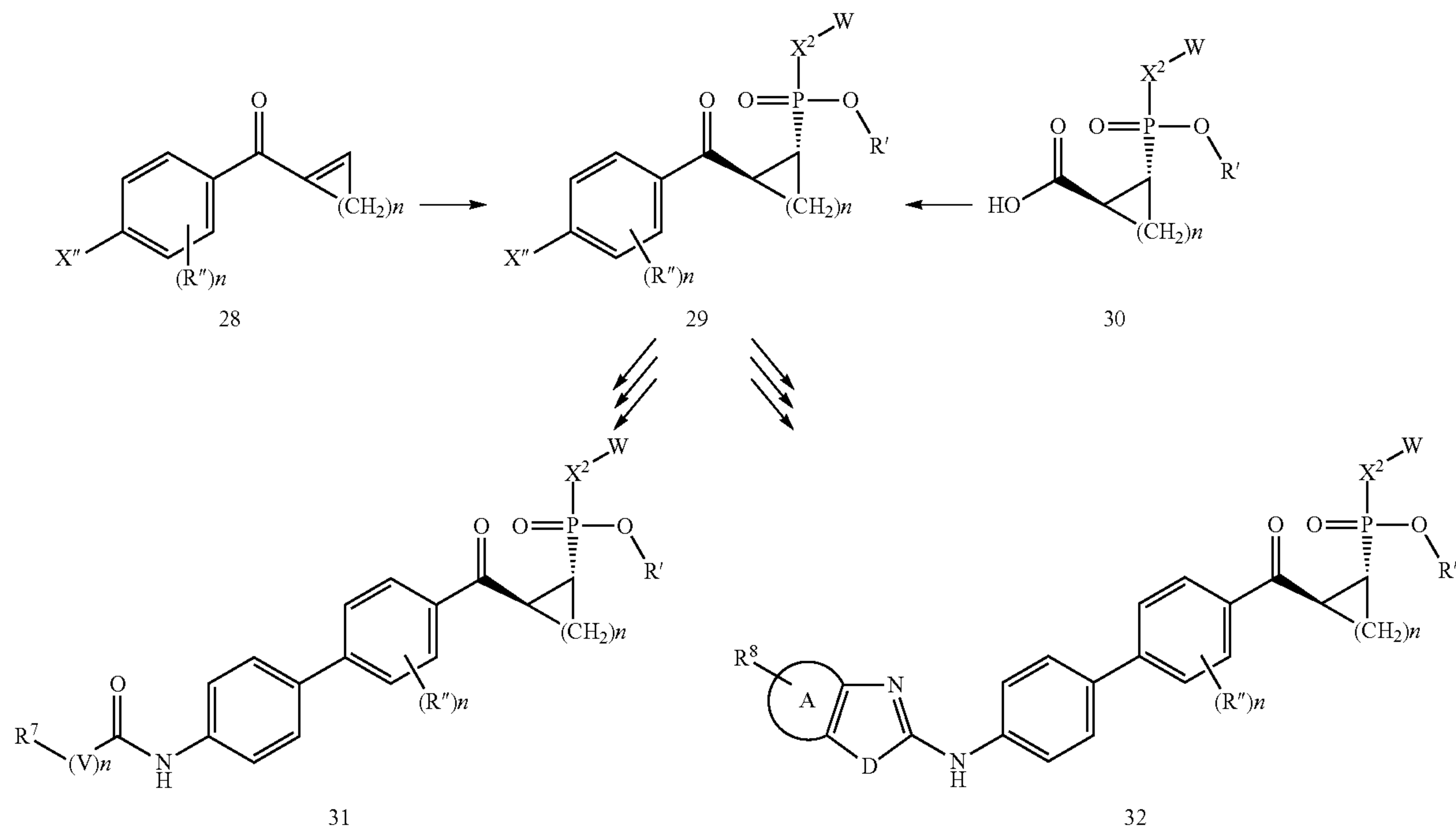
Scheme 7
