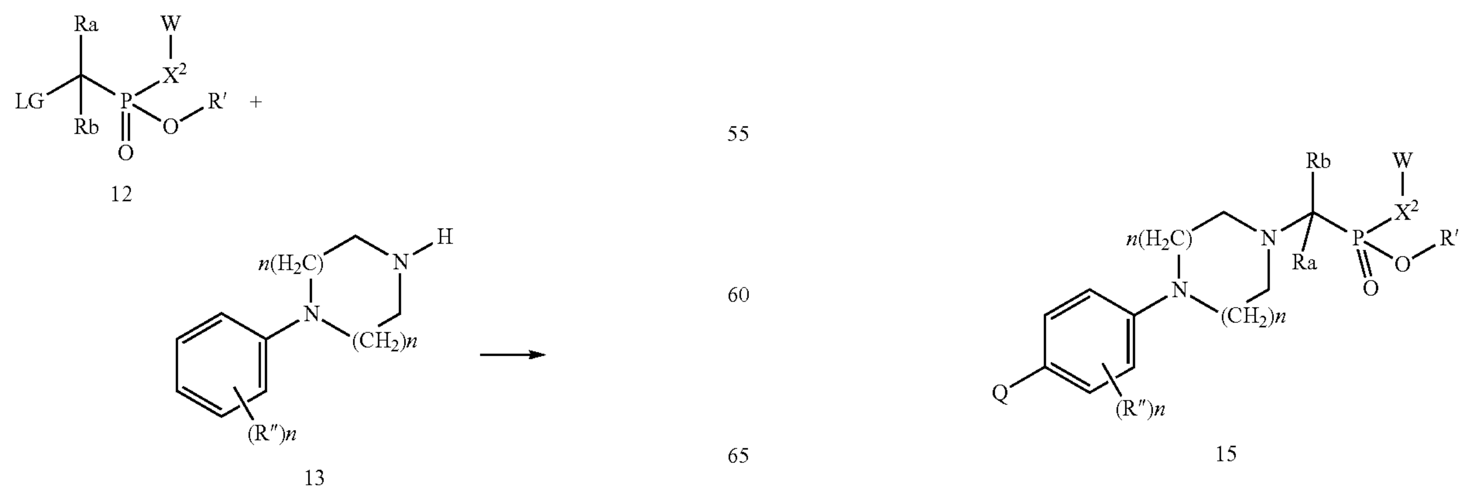
Scheme 3
