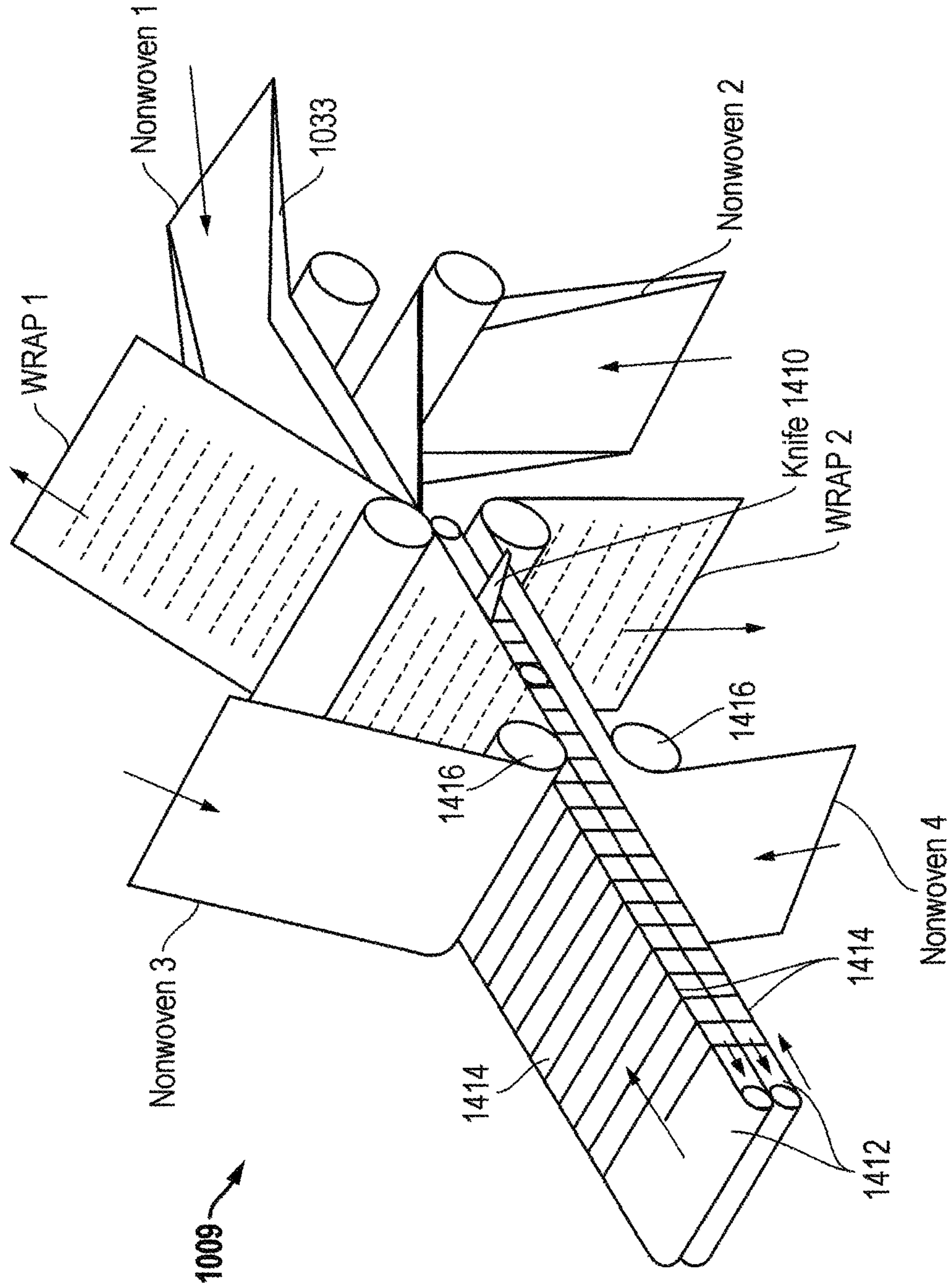
FIG. 10 (PRIOR ART)
