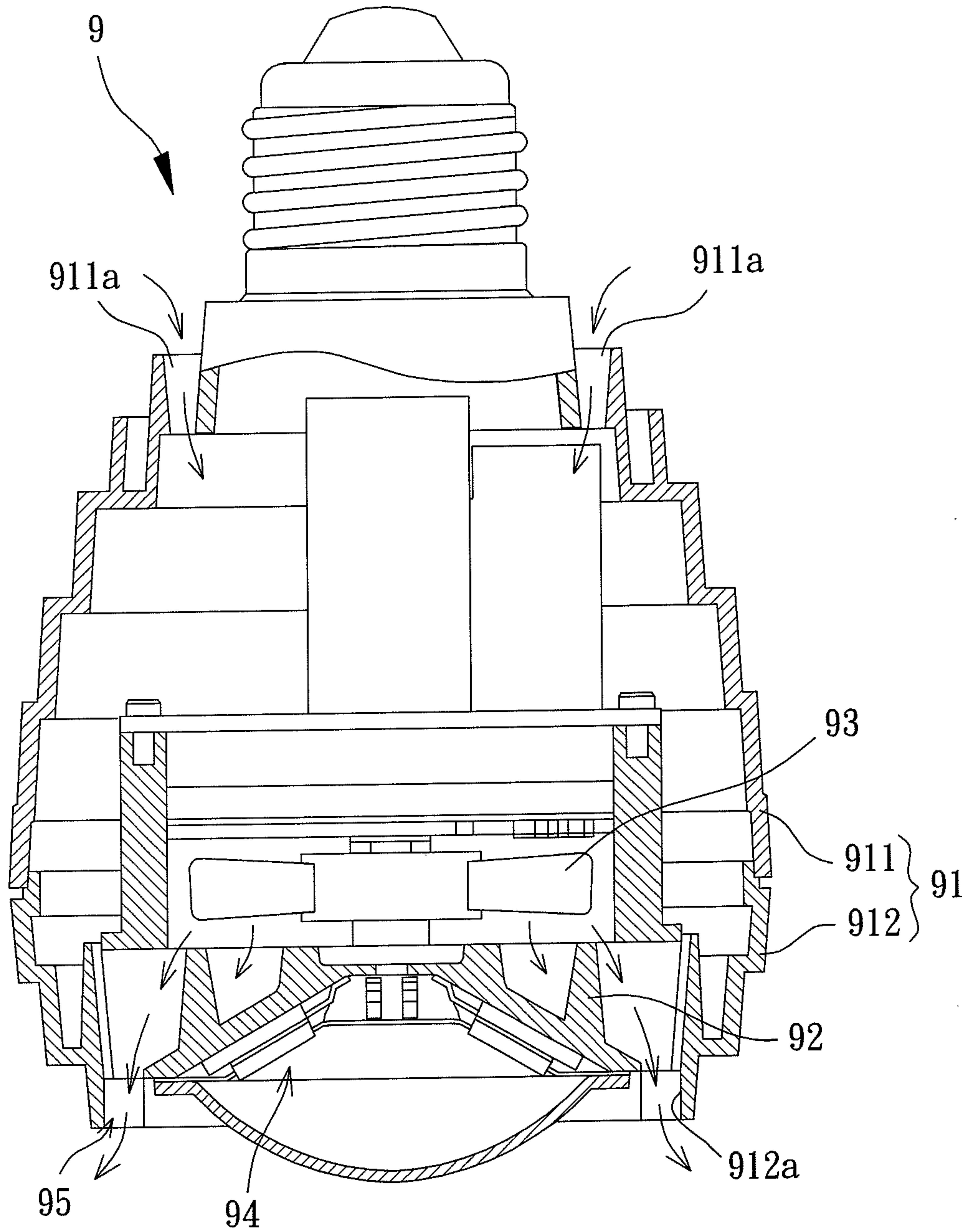
FIG. 2 PRIOR ART
