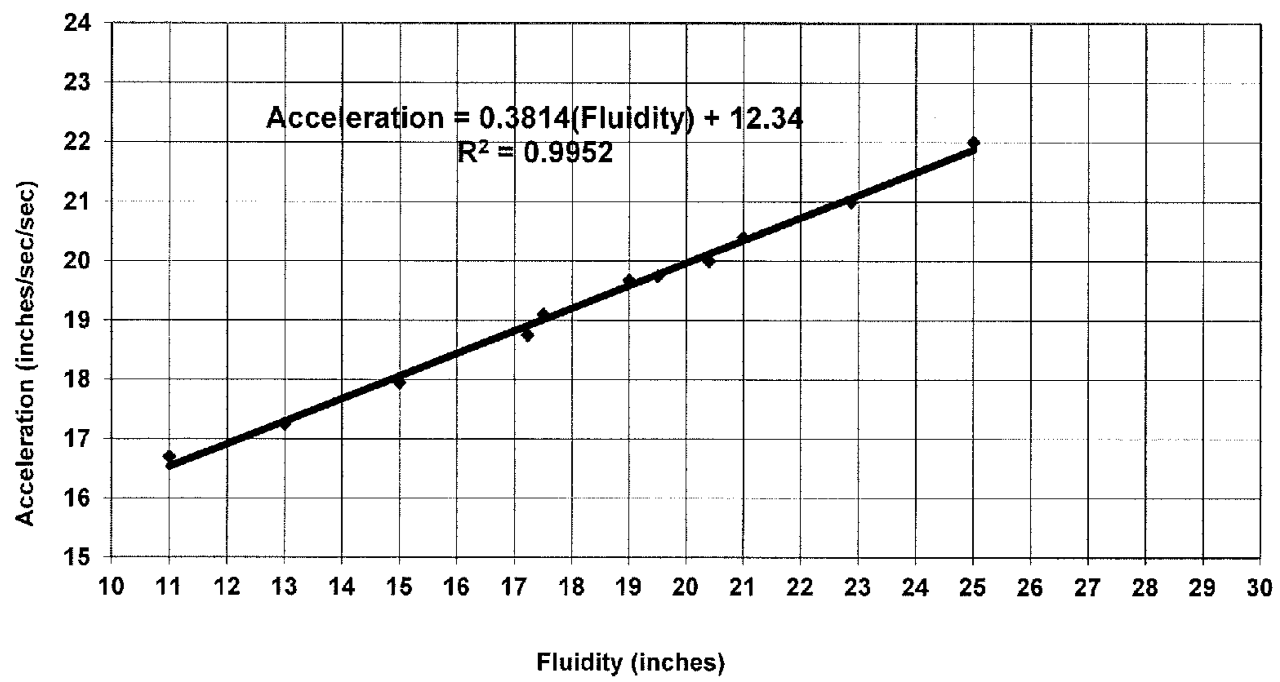
FIG 5B Bell Acceleration Equation
