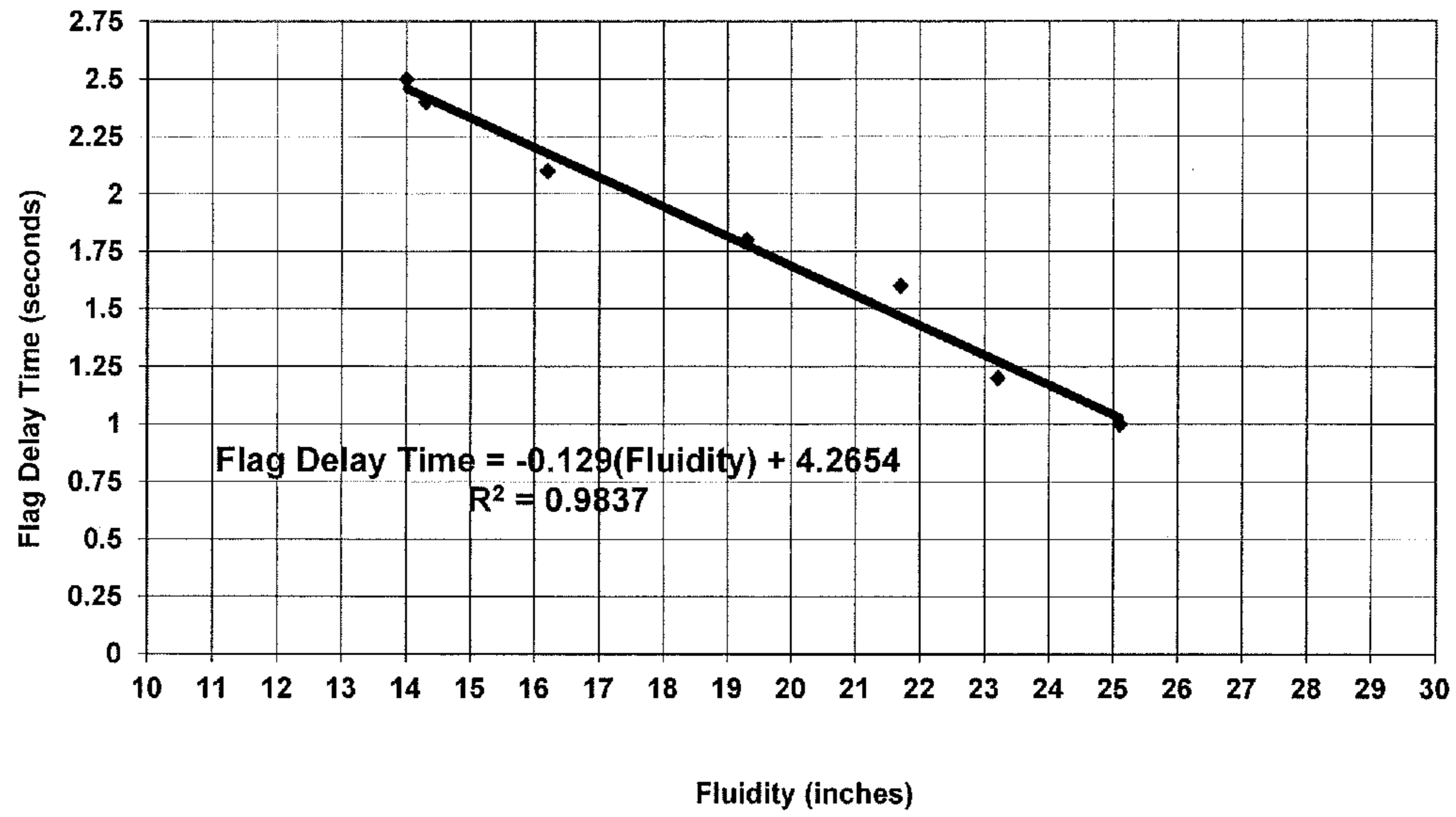
FIG 5A Flag Delay Time Equation
