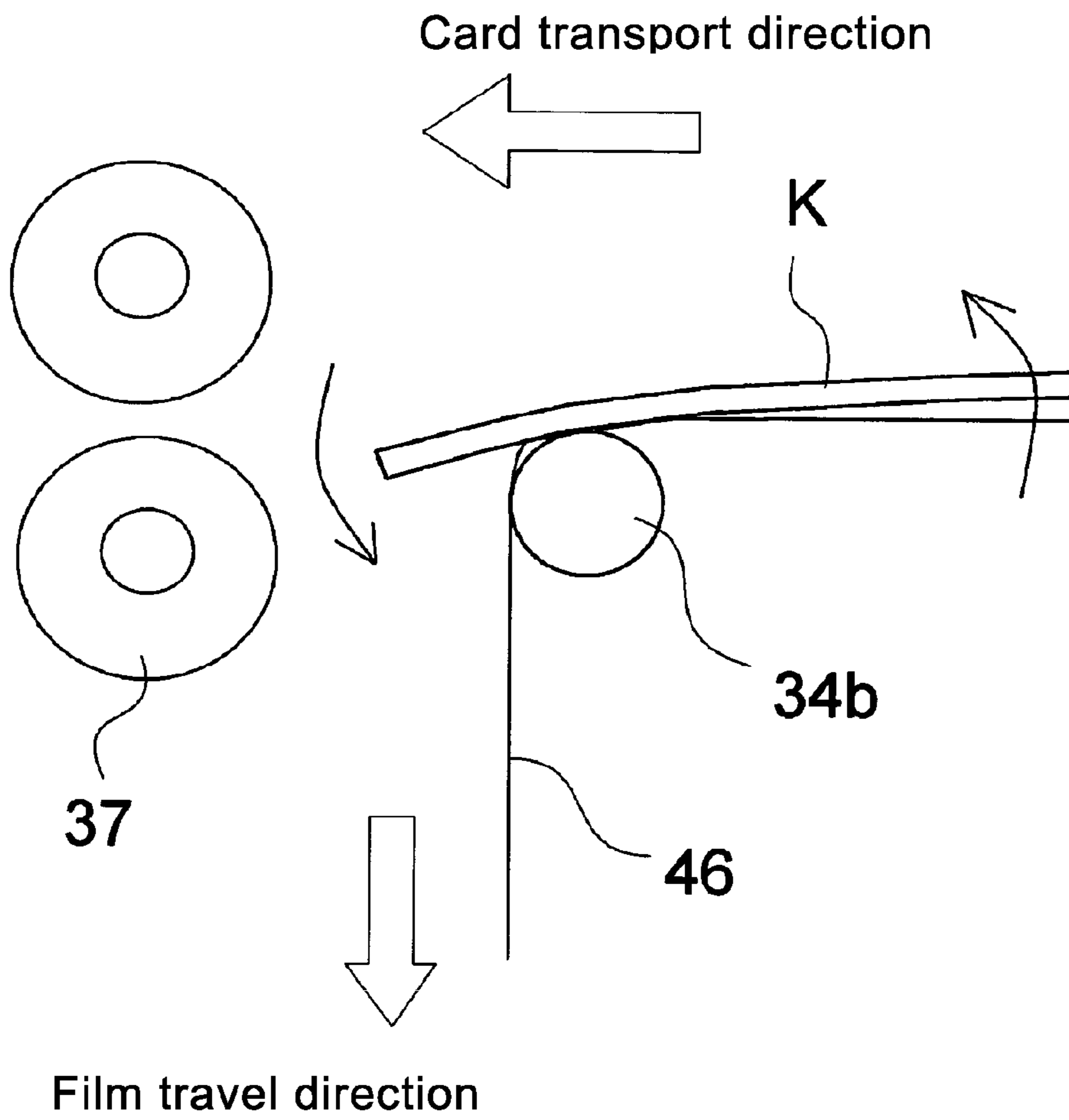
FIG. 17 PRIOR ART
