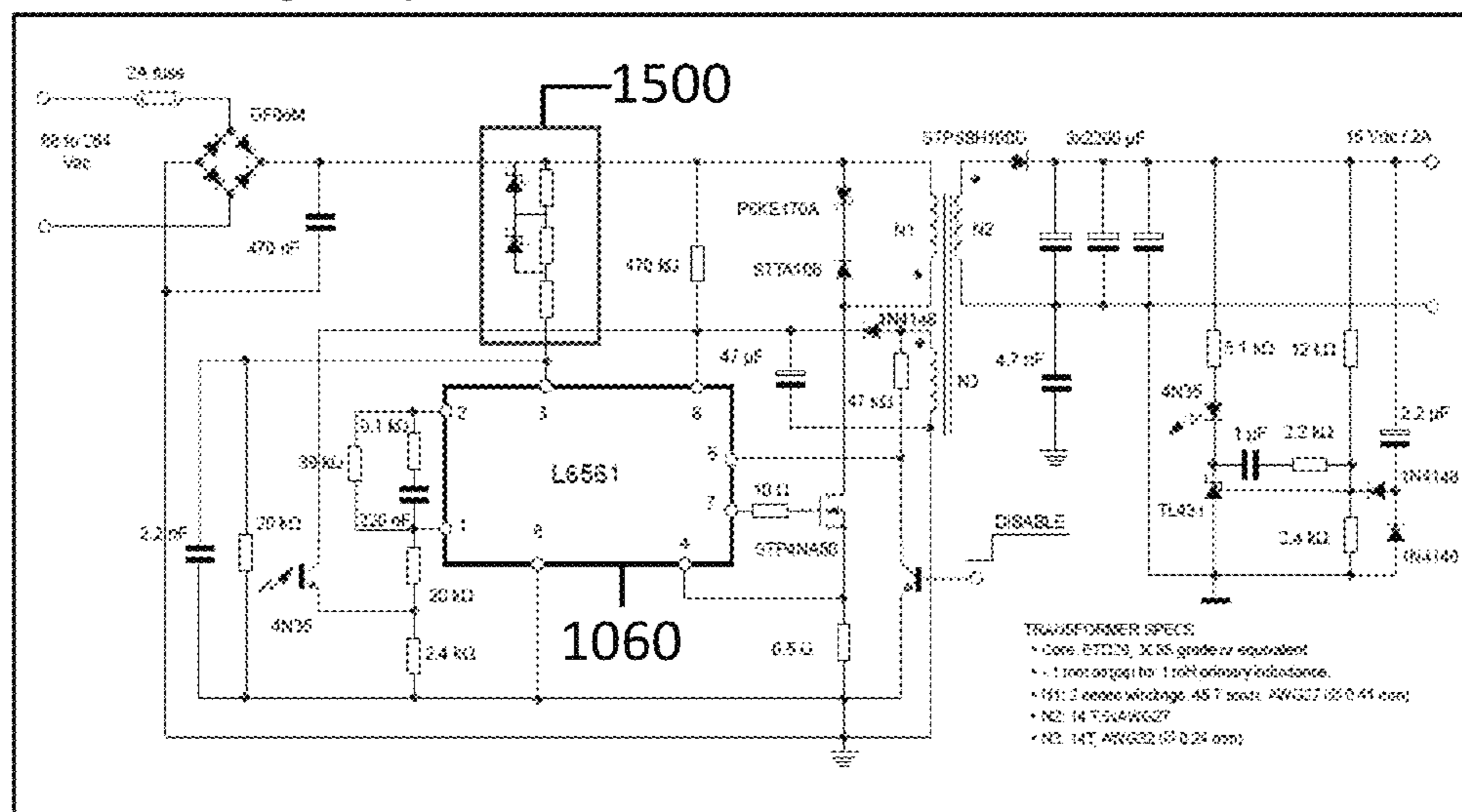
Improved High-PF Flyback with the L6561: electrical schematic with Zener ladder
