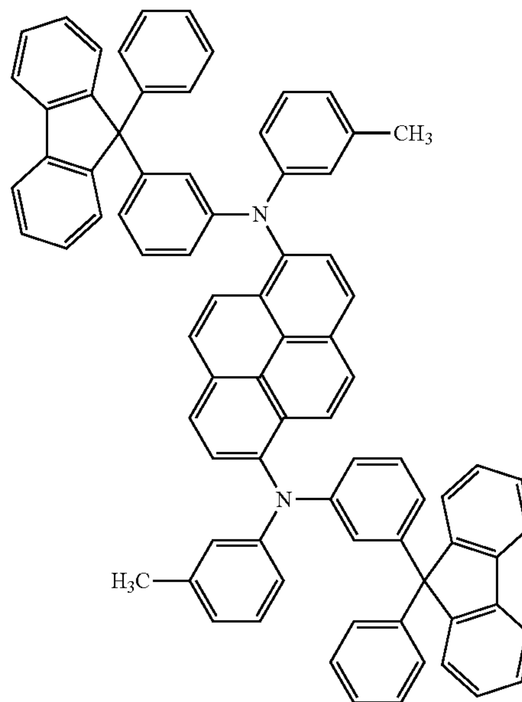
1,6mMemFLPAPrn
