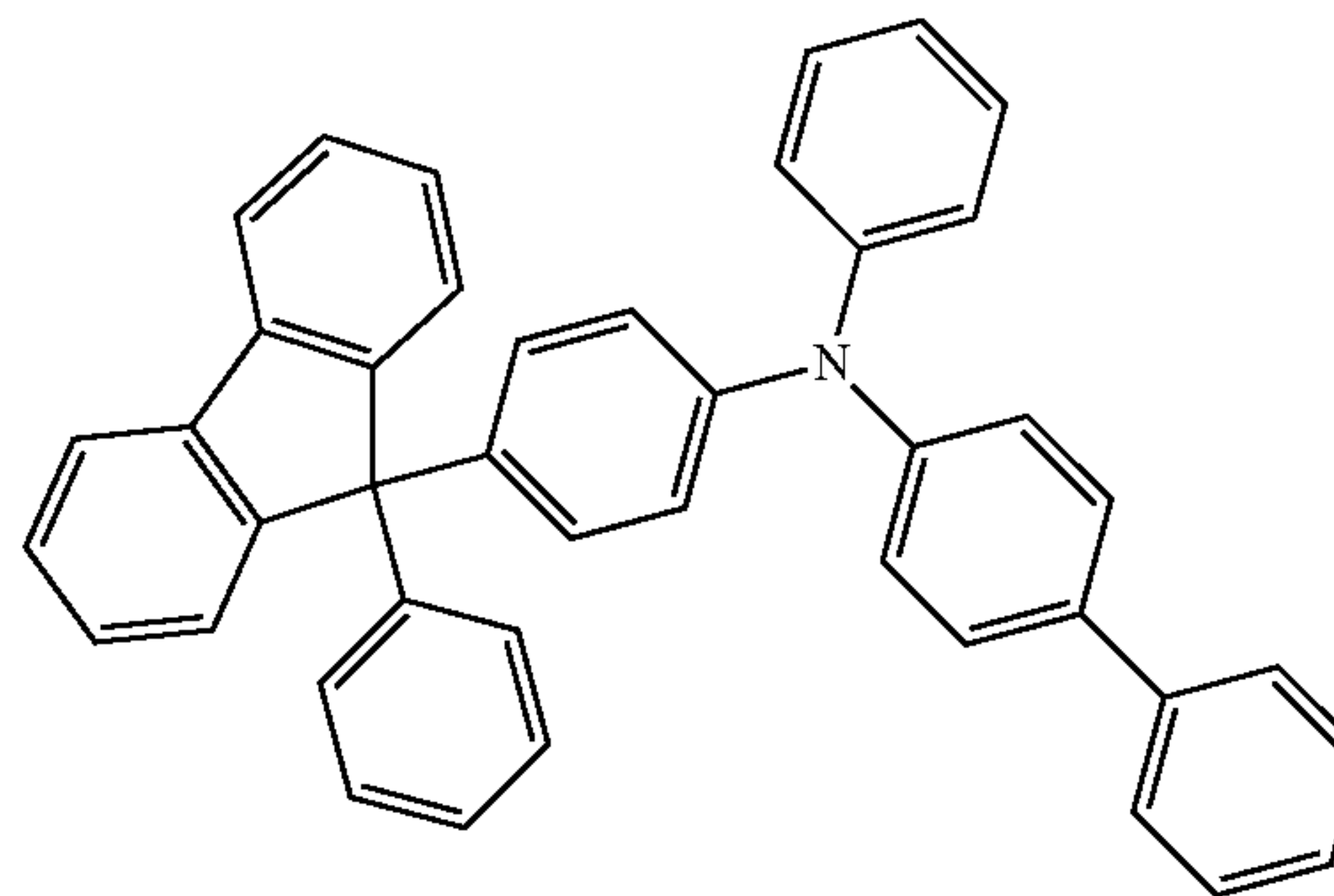
BPAFLP
