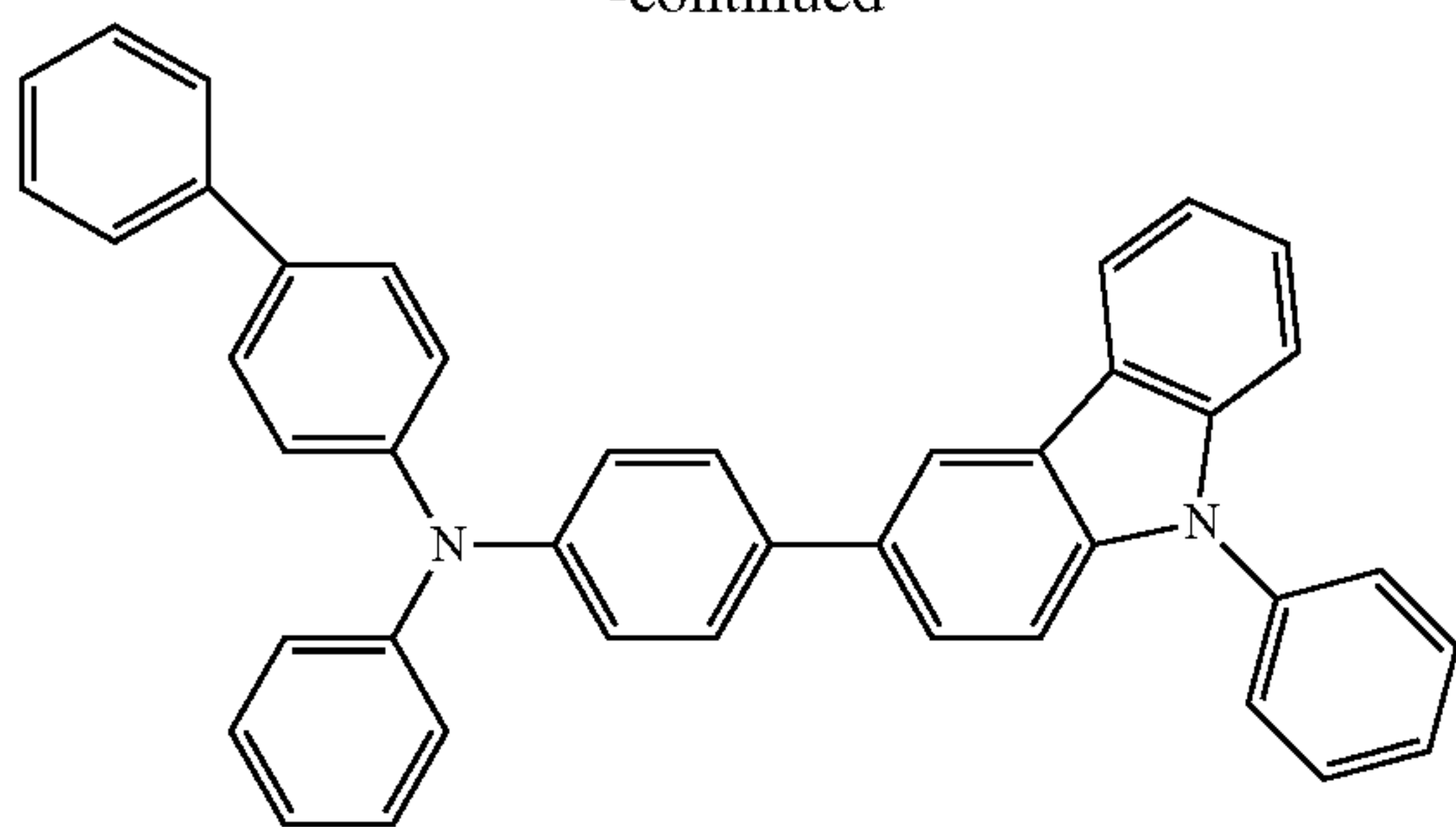
PCBA1BP
