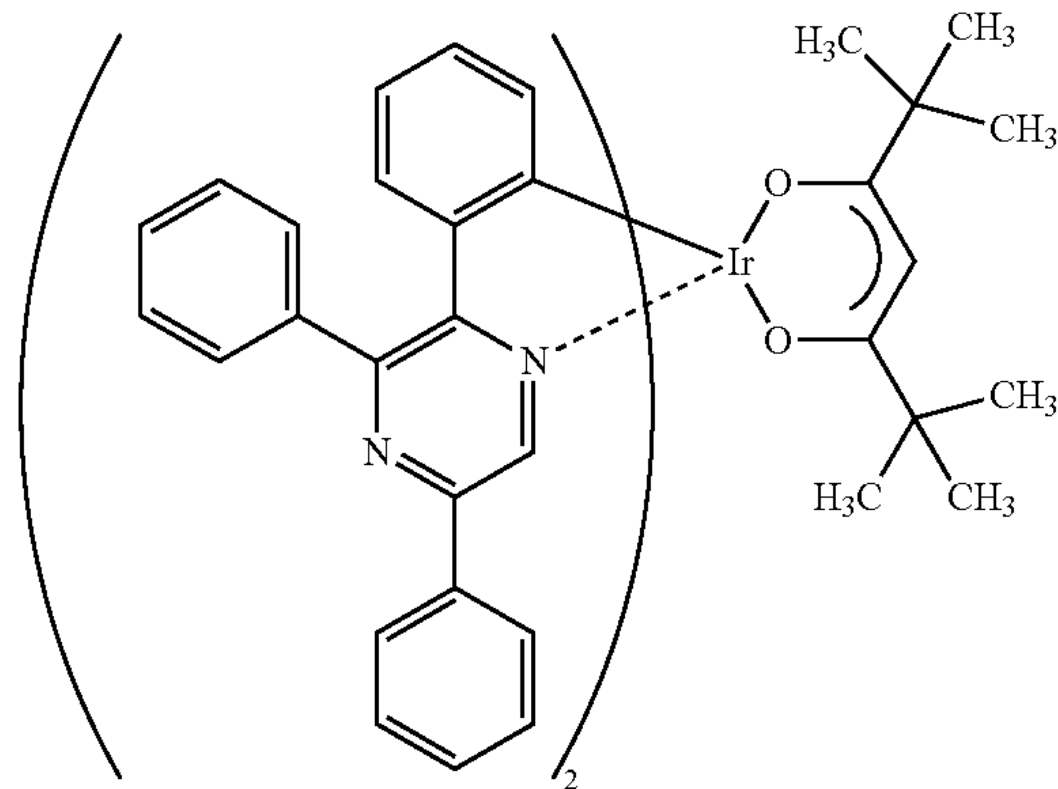
Ir(tppr) 2 (dpm)
