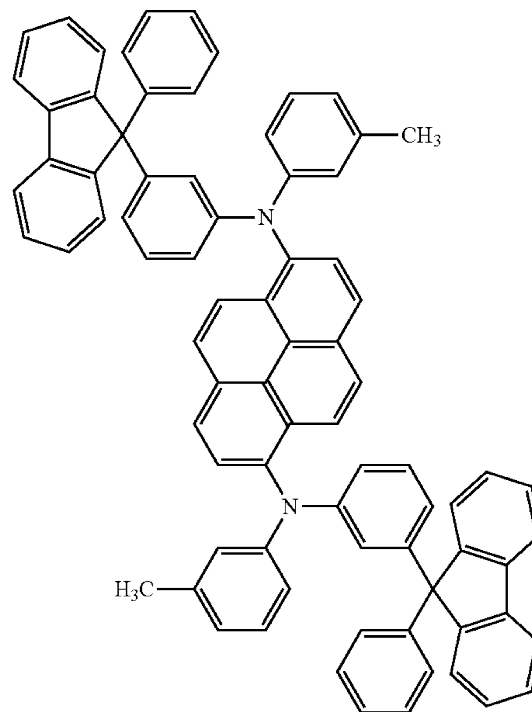
1,6mMemFLPAPrn
