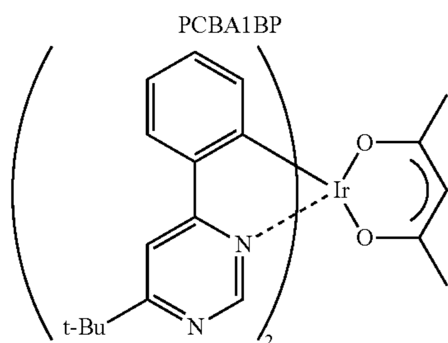
Ir(tBuppm) 2 (acac)
