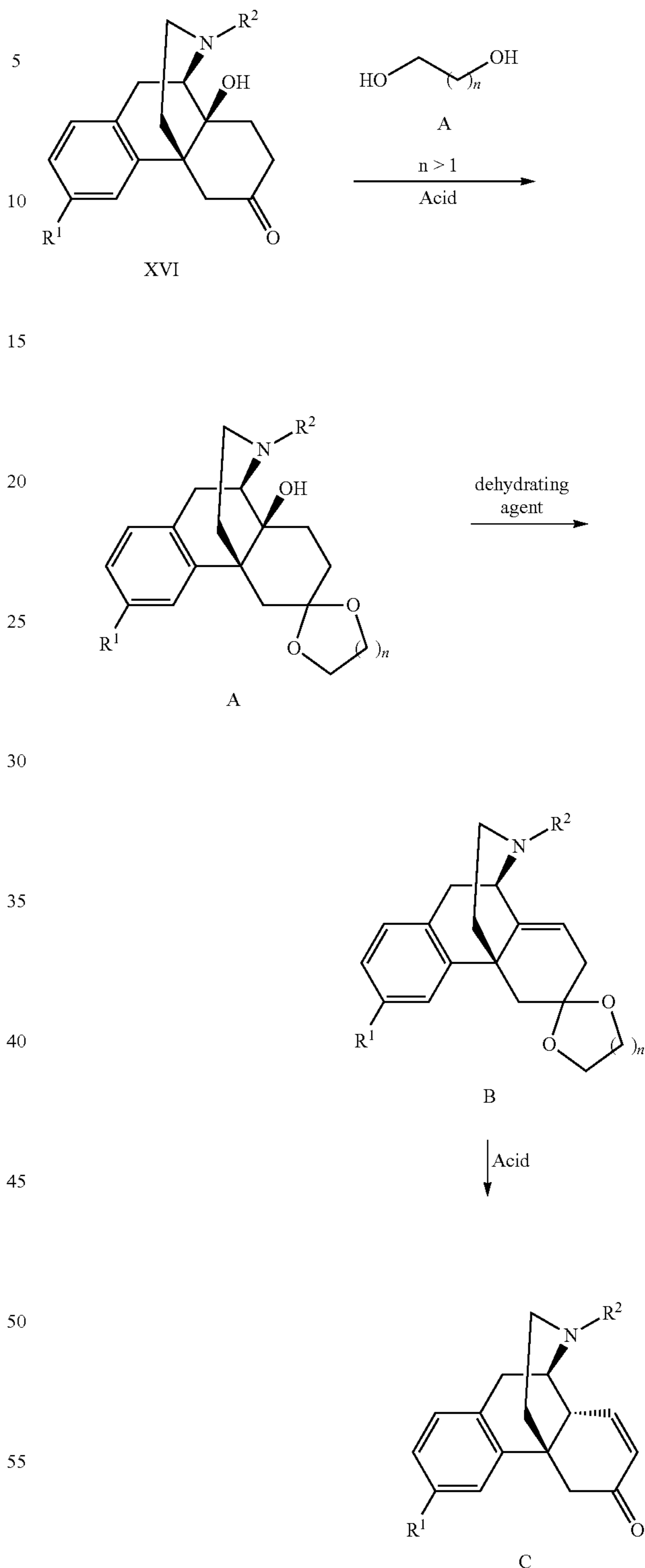
Scheme 1
