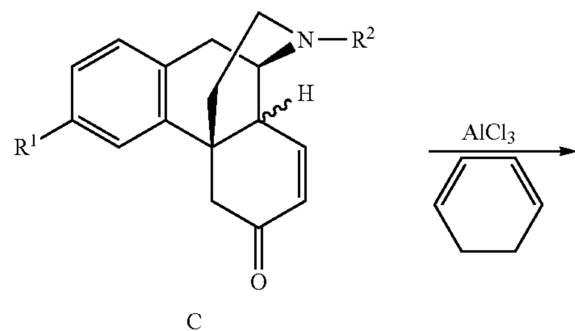
Scheme 4
