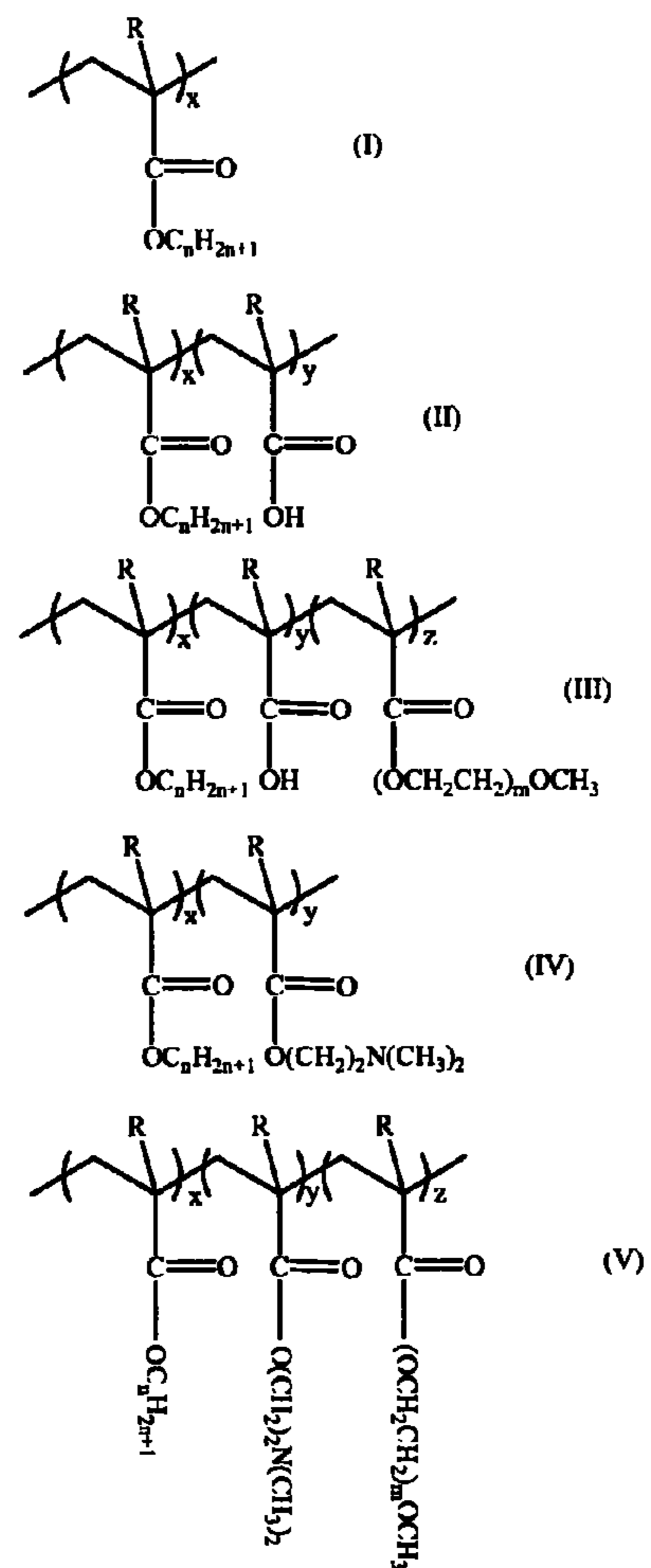
Figure 41 General chemical structure of CYSC polymers (R=H or CH 3 , n ≥ 12, m ≥ 2)
