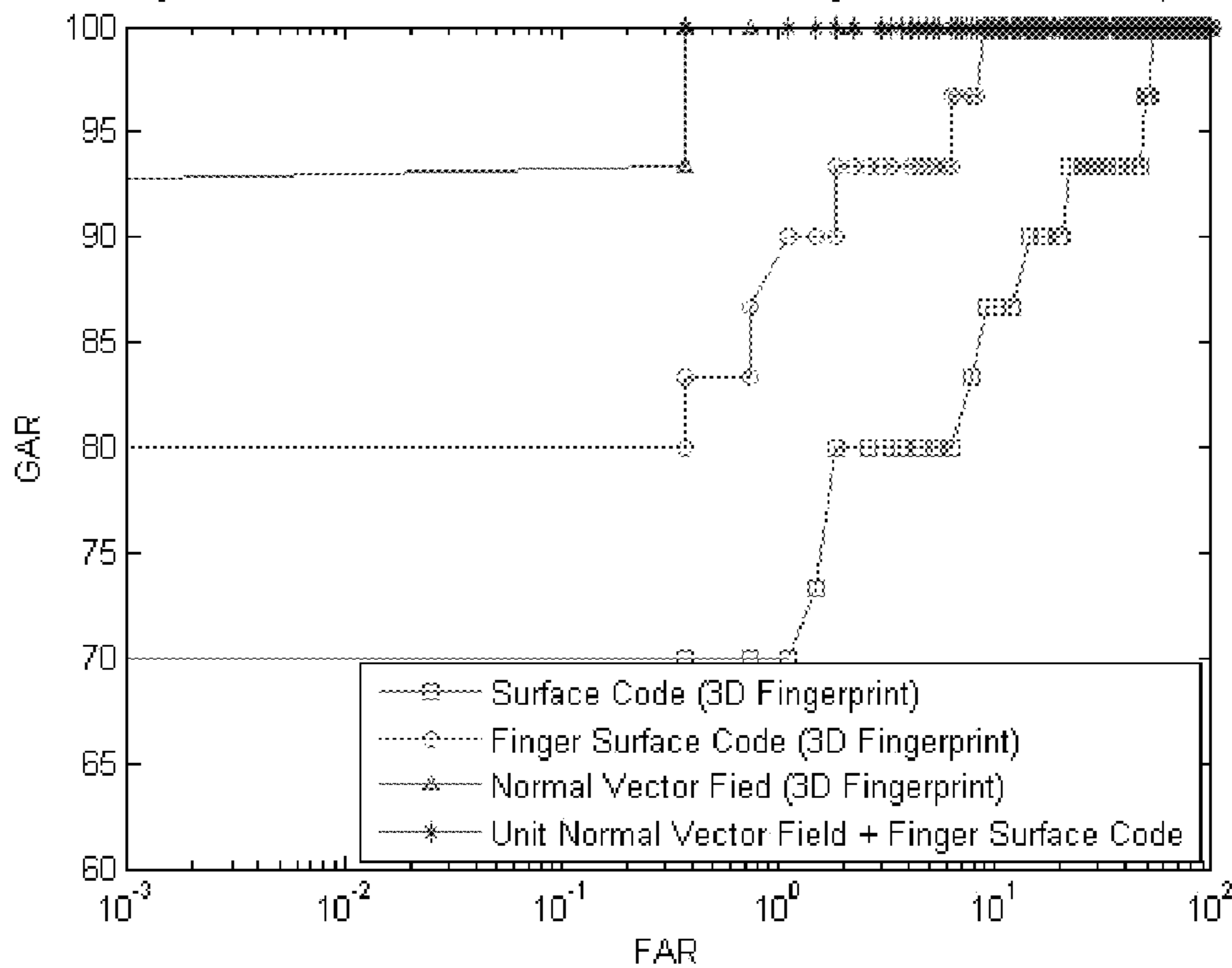
ROC from Finger Surface Code, Unit Normal Vector Matching and its Combination (10 Clients)
