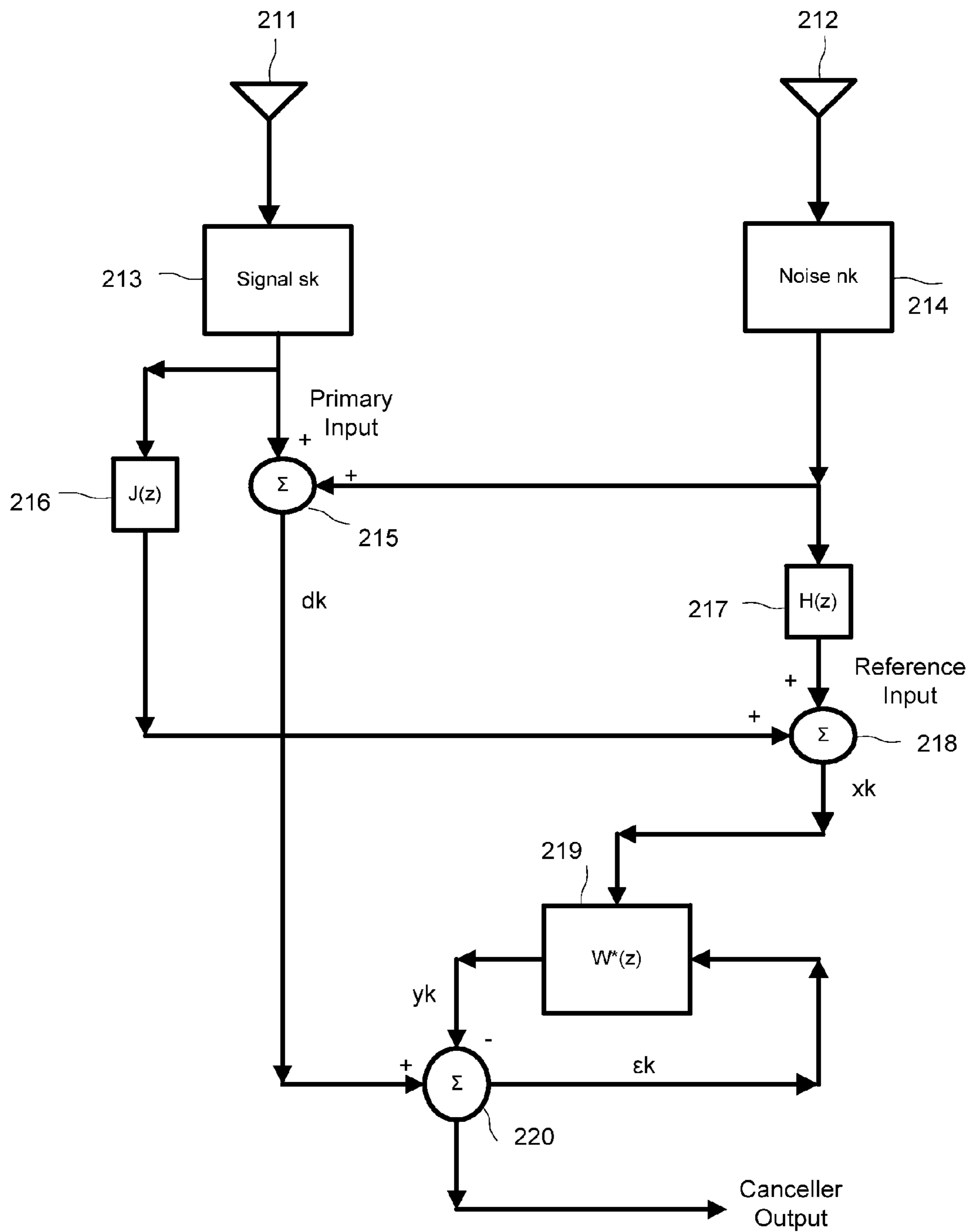
FIG. 2 PRIOR ART
