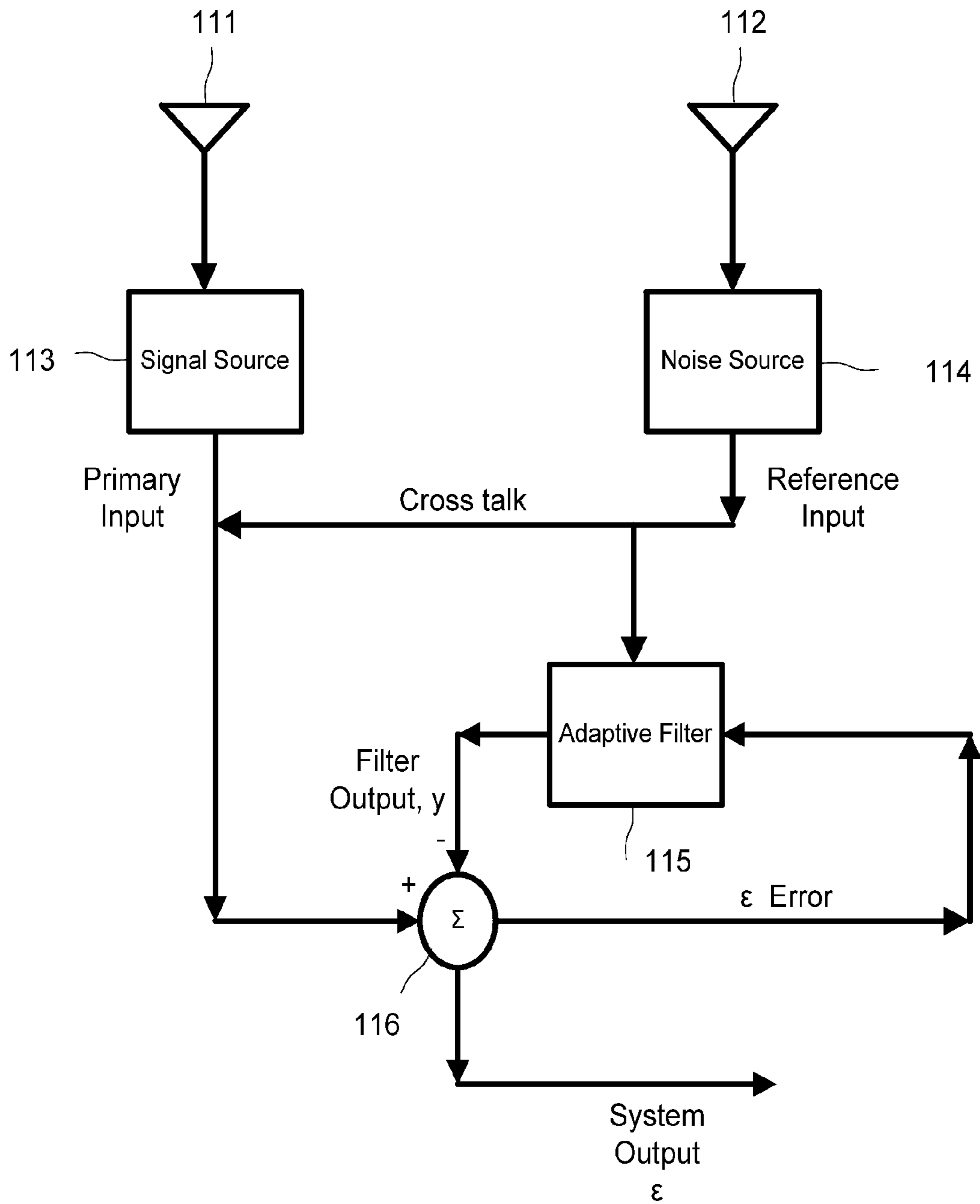
FIG. 1 PRIOR ART
