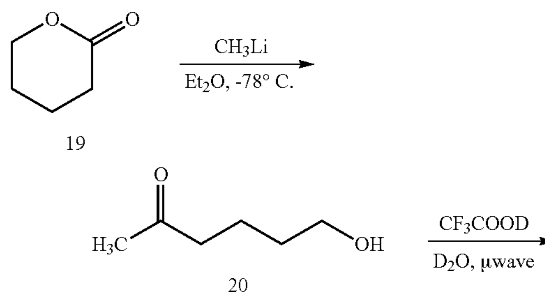
Scheme 3. Synthesis of Intermediate 11a- d_5
