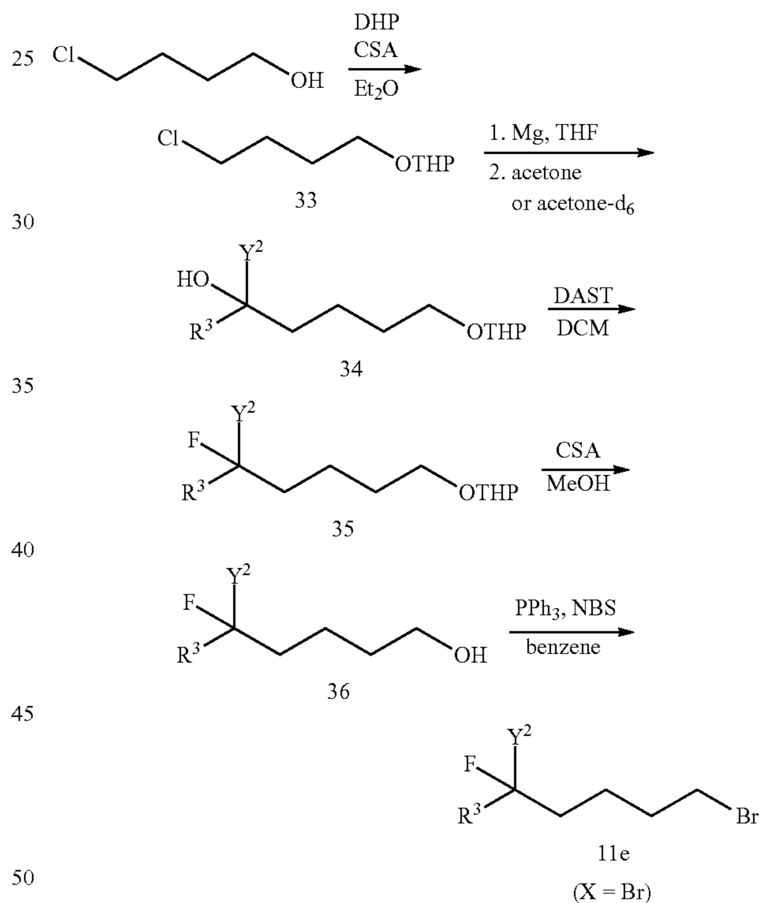
Scheme 6. Synthesis of Intermediate 11e (X = Br)
