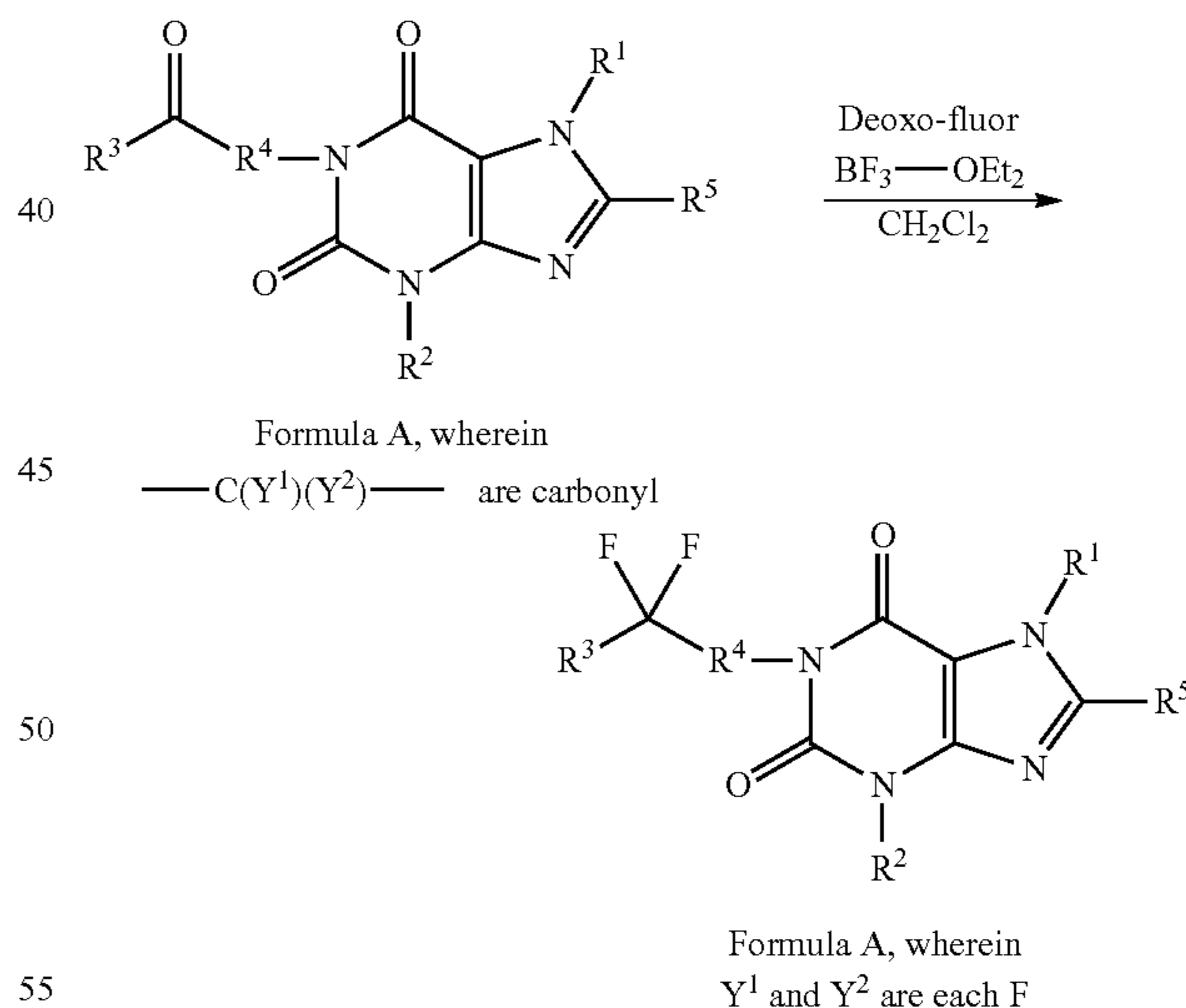
Scheme 12b. Alternative Synthesis of Compounds of Formula A, wherein Y 1 and Y 2 are each Fluorine.
