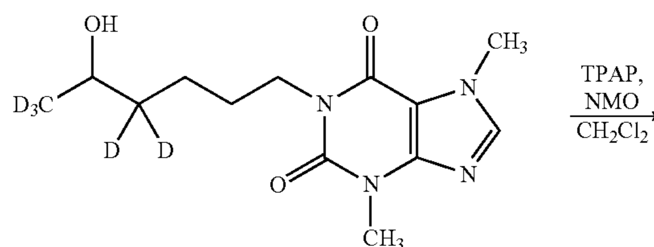
Scheme 23. Preparation of Compound 107.
