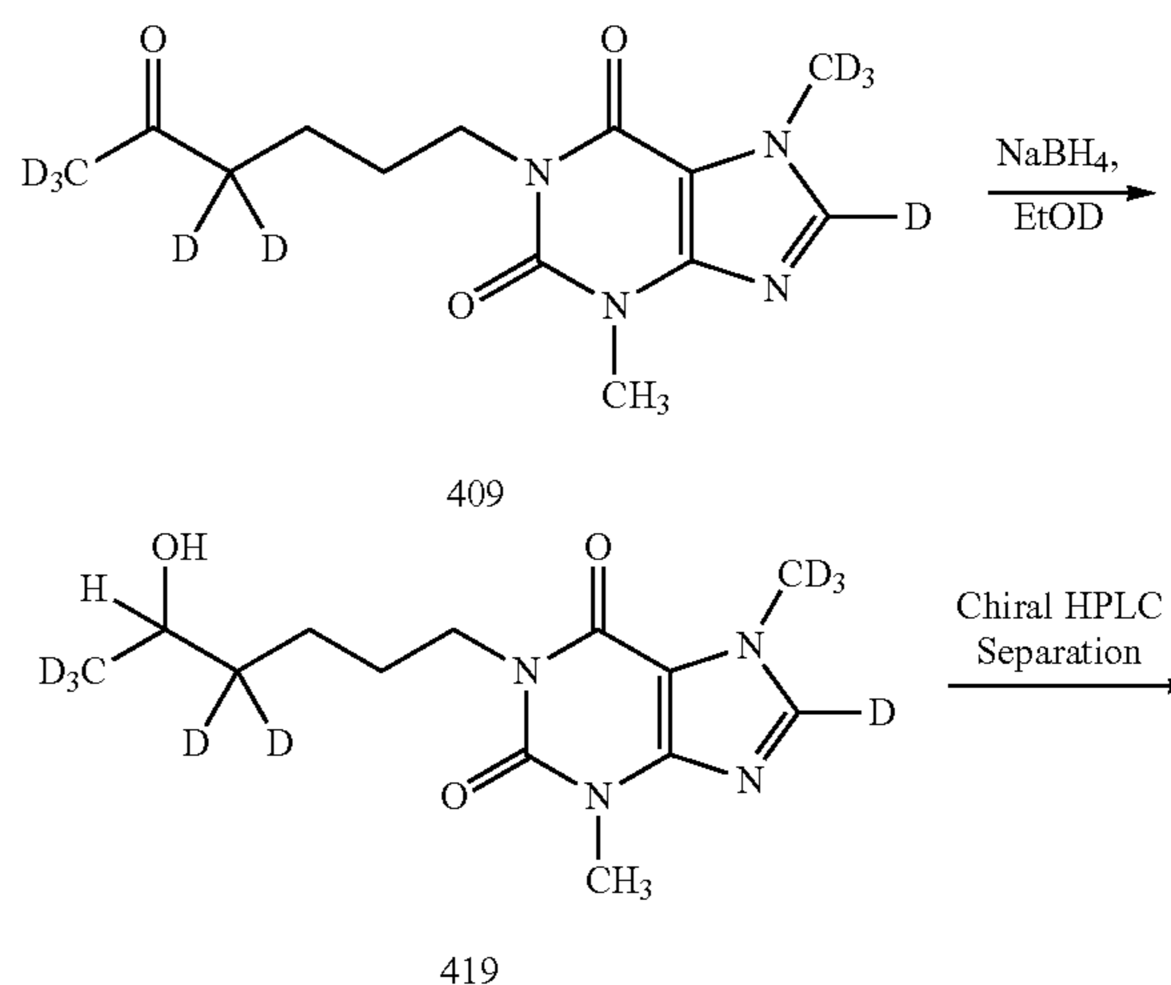
Scheme 16. Preparation of Compounds 419, 419(R), and 419(S).
