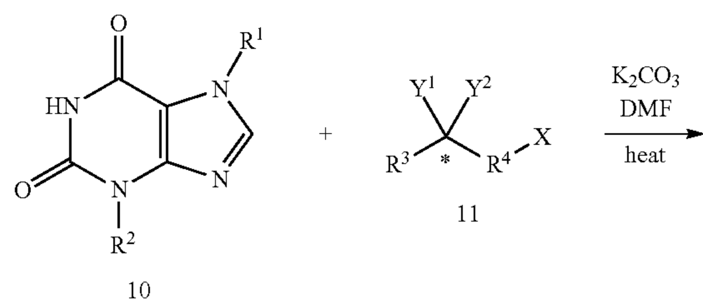
Scheme 1A. Synthesis of Compounds of Formula I
