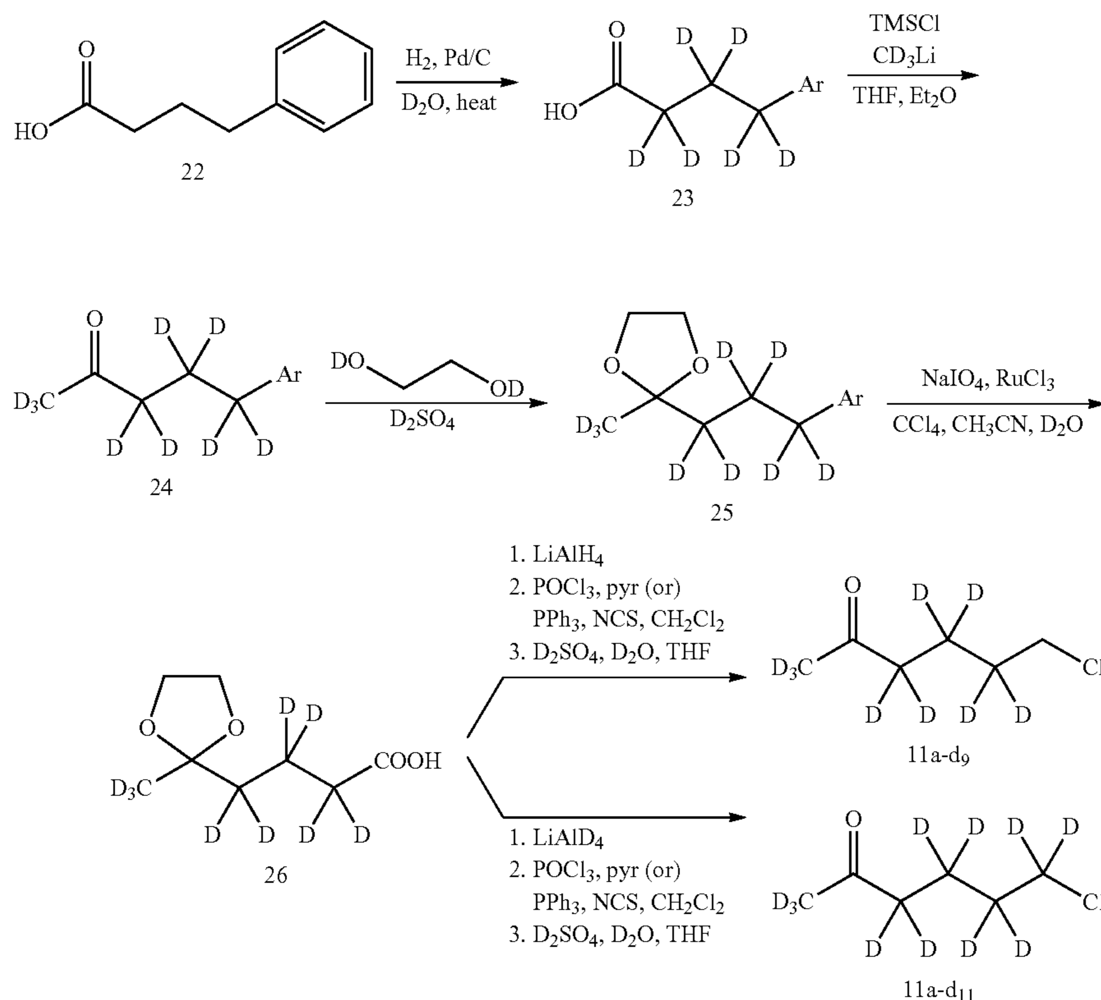
Scheme 4. Synthesis of Intermediates 11a-d 9 and 11a-d 11
