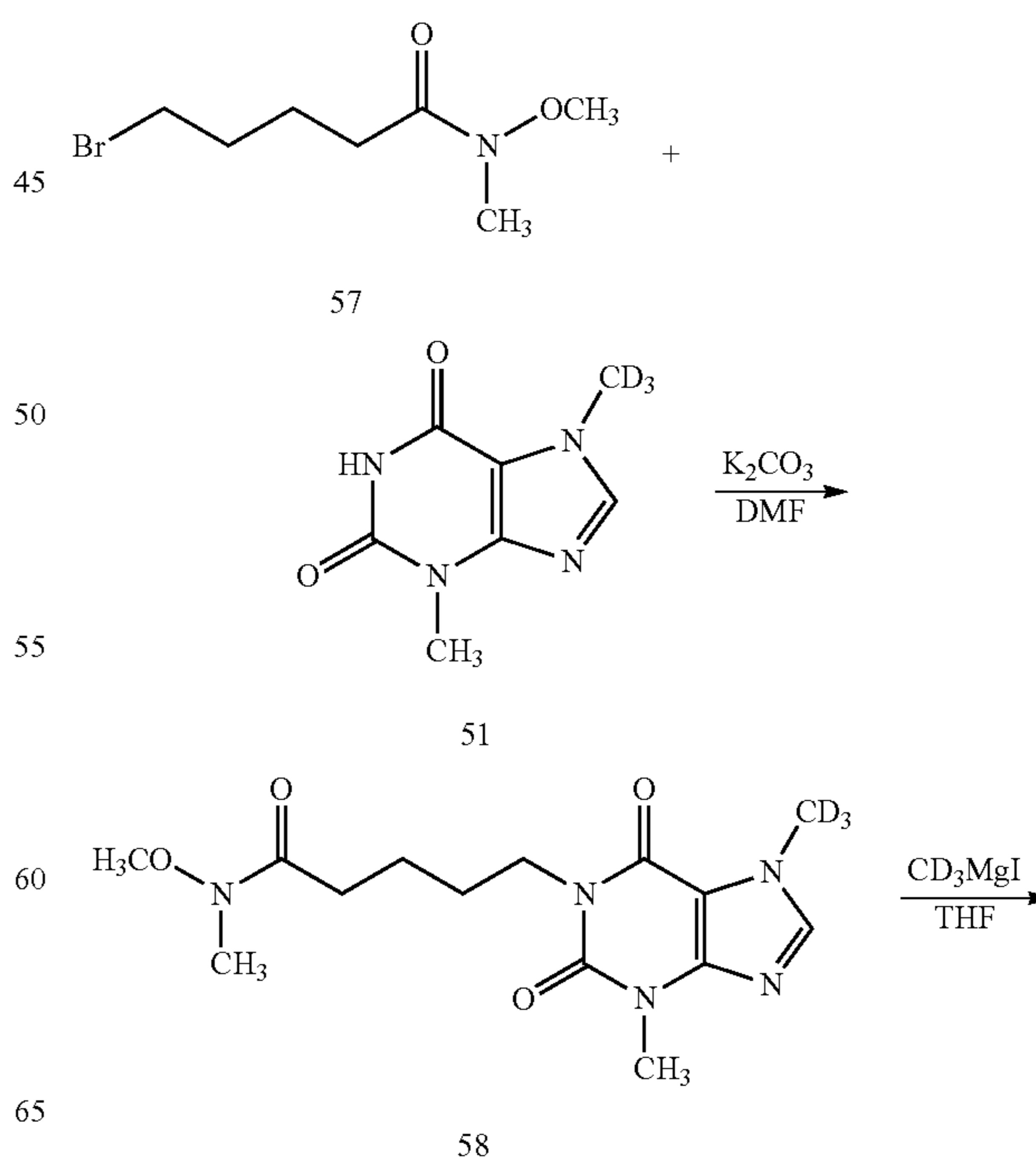
Scheme 15. Preparation of Compound 99.
