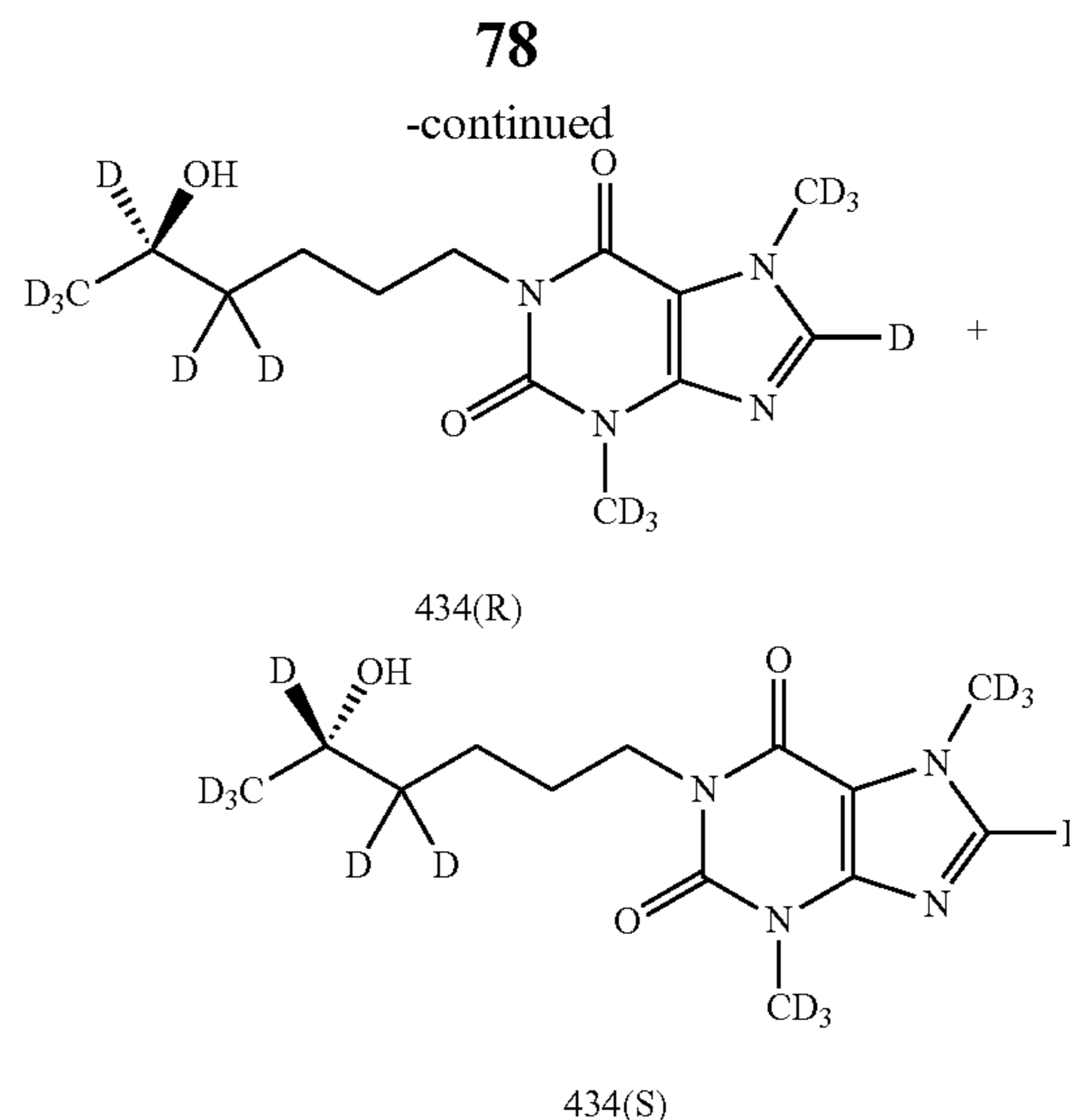
Synthesis of (±) 1-(4,4,5,6,6,6-d 6 -5-Hydroxyhexyl)-3,7-di(methyl-d 3 )-1H-purine-2,6(3H,7H)-dione (Compound 434)
