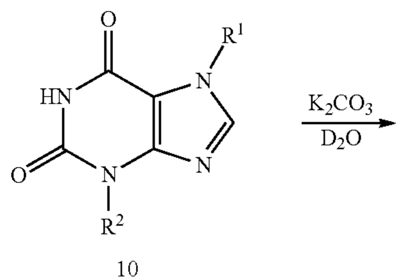
Scheme 12. Alternative Synthesis of Compounds of Formula A1
