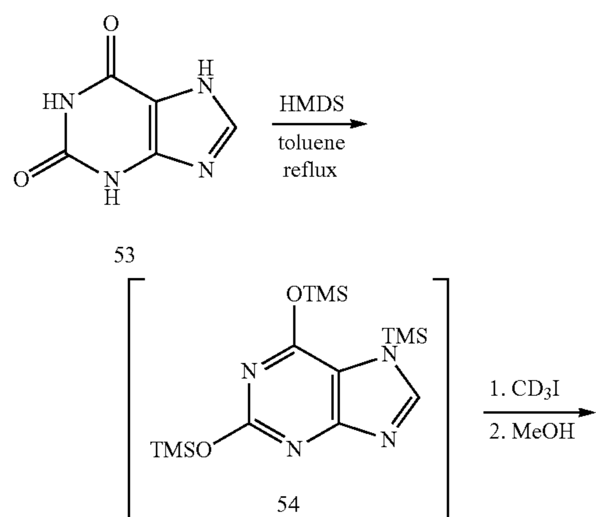
Scheme 14. Preparation of Compounds 101 and 413.
