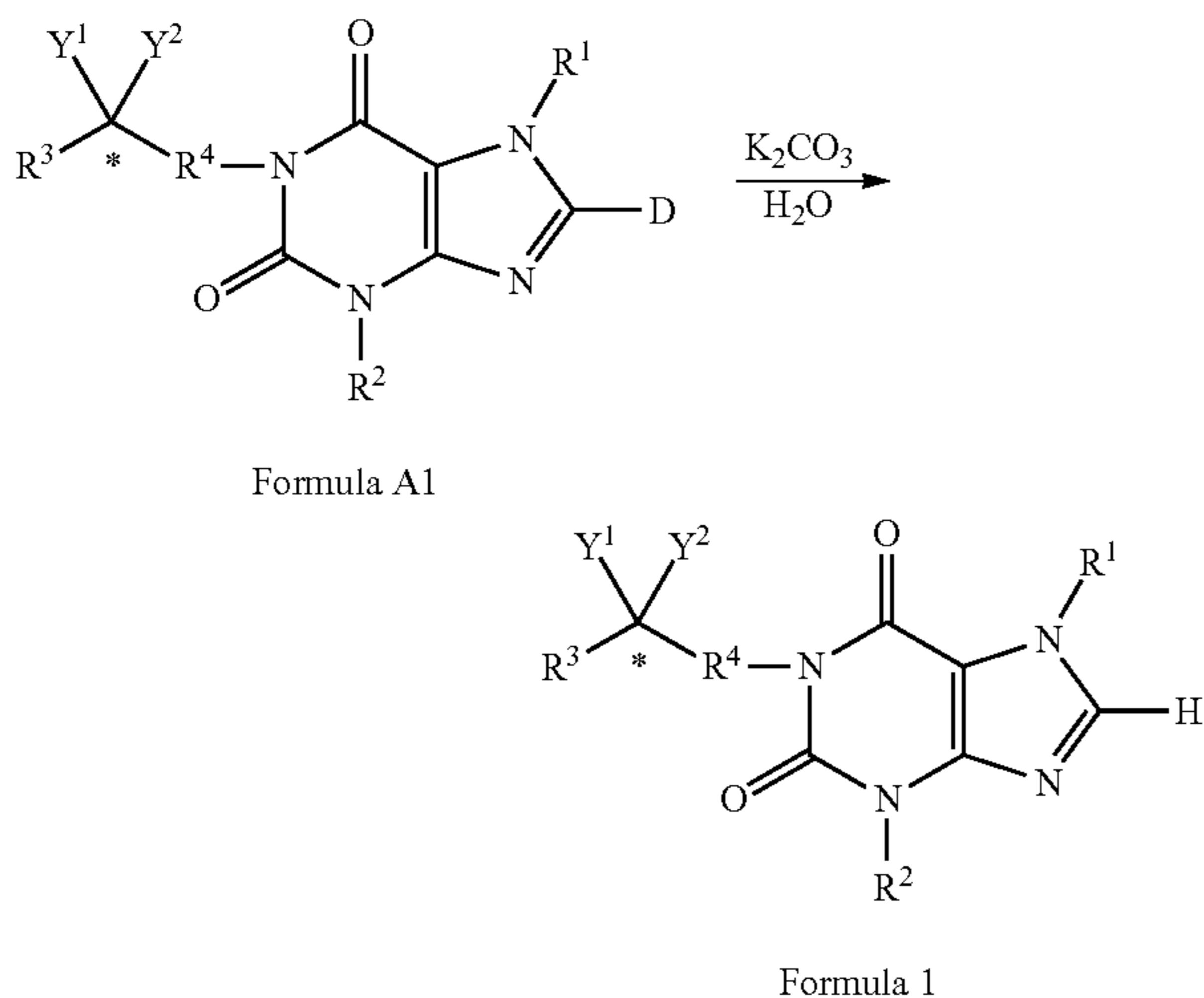
Scheme 12d. Alternative Synthesis of Compounds of Formula I.
