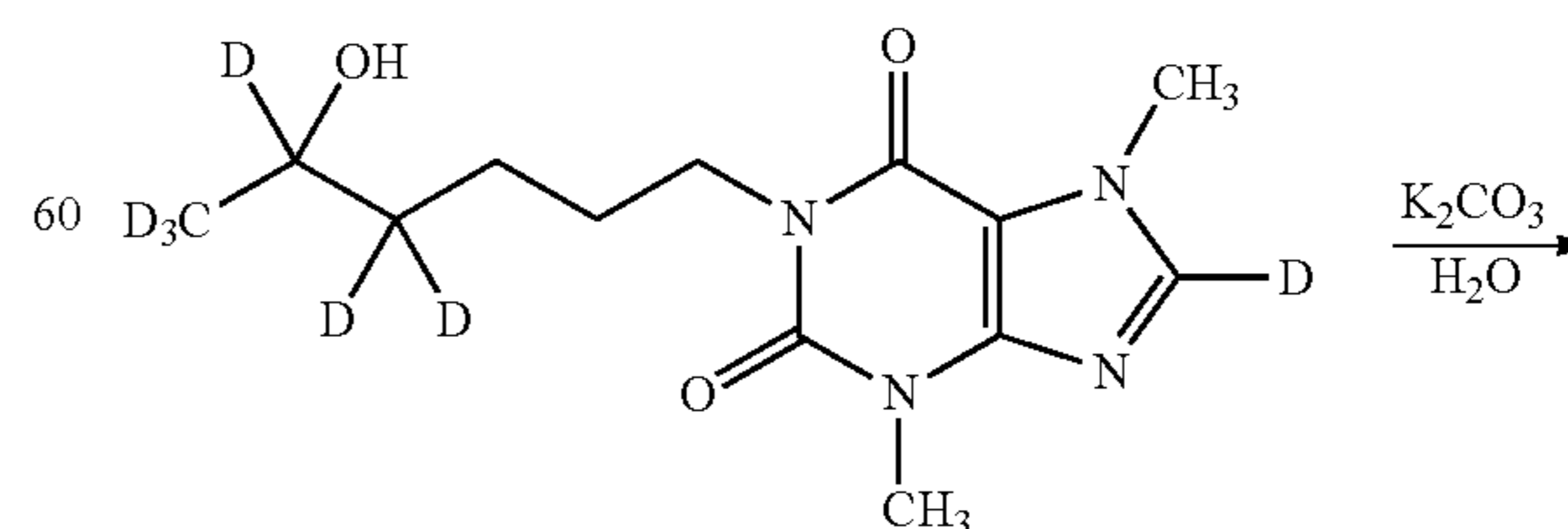
Scheme 21. Preparation of Compound 137.
