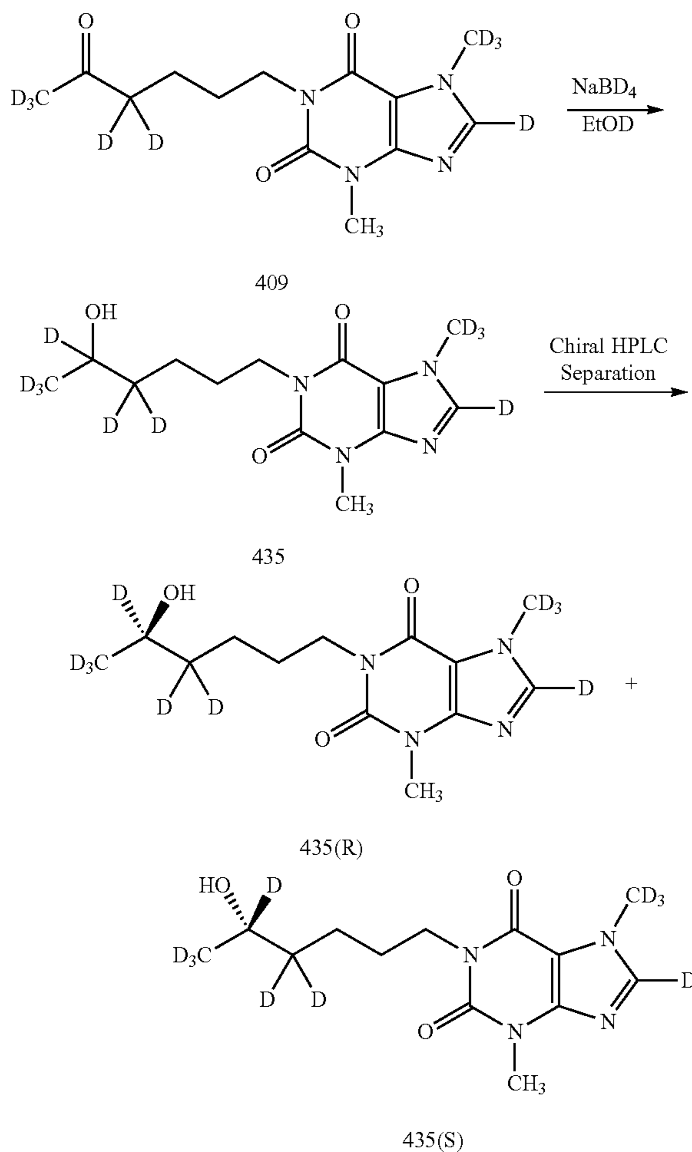
Scheme 17. Preparation of Compounds 435, 435(R), and 435(S).
