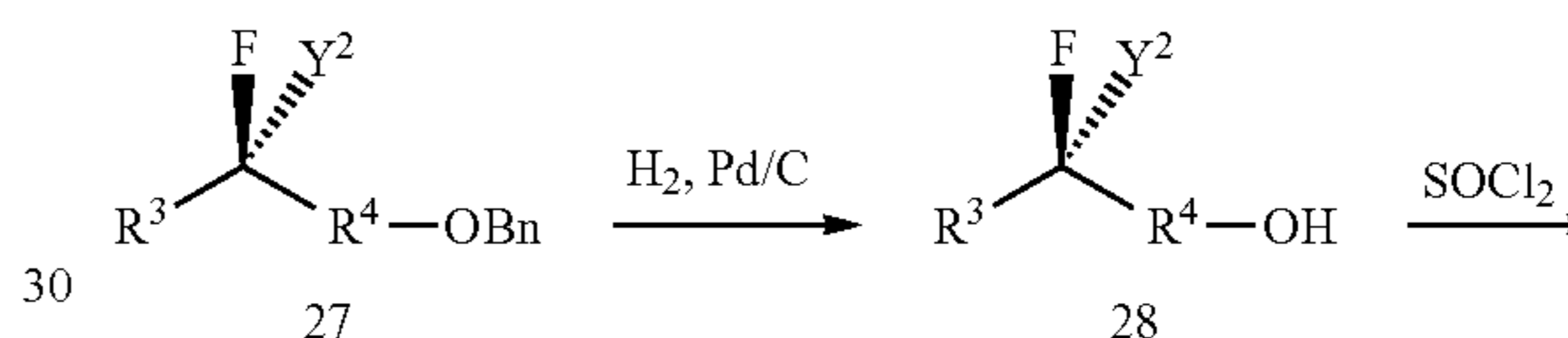
Scheme 4a. Synthesis of Intermediates 11b-(R)
