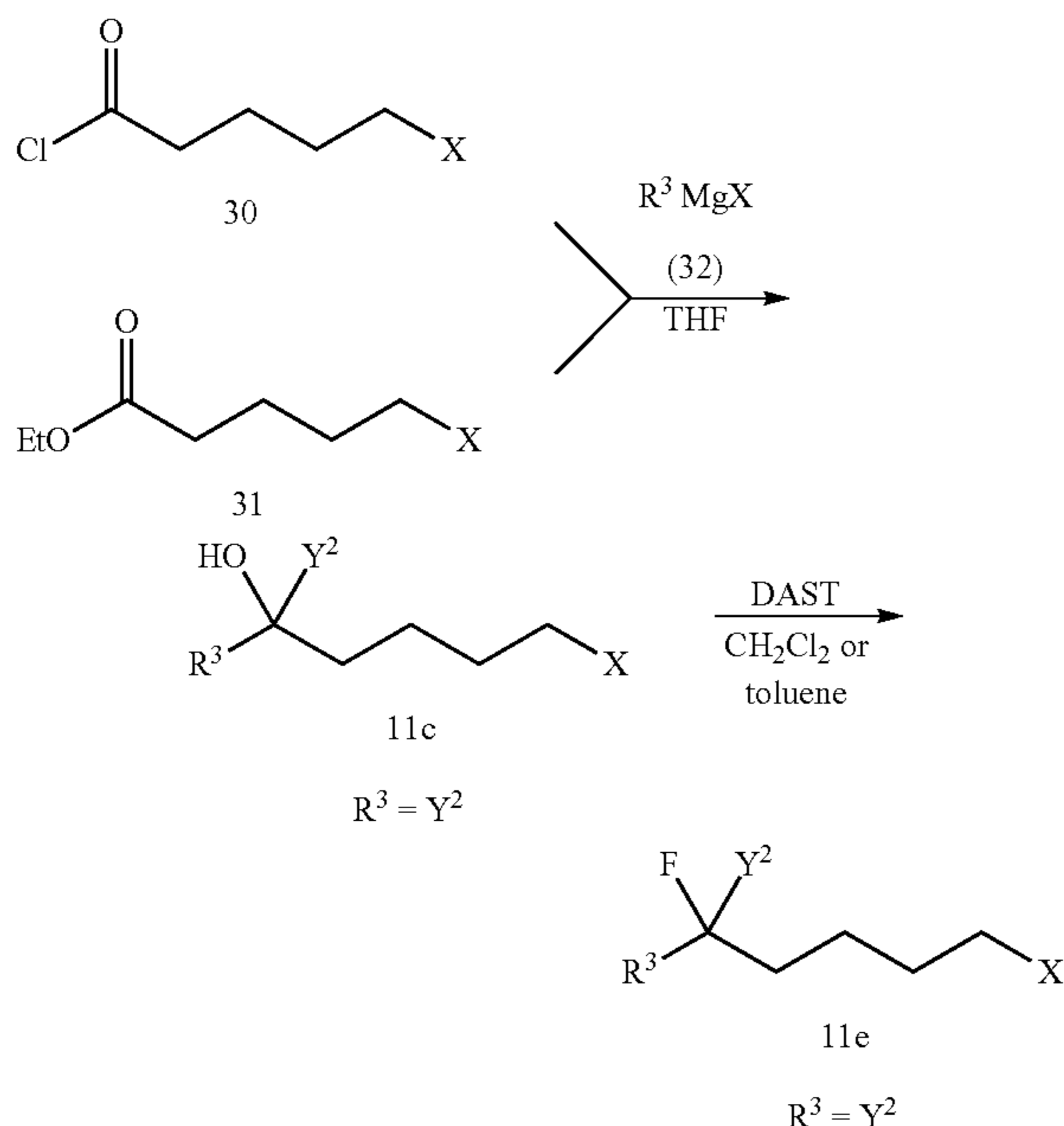
Scheme 5. Synthesis of Intermediates 11c and 11e
