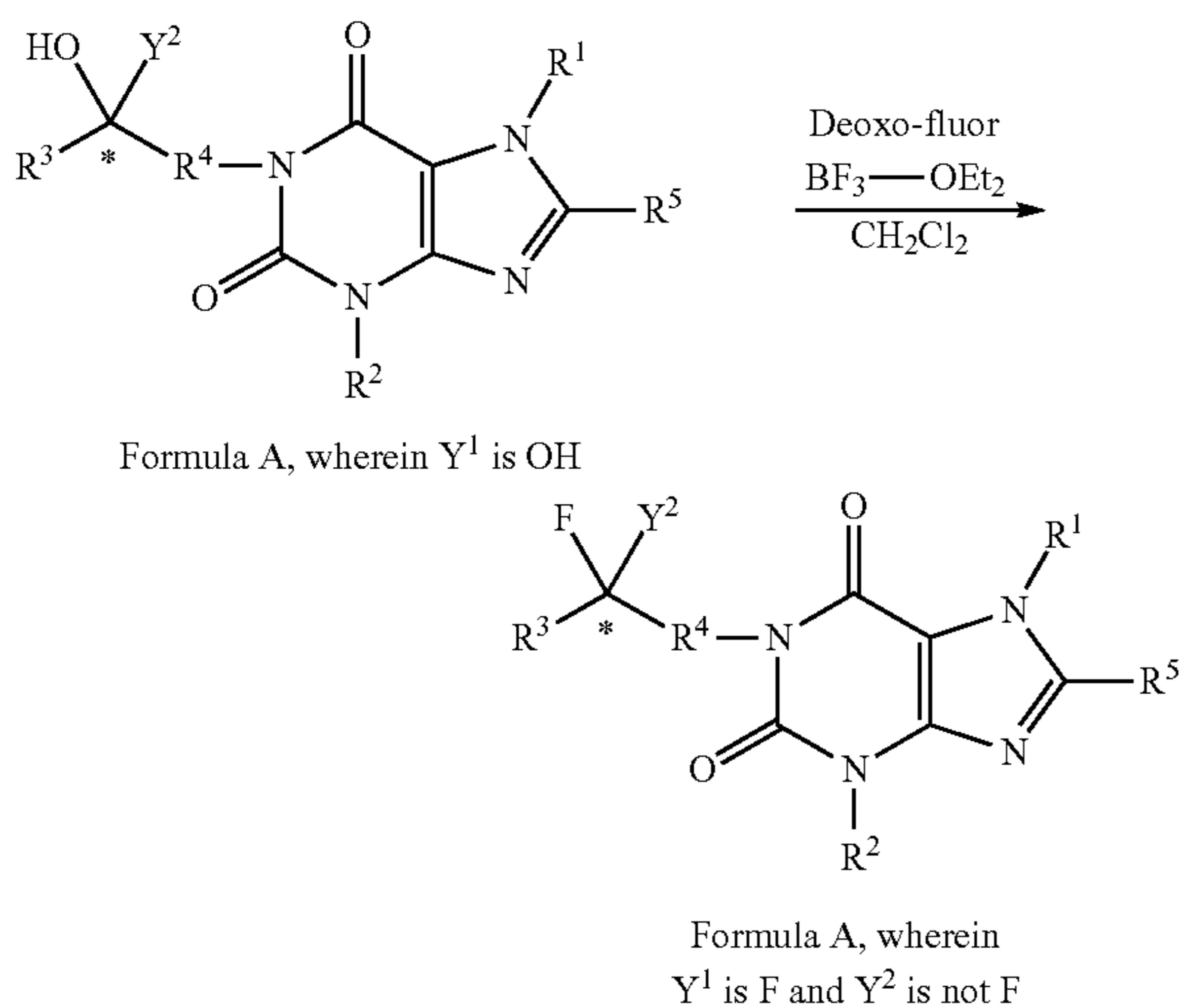
Scheme 12c. Alternative Synthesis of Compounds of Formula A, wherein Y 1 is Fluorine and Y 2 is not Fluorine.
