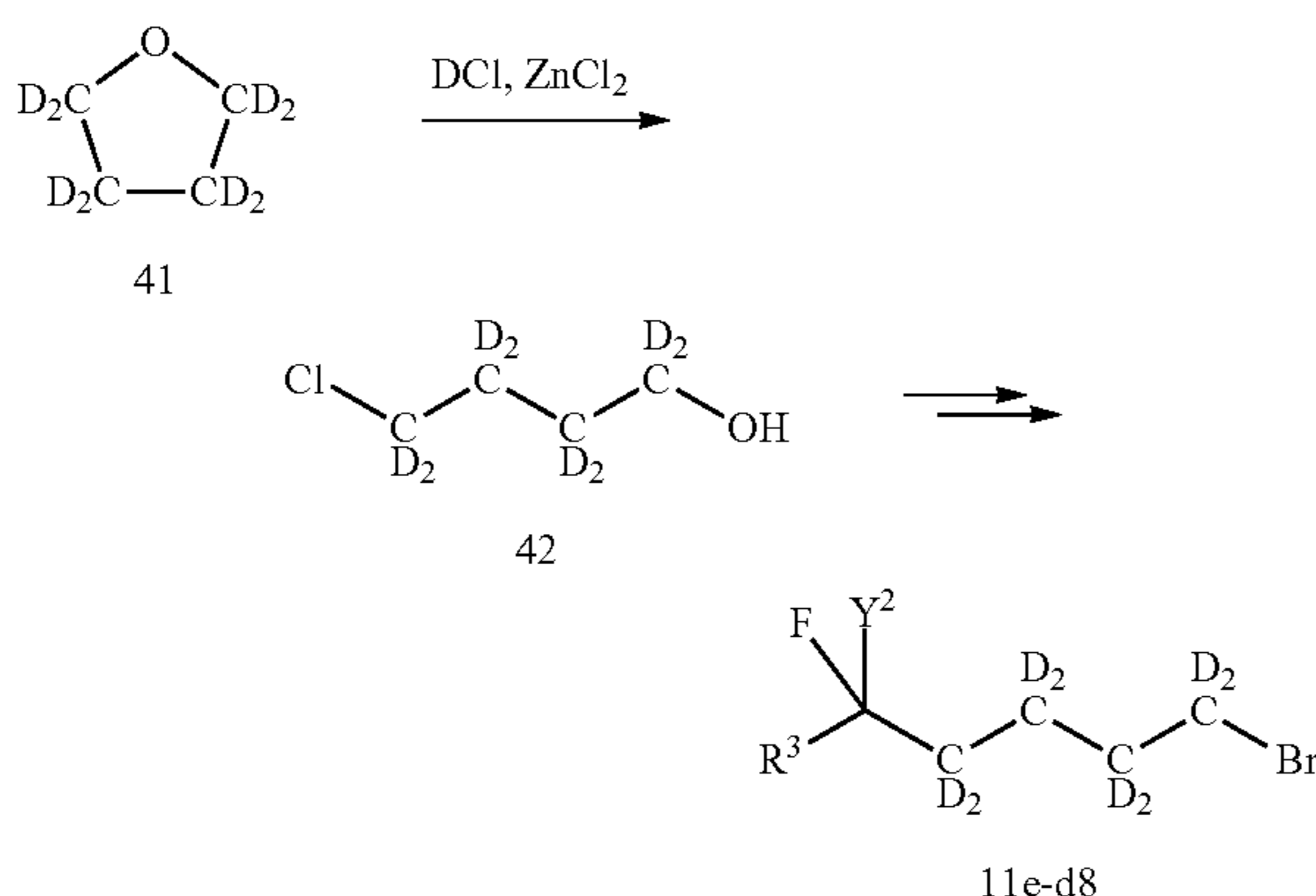
Scheme 8. Synthesis of Intermediate 11e-d 8 (X = Br)
