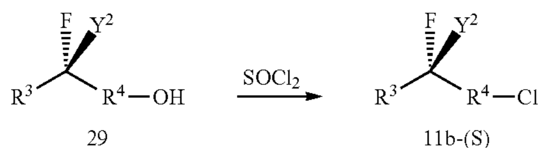
Scheme 4b. Synthesis of Chloride 11b-(S)
