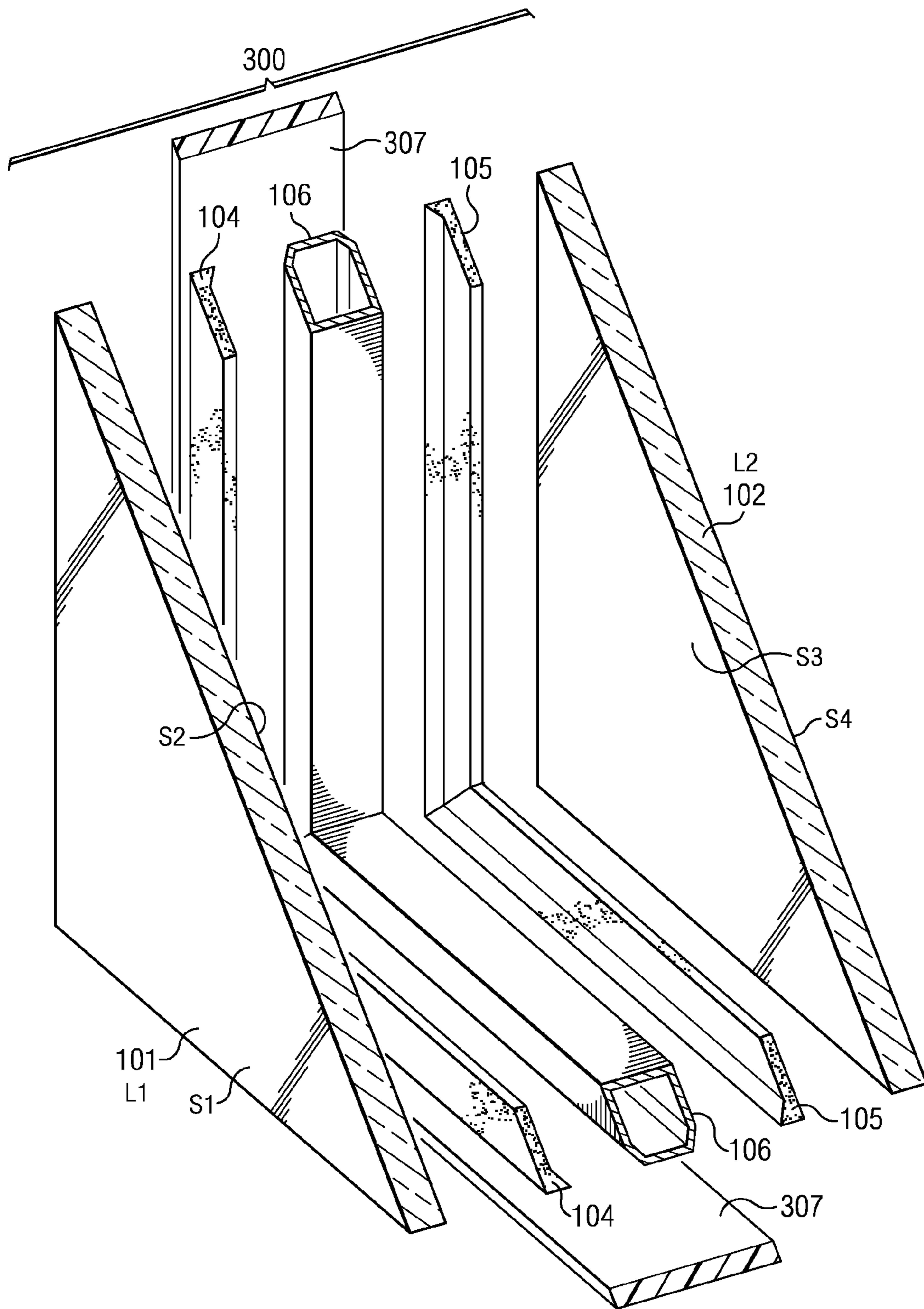
FIG. 3c (PRIOR ART)
