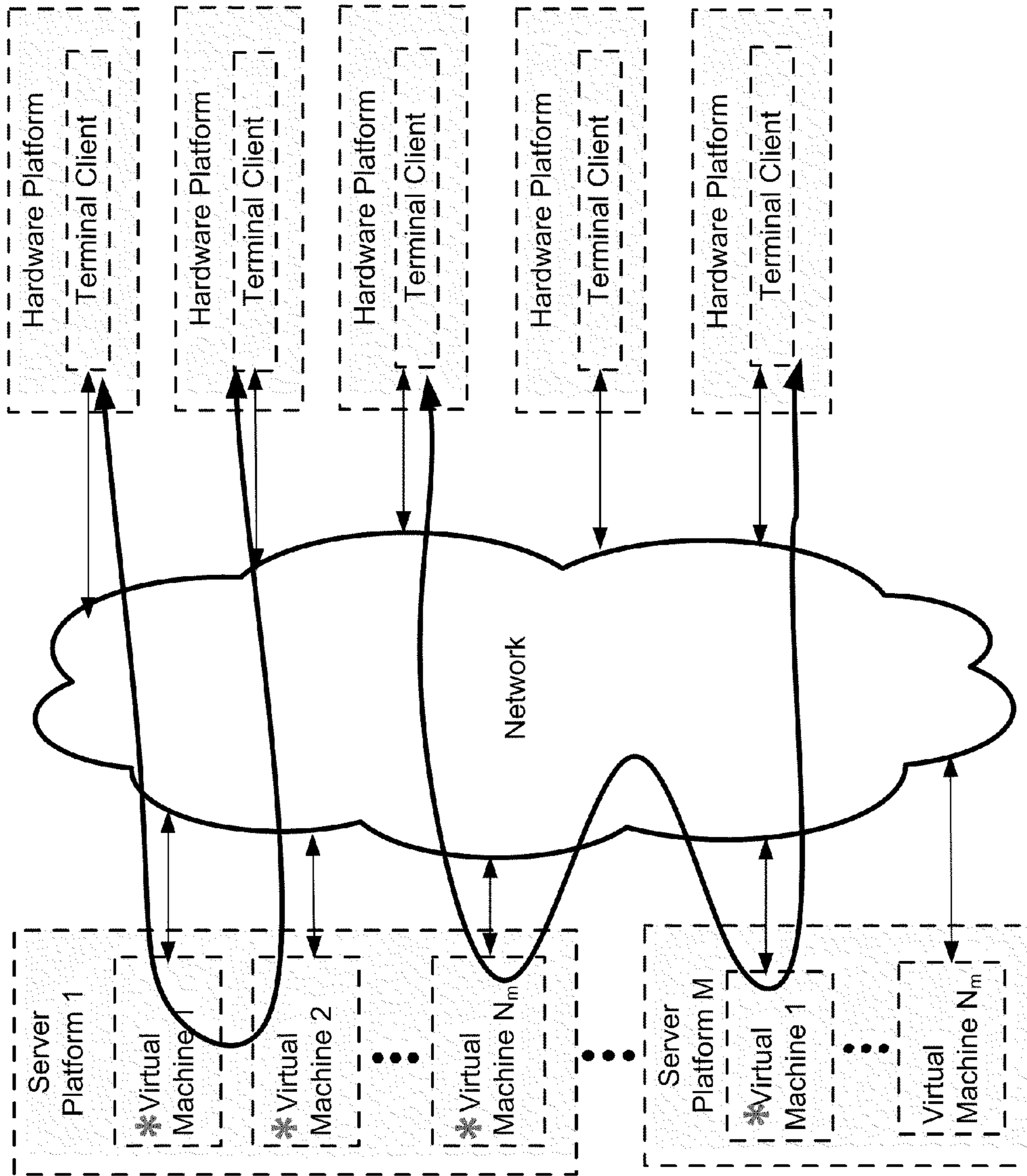
Figure 6 – High bandwidth uncompressed streams ( * ) and computation loads ( * )
