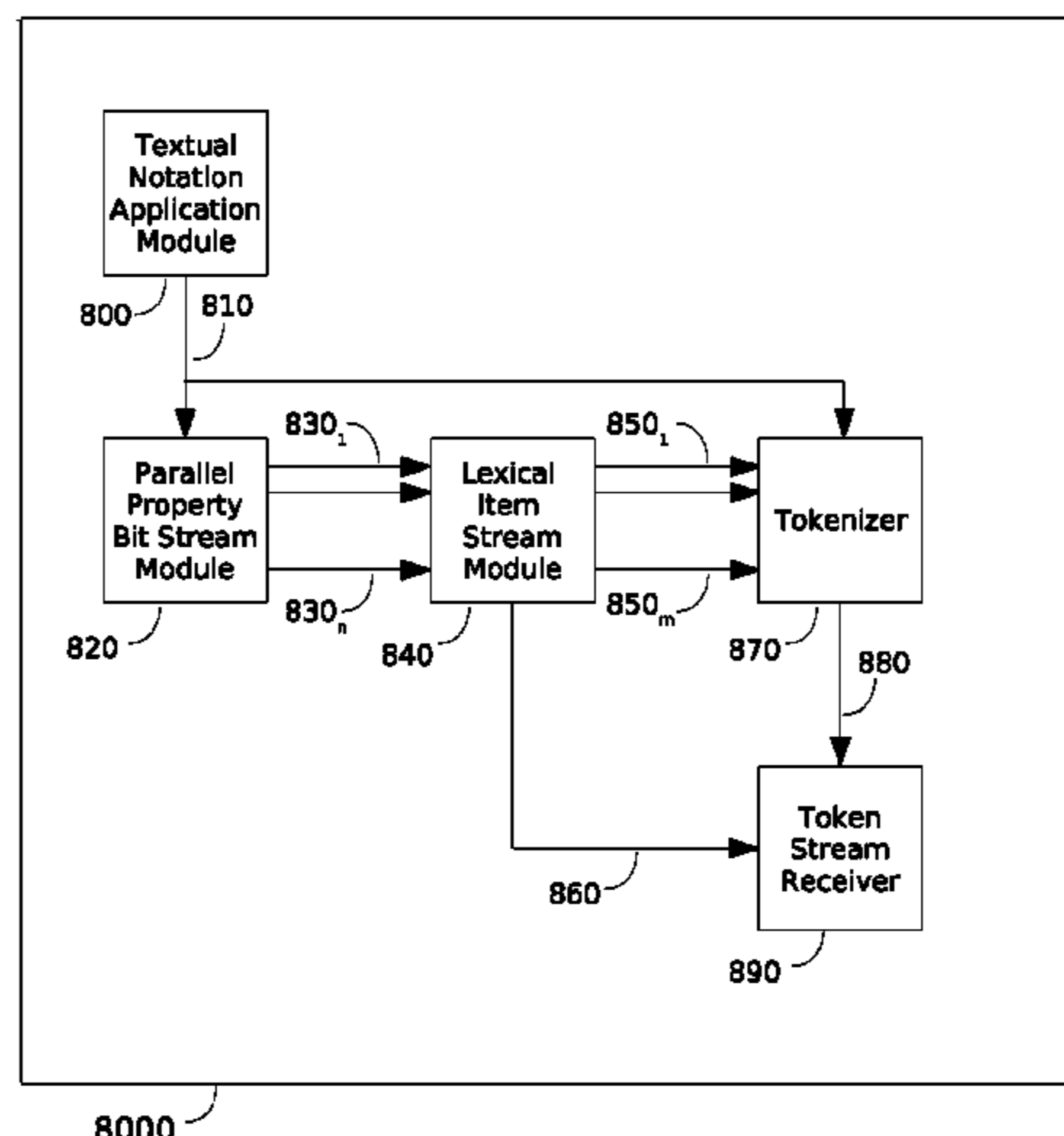
Application Module Utilizing Lexical Analyzer
