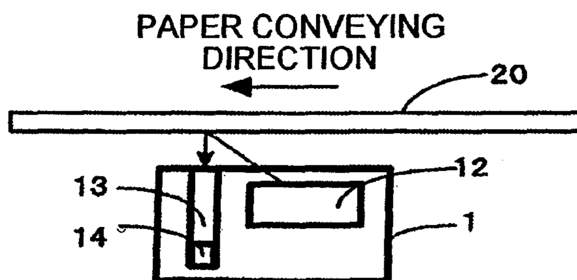
FIG.7C -CONVENTIONAL ART-
