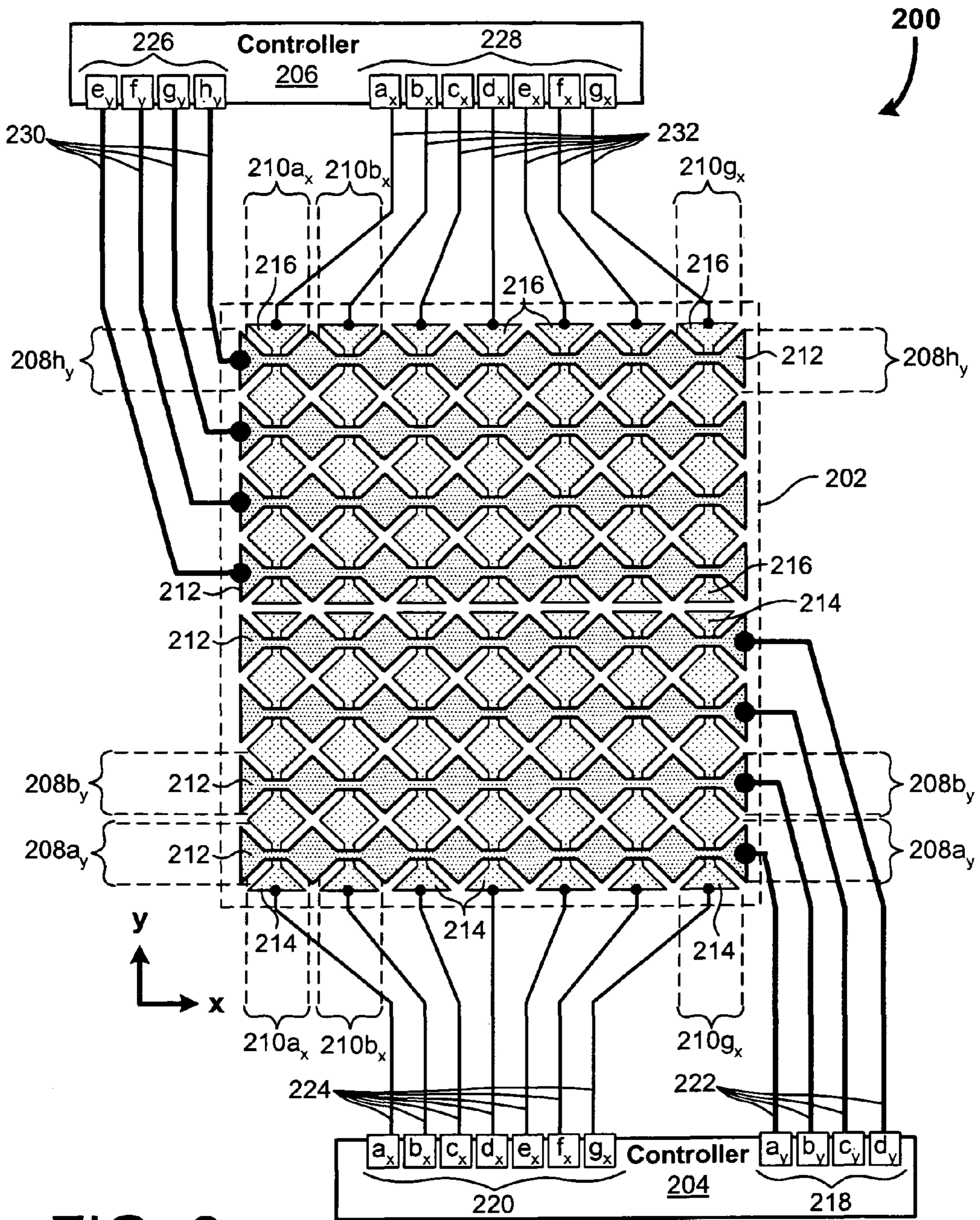
FIG. 2 (PRIOR ART)
