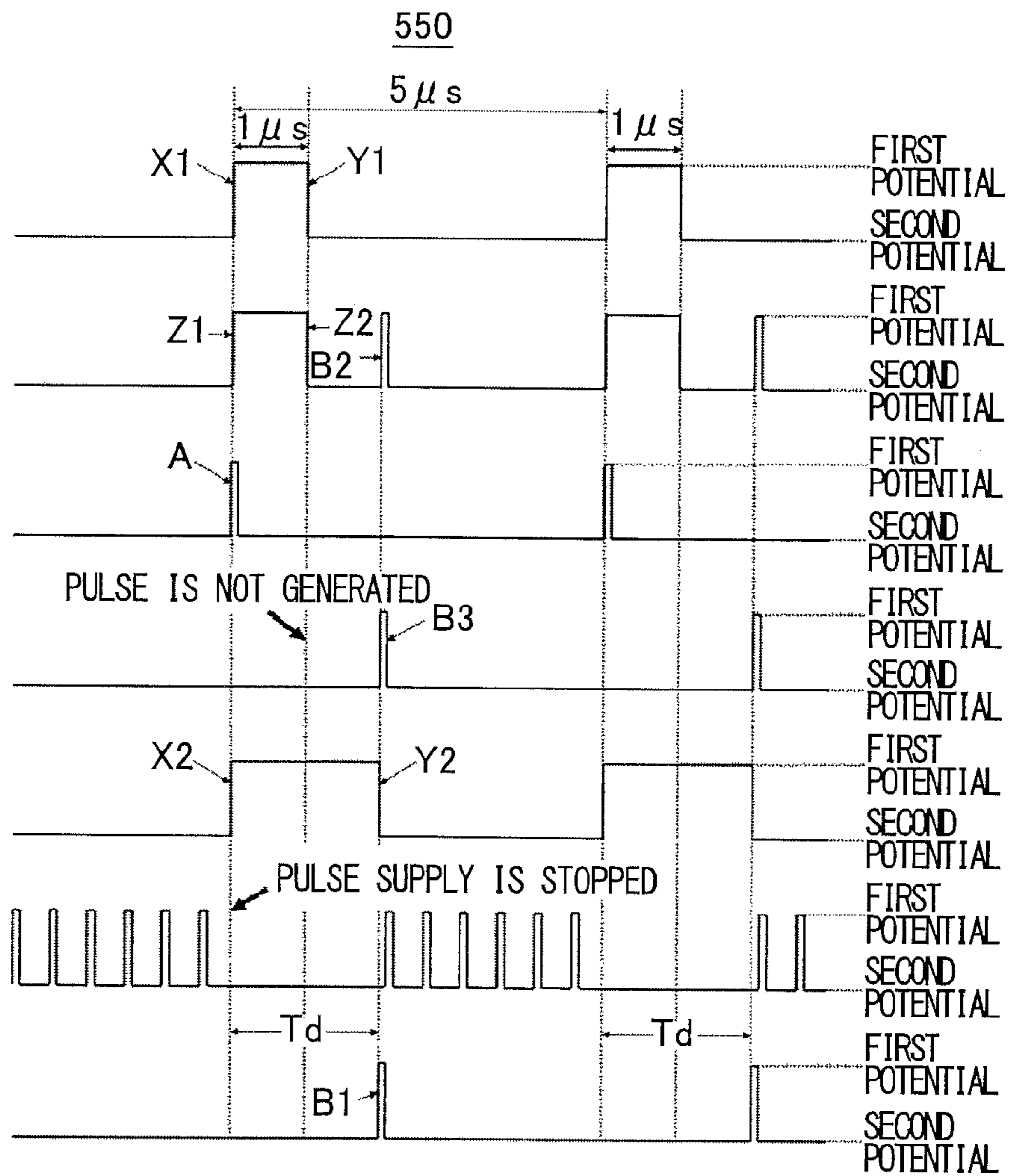
FIG. 7A CONTROL INPUT SIGNAL S_{in}
