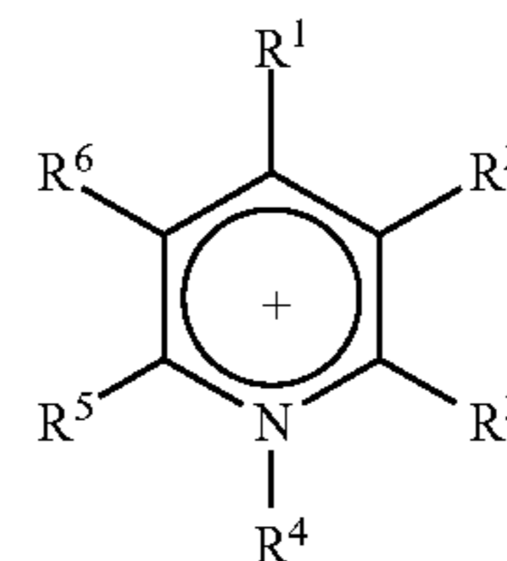
Pyridinium
