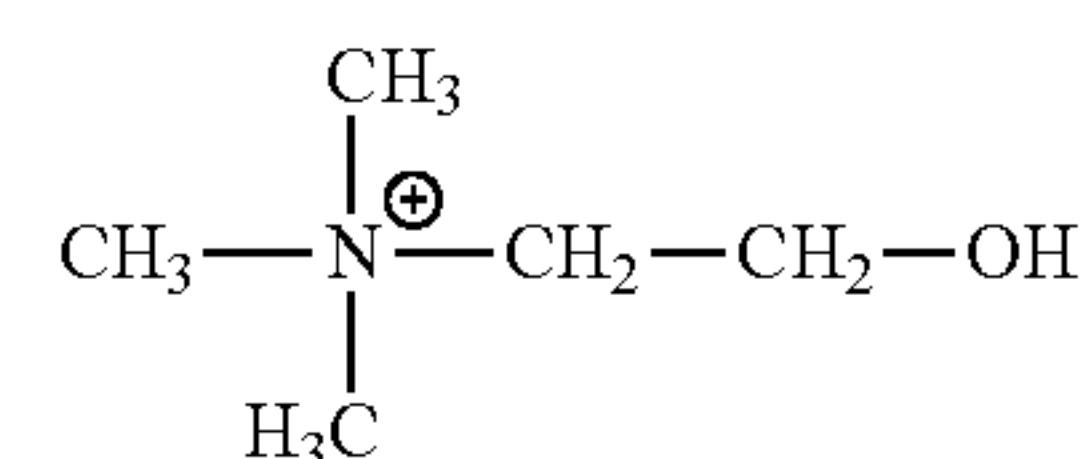
Choline
