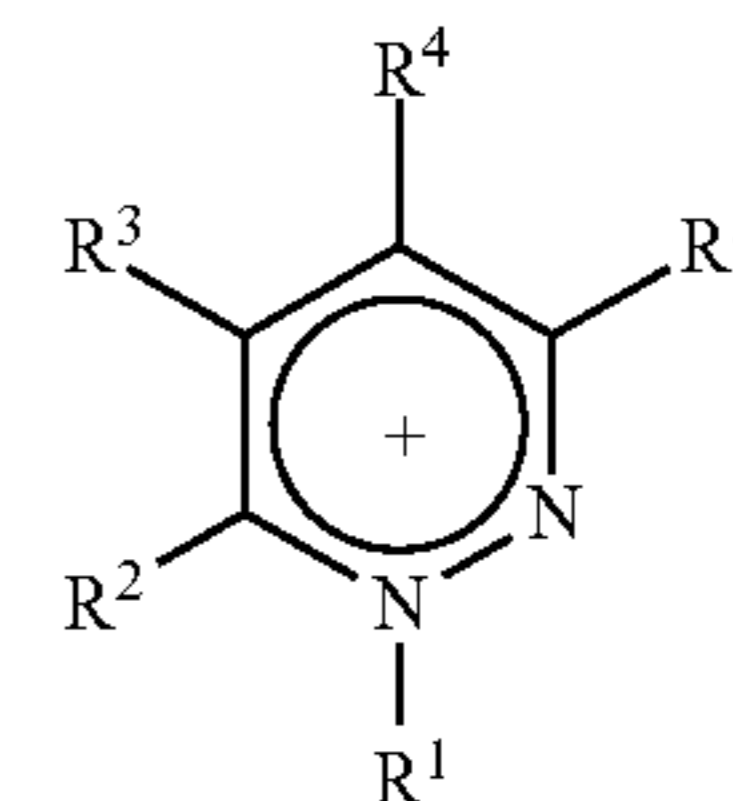
Pyridazinium
