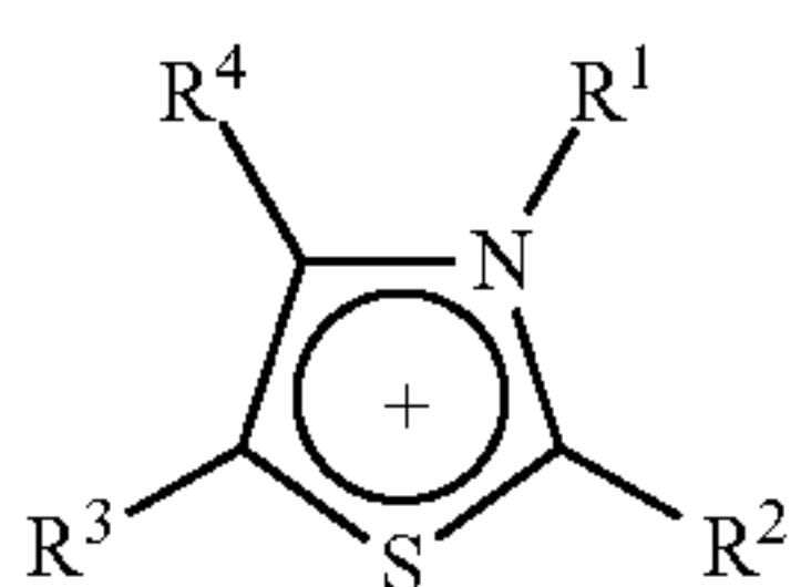
Thiazolium
