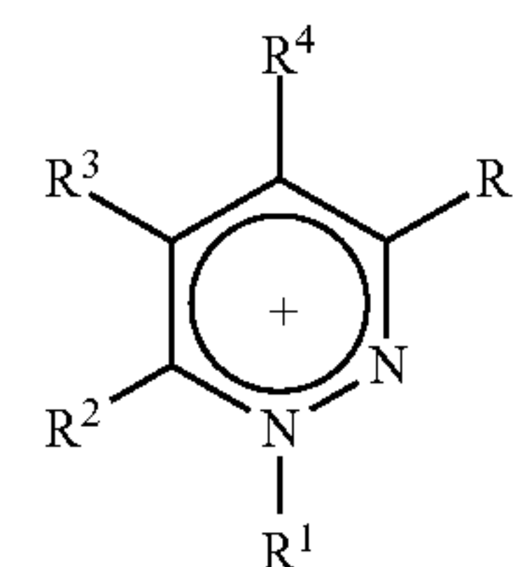
Pyridazinium
