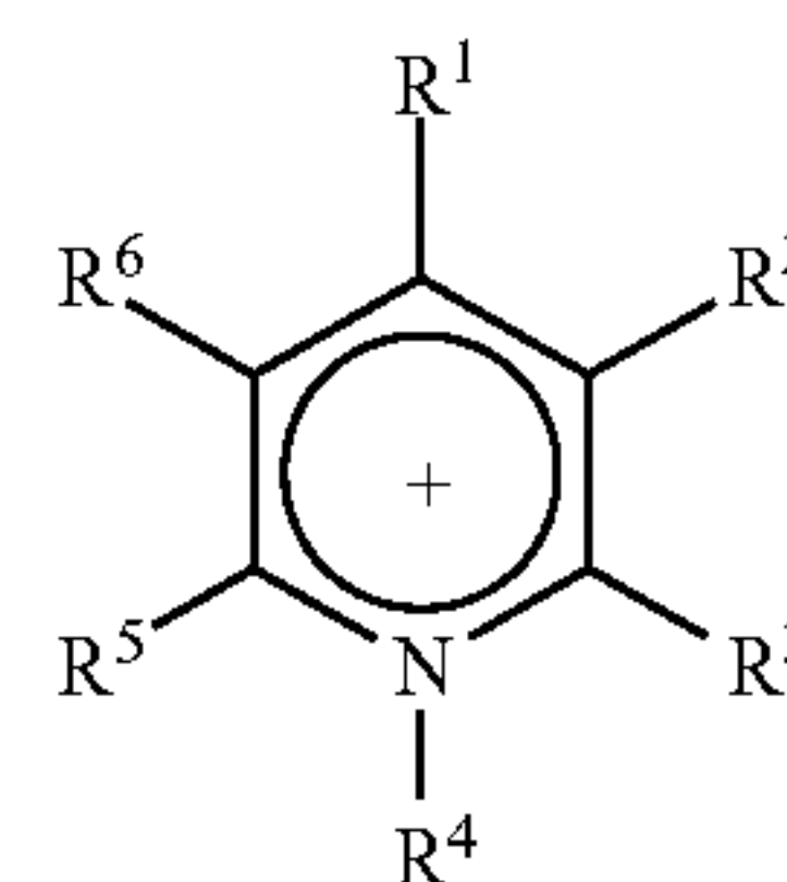
Pyridinium
