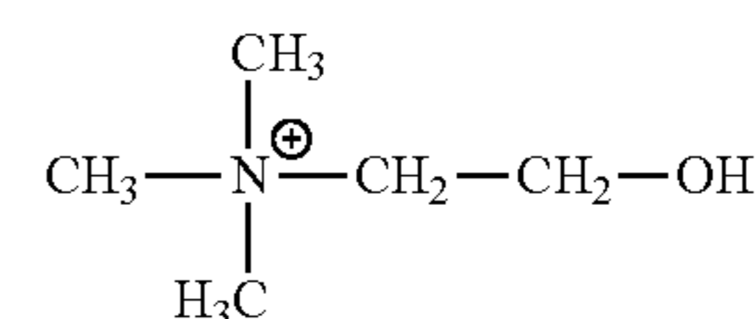
Choline
