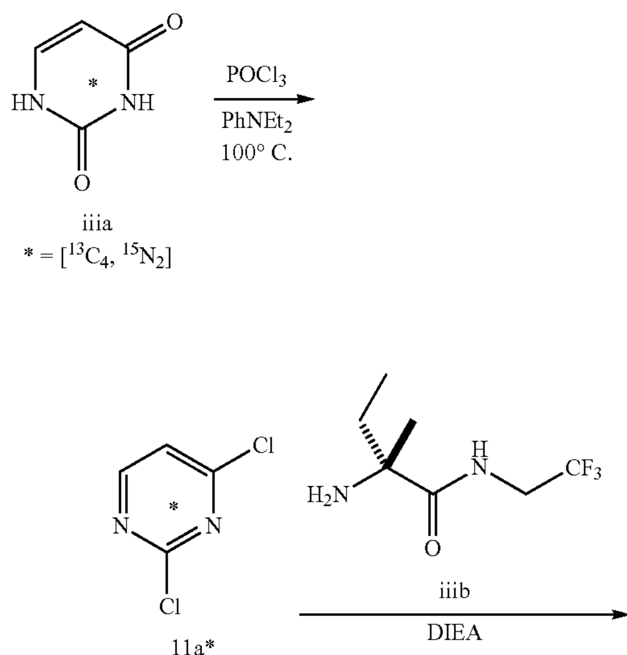
Scheme III
