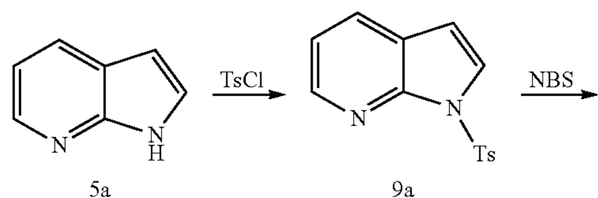
Scheme IIb:
