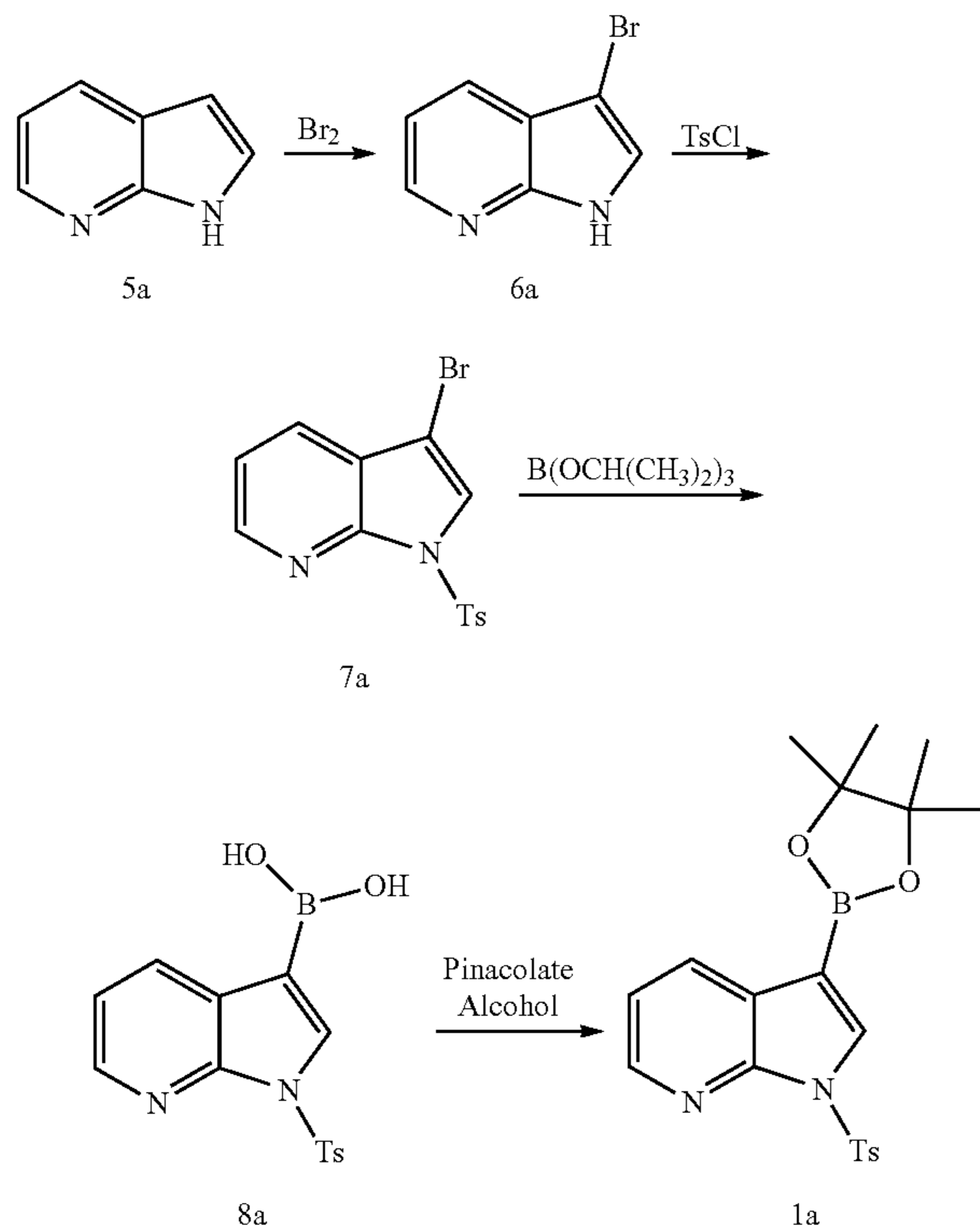
Scheme IIa:
