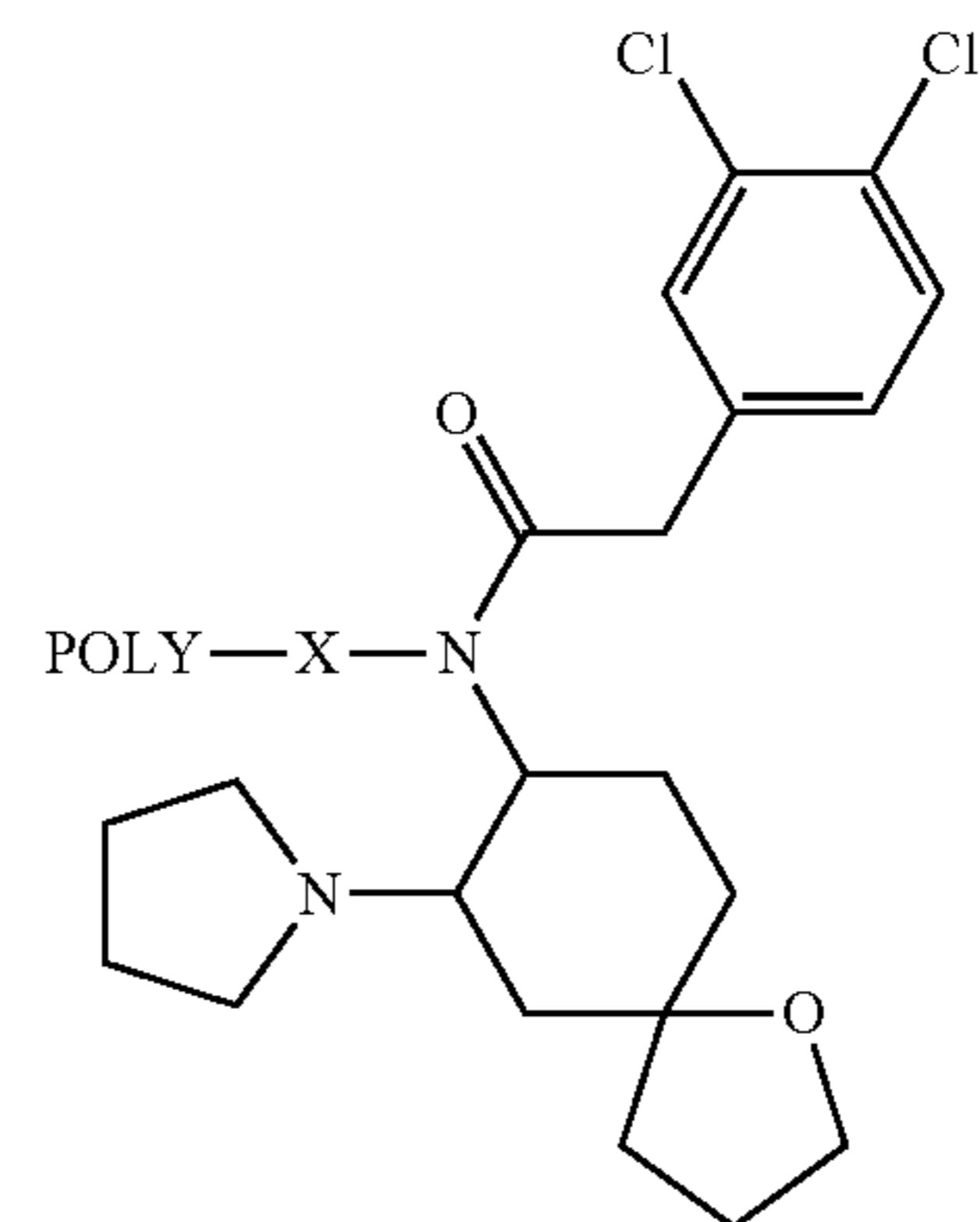
(exemplary spiradoline conjugate)
