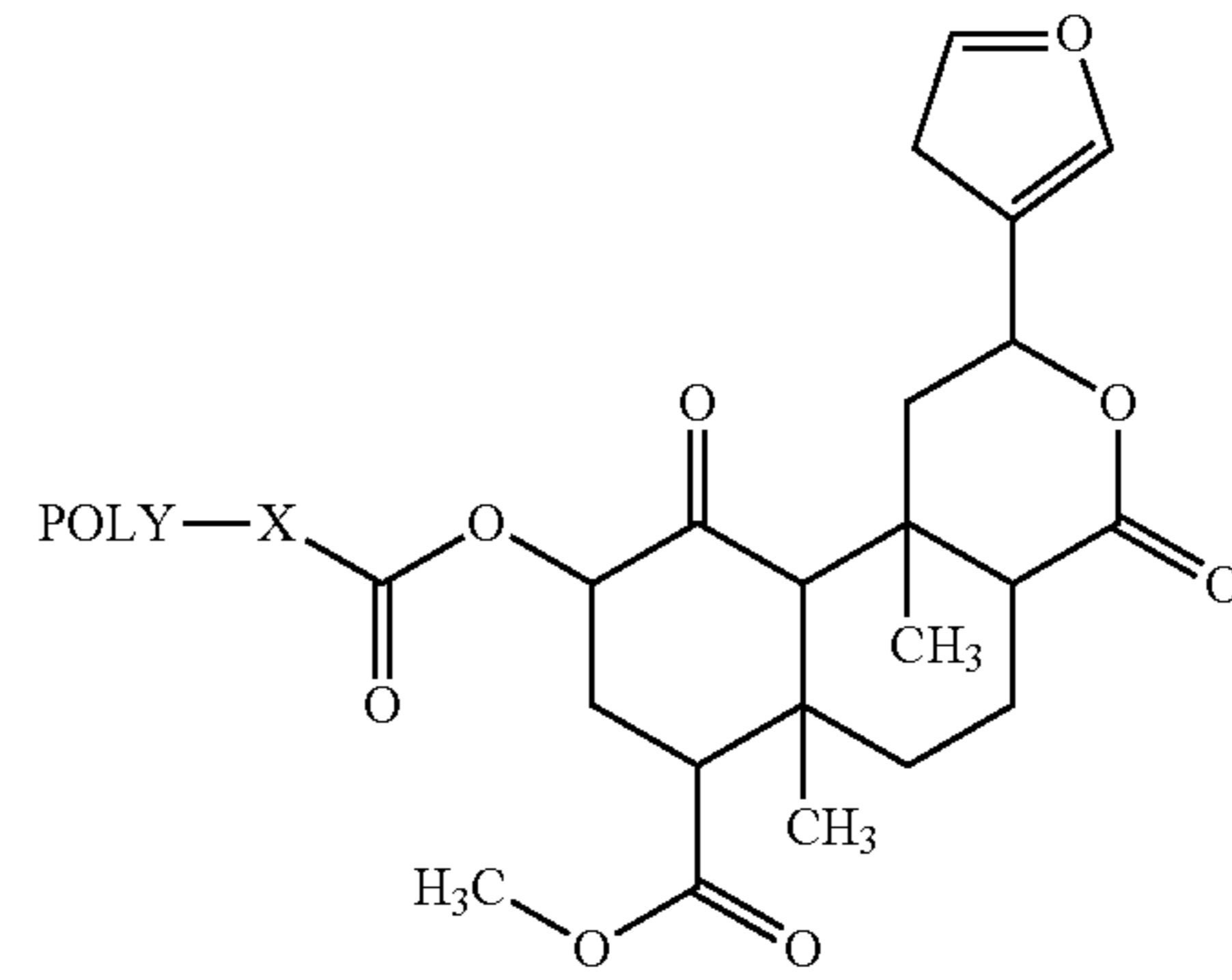
(exemplary salvinorin A conjugate)
