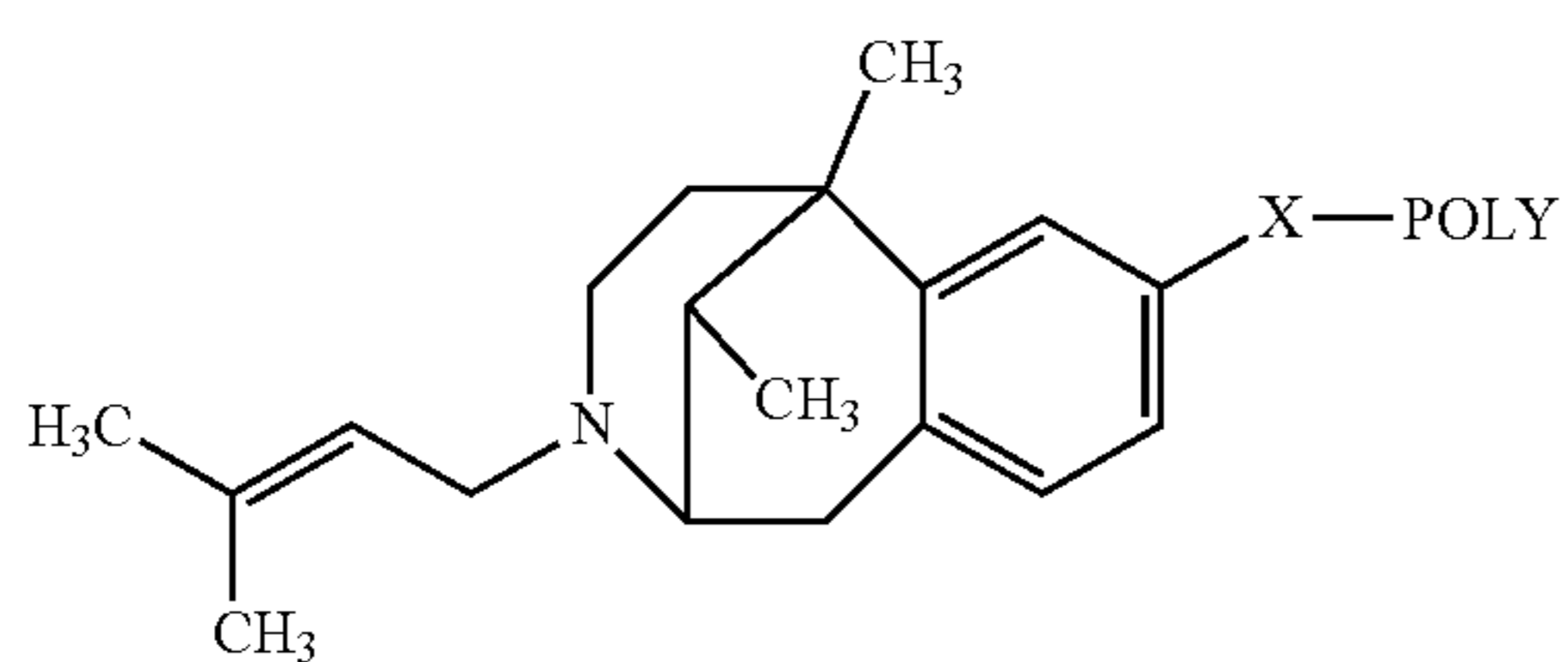
(exemplary pentazocine conjugate)
