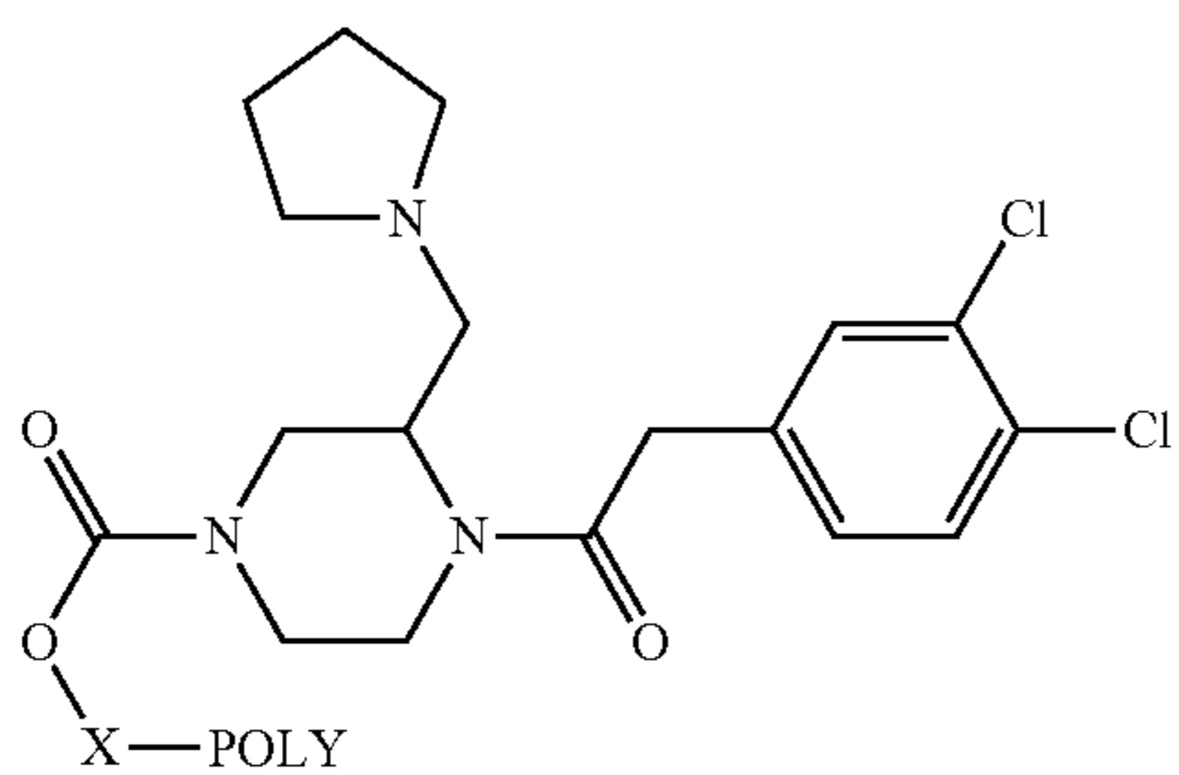
(exemplary ethylketocyclazocine conjugate)
