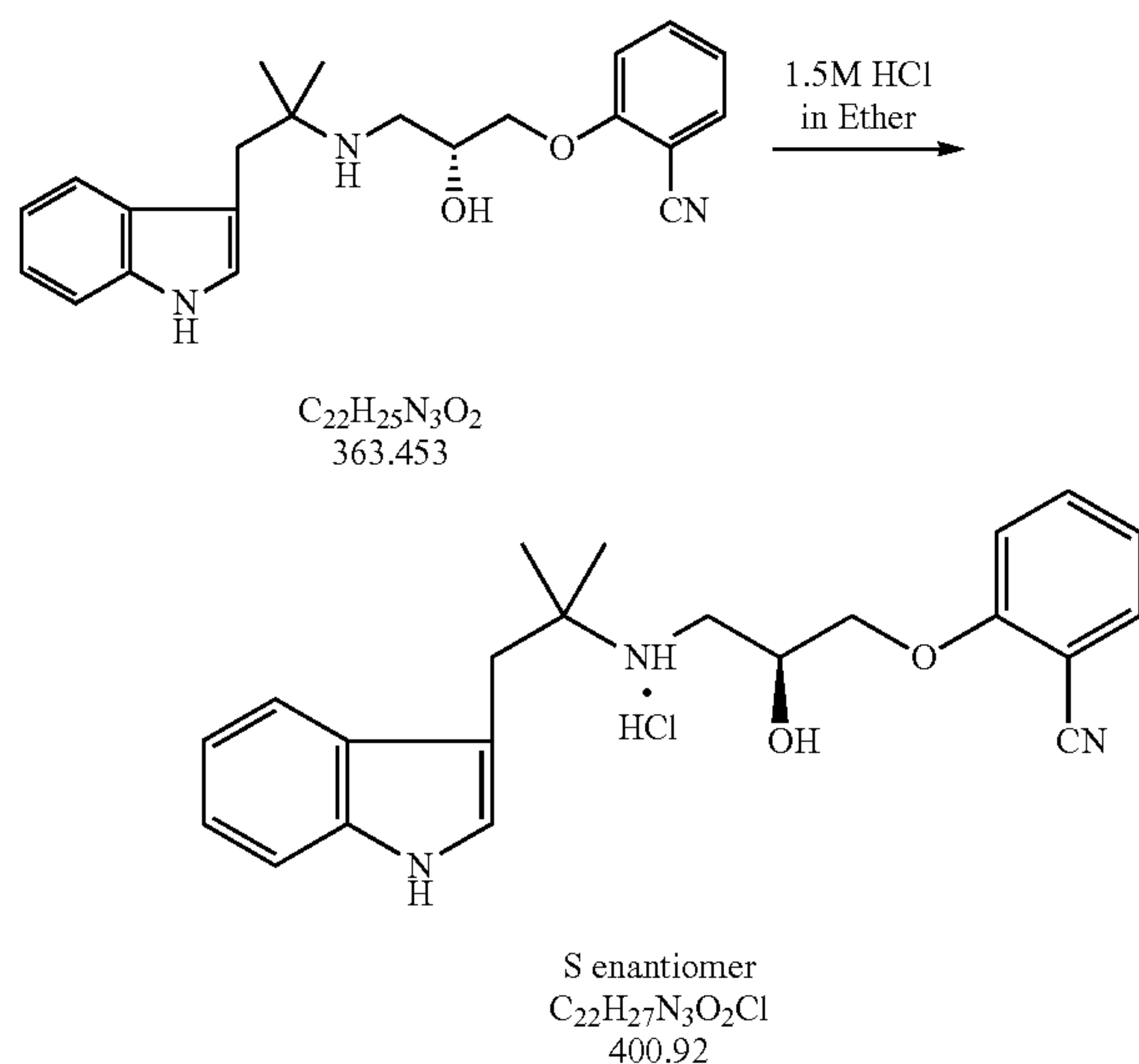
Reaction 4.
