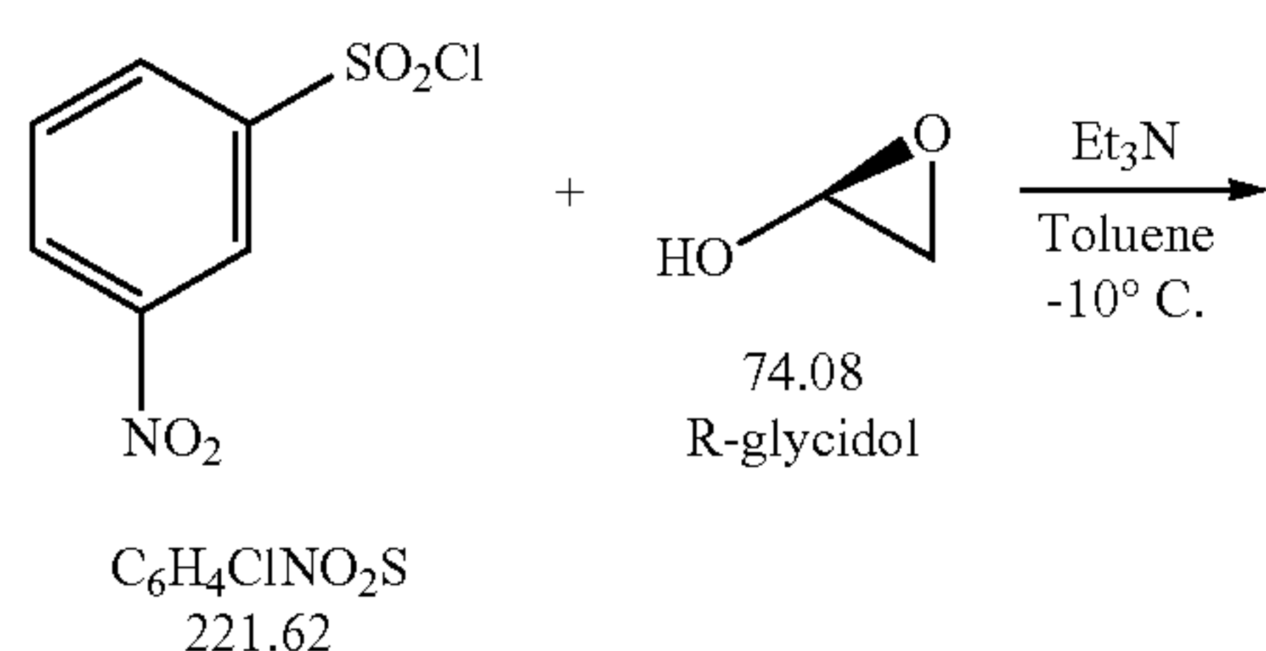
Reaction 5.
