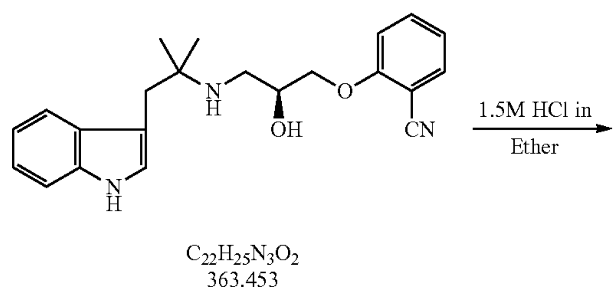
Reaction 8.
