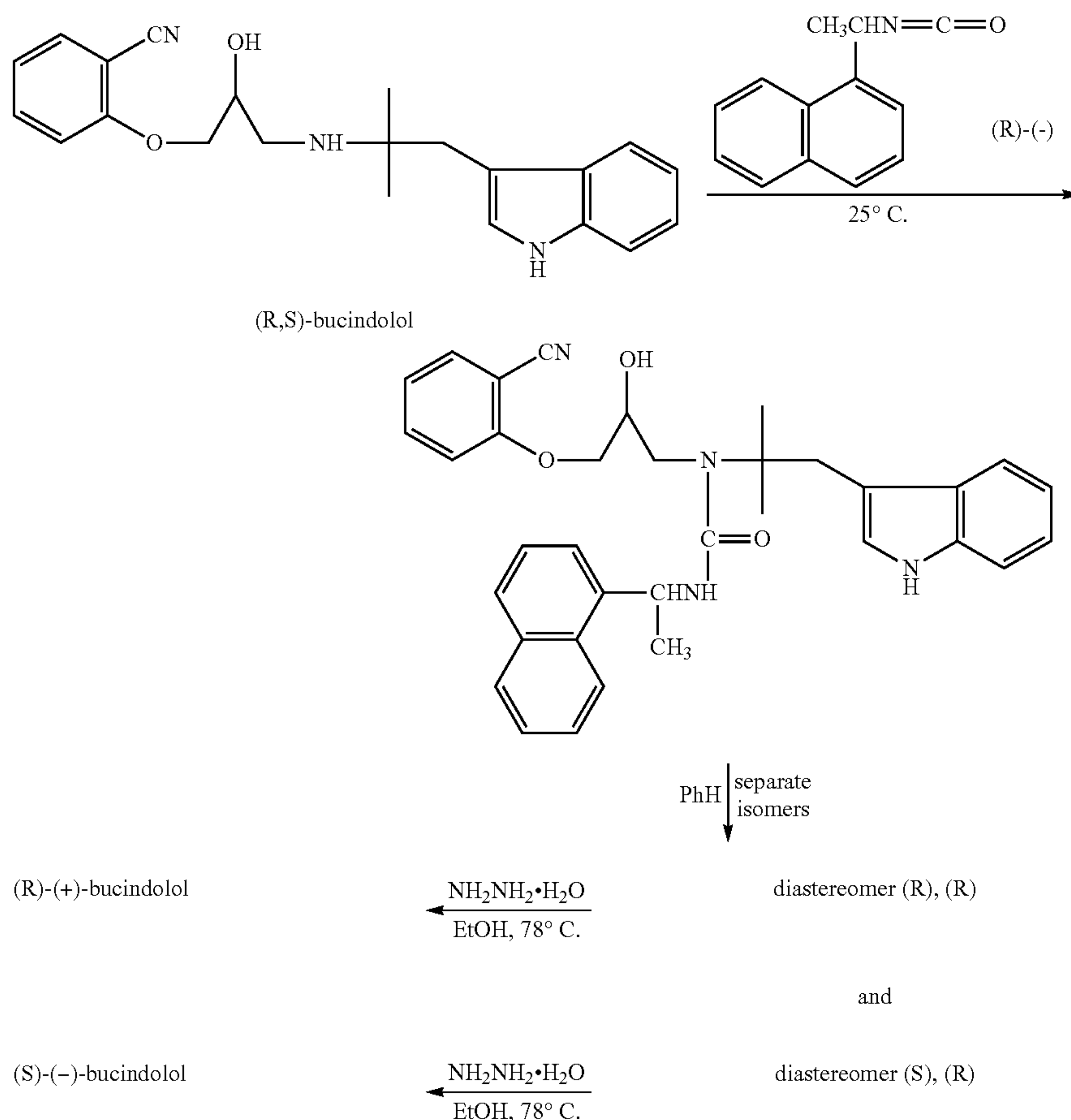
SCHEME 1
