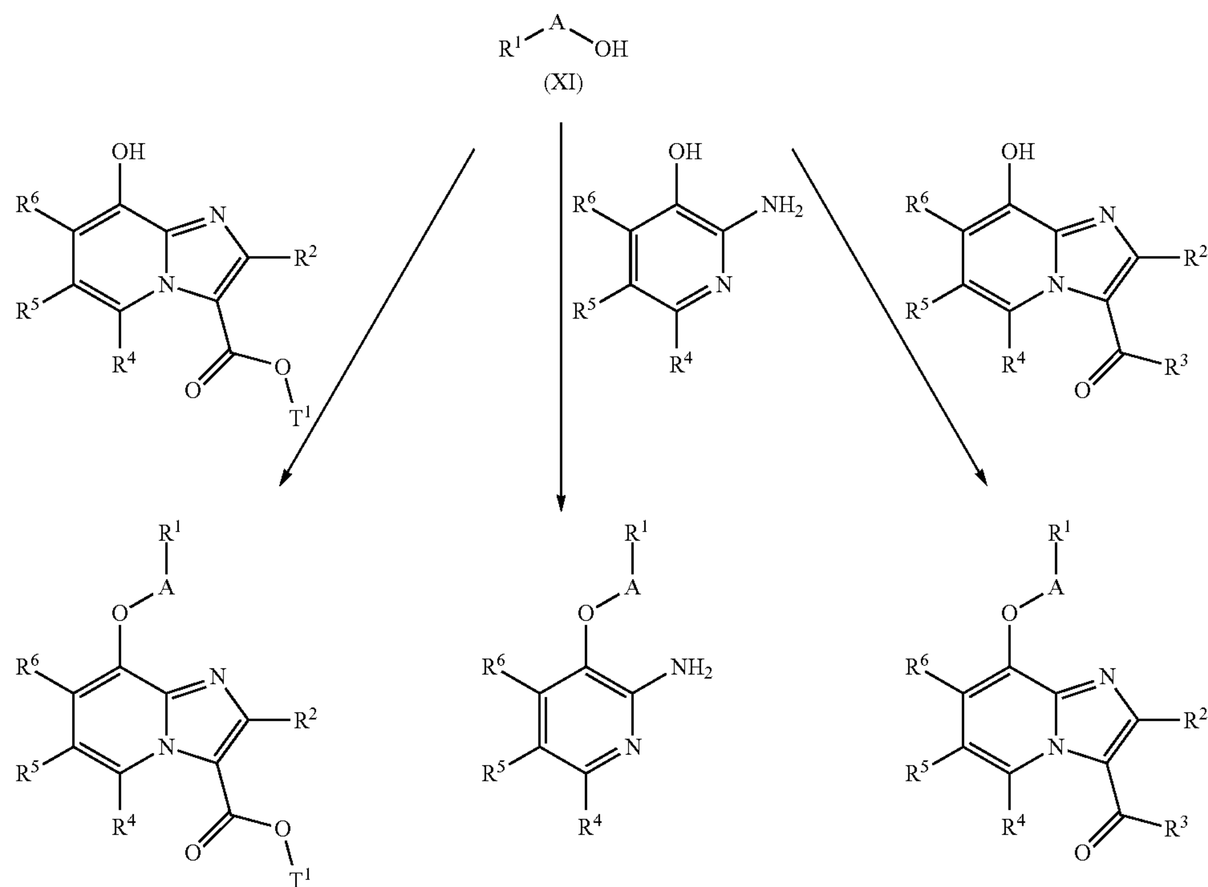
Scheme 5:
