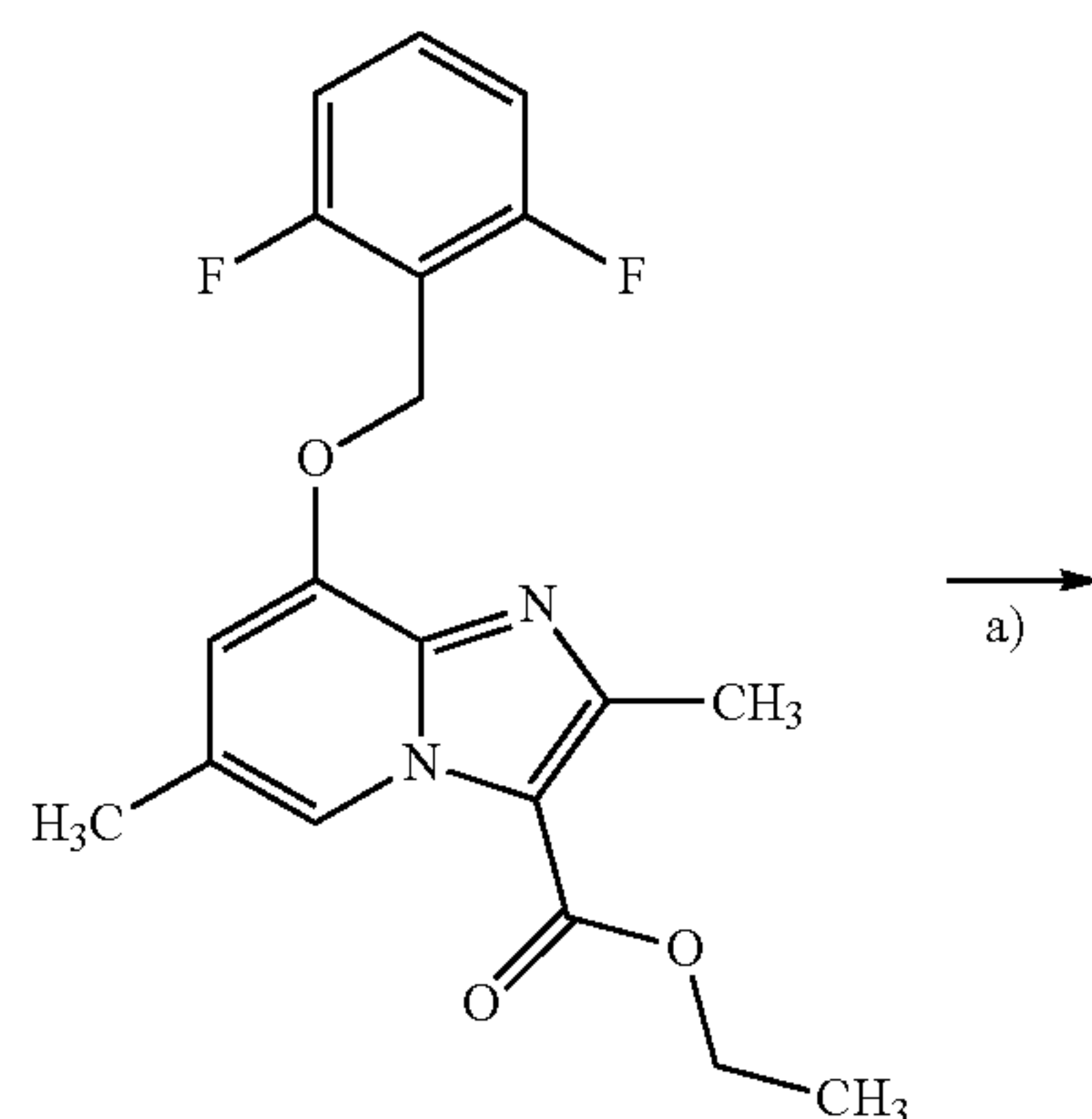
Scheme 1:
