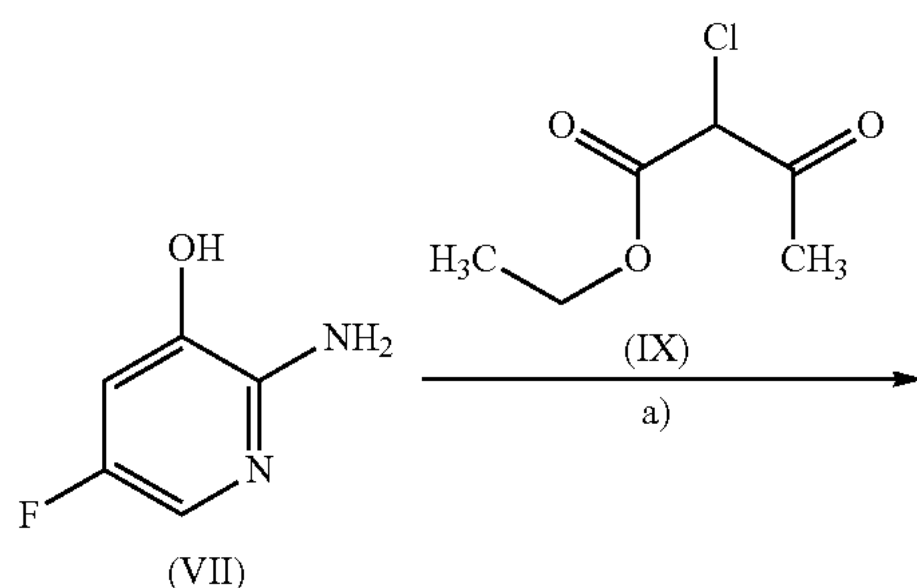
Scheme 4:
