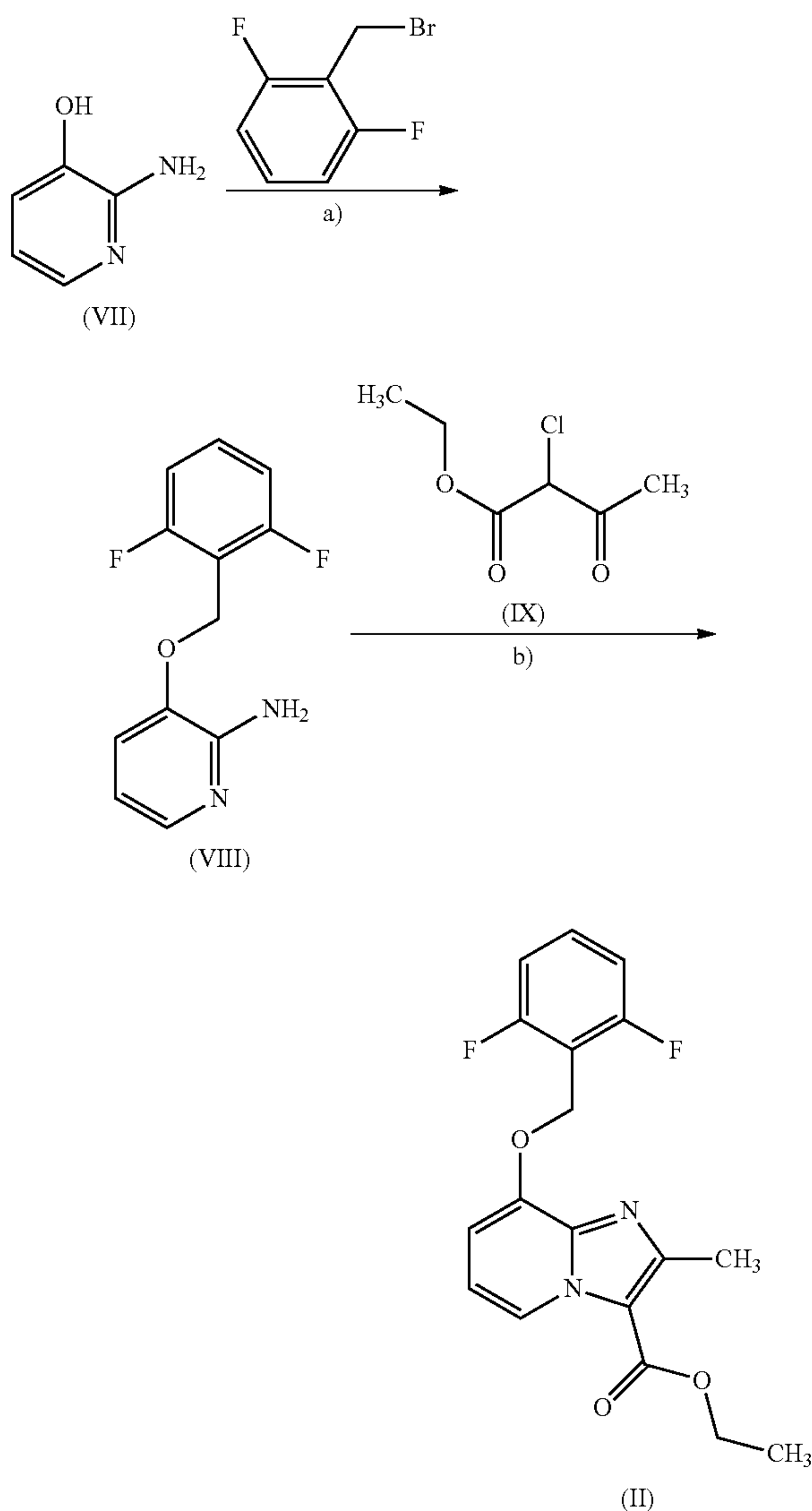
Scheme 3:
