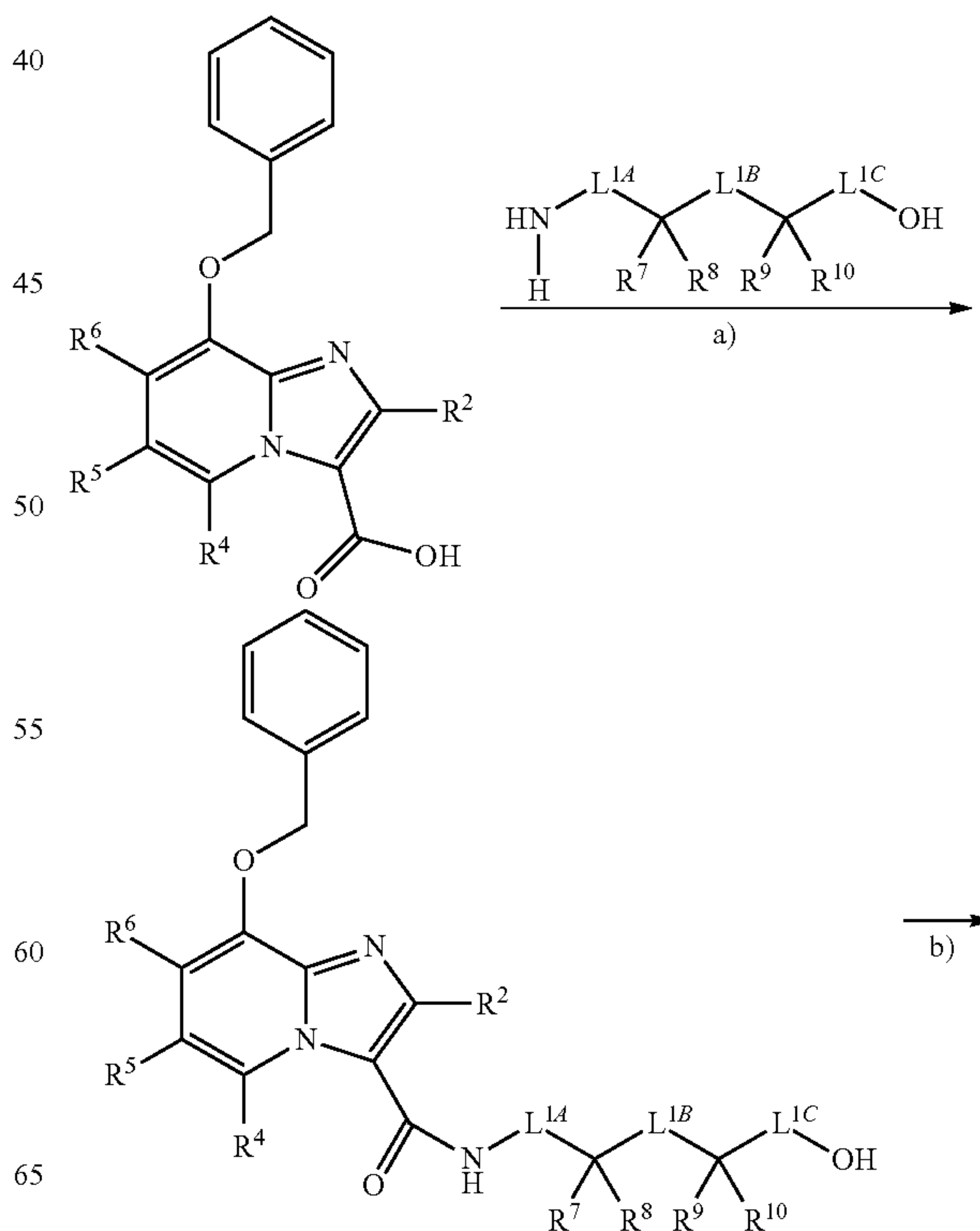
Scheme 2:
