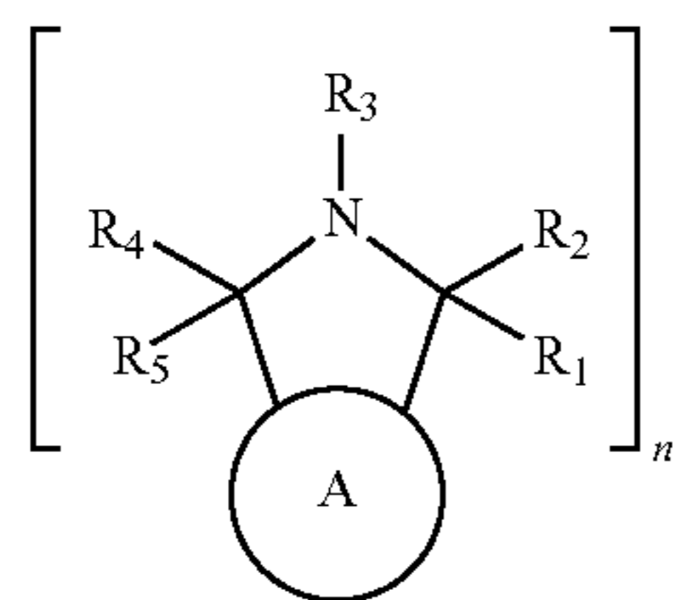
Prato Derivative
