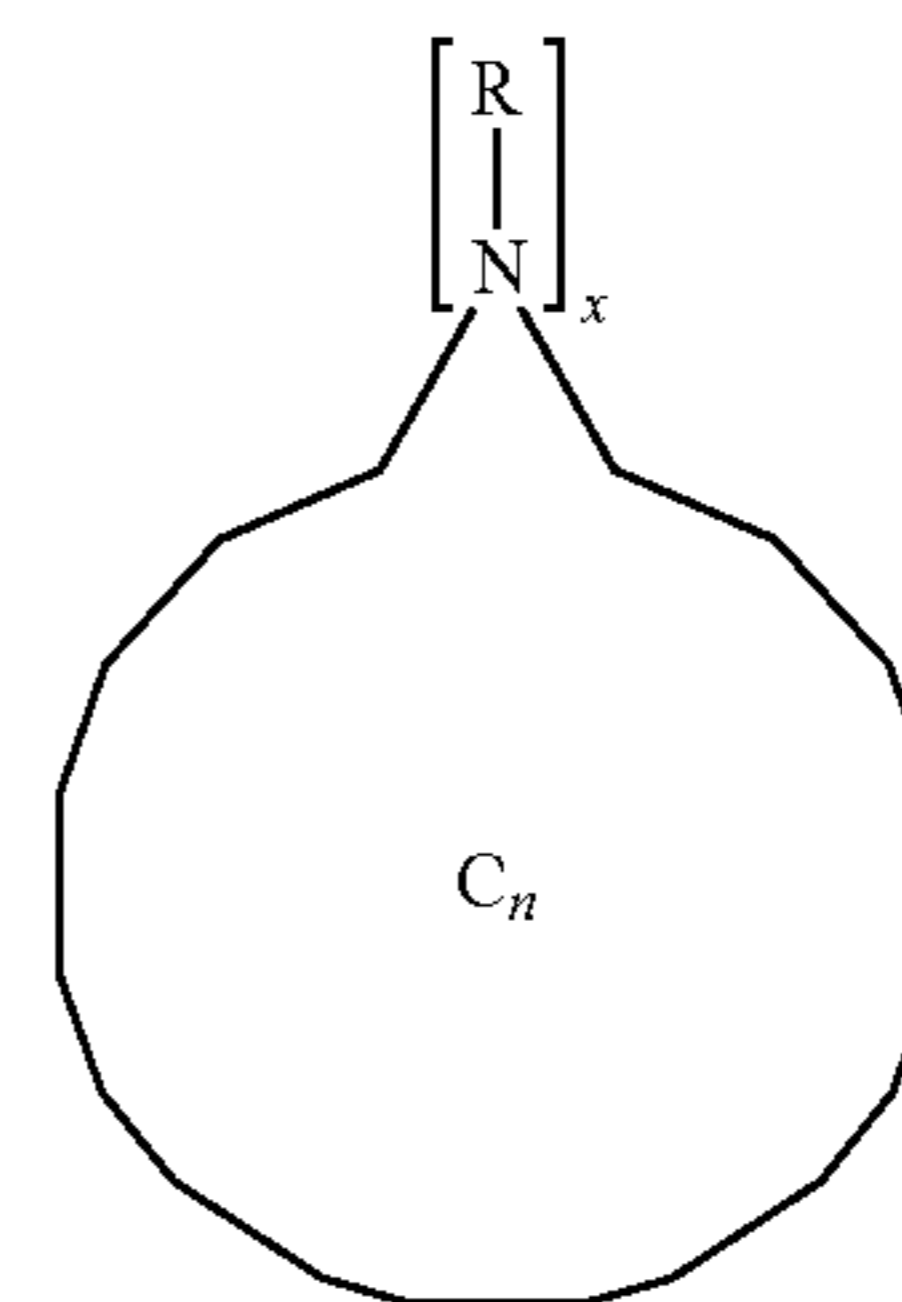
Azafulleroid
