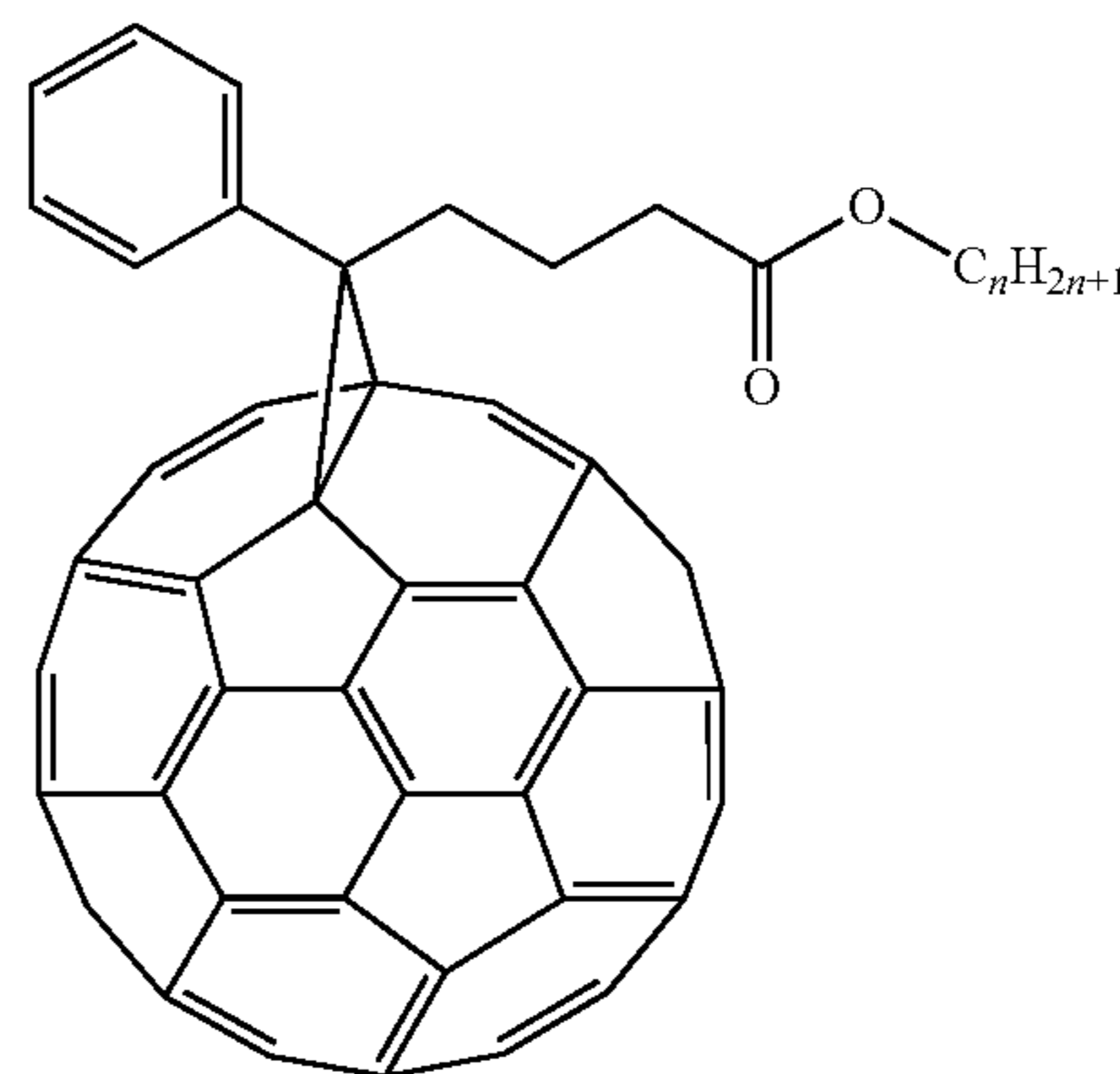
PCB- C_nH_{2n+1}
