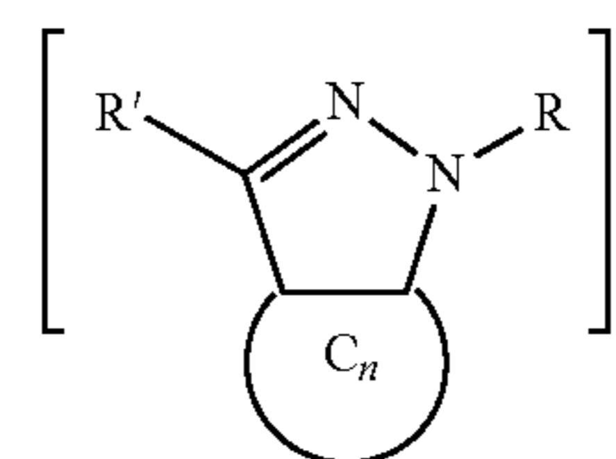
Diazoline
