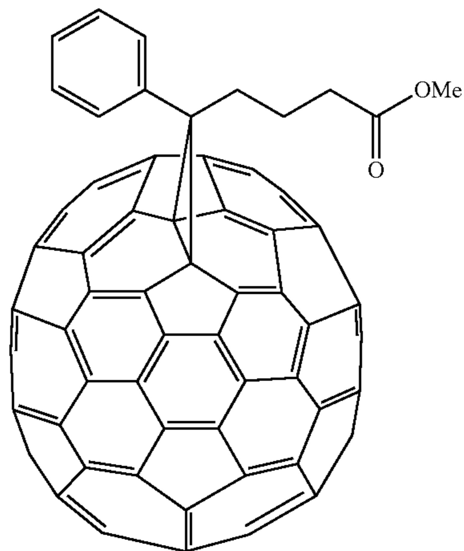
[70]PCBM
