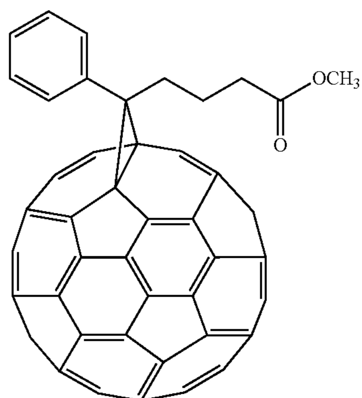
[60]PCBM
