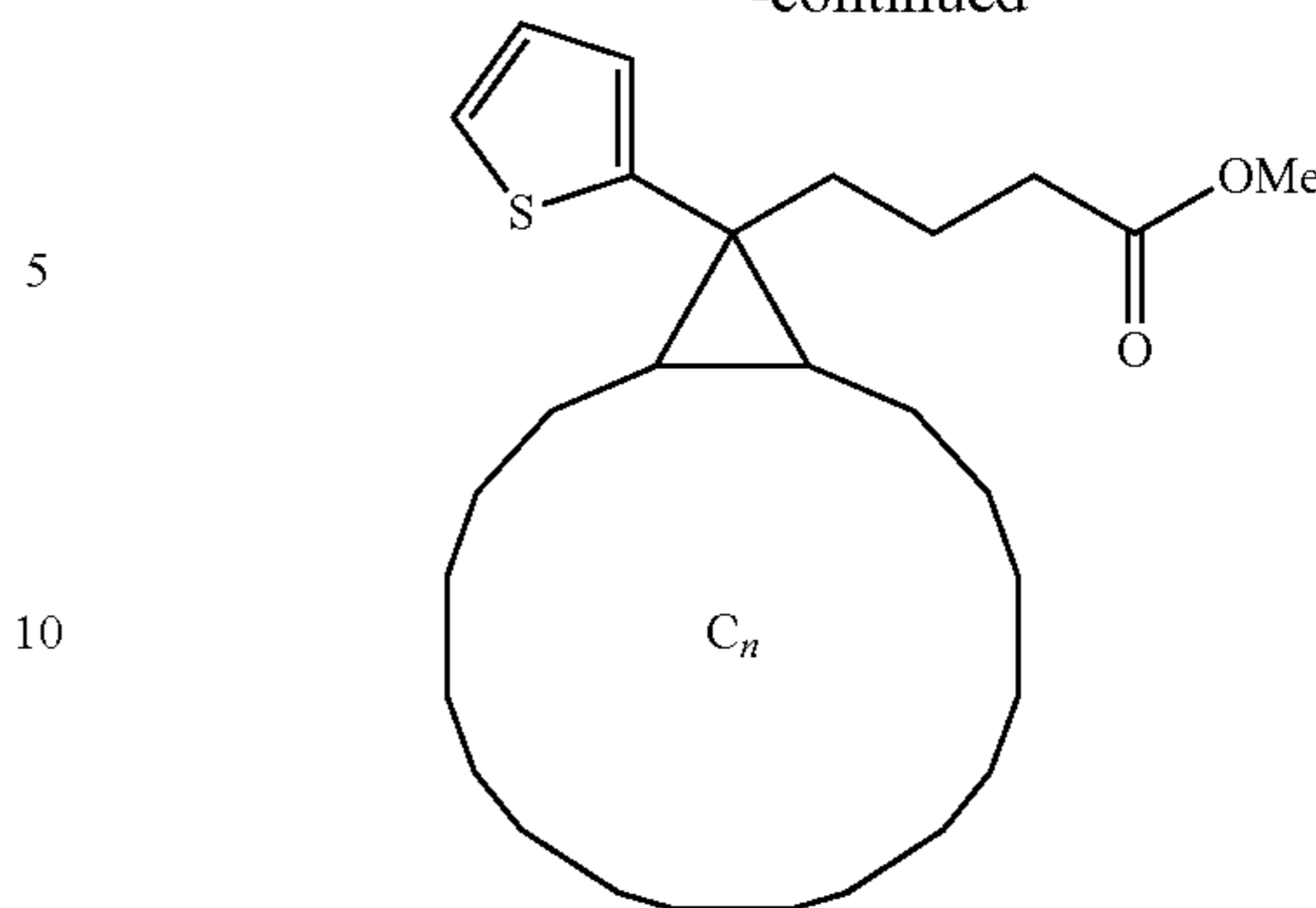
[ C_n ]ThCBM
