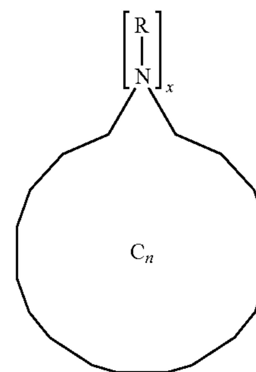
Azafulleroid
