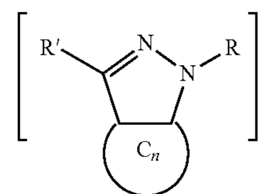
Diazoline
