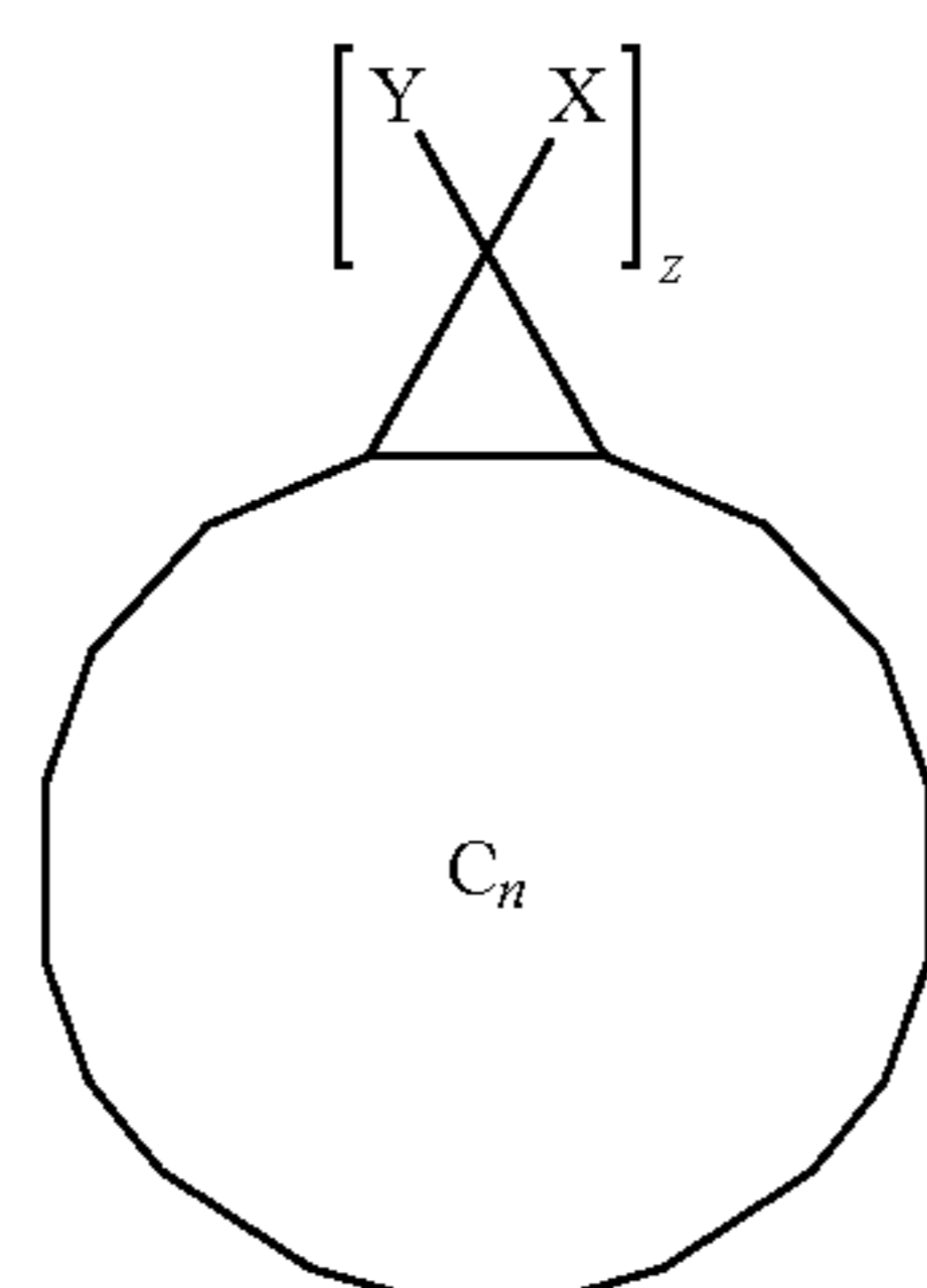
Bingel Derivative
