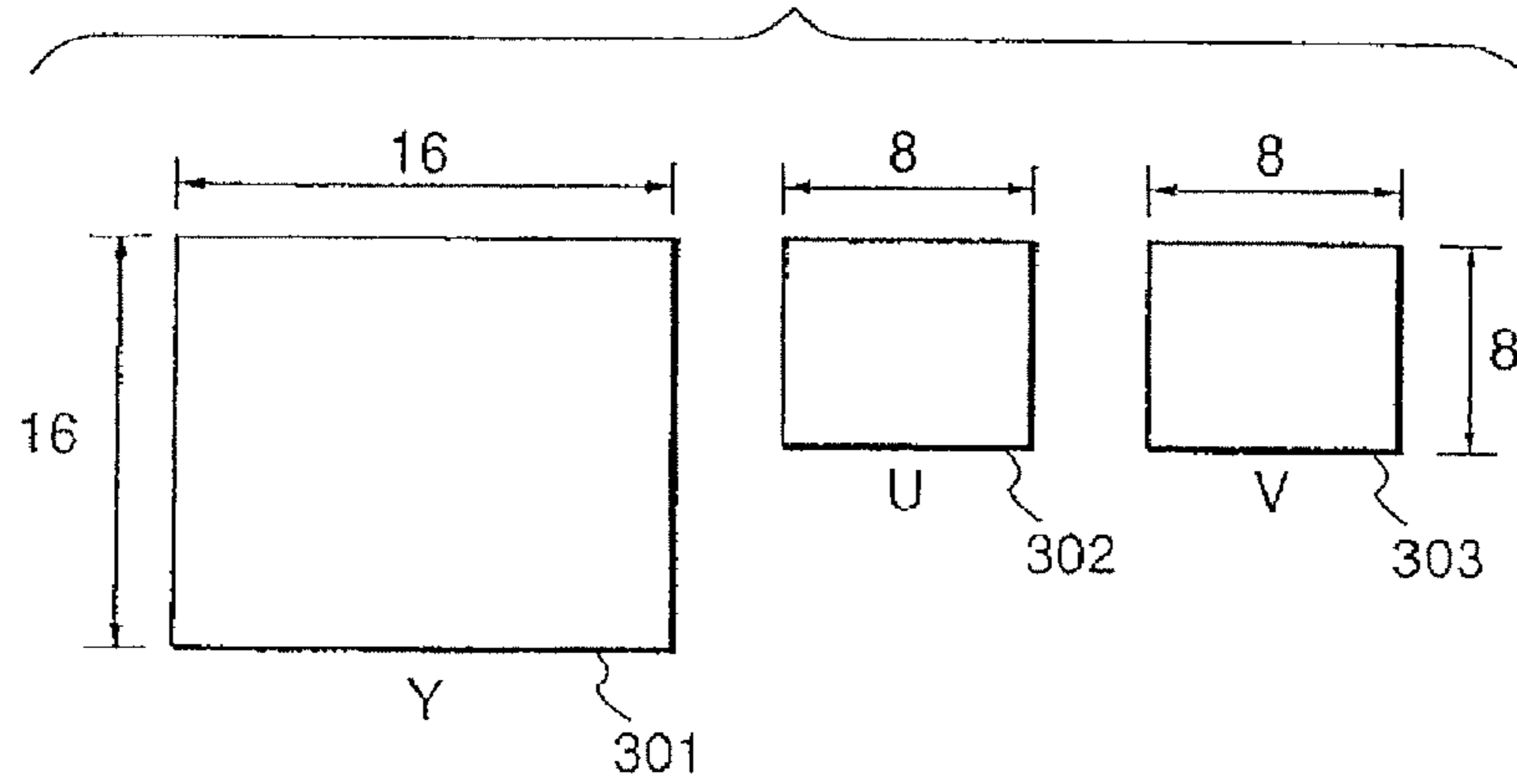
FIG. 3 (PRIOR ART)
