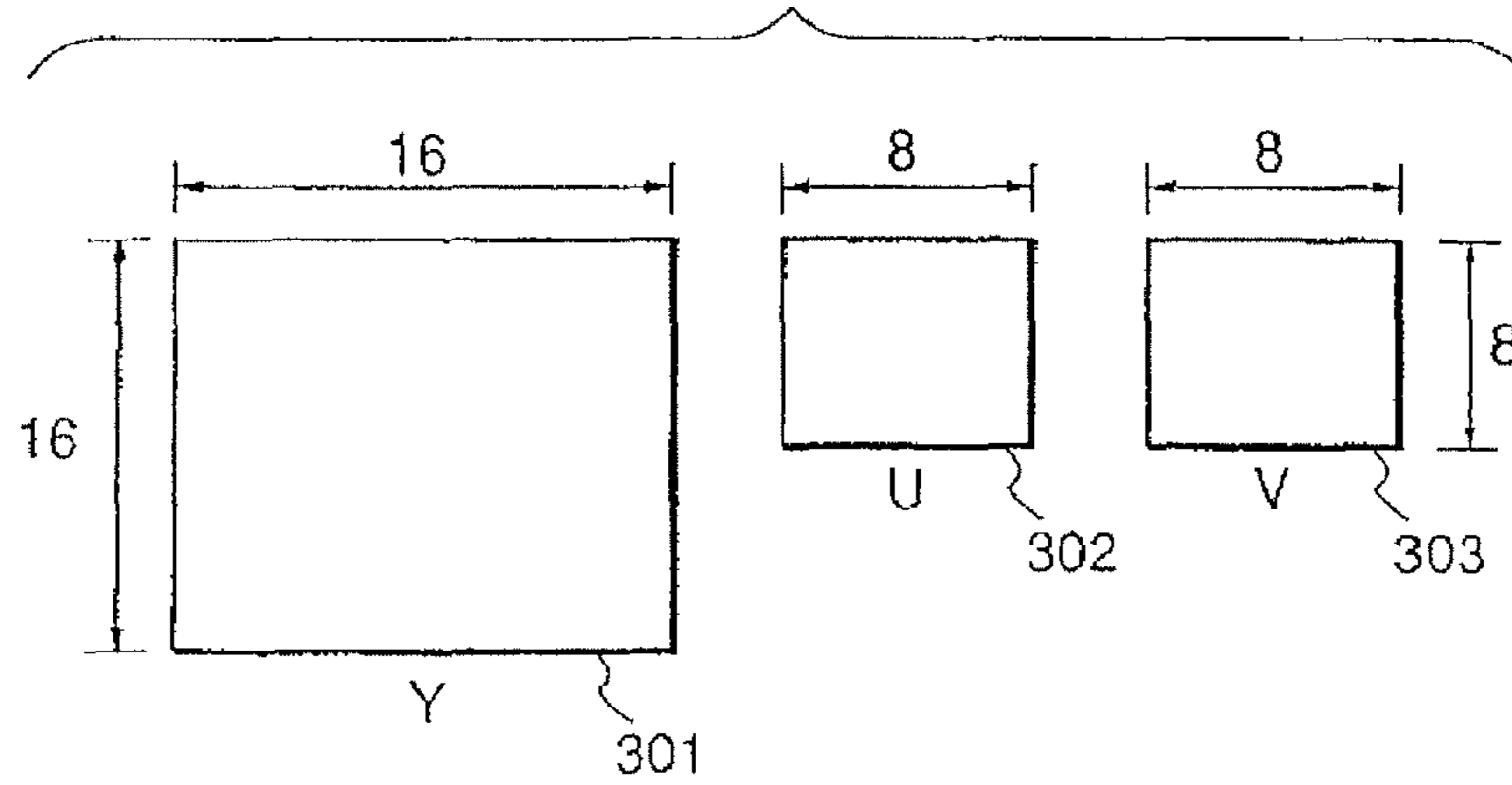
FIG. 3 (PRIOR ART)
