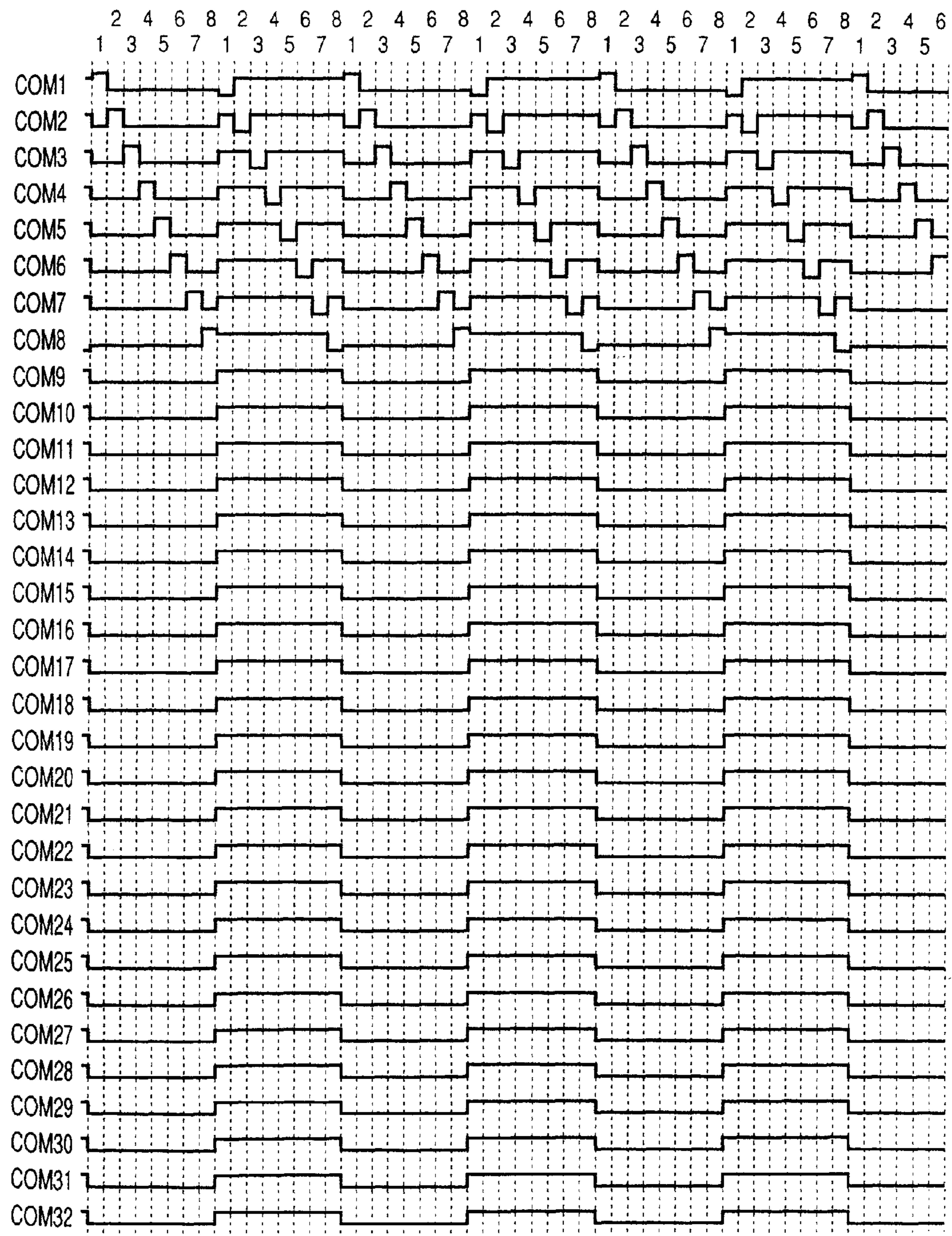
1/8 DUTY DRIVE (COM1~COM8)
