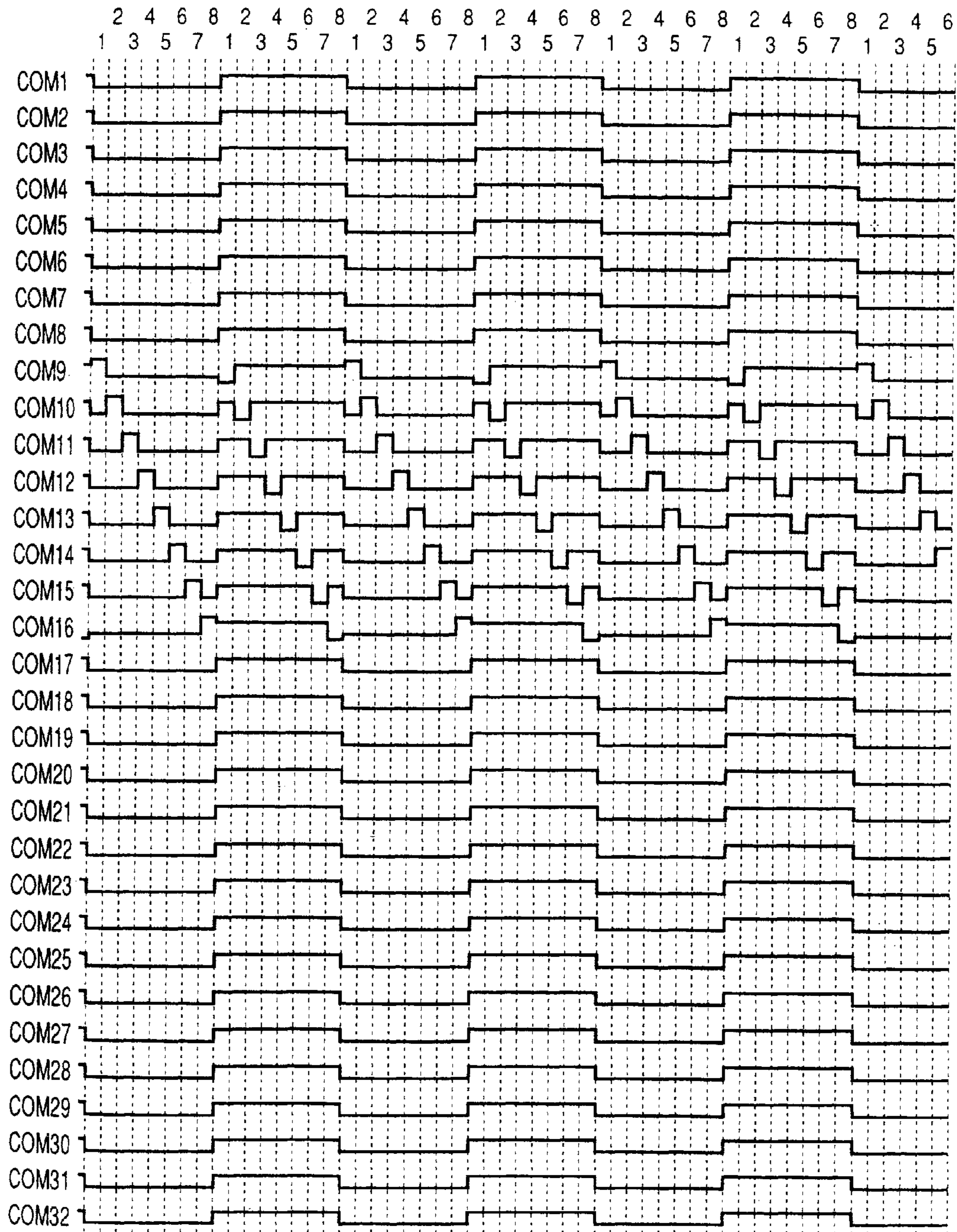
1/8 DUTY DRIVE (COM9~COM16)
