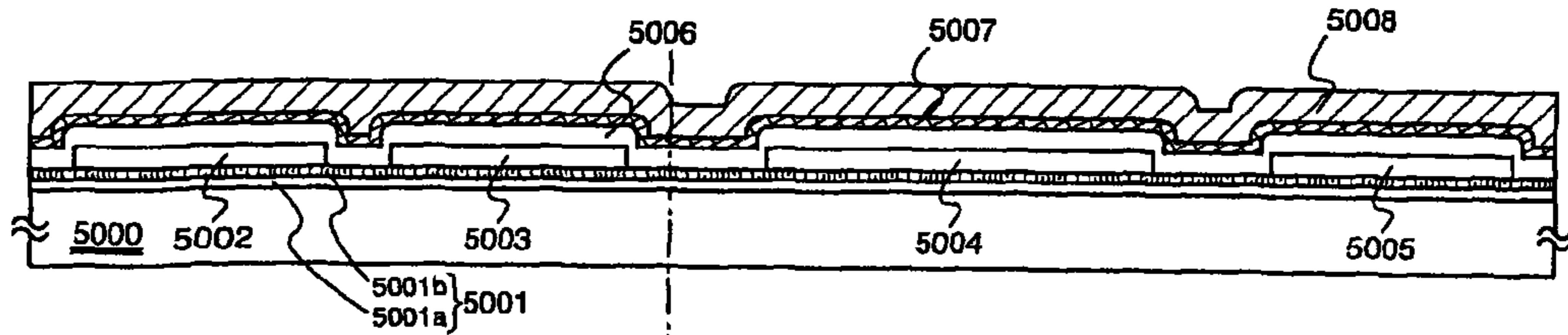
Fig. 13A forming base insulating film/forming semiconductor film/forming gate insulating film/forming first and second conductive layer
