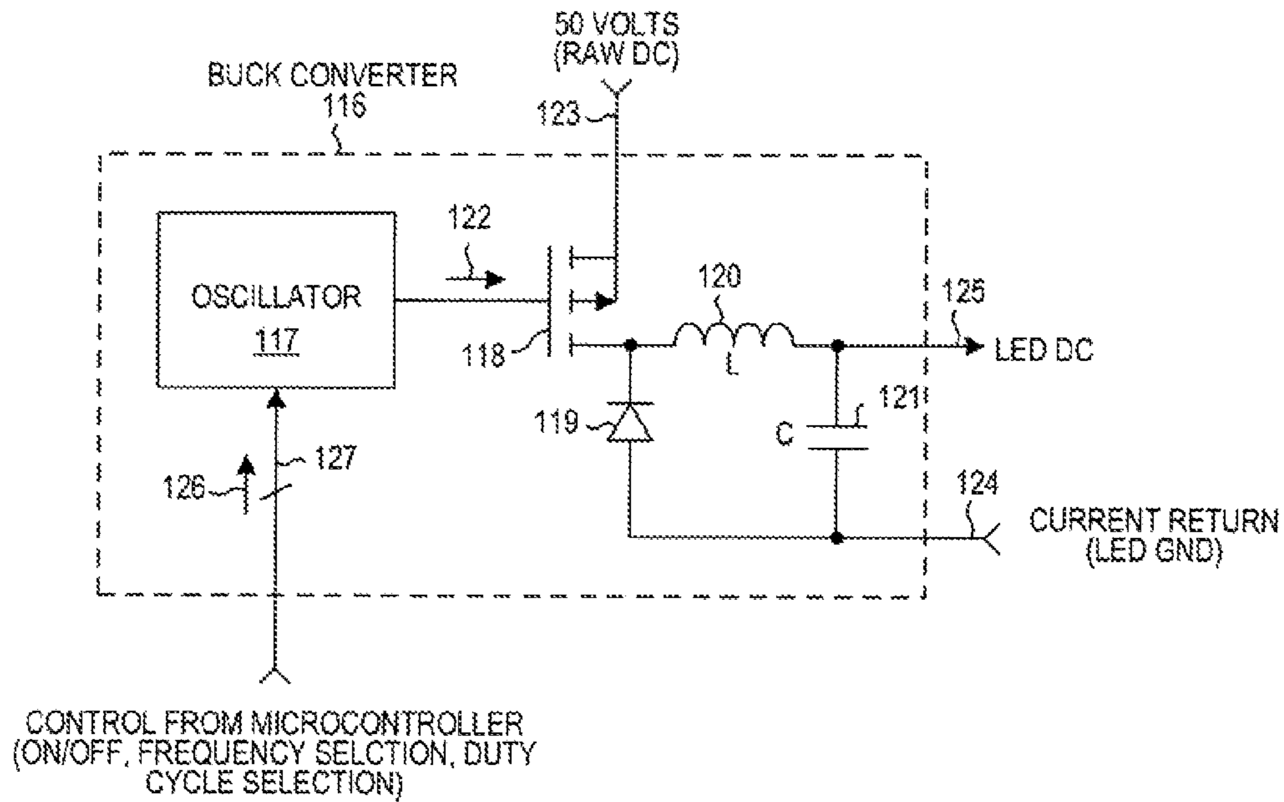
BUCK CONVERTER
