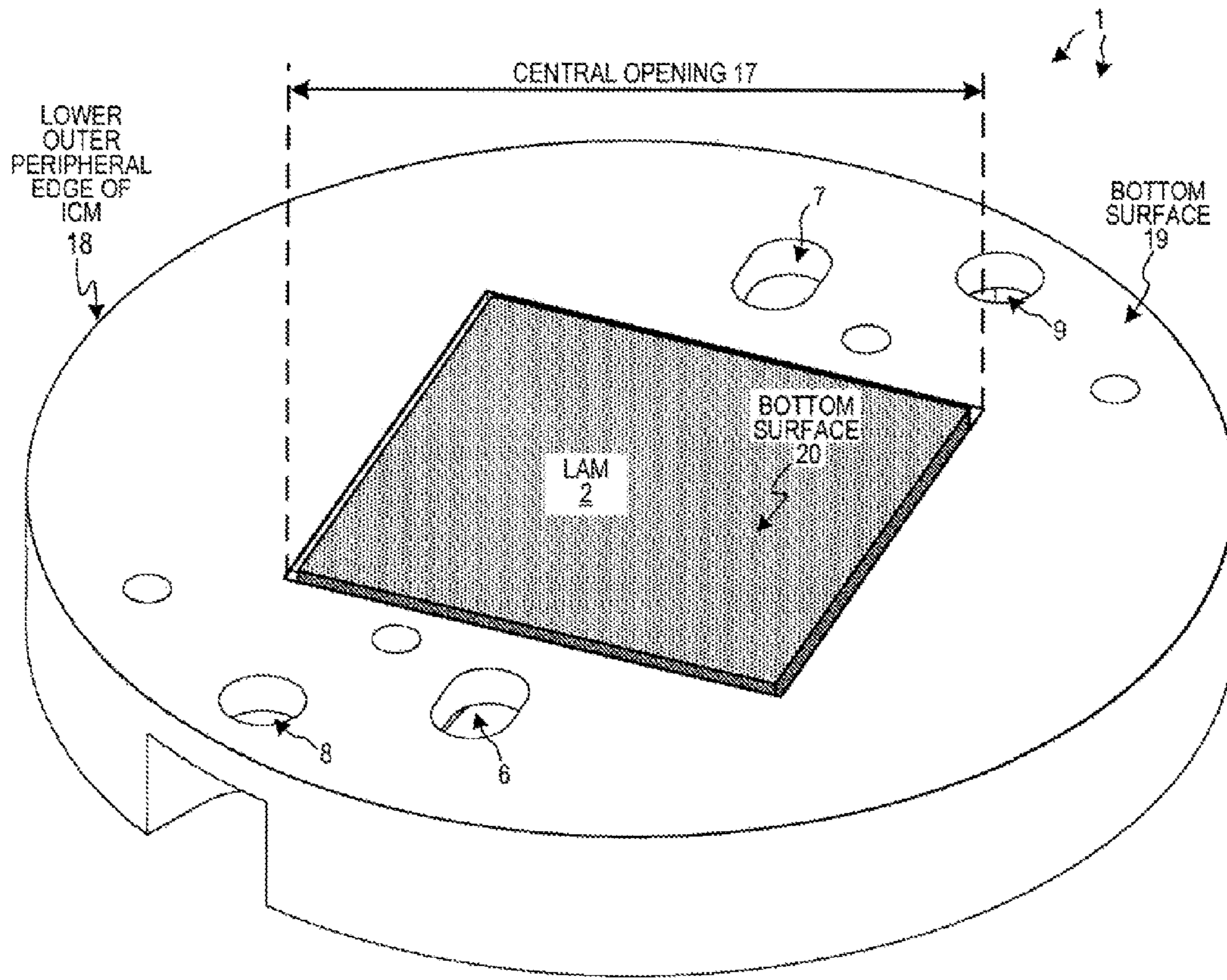
VIEW OF BOTTOM OF LAM/ICM ASSEMBLY (PERSPECTIVE VIEW)
