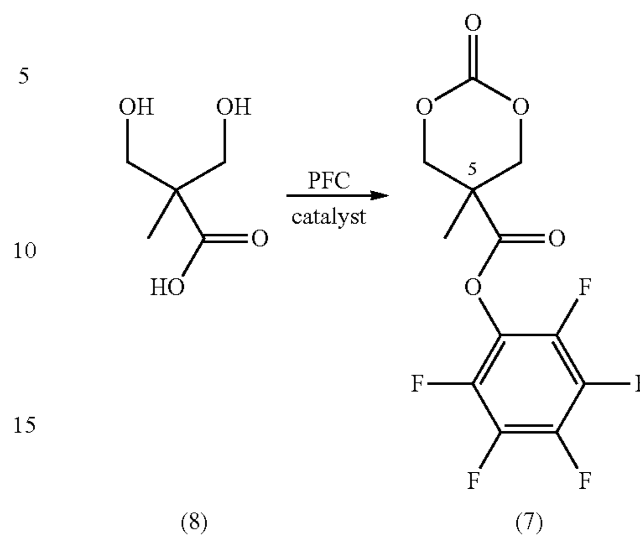
Scheme 2.
