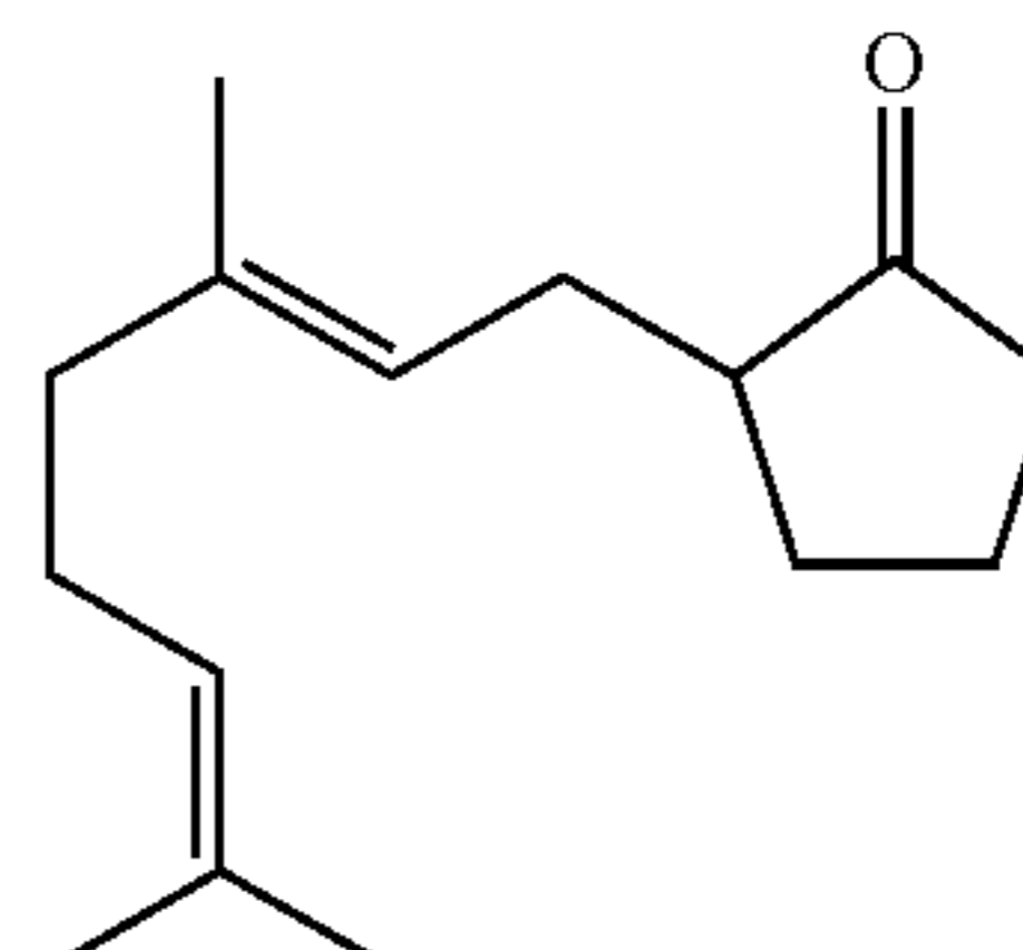
bisabolol (CAS #515-69-5)
