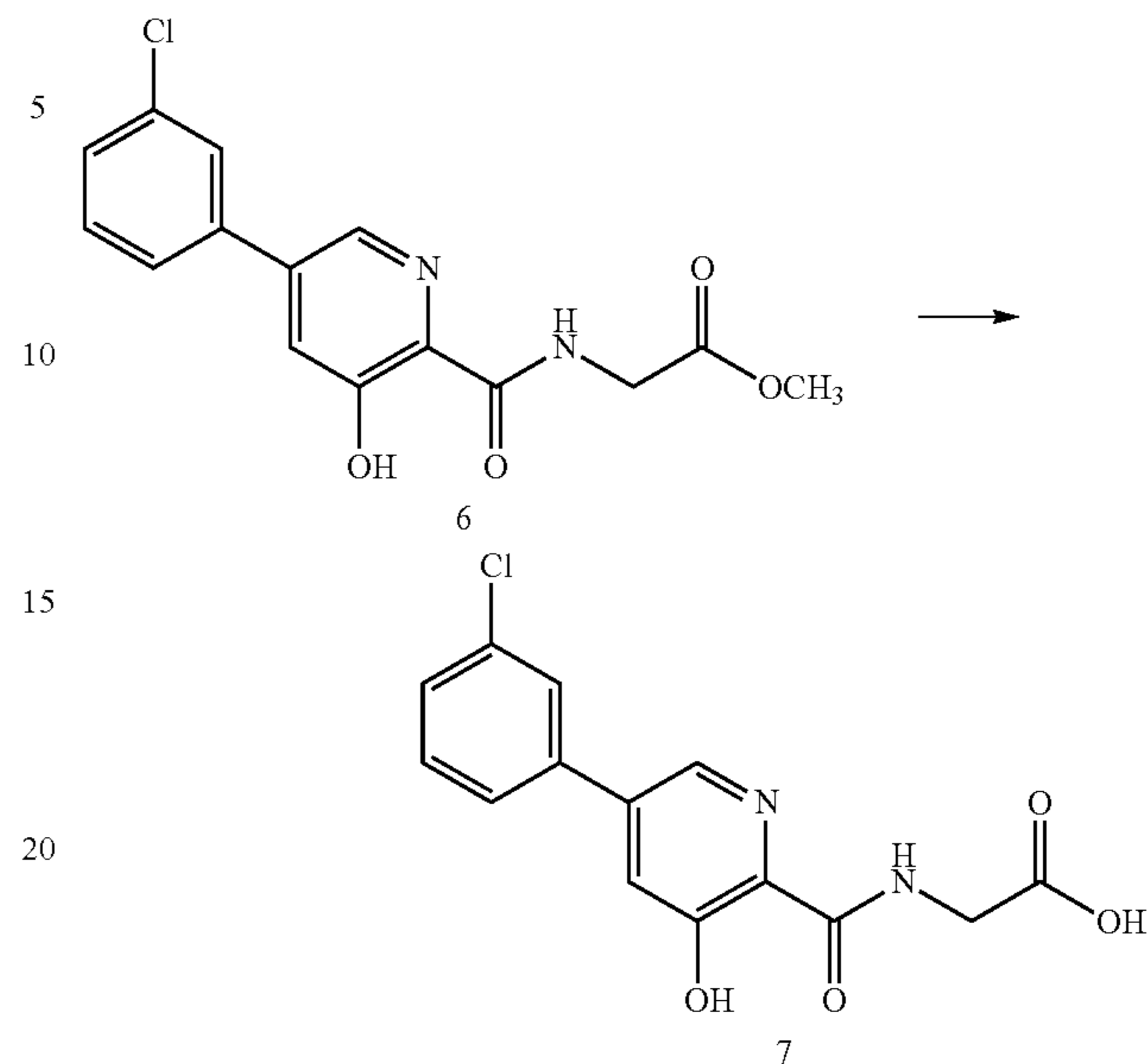
Scheme II
