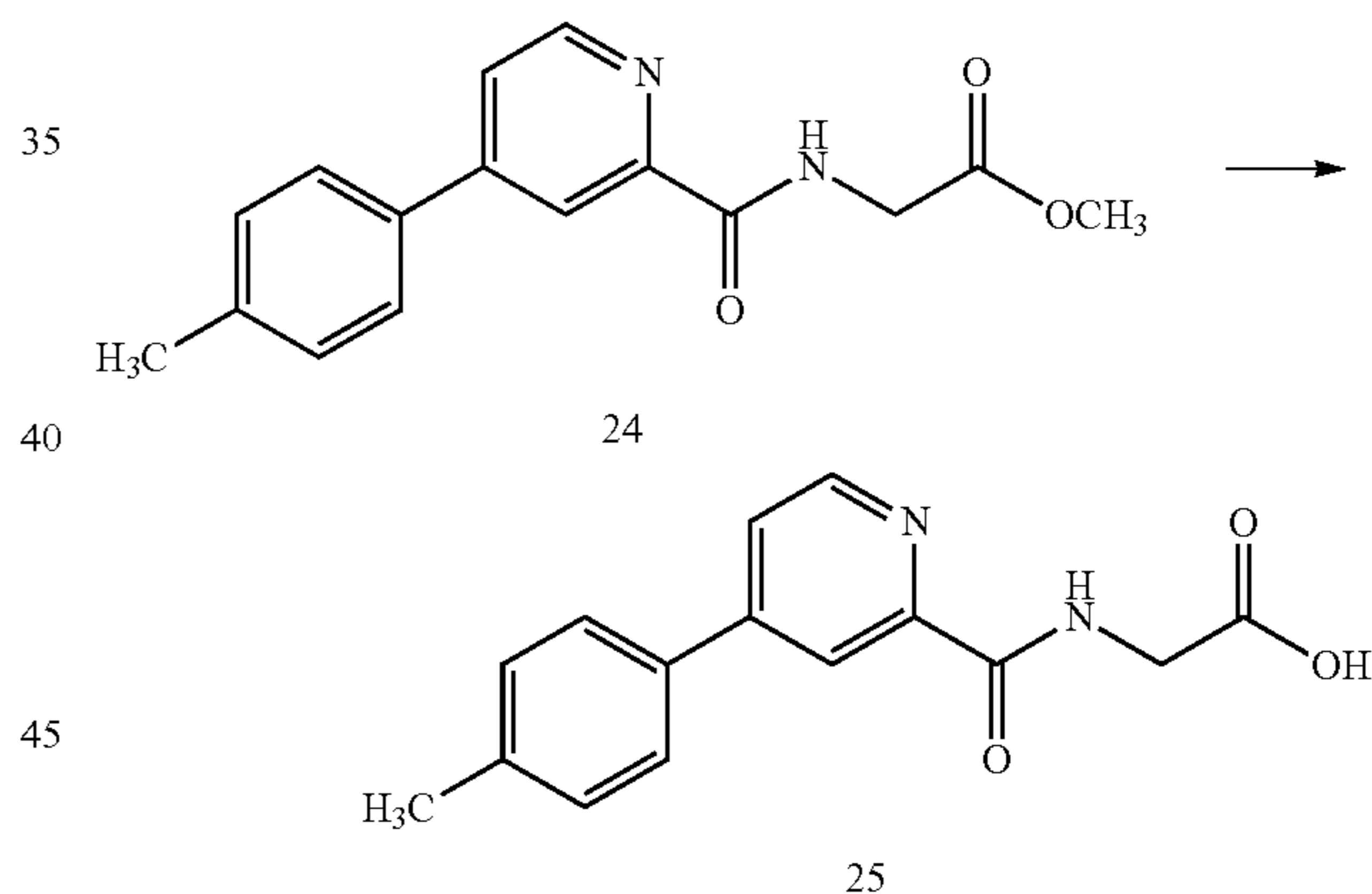
Scheme XIII
