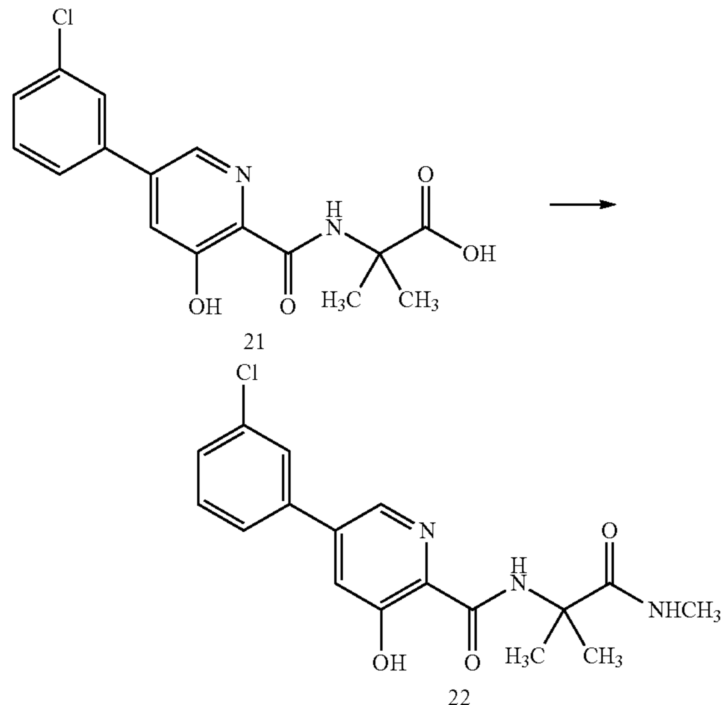
Scheme XI
