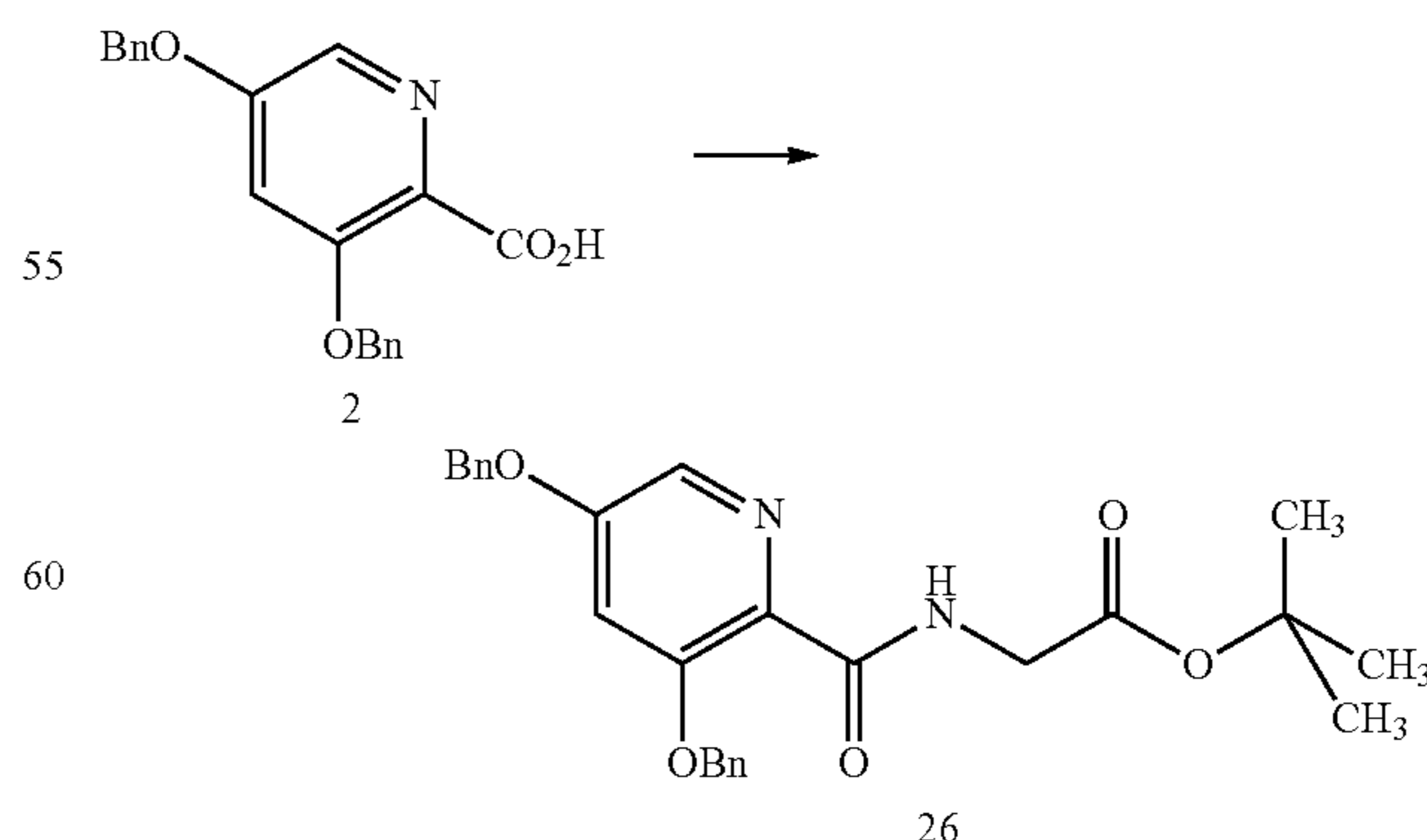
Scheme XIV
