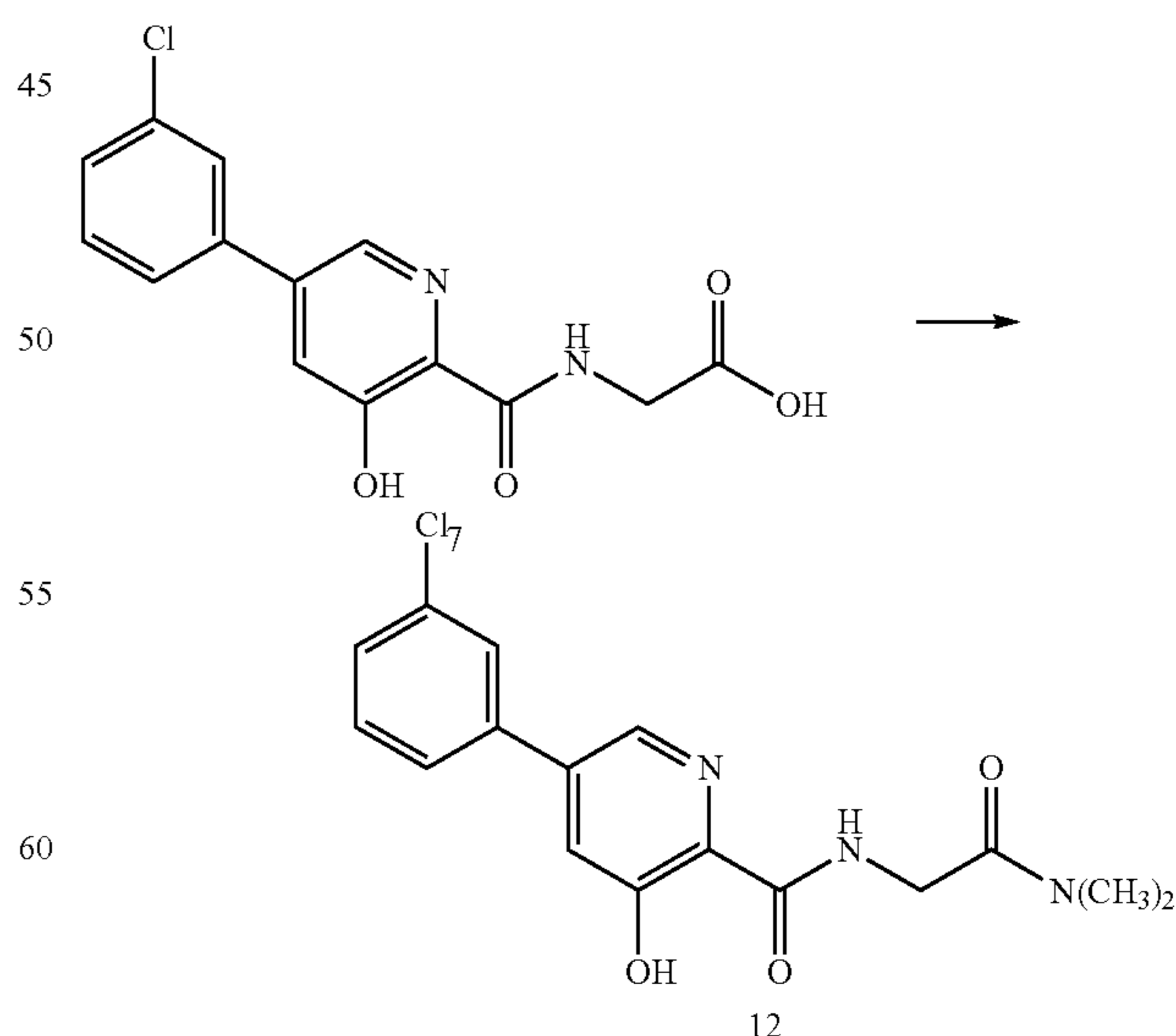
Scheme VII
