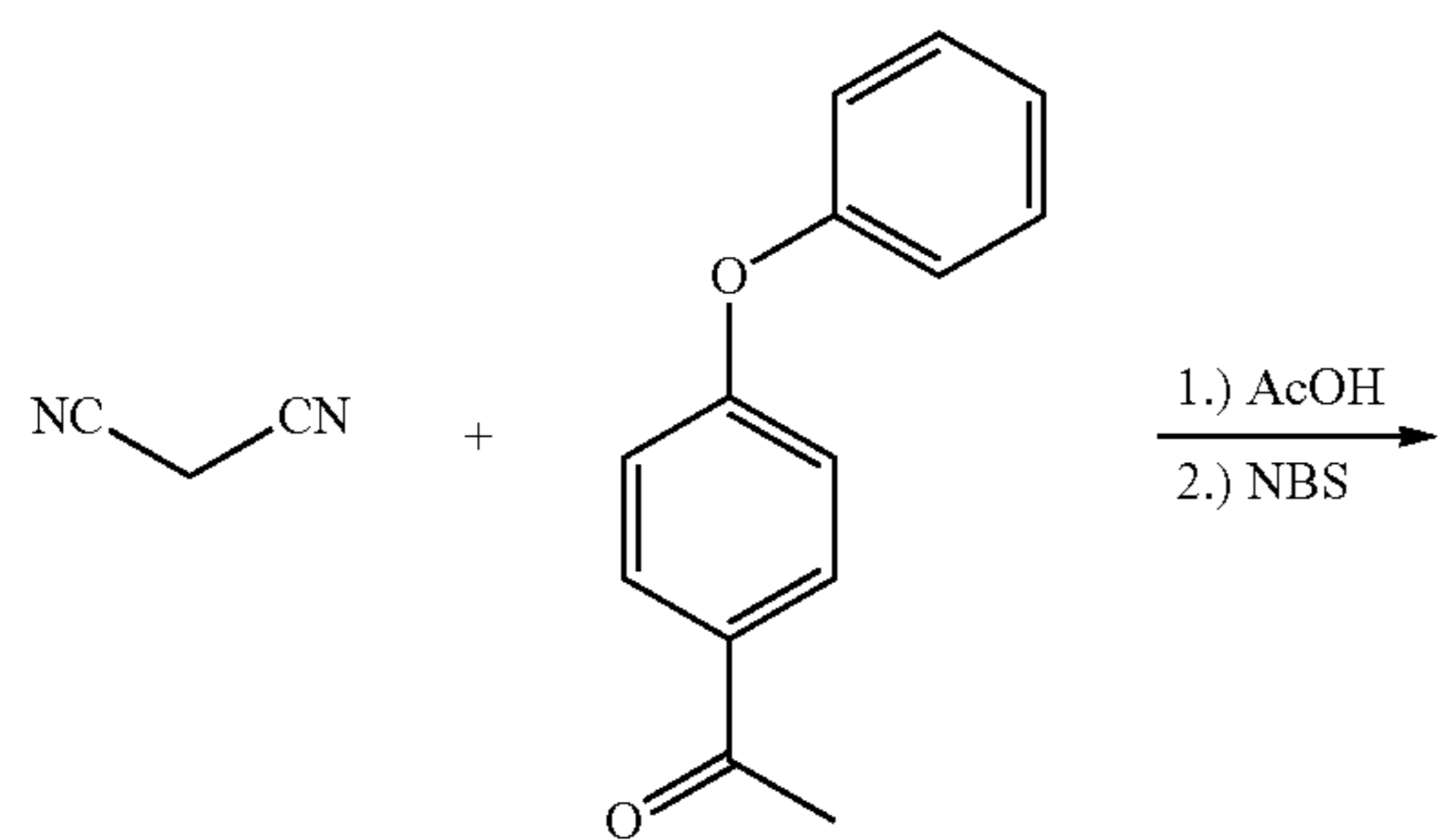
Scheme IV.
