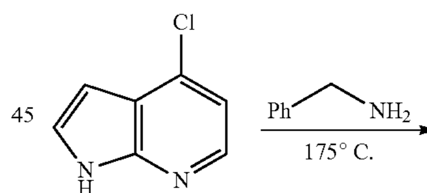
Scheme V.
