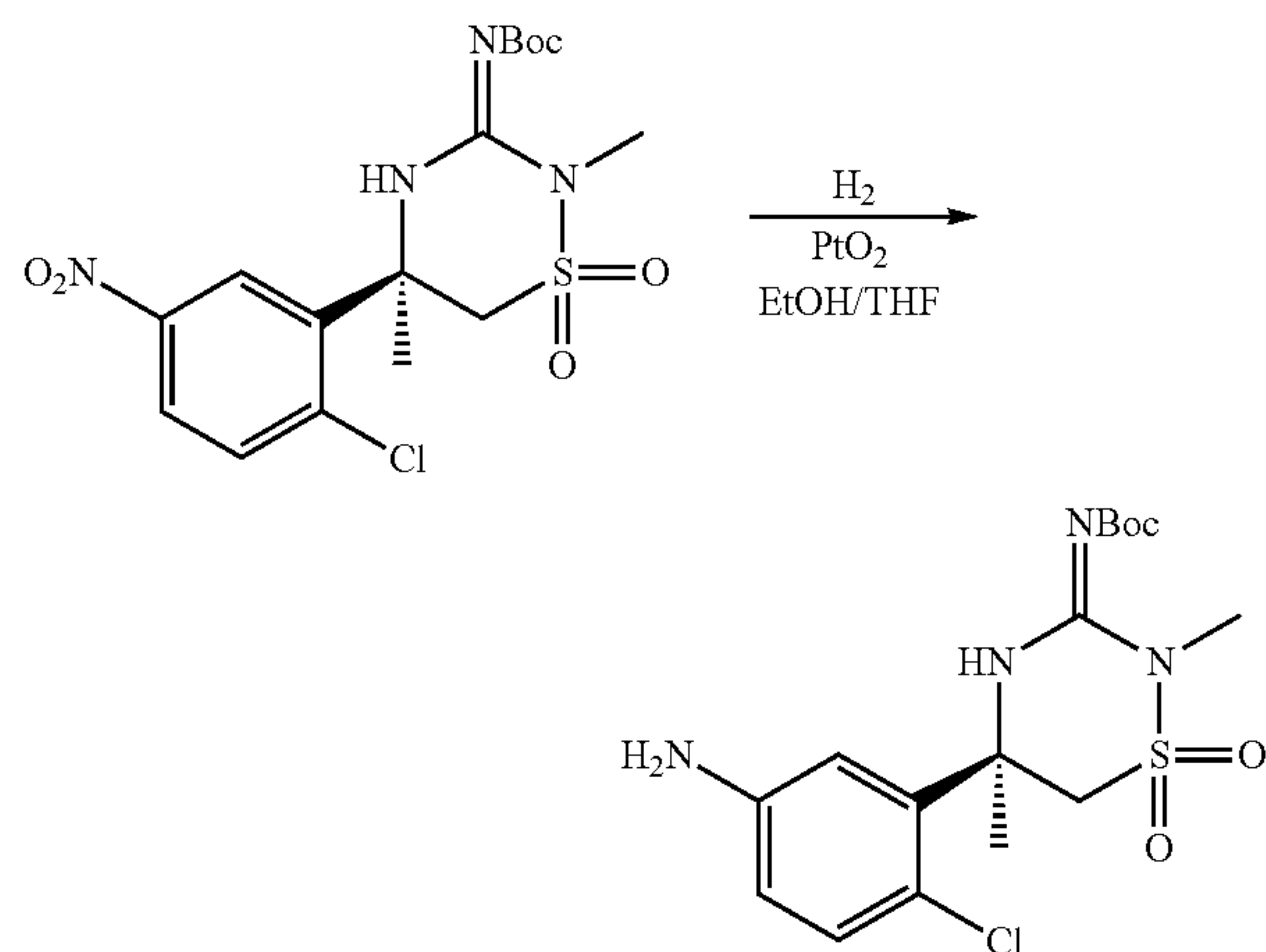
Scheme 11a:
