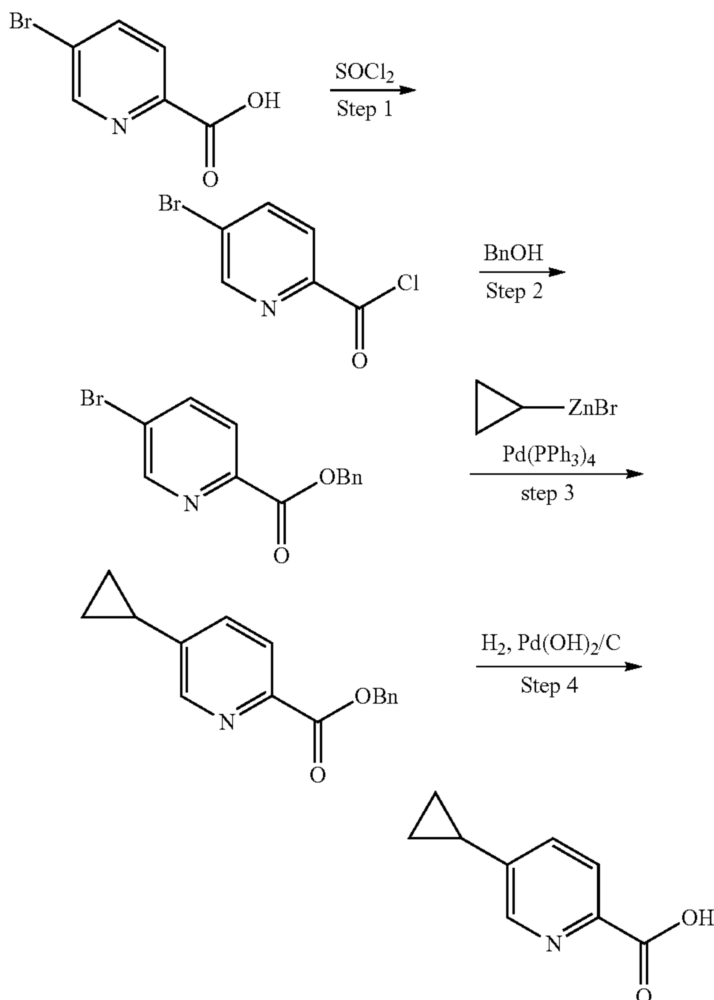
Scheme 11u:
