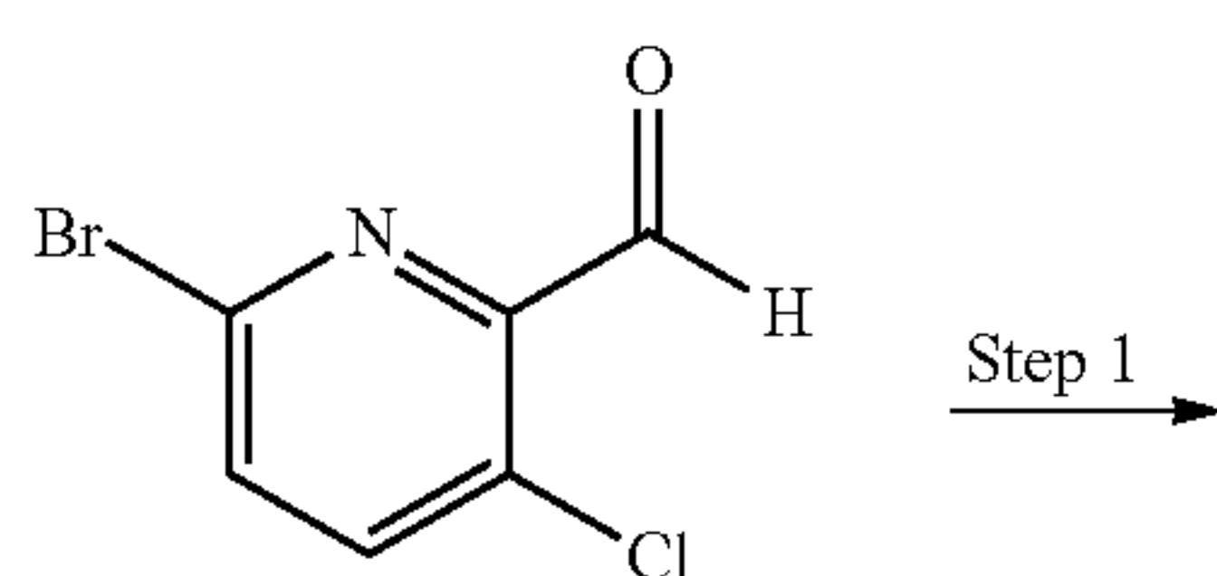
Scheme 2b:
