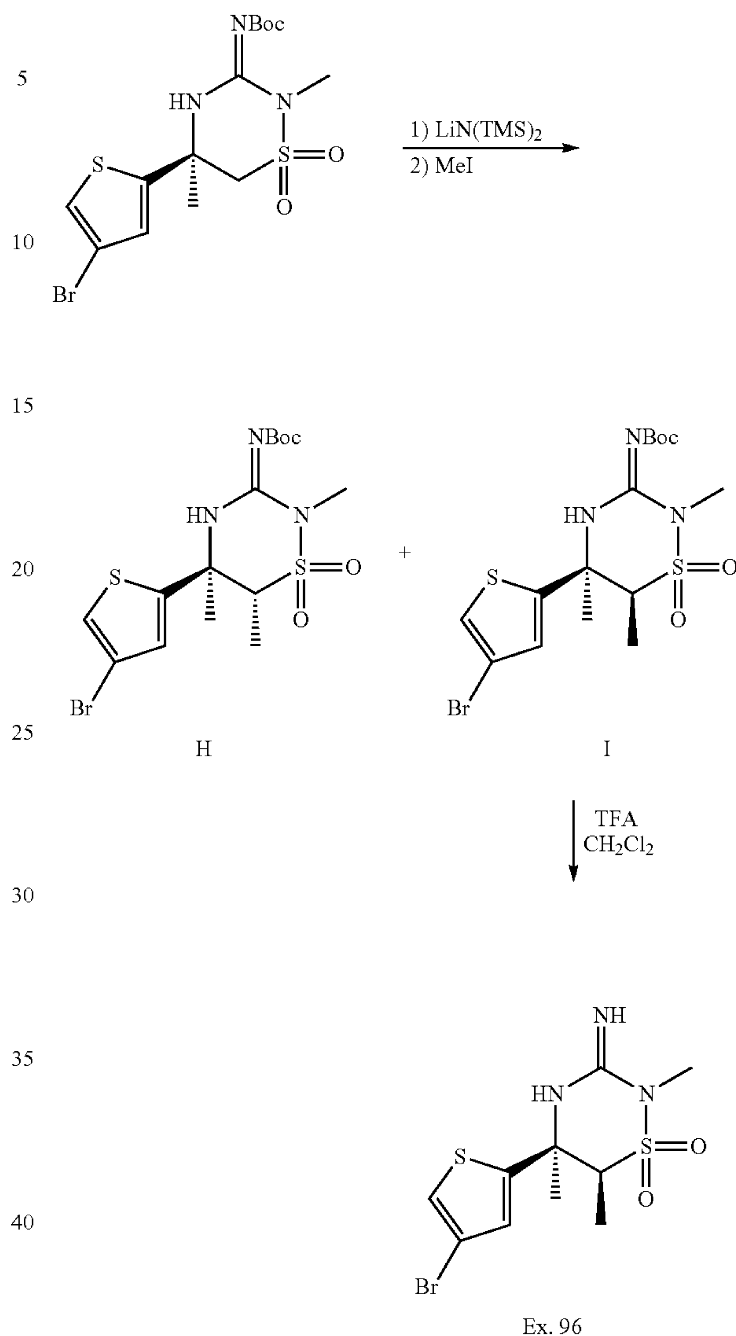
Scheme 16:
