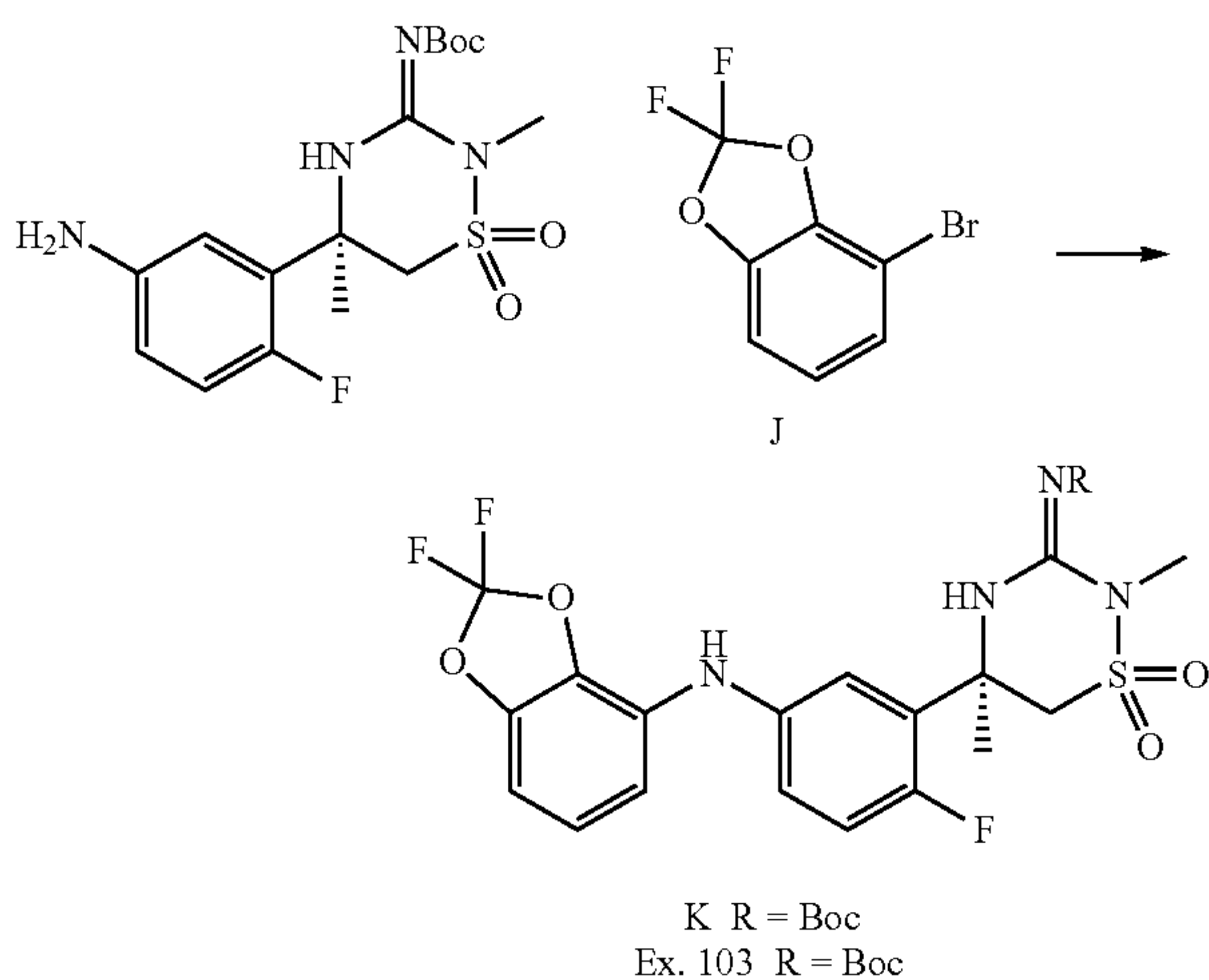
Scheme 18:
