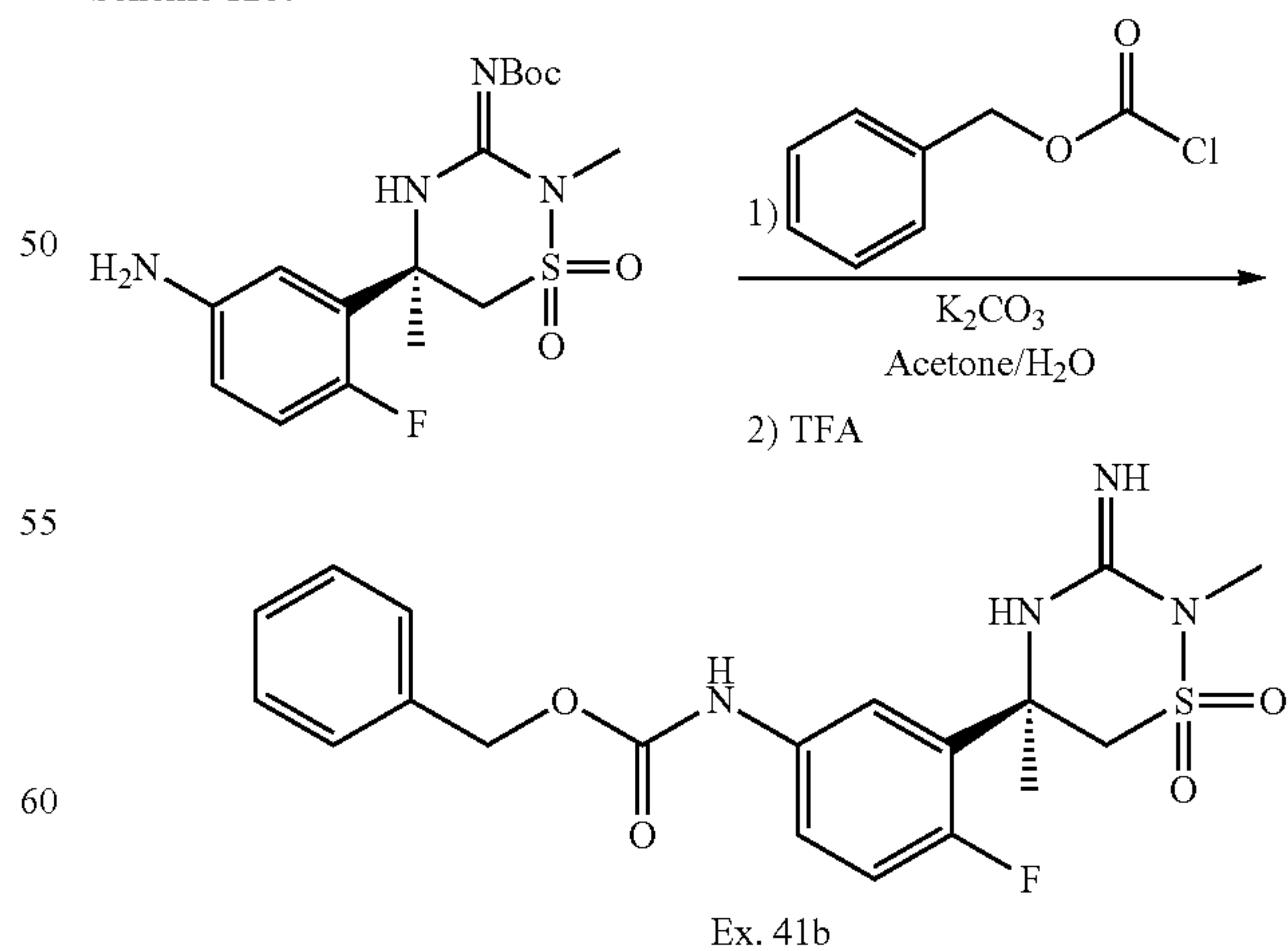
Scheme 12b:
