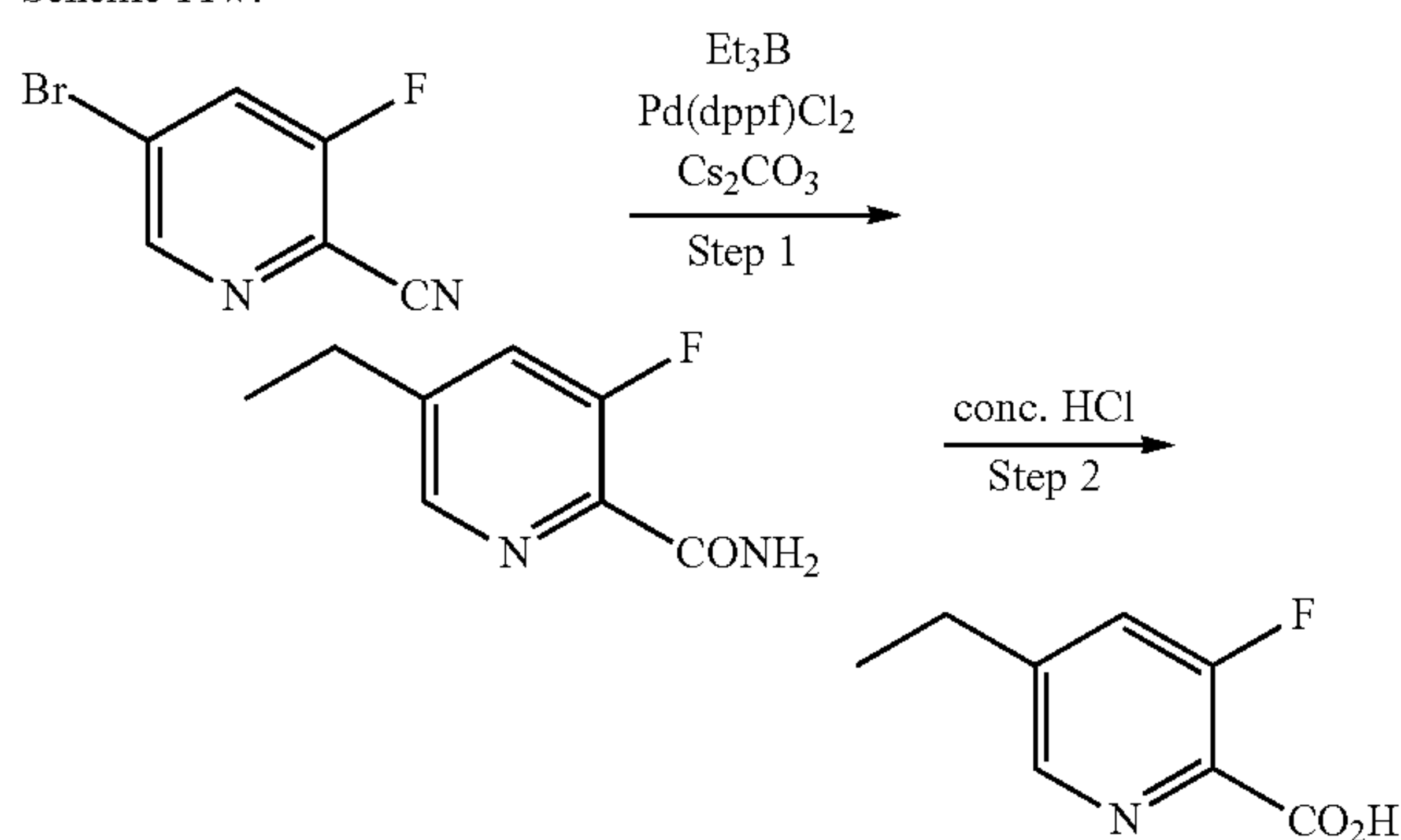
Scheme 11w:
