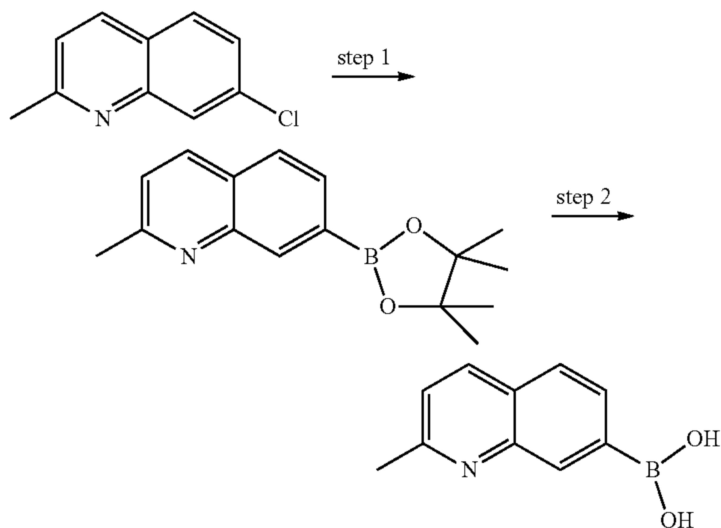
Scheme 29:
