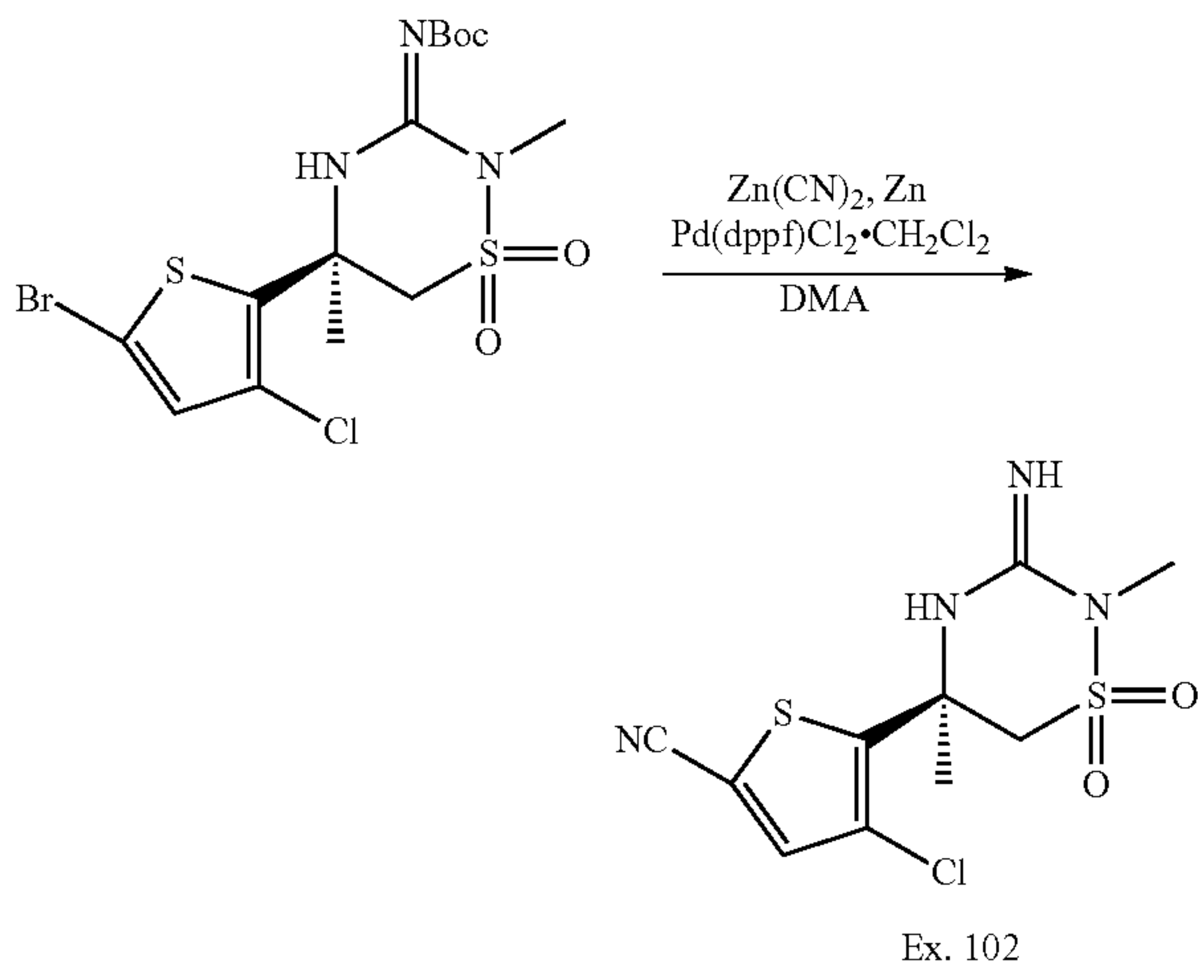
Scheme 17:
