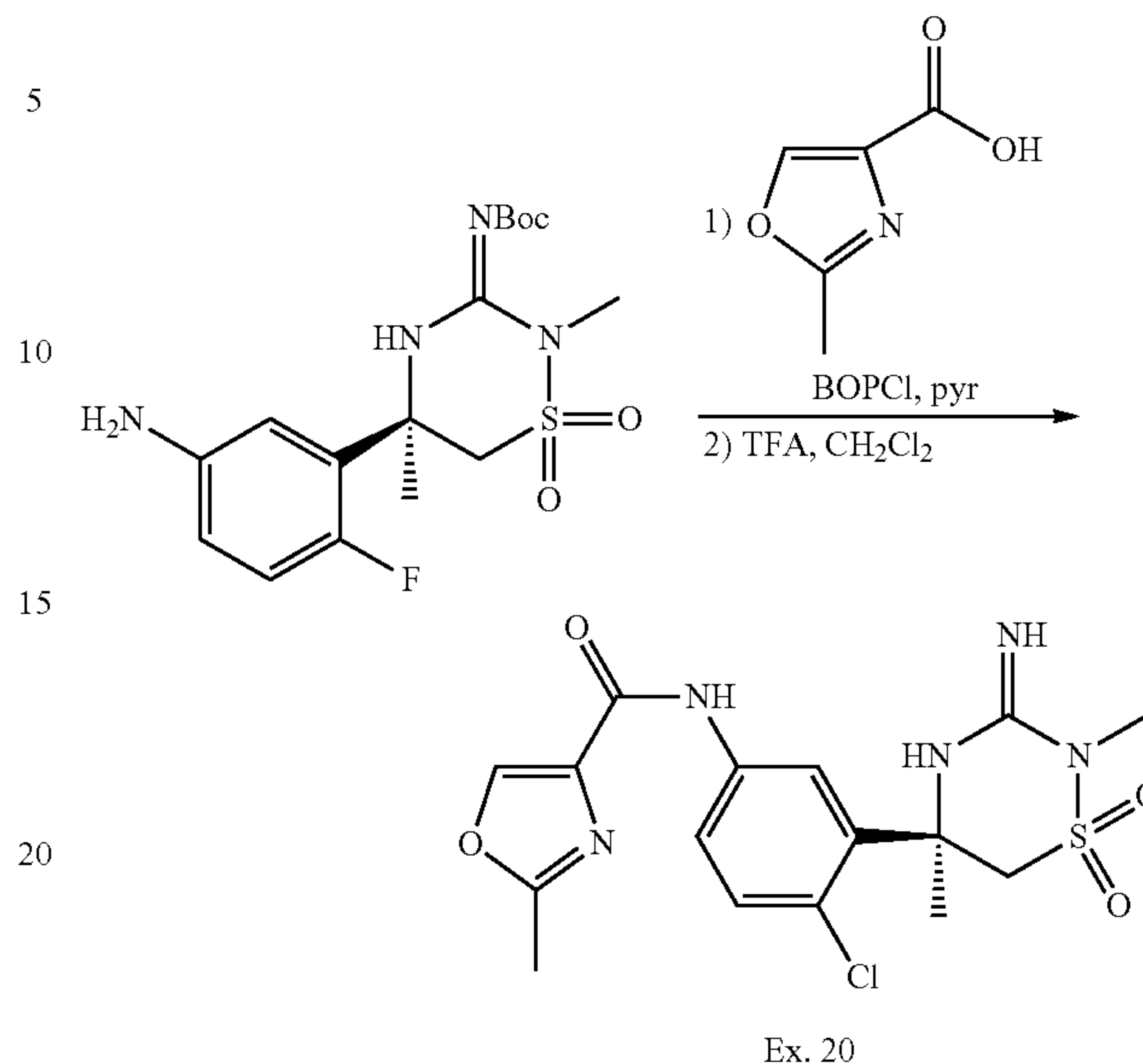
Scheme 11b:
