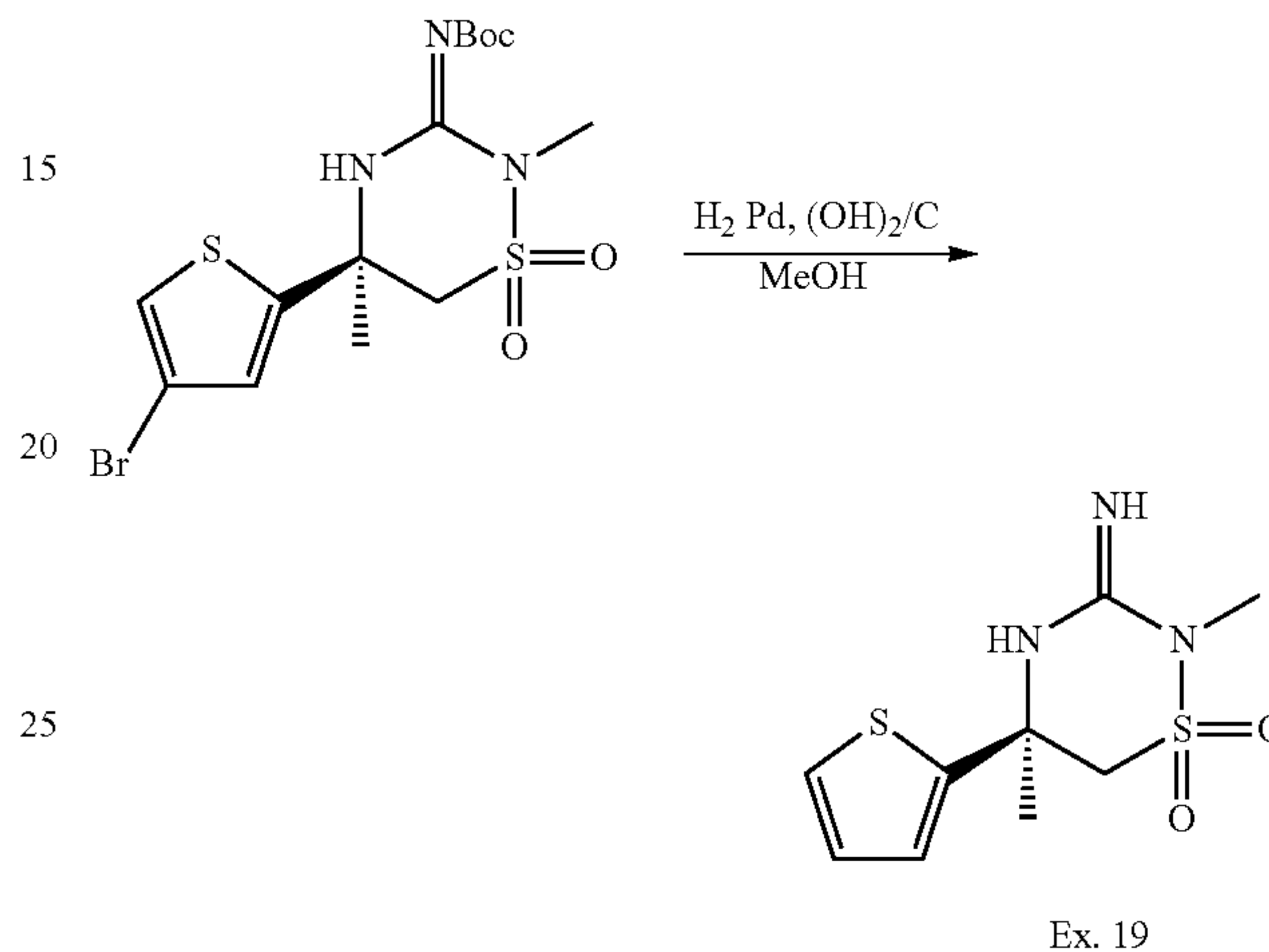
Scheme 9:
