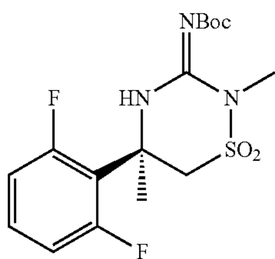
Scheme 7c:
