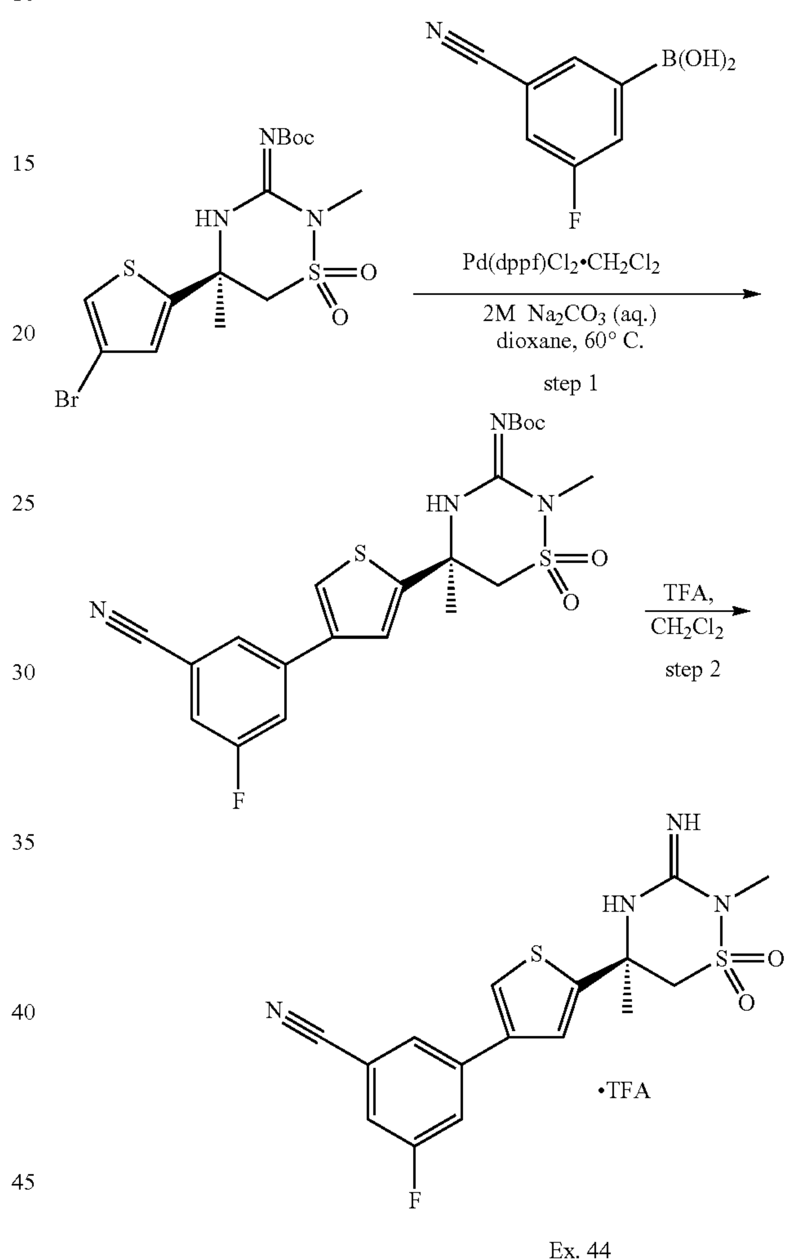
Scheme 15:
