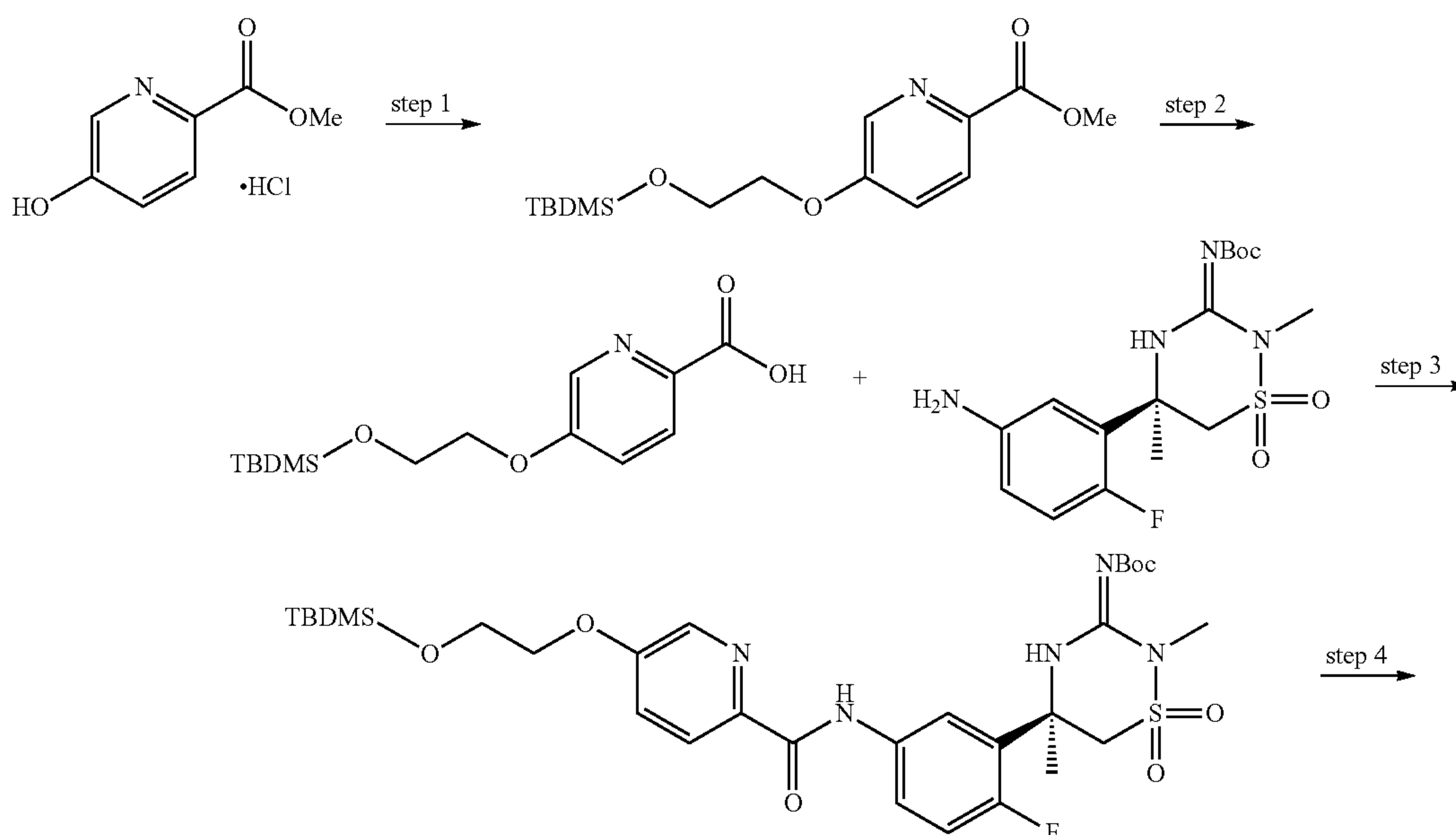
Scheme 24:
