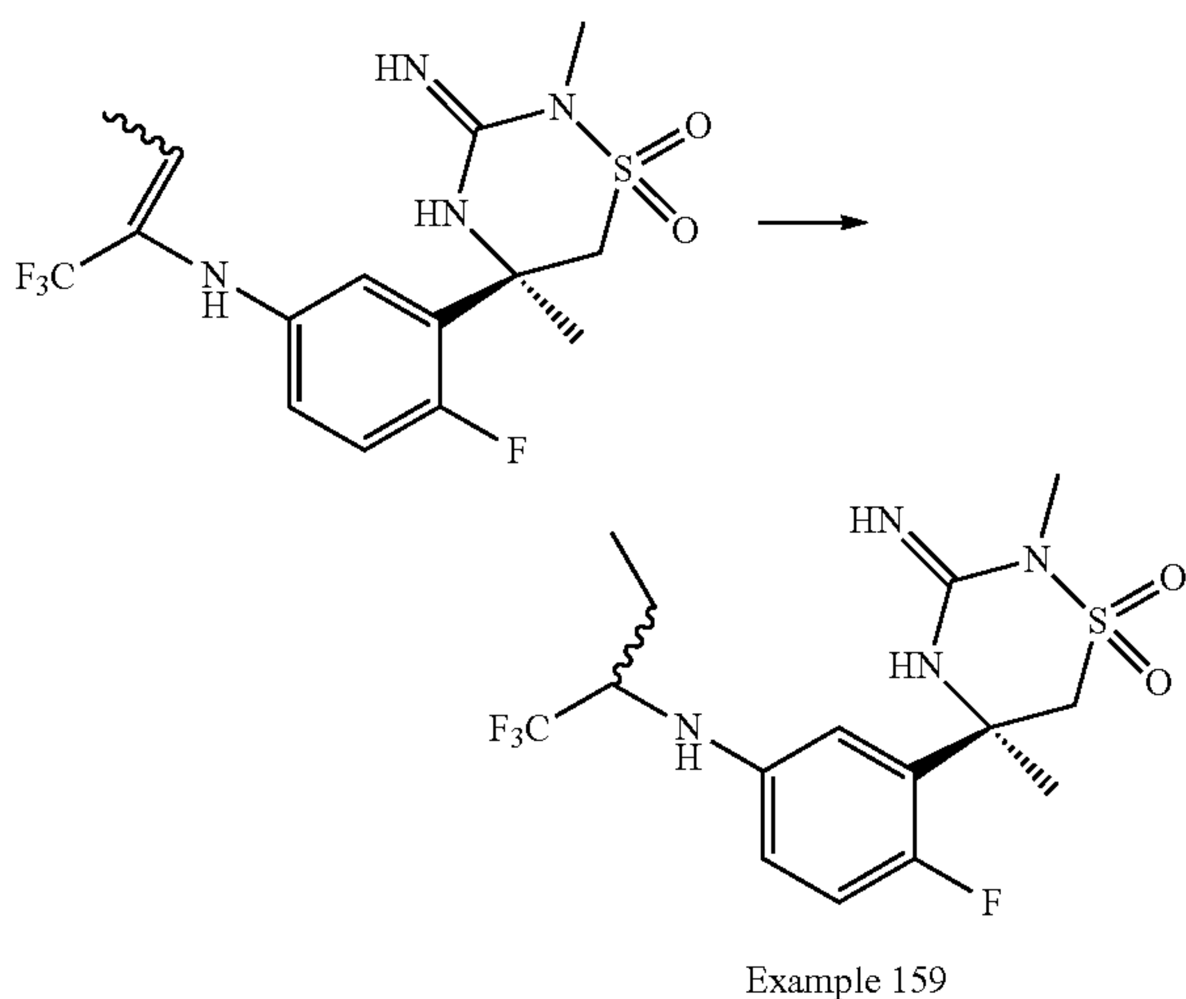
Scheme 38:
