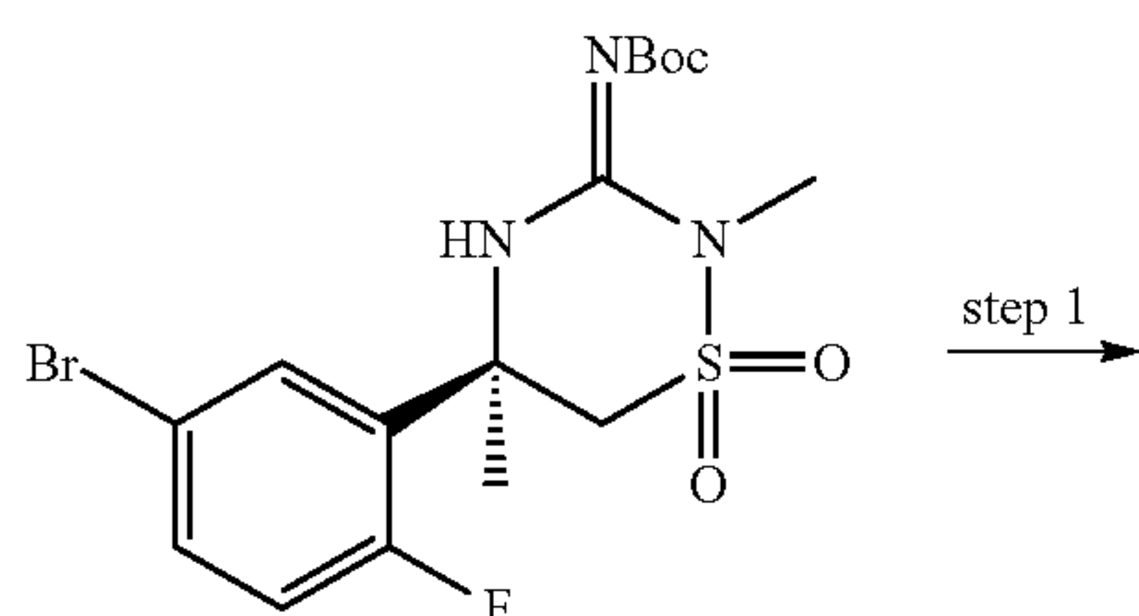
Scheme 30:
