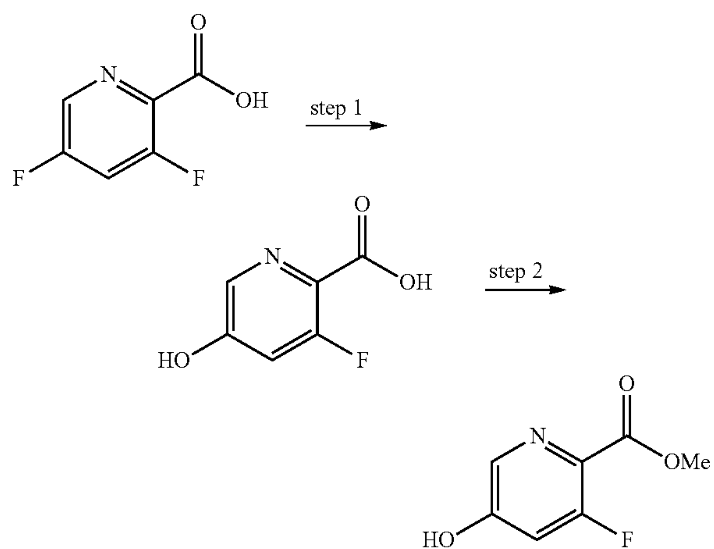
Scheme 11h:
