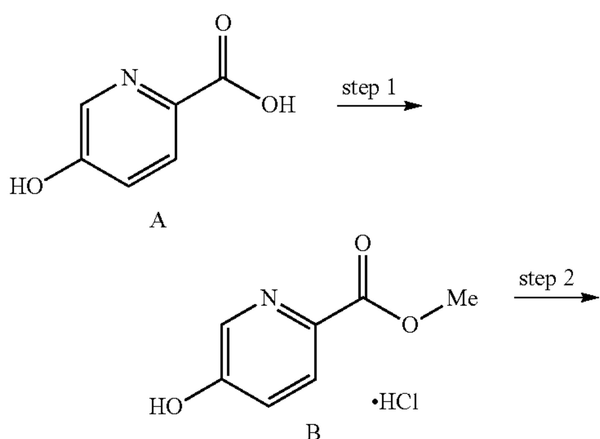
Scheme 11g:
