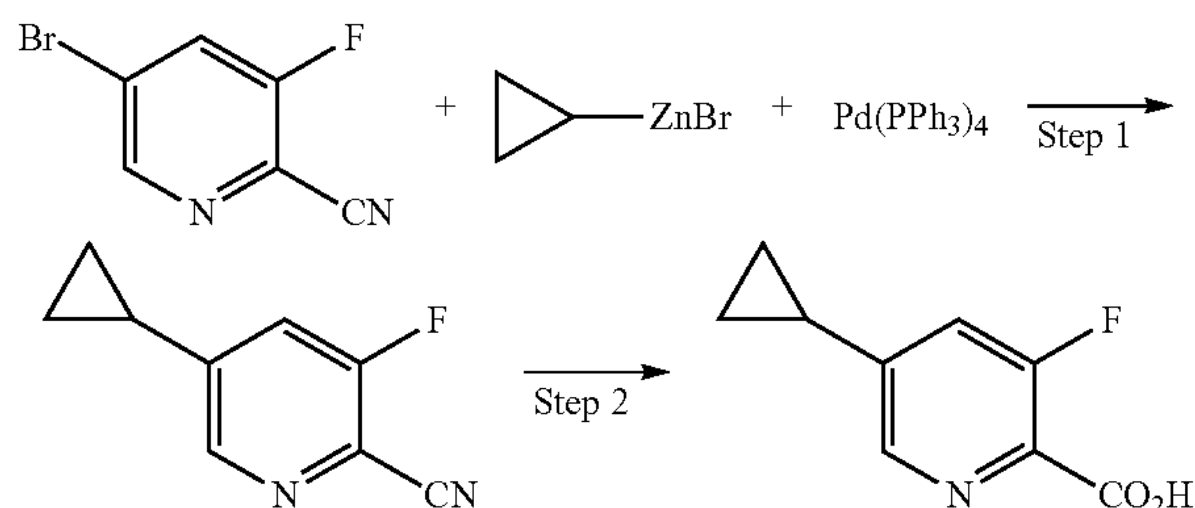
Scheme 11x:
