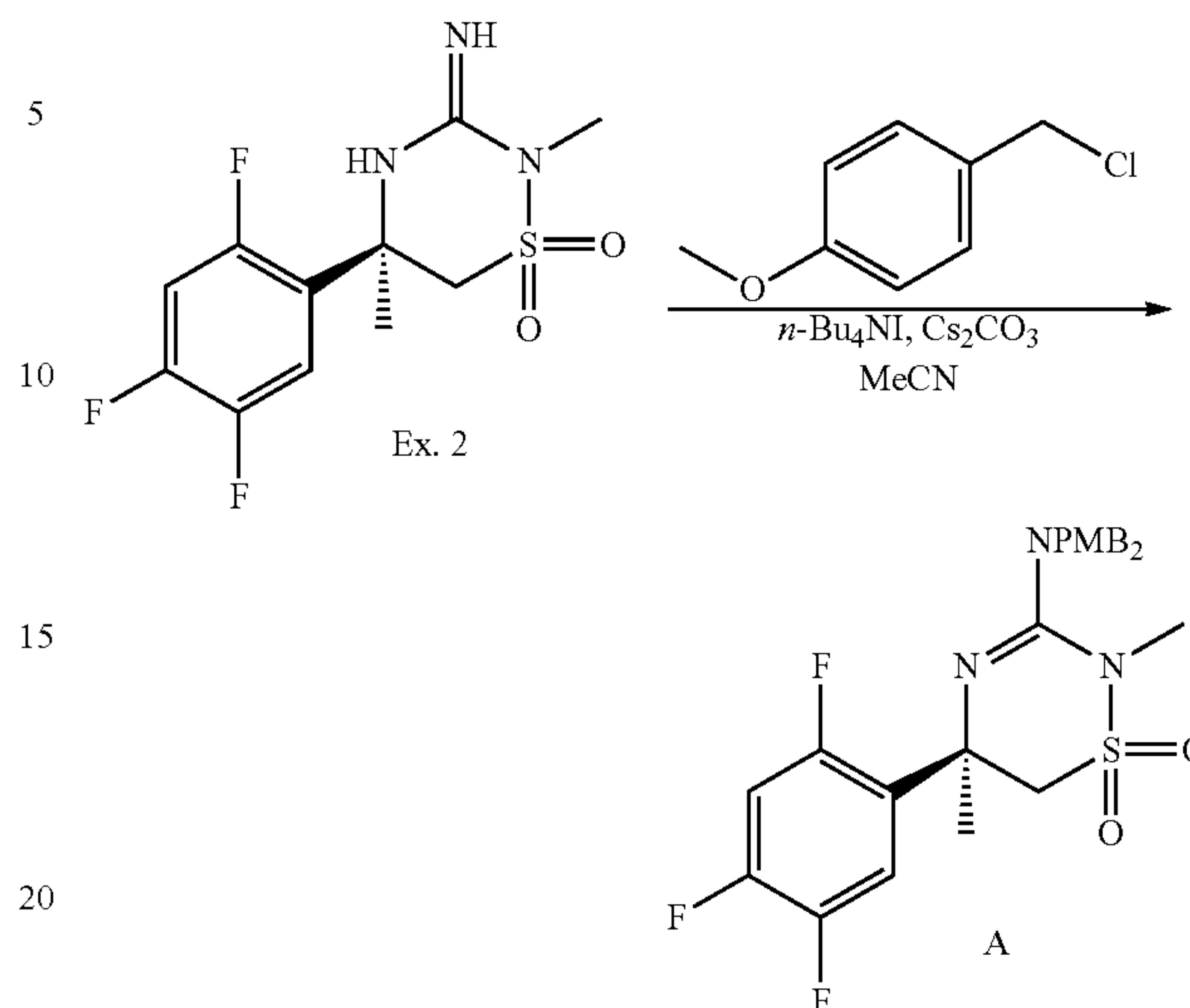
Scheme 4:
