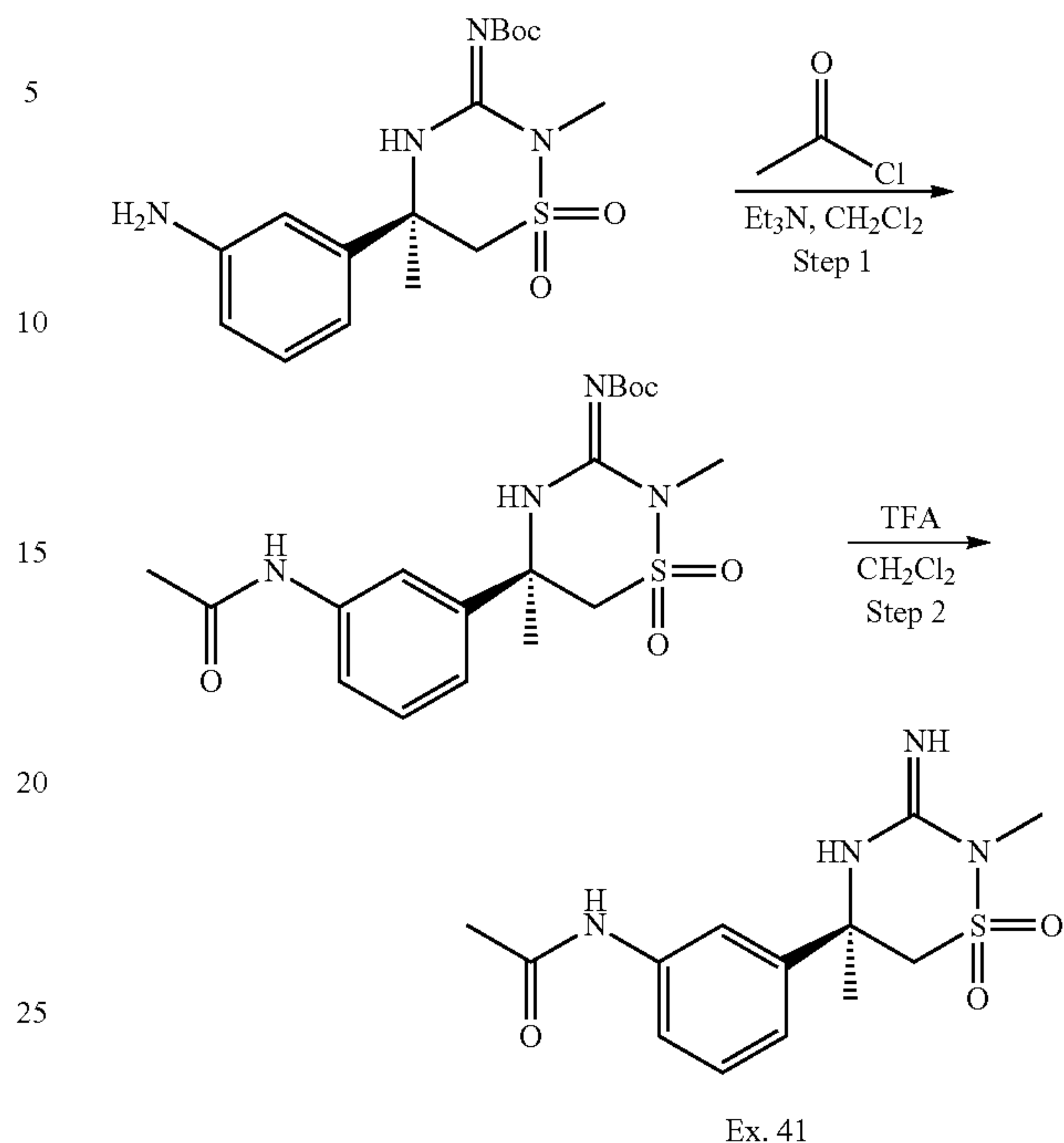
Scheme 12:
