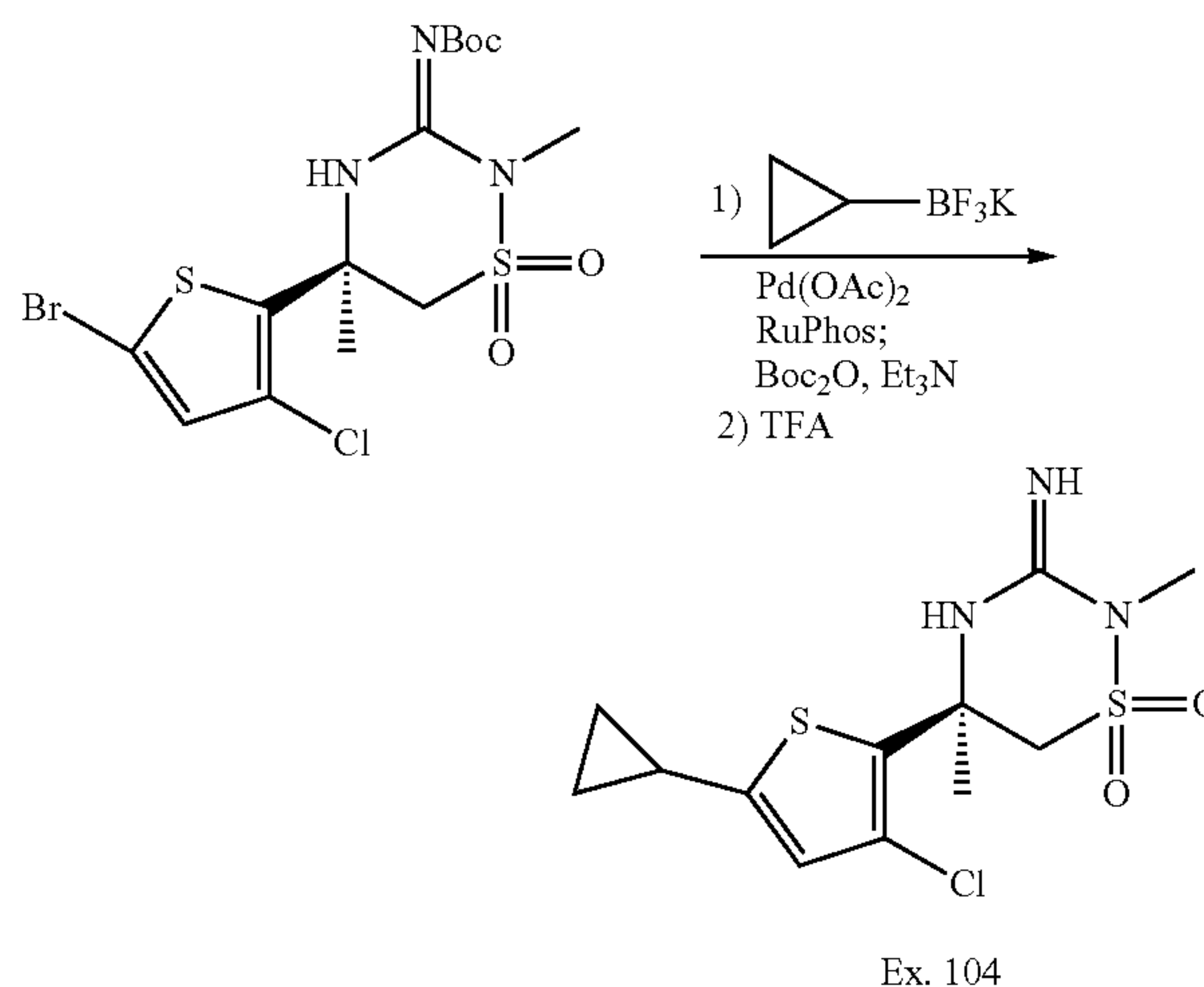
Scheme 19:
