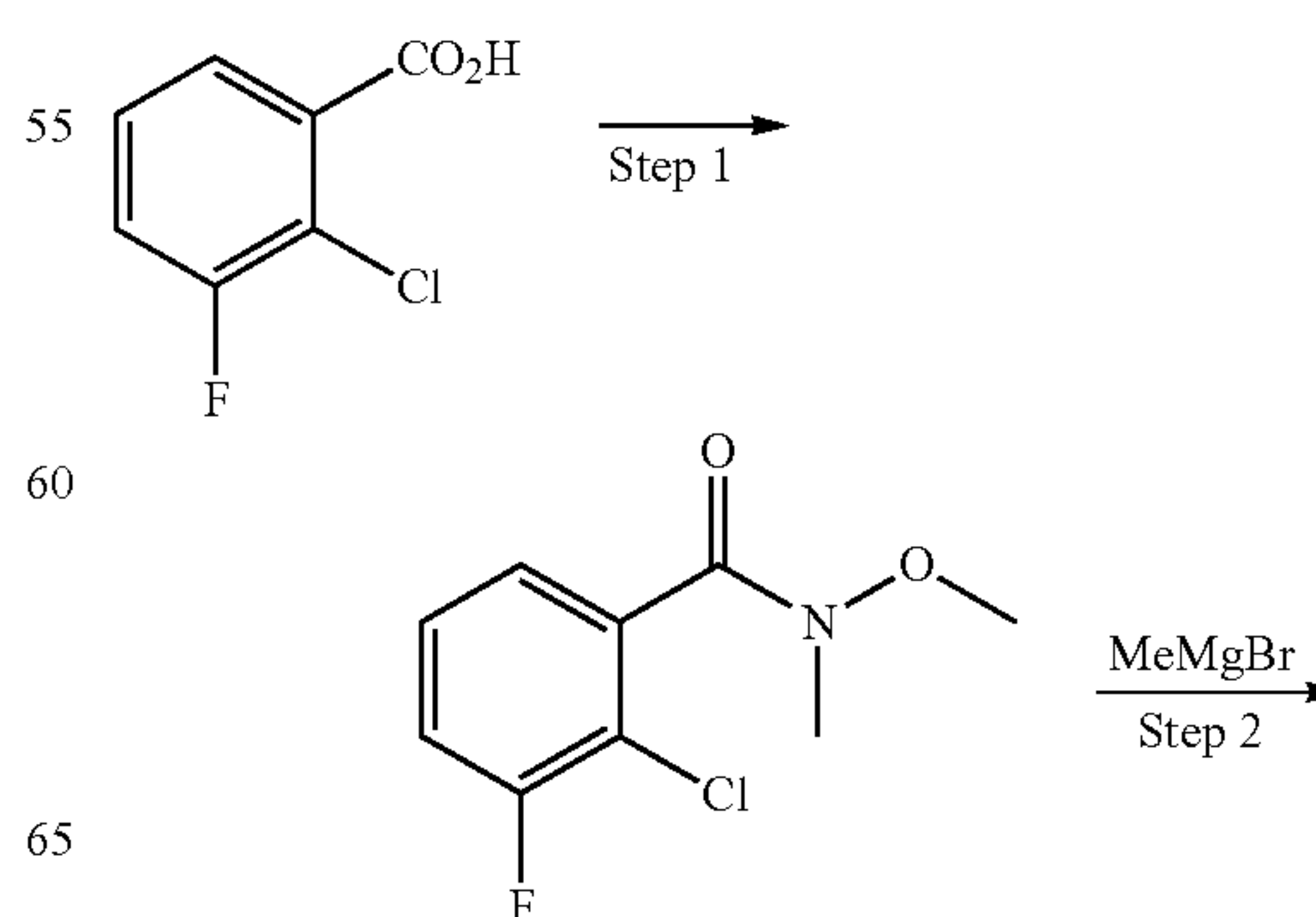
Scheme 2c:
