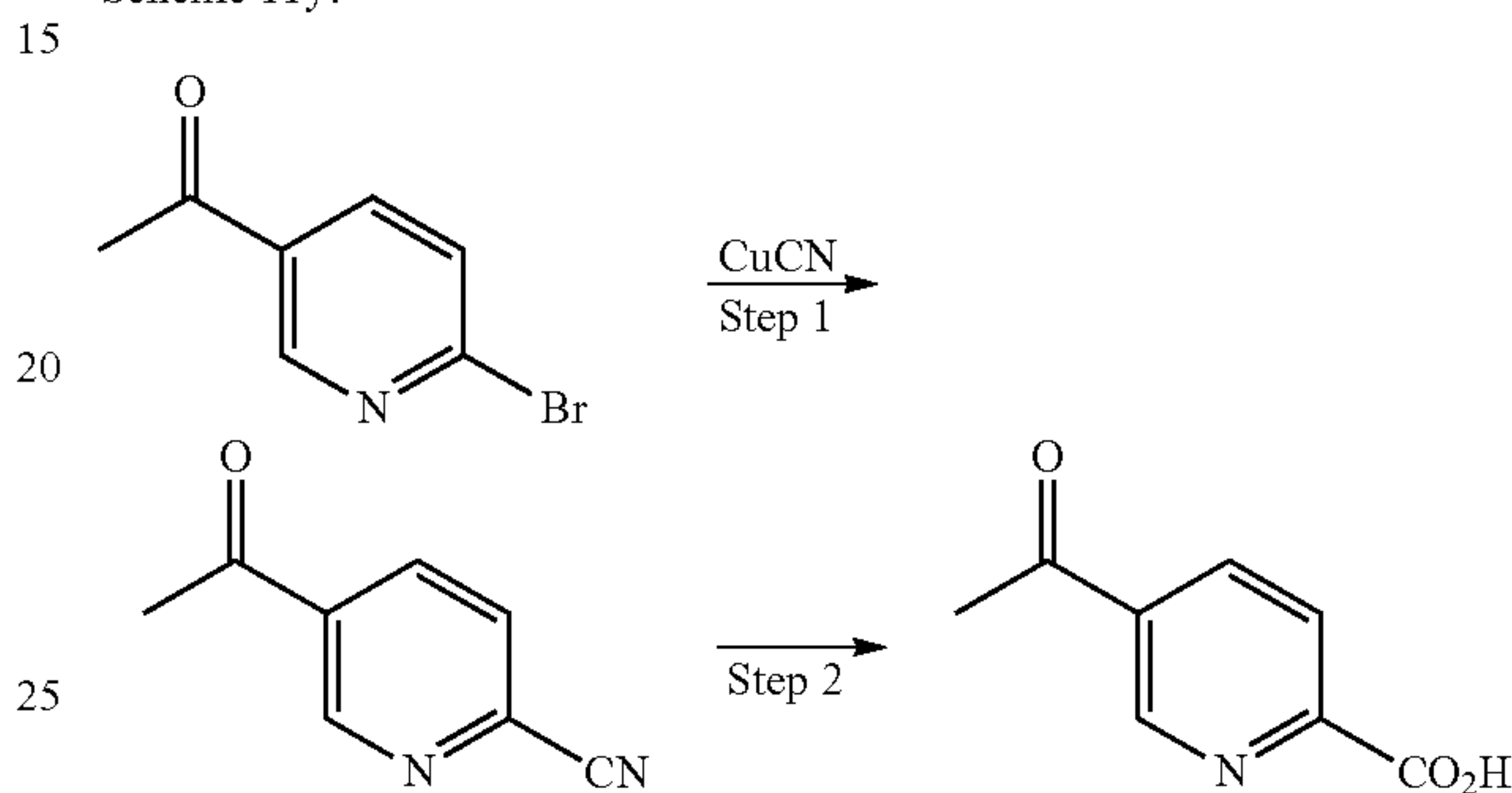
Scheme 11y:
