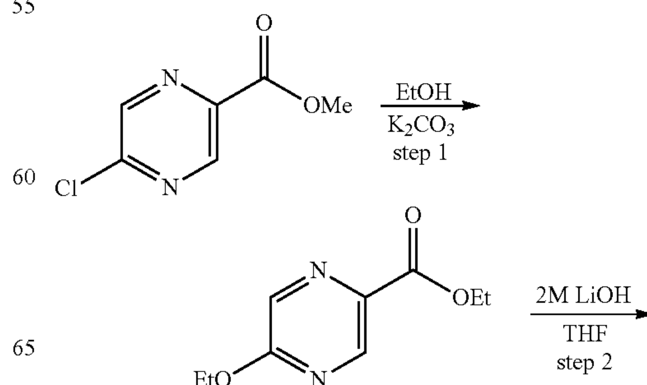
Scheme 11c:
