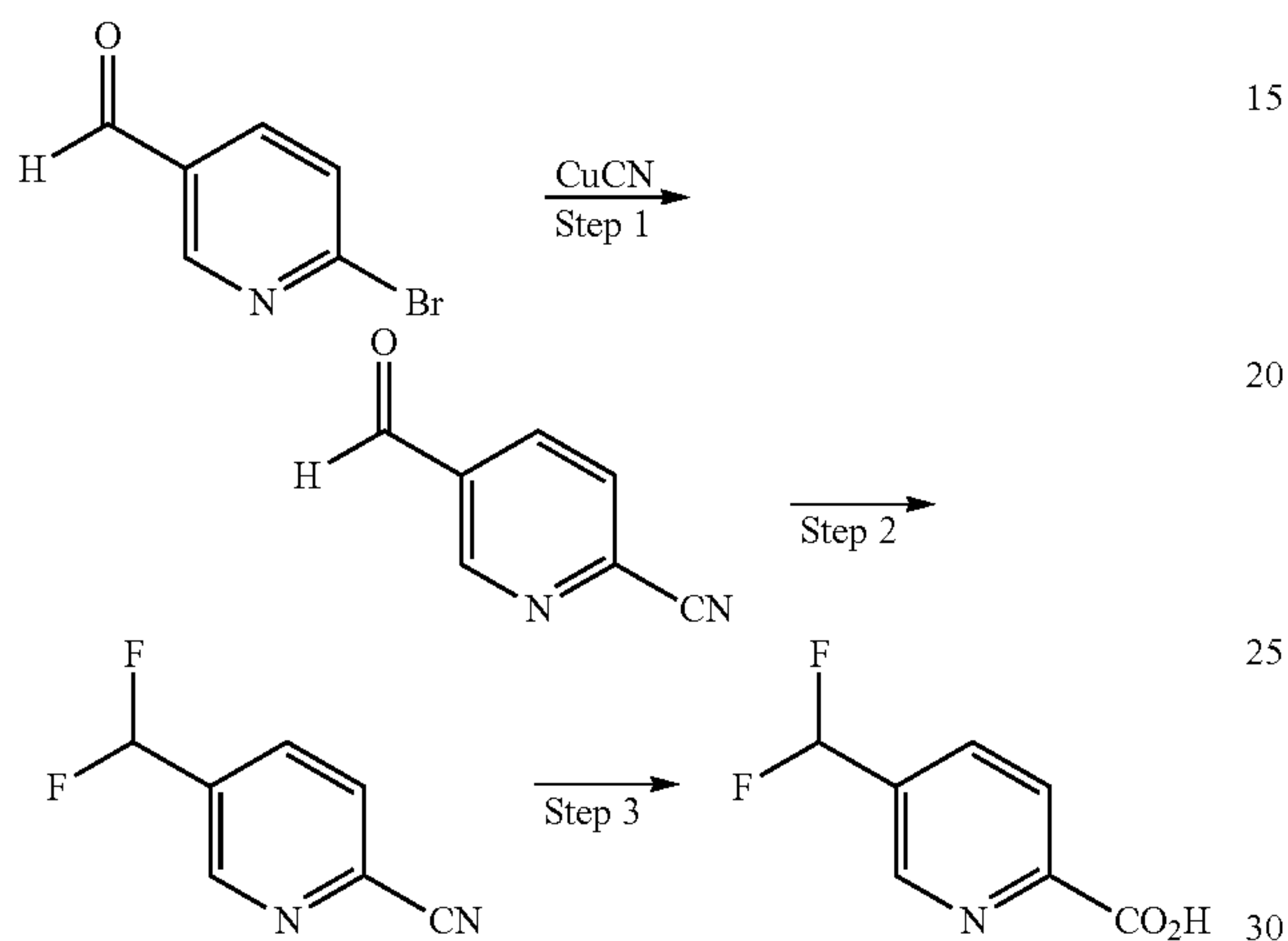
Scheme 11aa:
