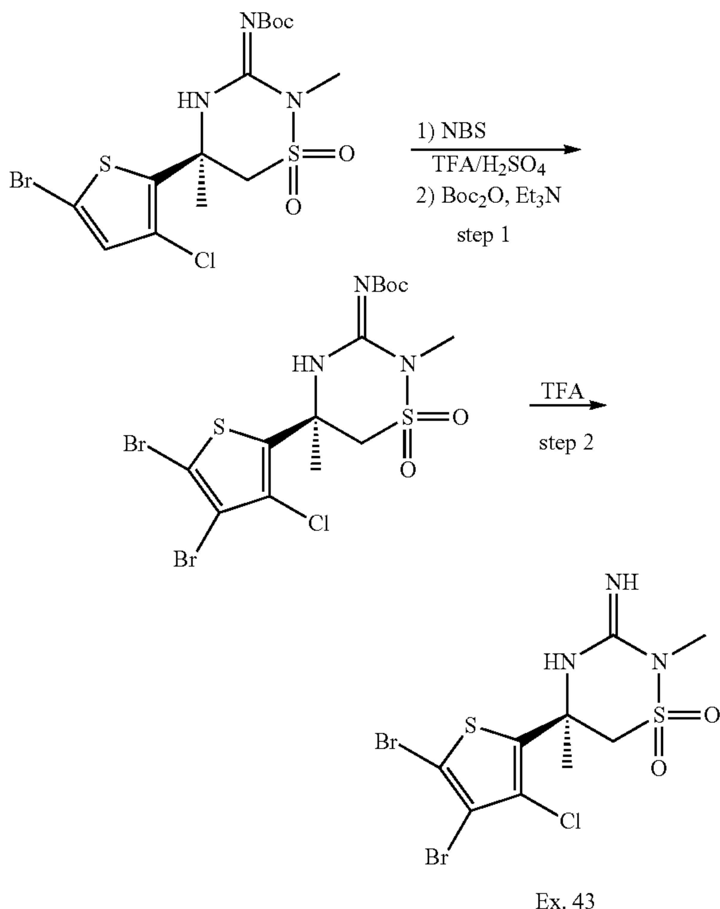
Scheme 14:
