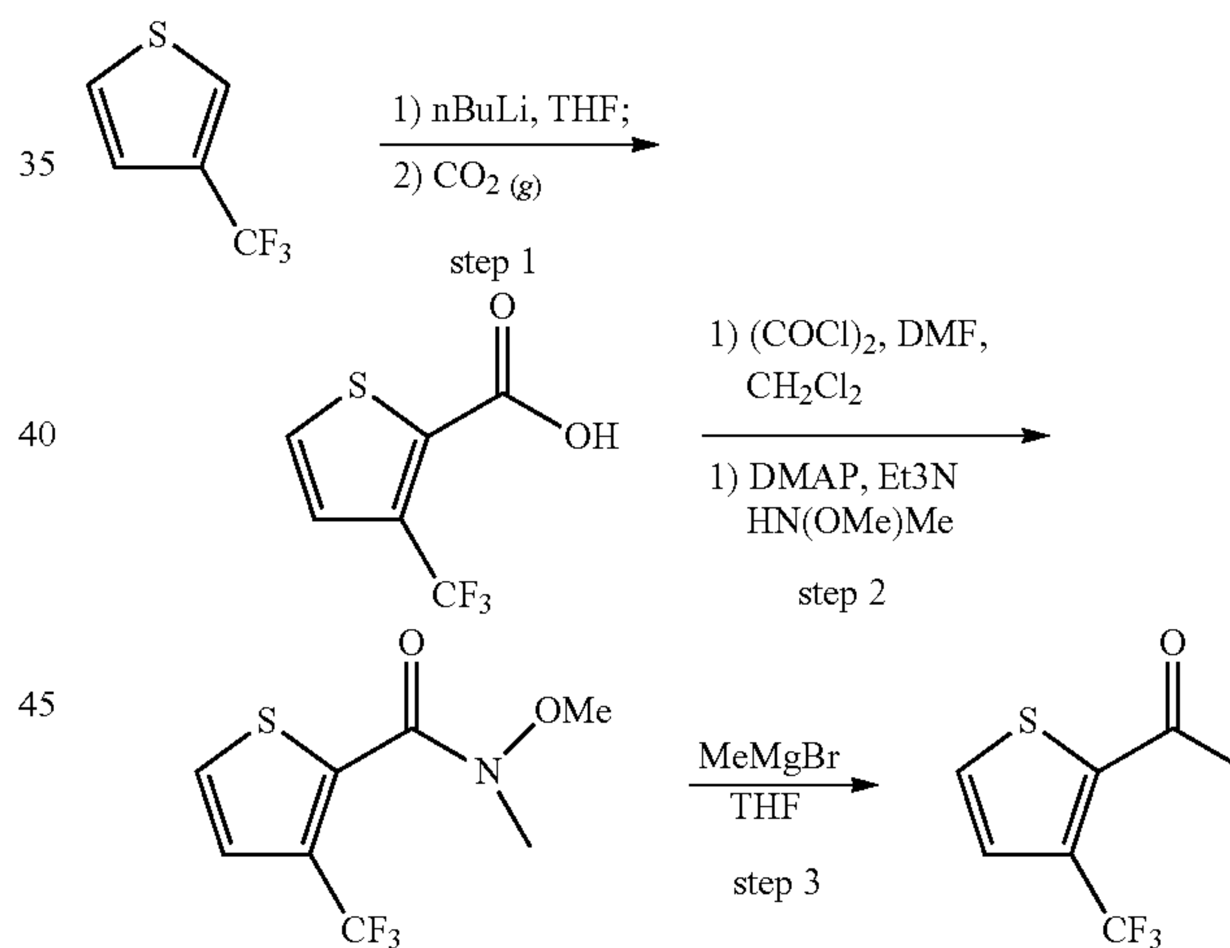
Scheme 2:
