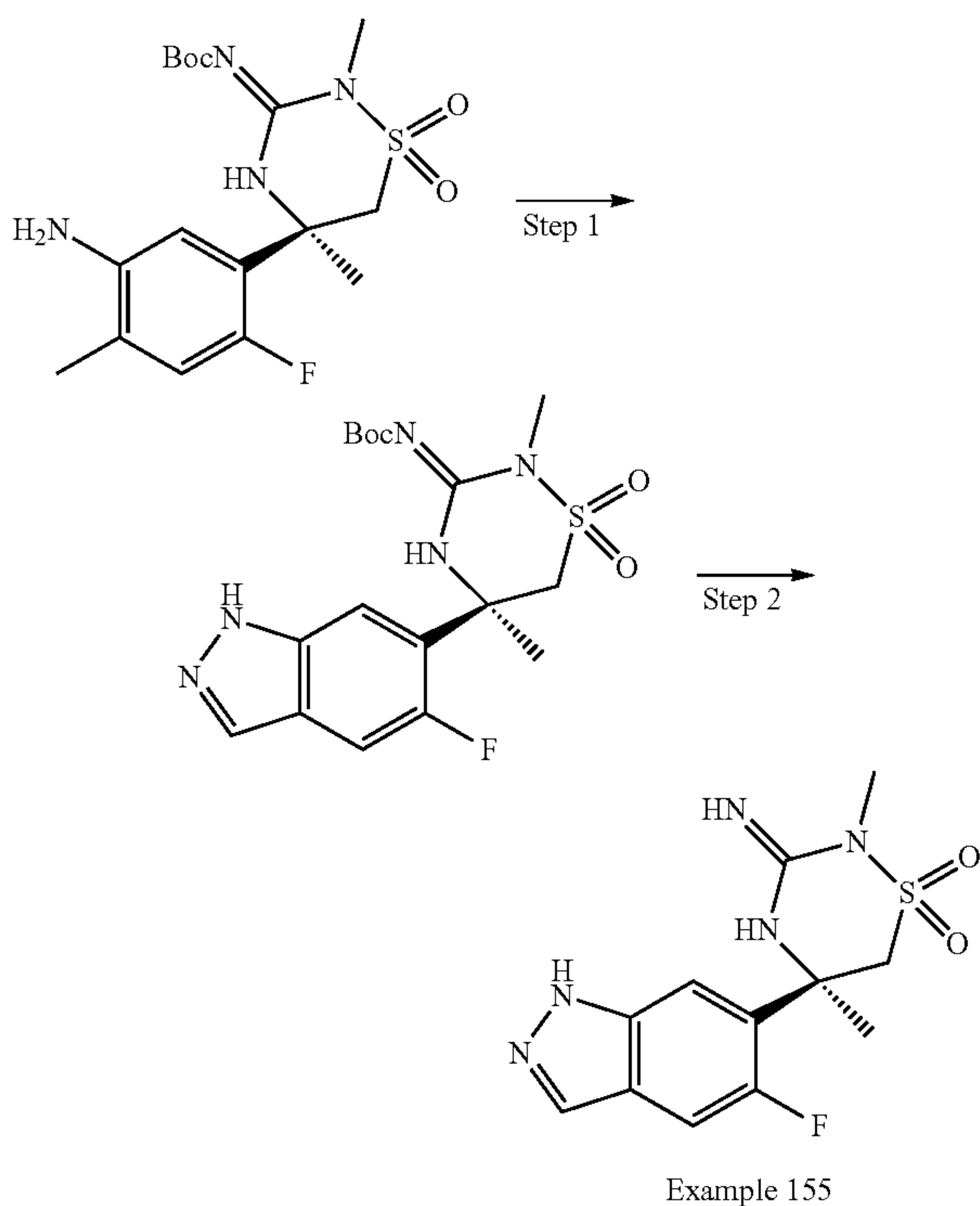
Scheme 36:
