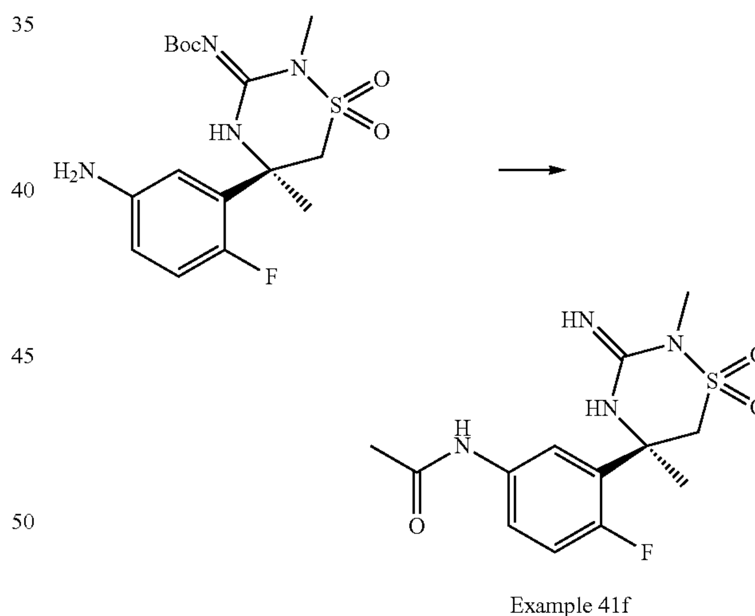
Scheme 12d:
