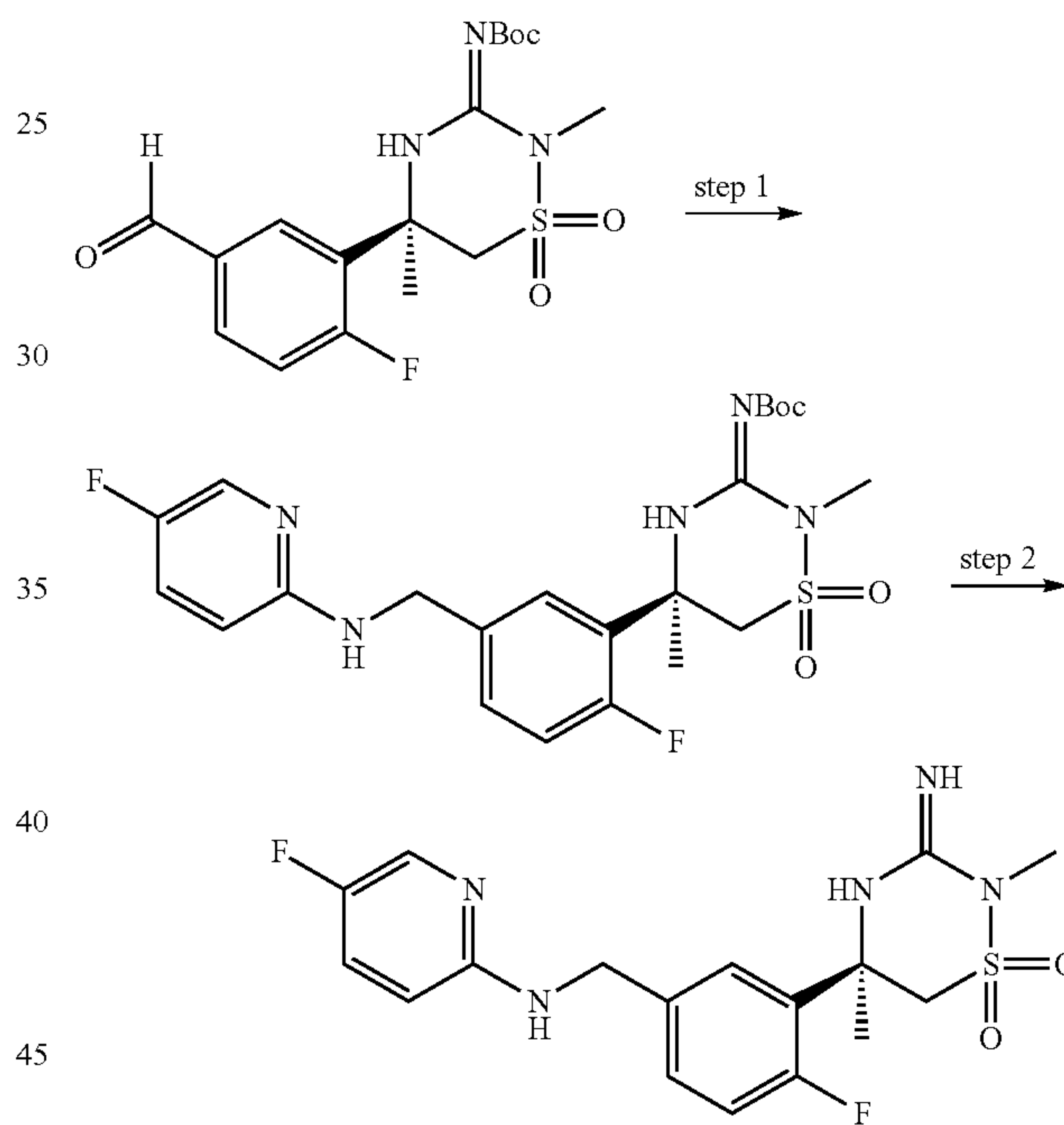
Scheme 28
