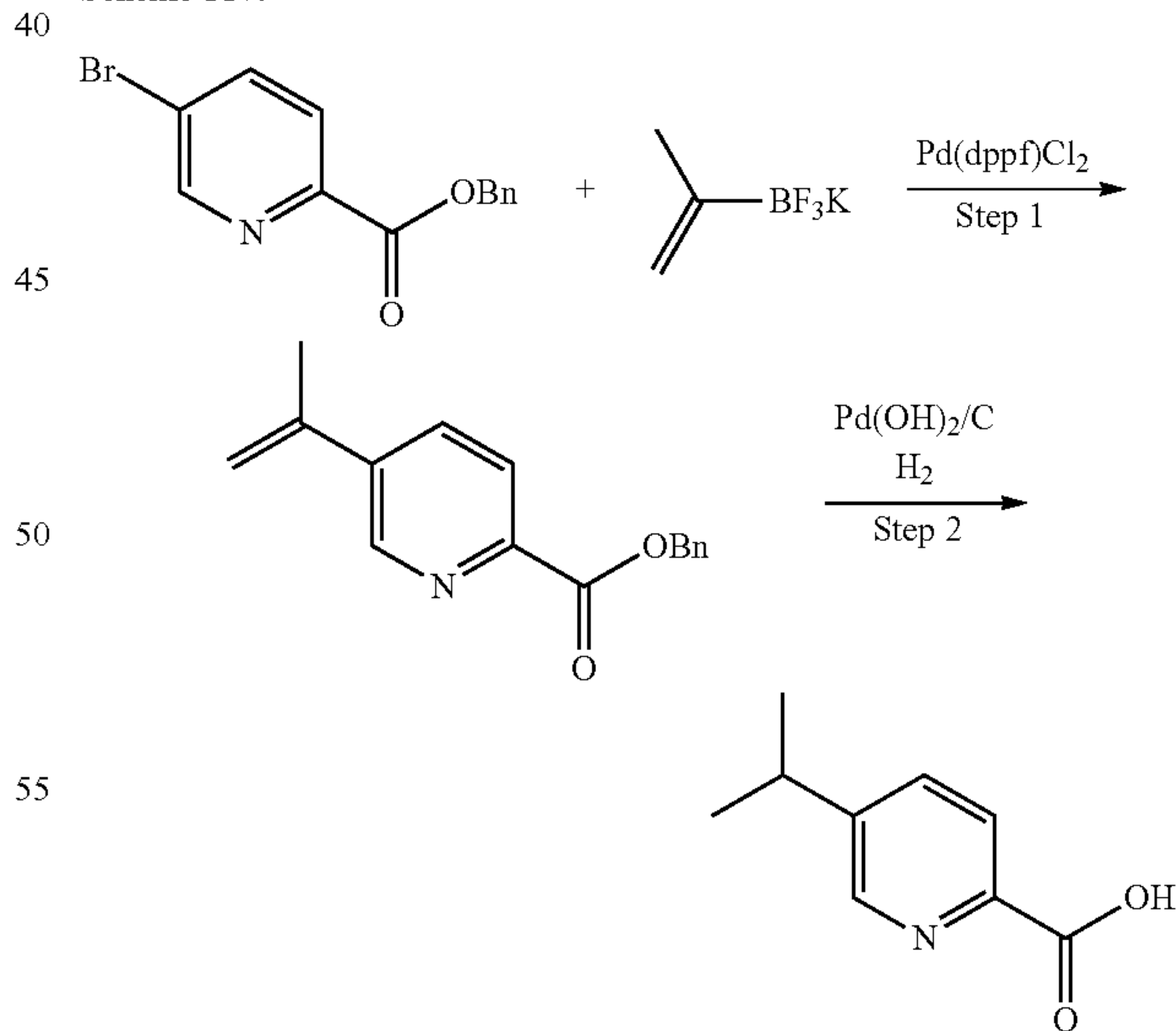
Scheme 11v:
