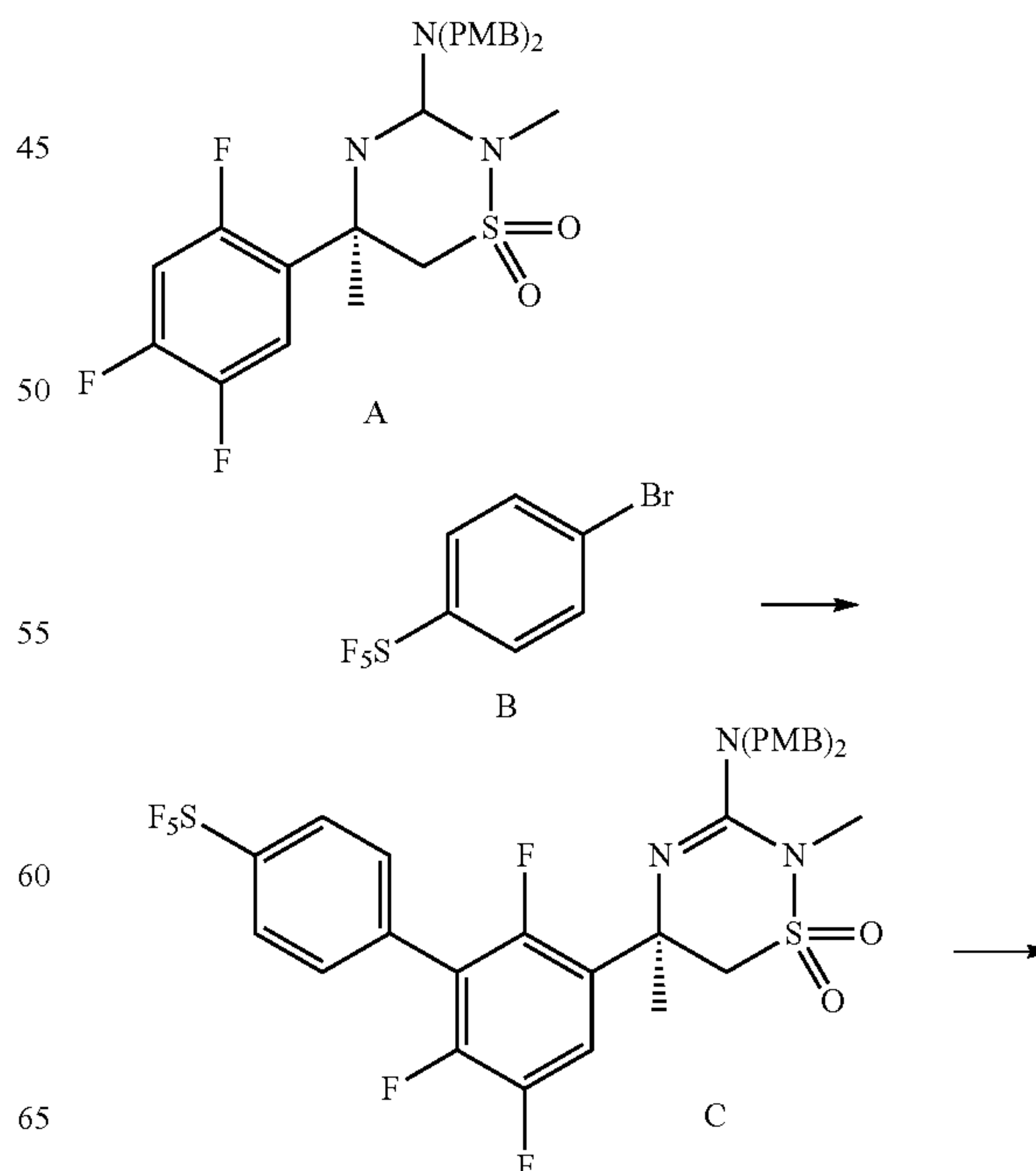
Scheme 5:
