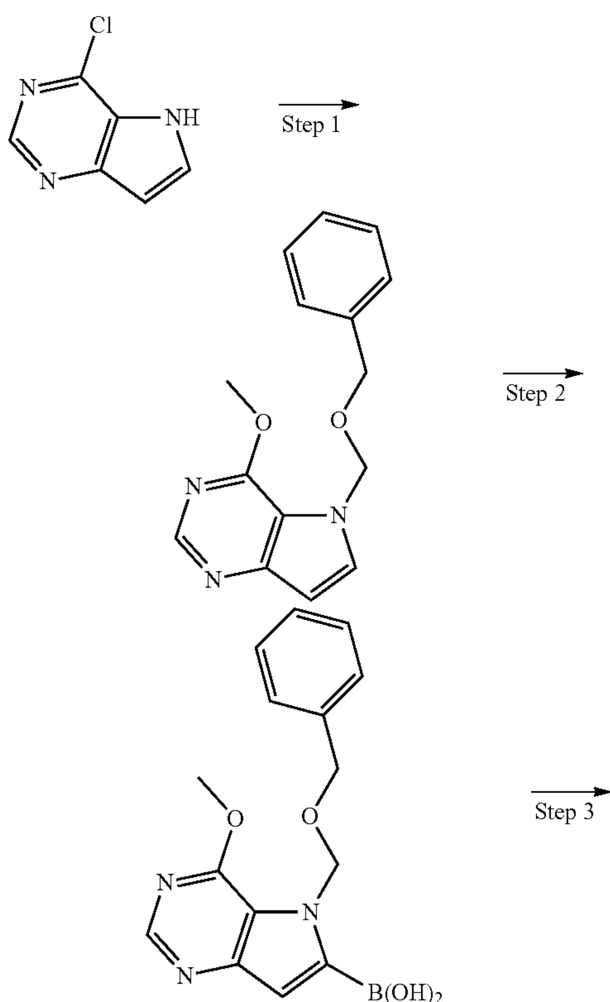
Scheme 52:
