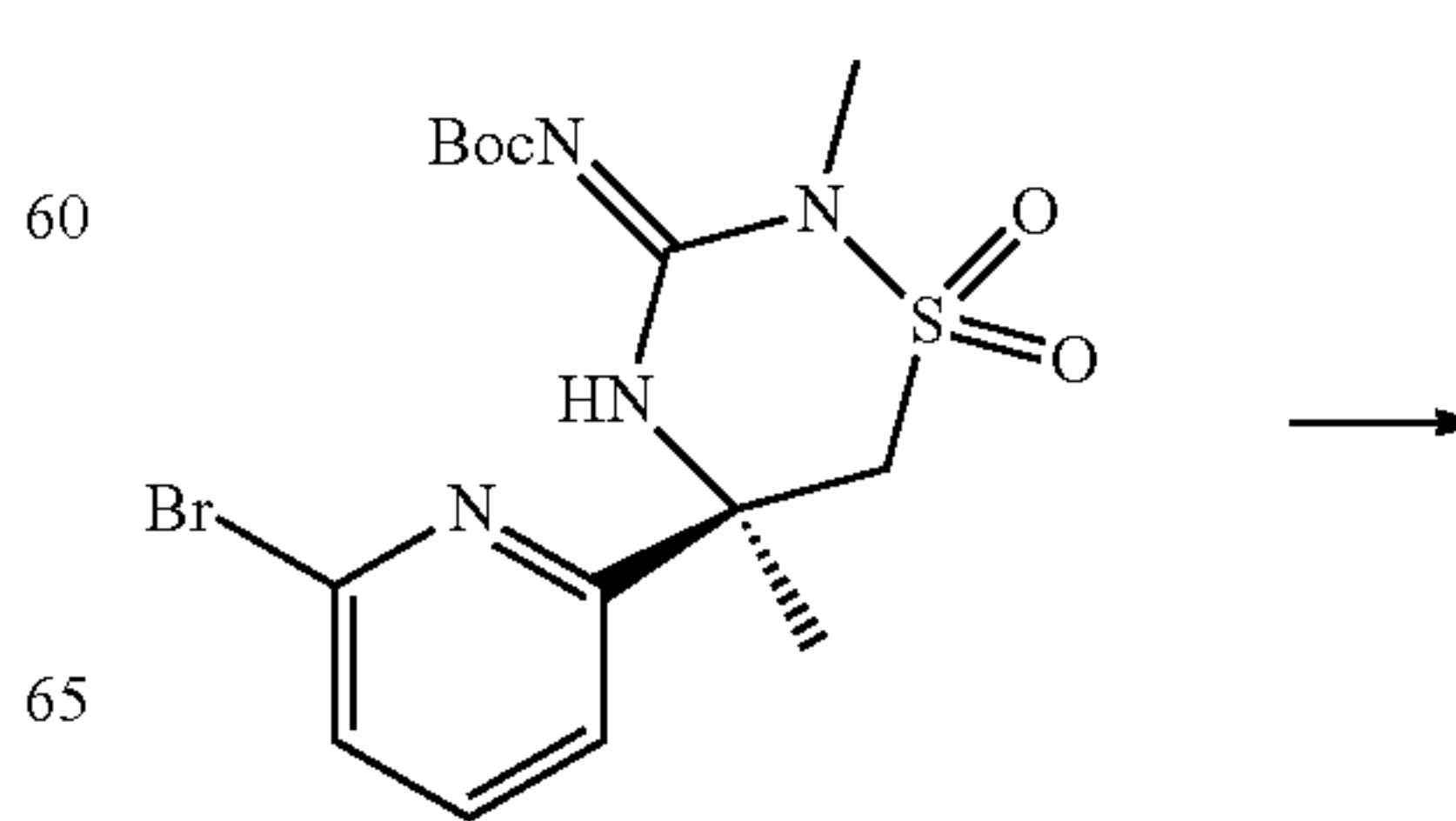
Scheme 40:
