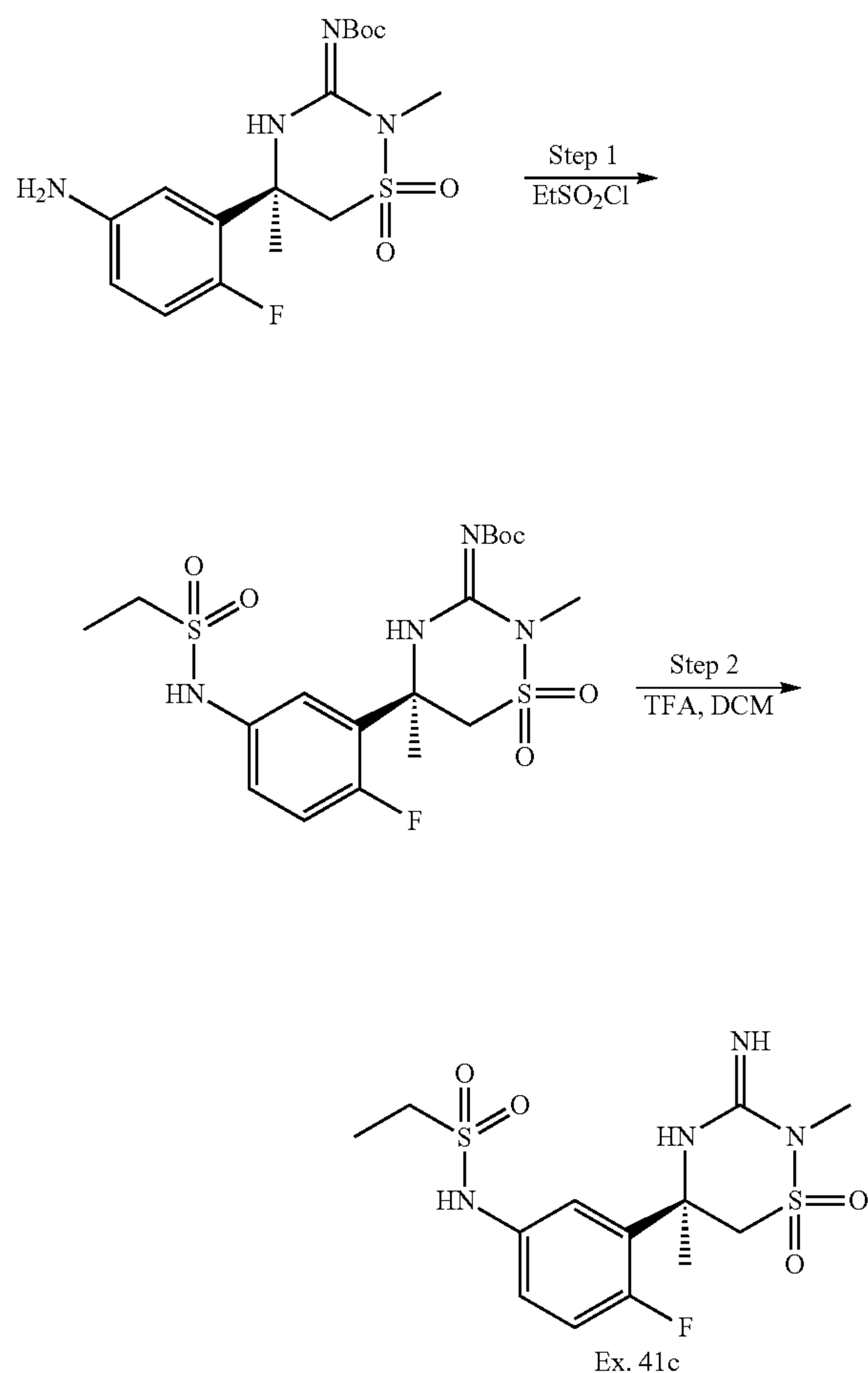
Scheme 12c:
