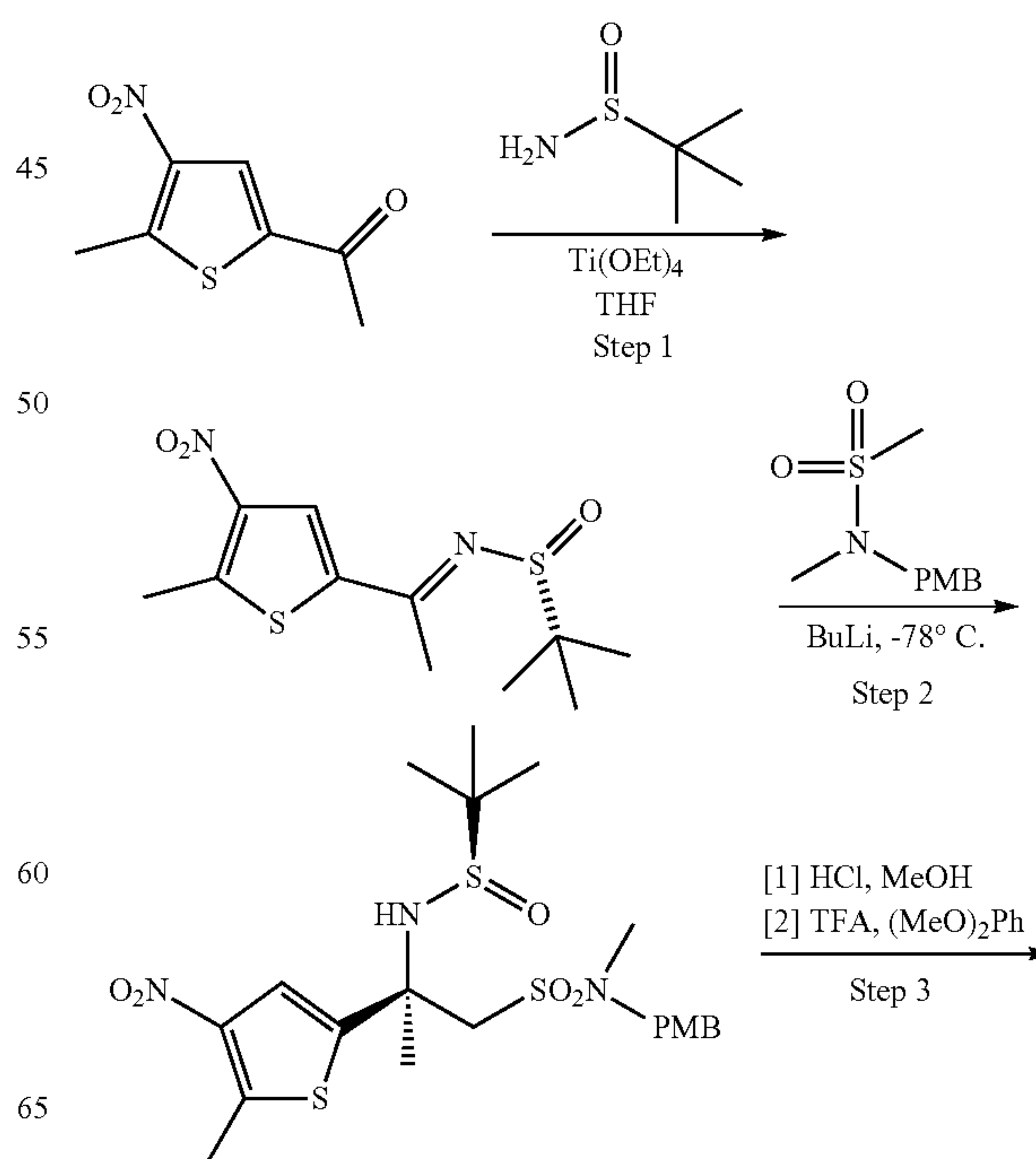
Scheme 44:
