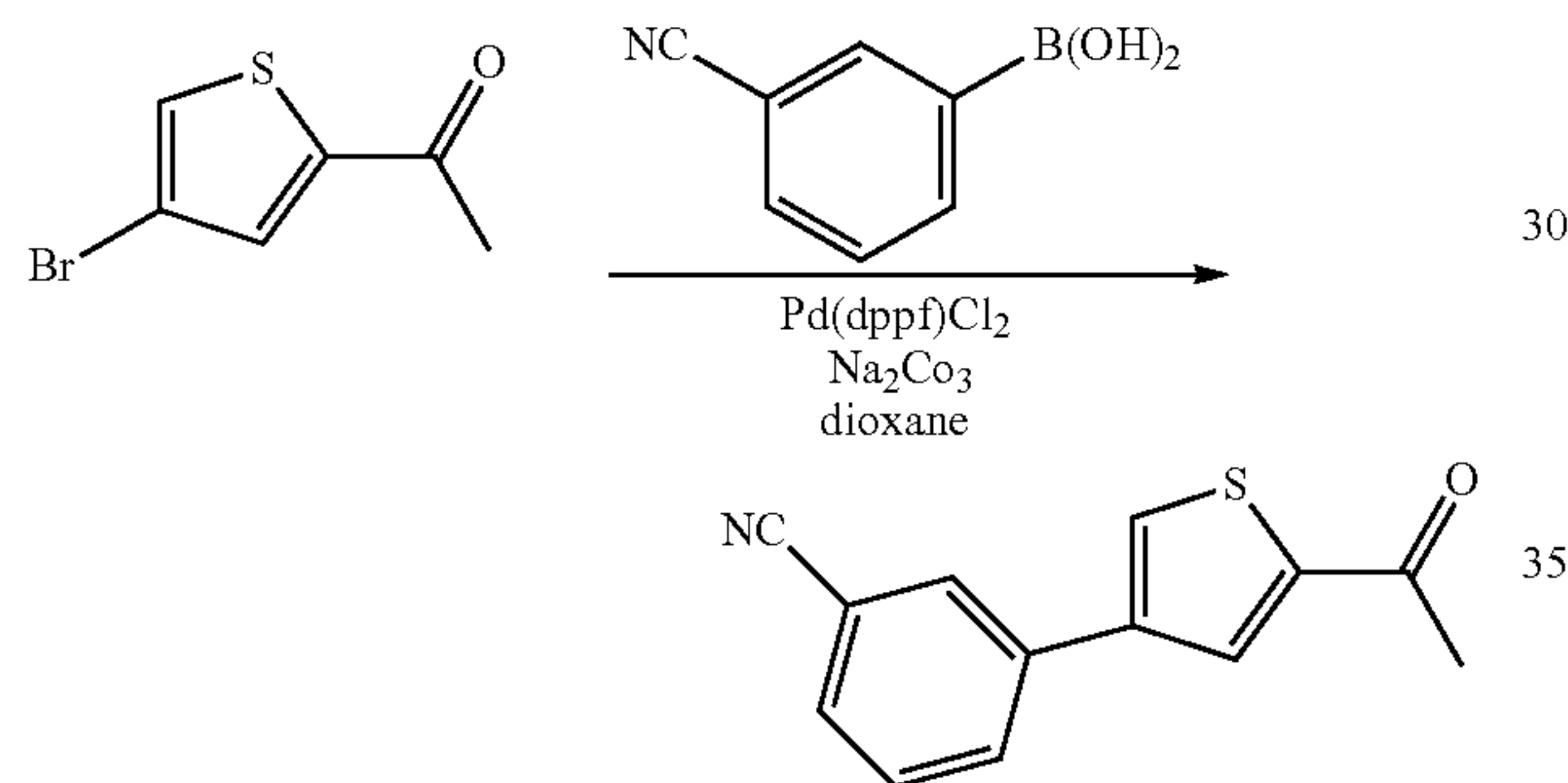
Scheme 20:
