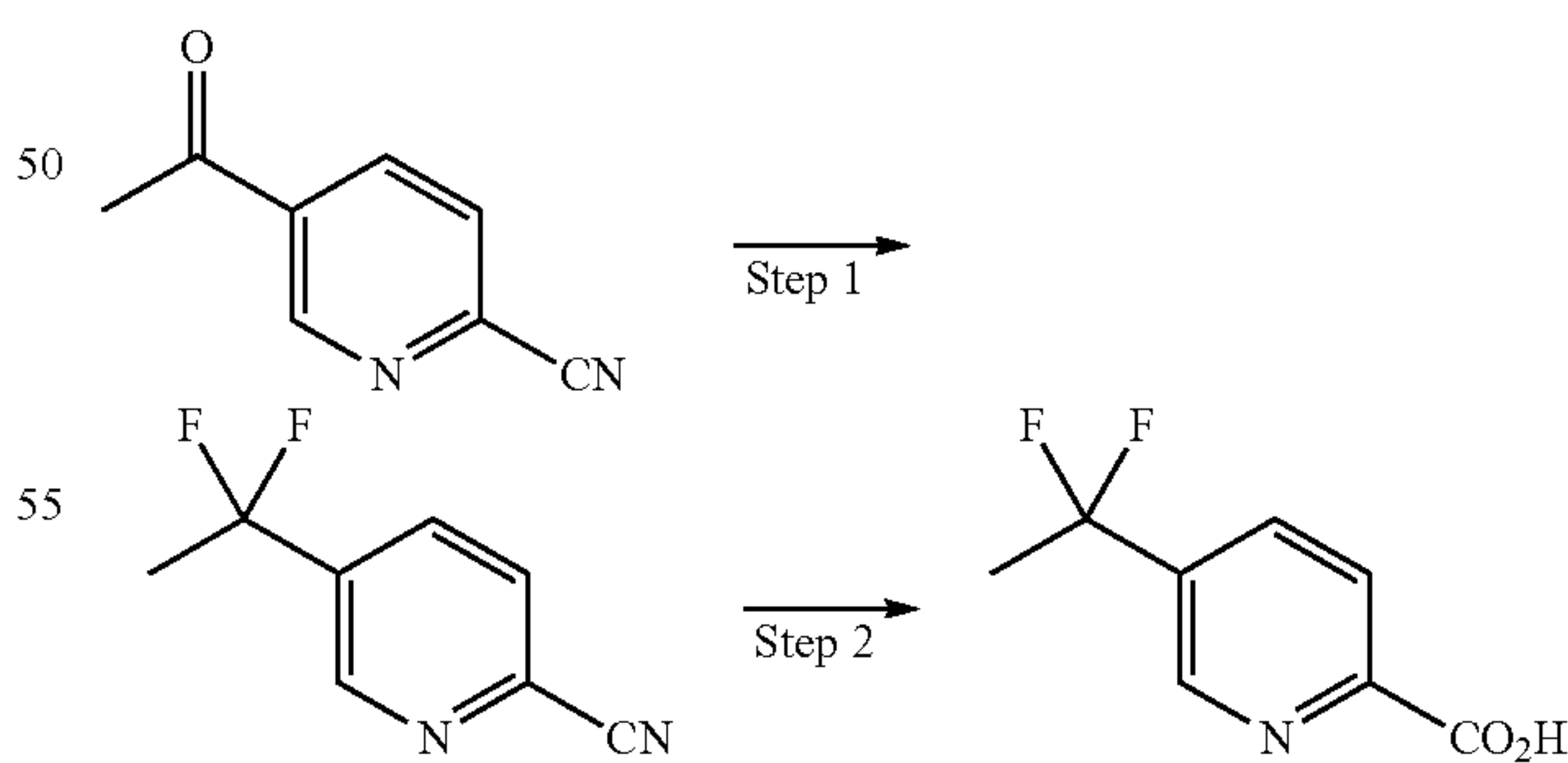
Scheme 11z:
