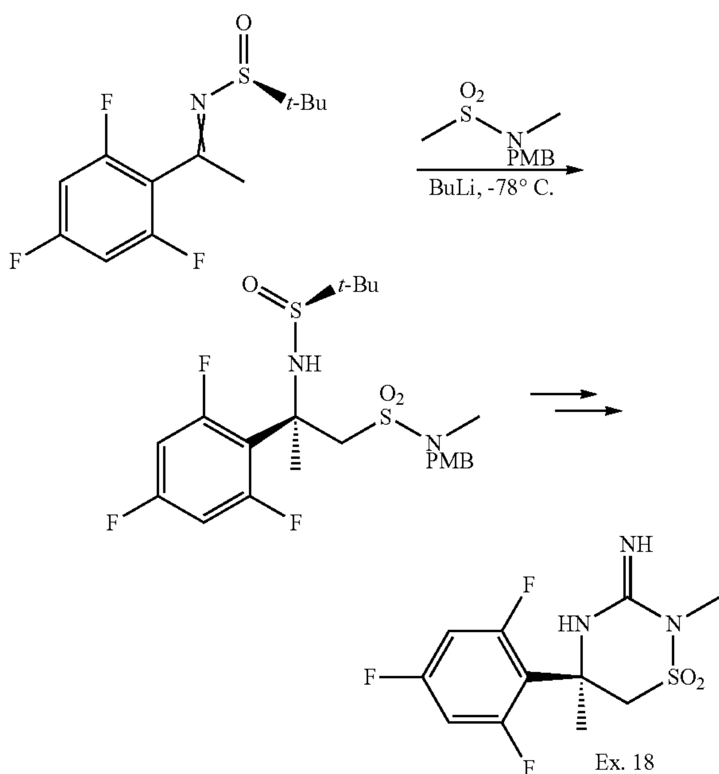
Scheme 8:
