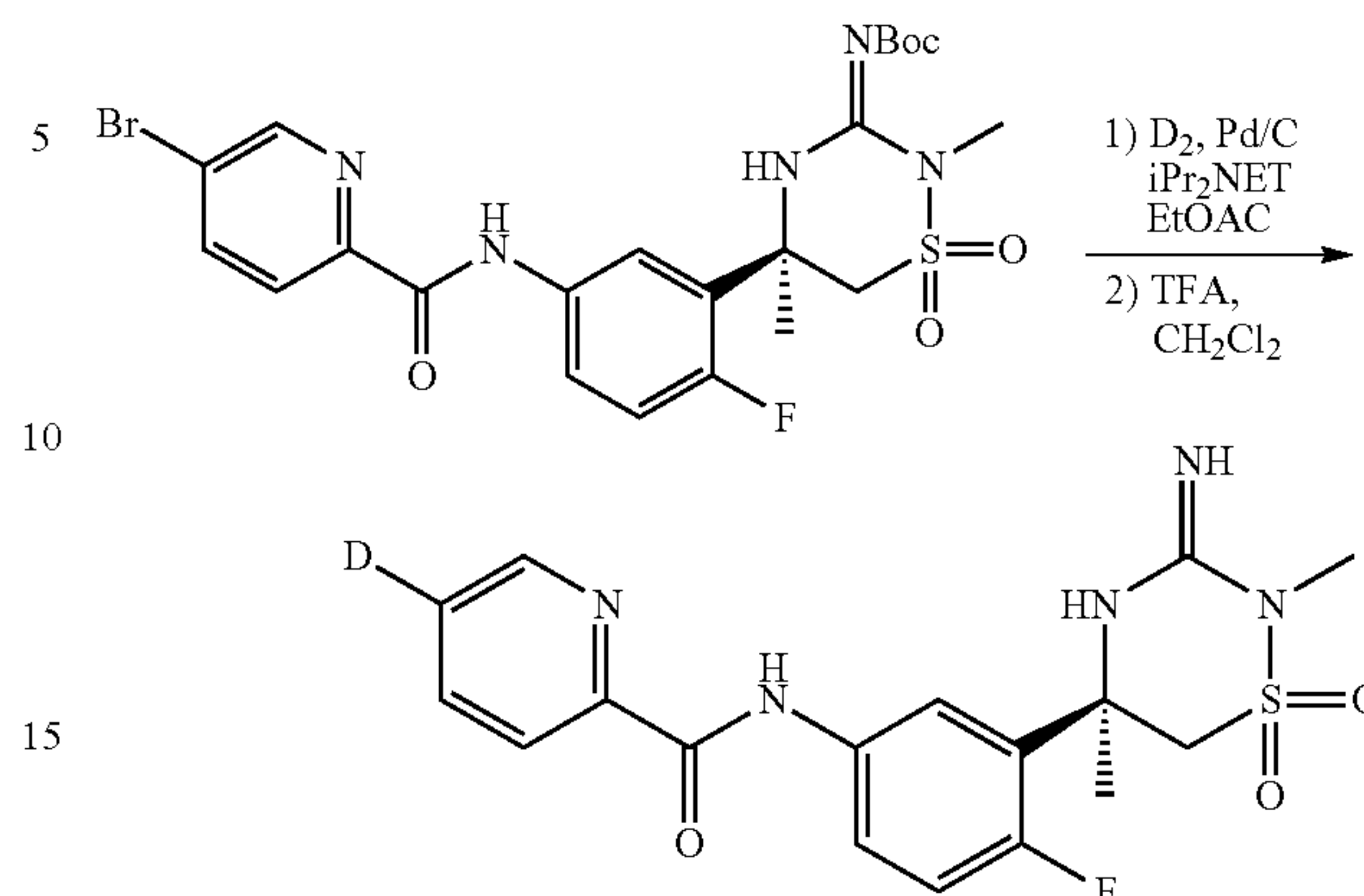
Scheme 23:
