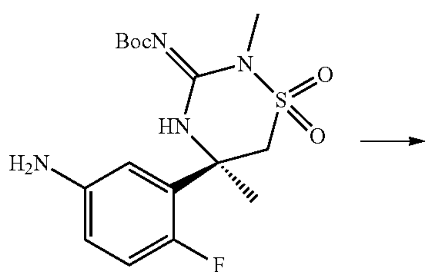
Scheme 39:
