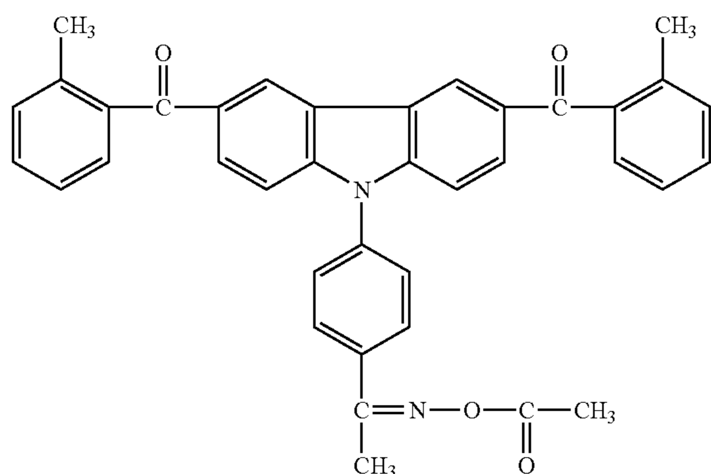
6.a 1-(4-Carbazol-9-yl-phenyl)-ethanone
