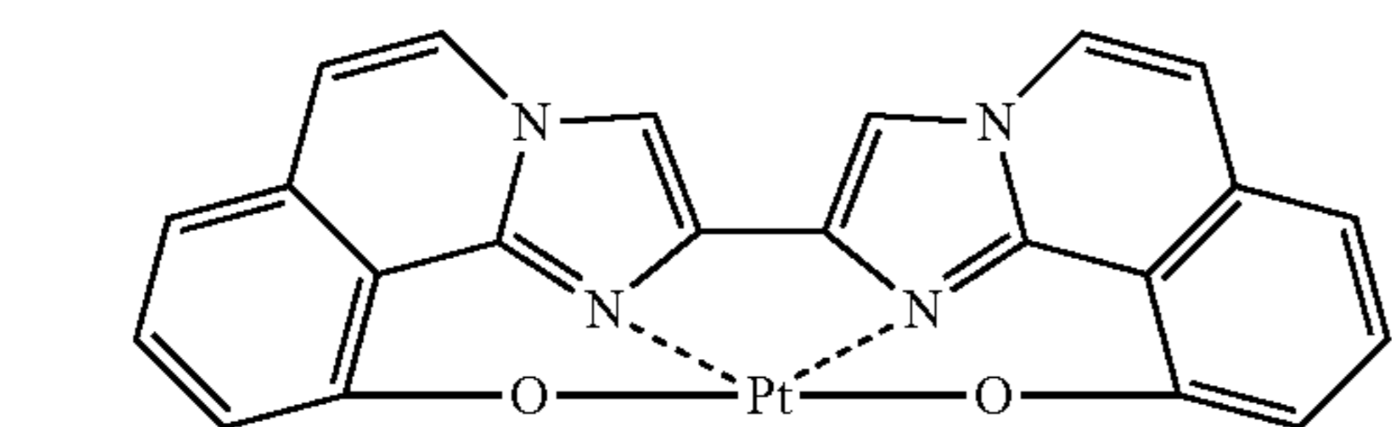
Compound (189)
