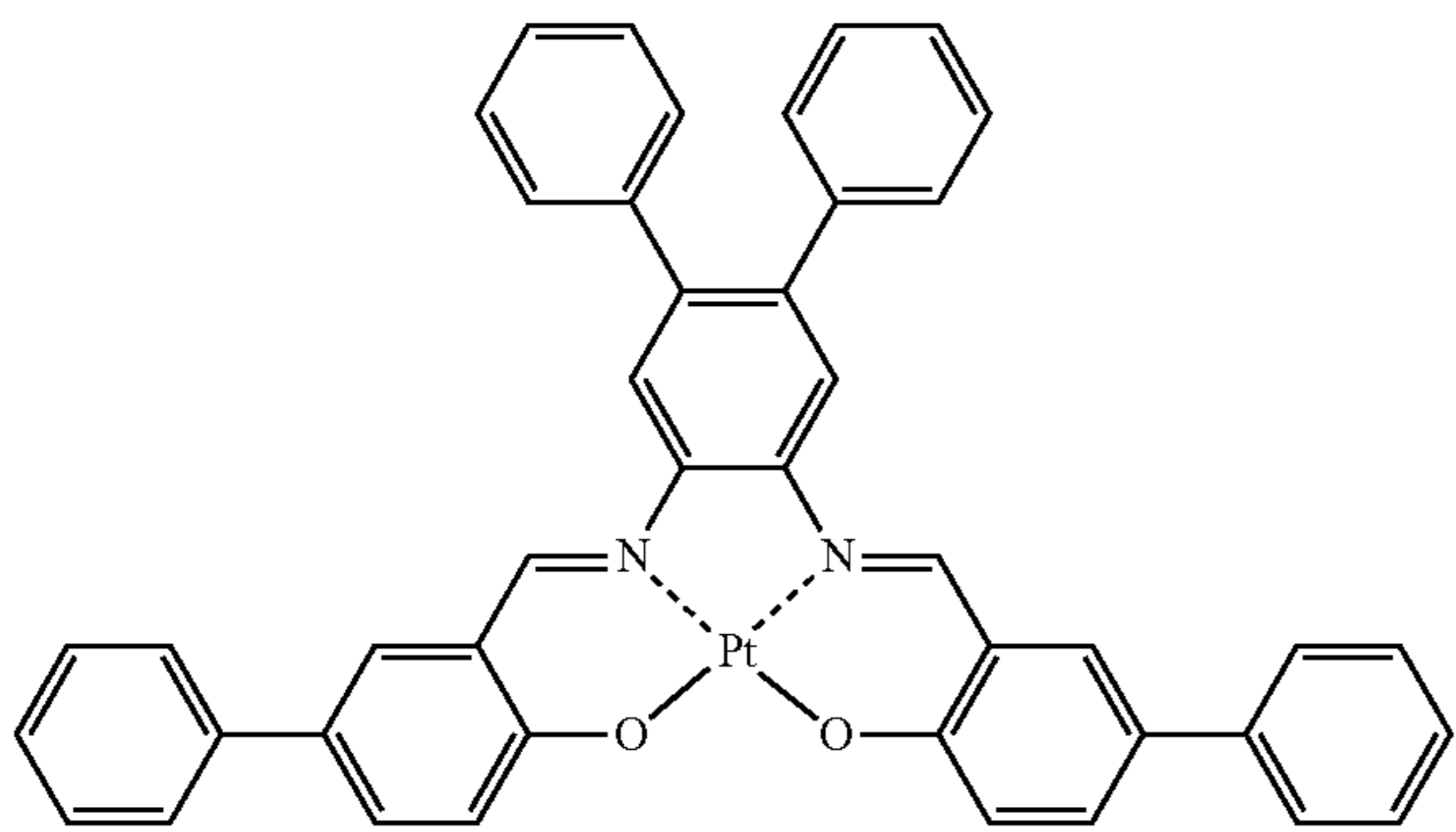
Compound (89)
