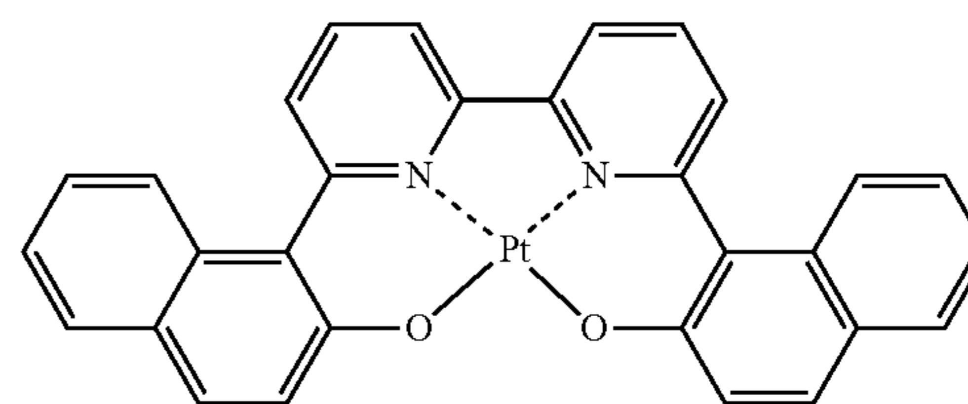
Compound (21)
