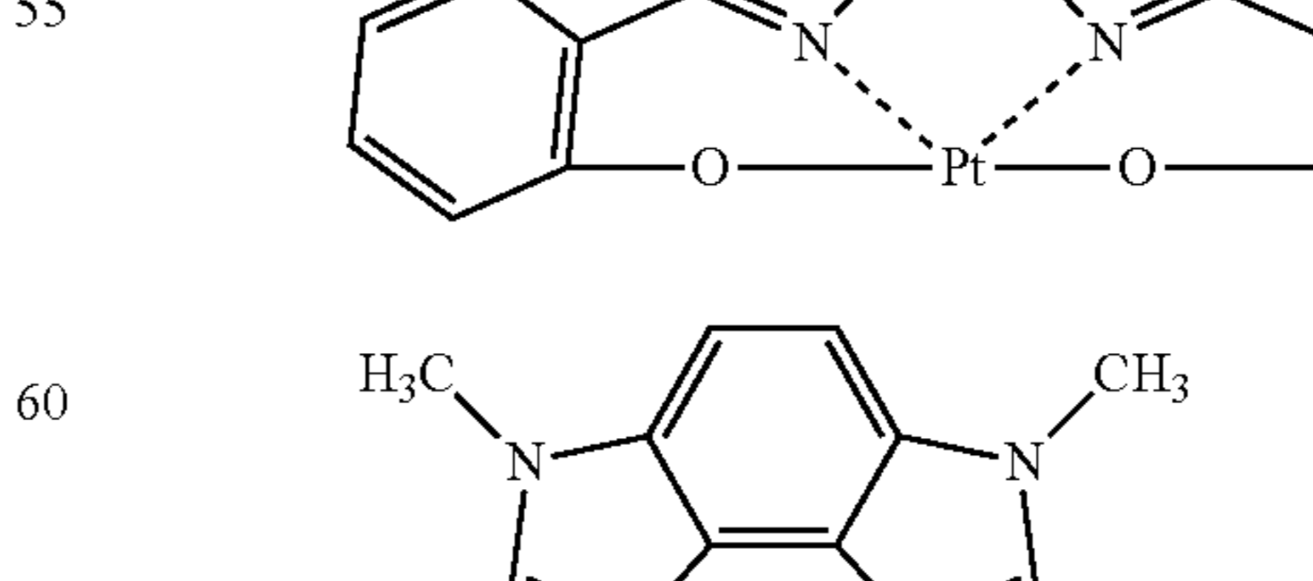
Compound (184)
