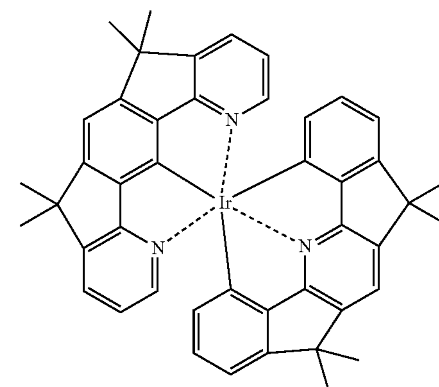
Compound (99)
