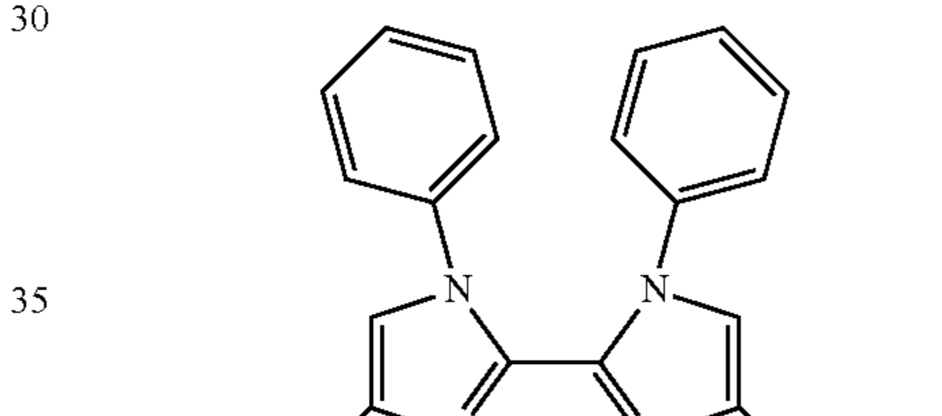
Compound (176)
