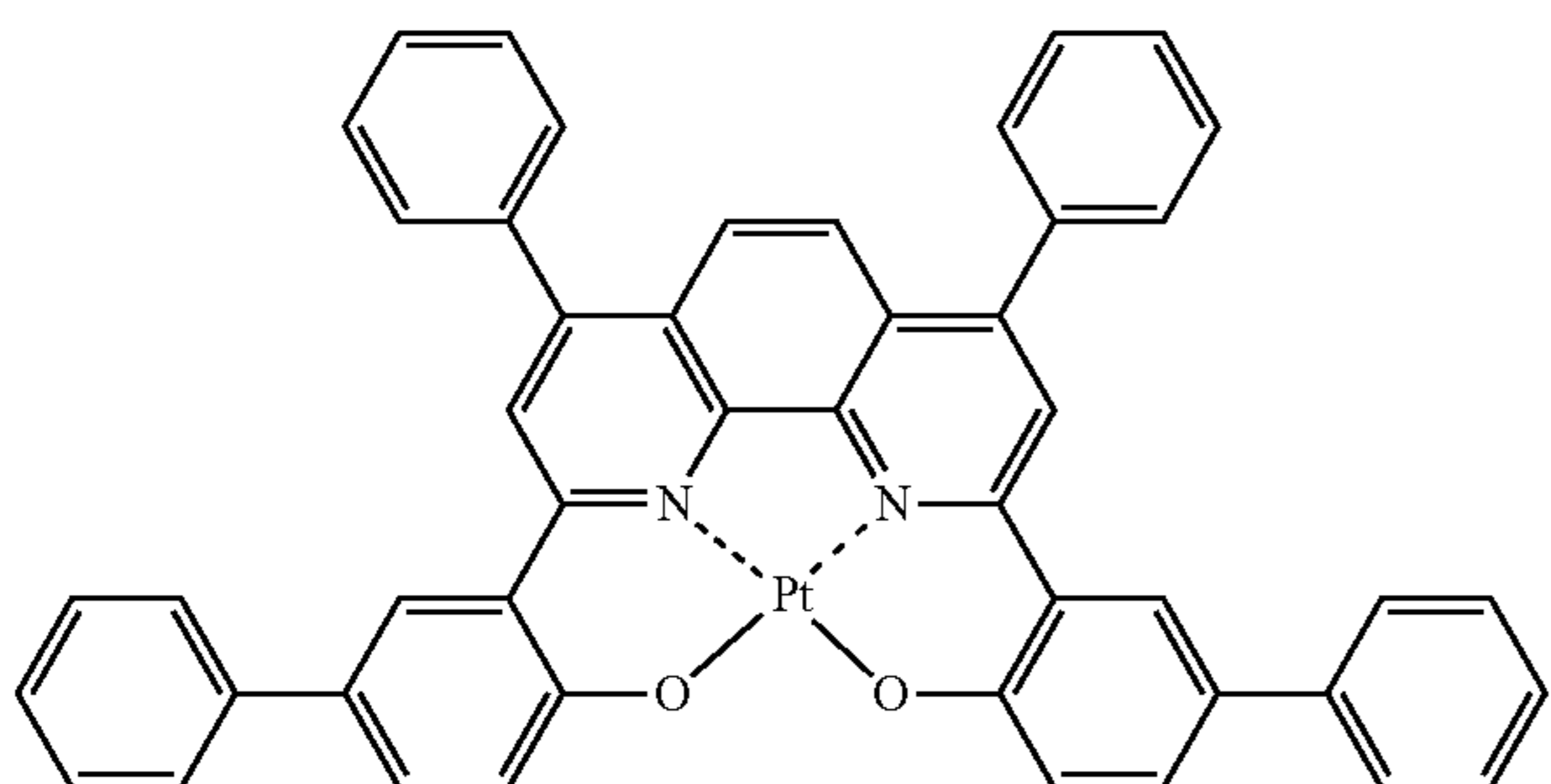
Compound (17)
