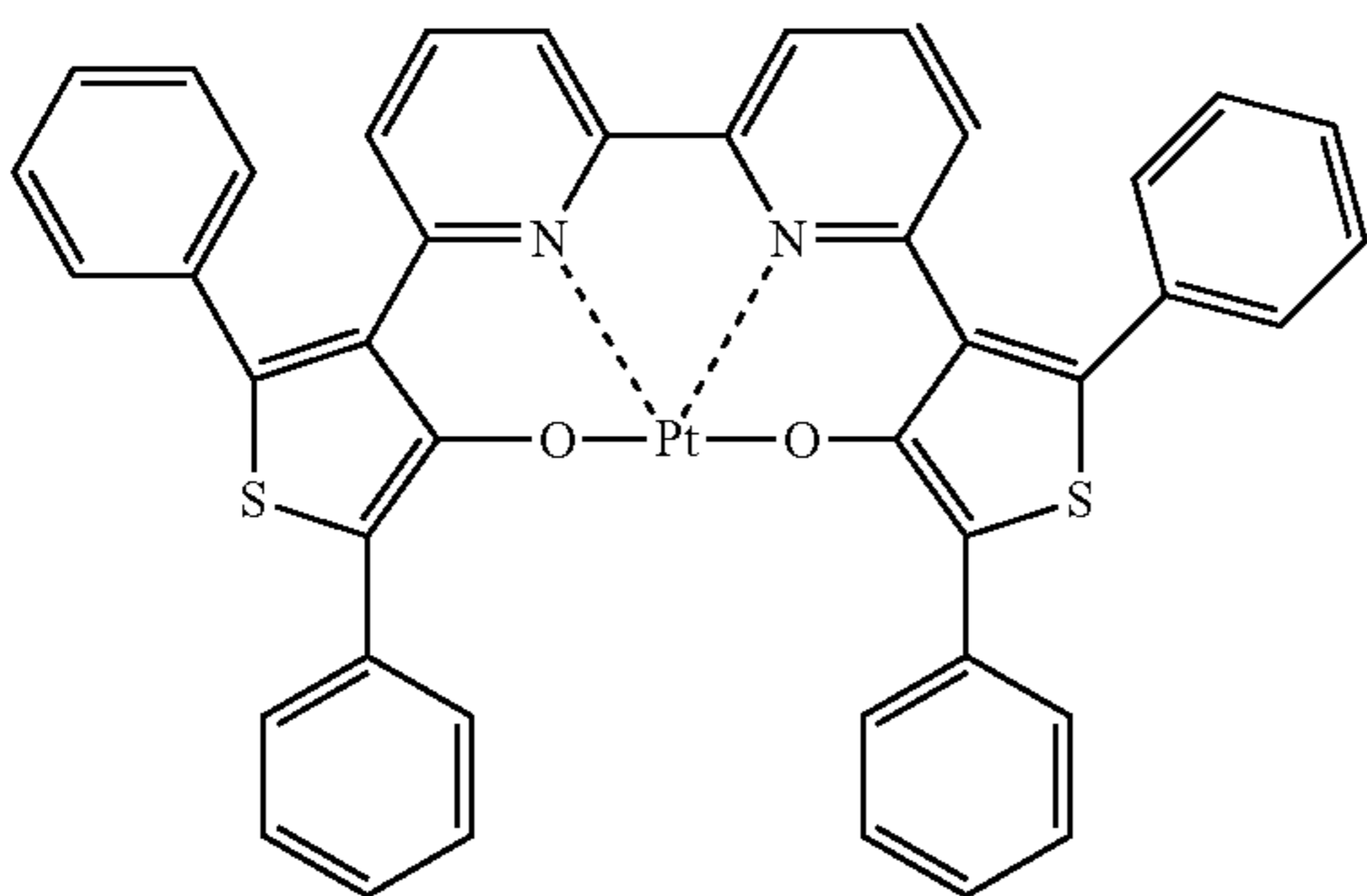
Compound (210)
