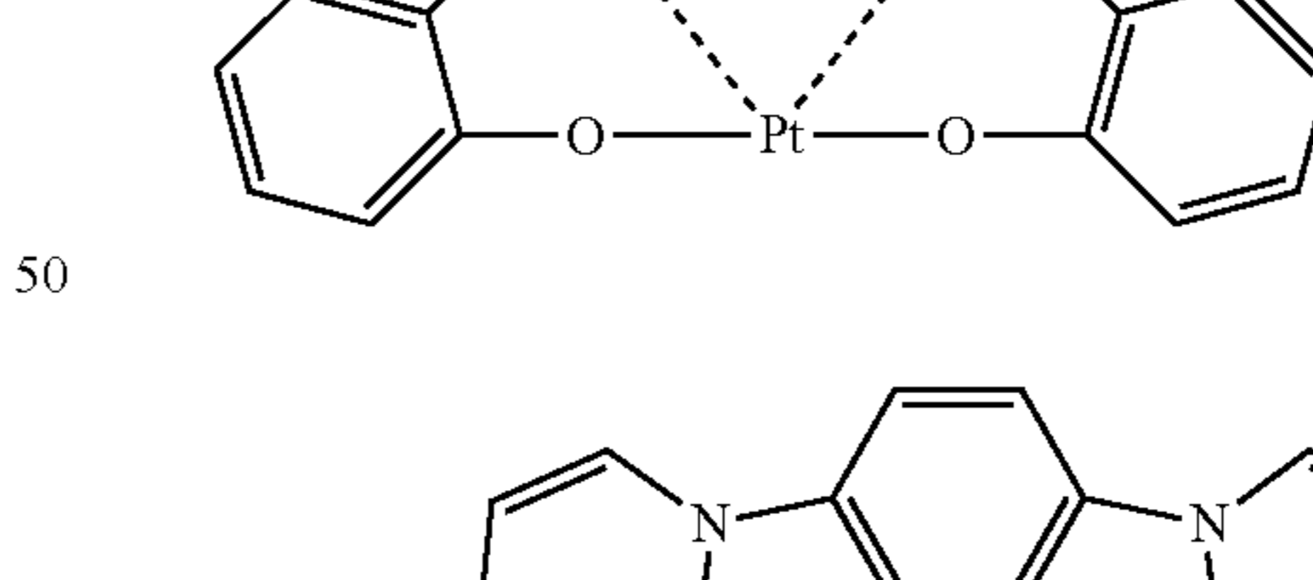
Compound (183)
