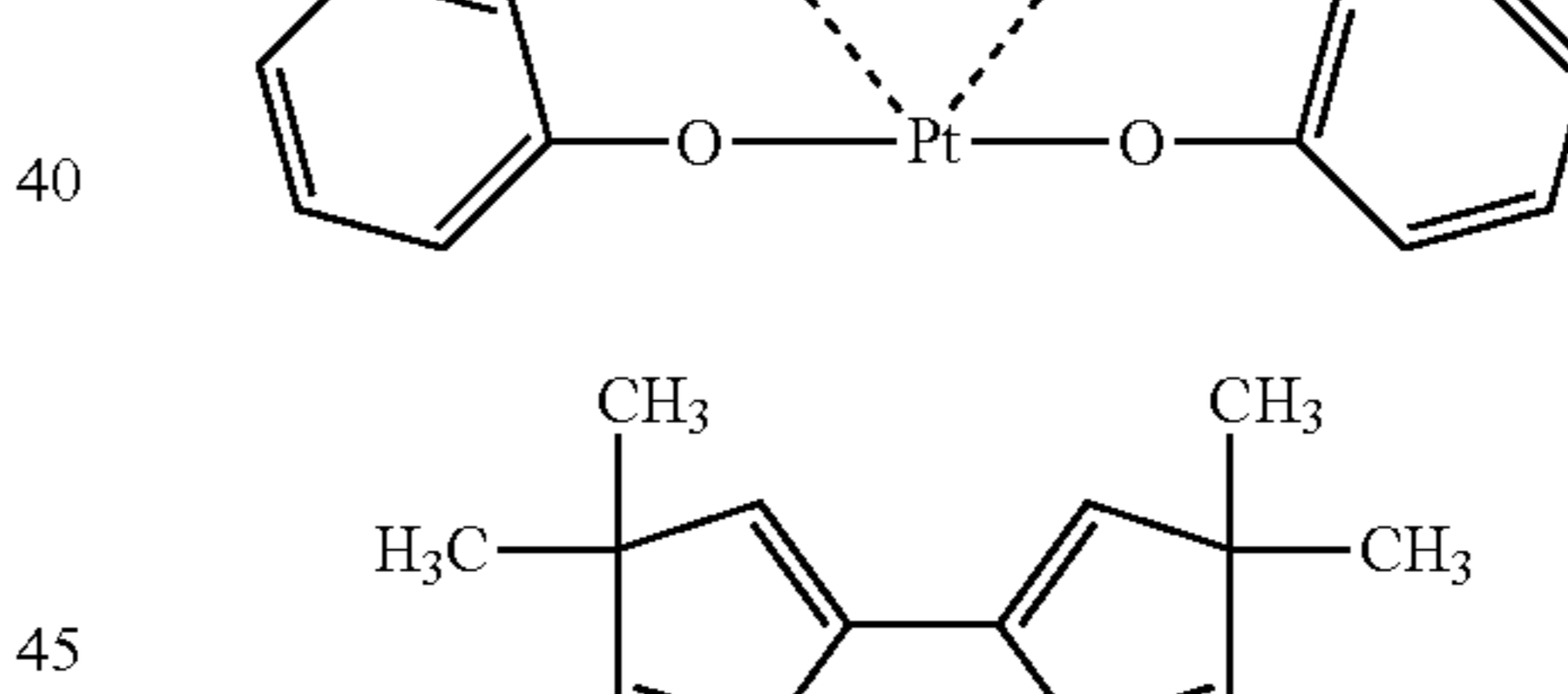
Compound (182)
