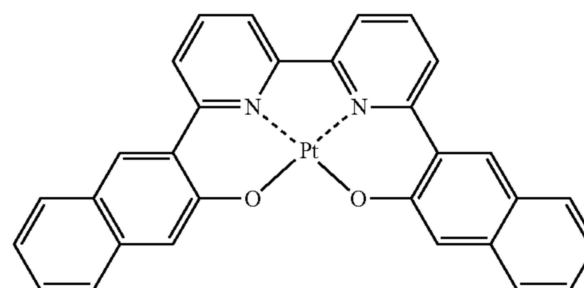
Compound (22)
