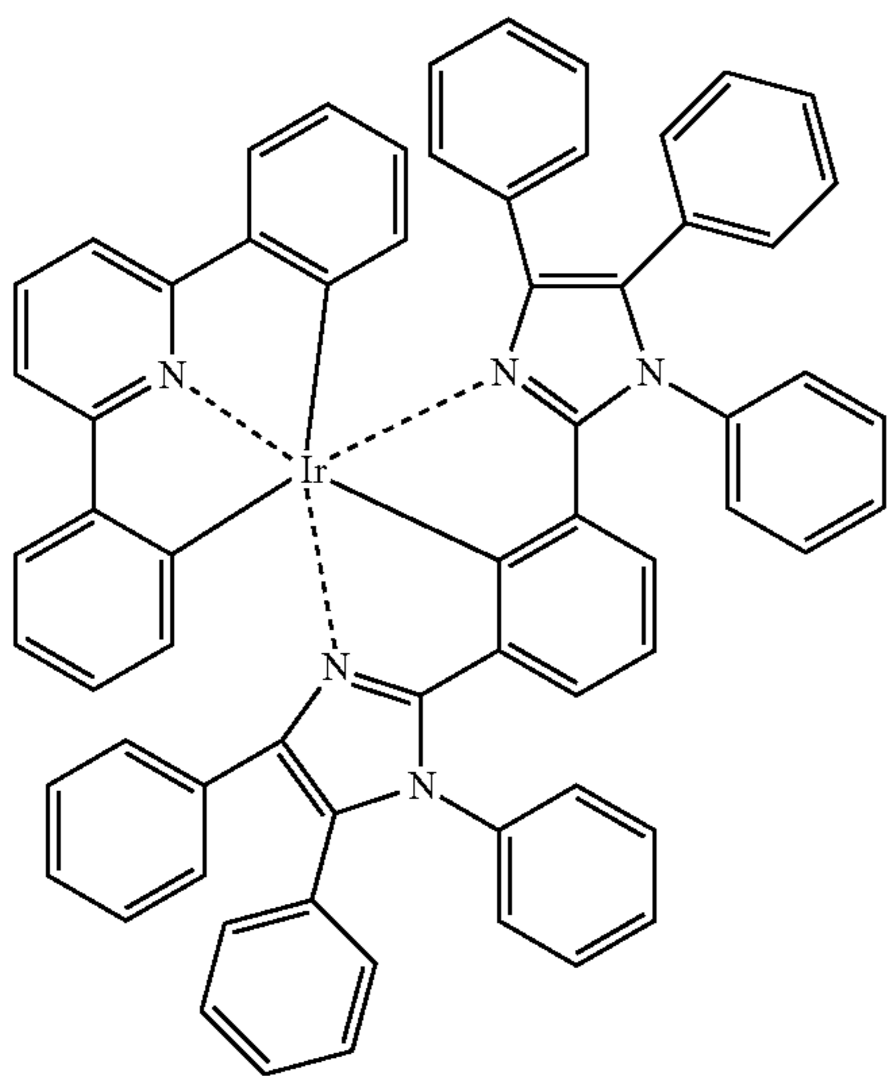
Compound (177)
