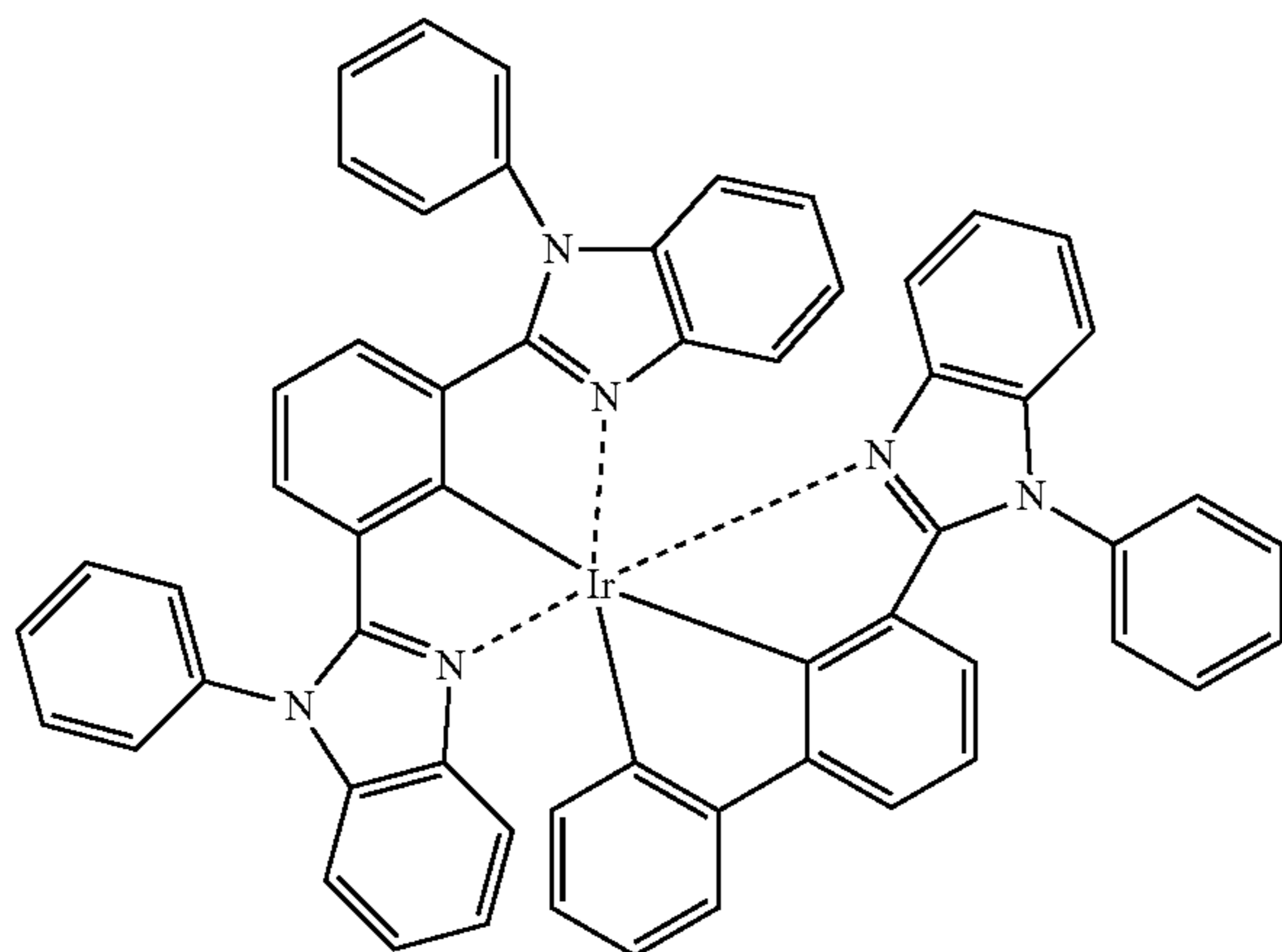
Compound (126)
