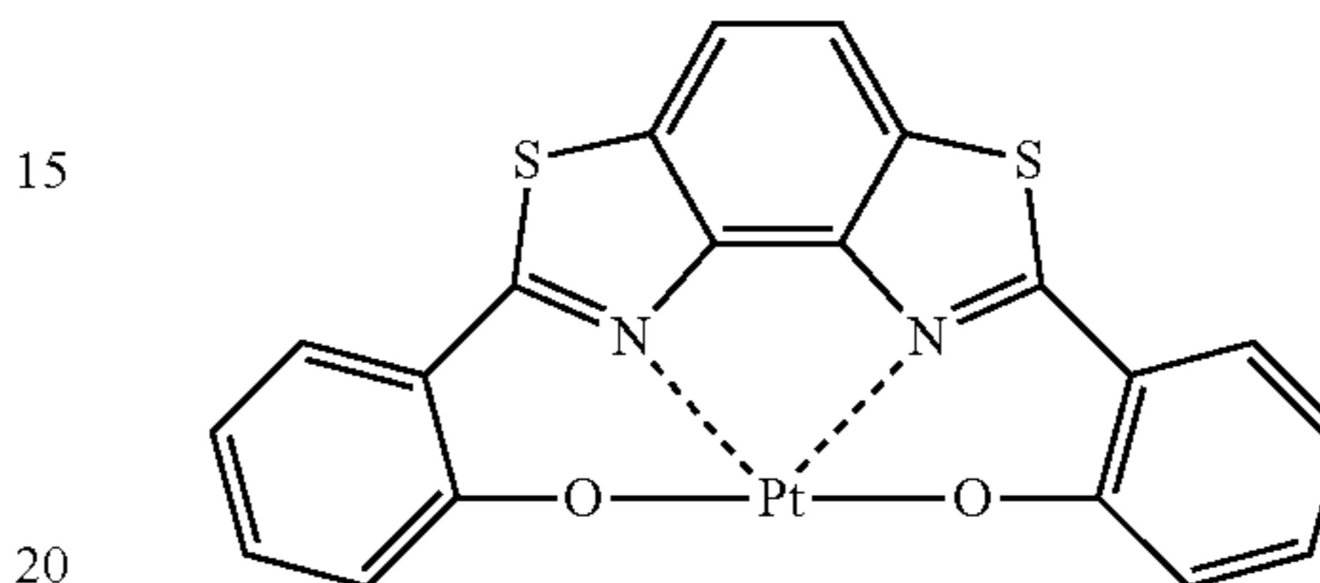
Compound (175)
