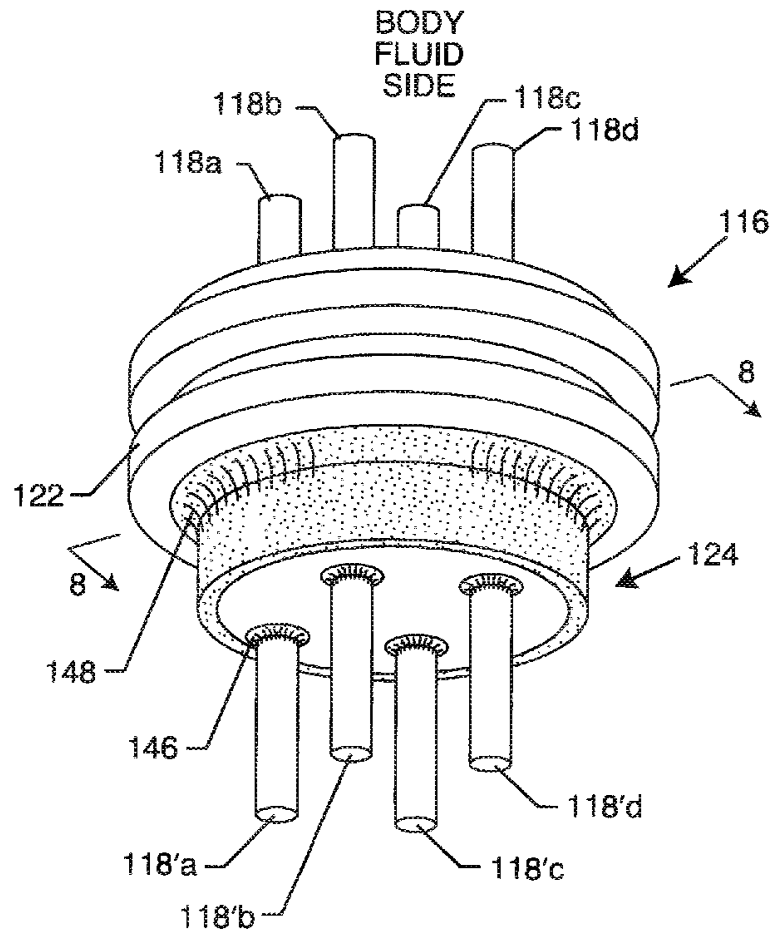
FIG. 7 PRIOR ART
