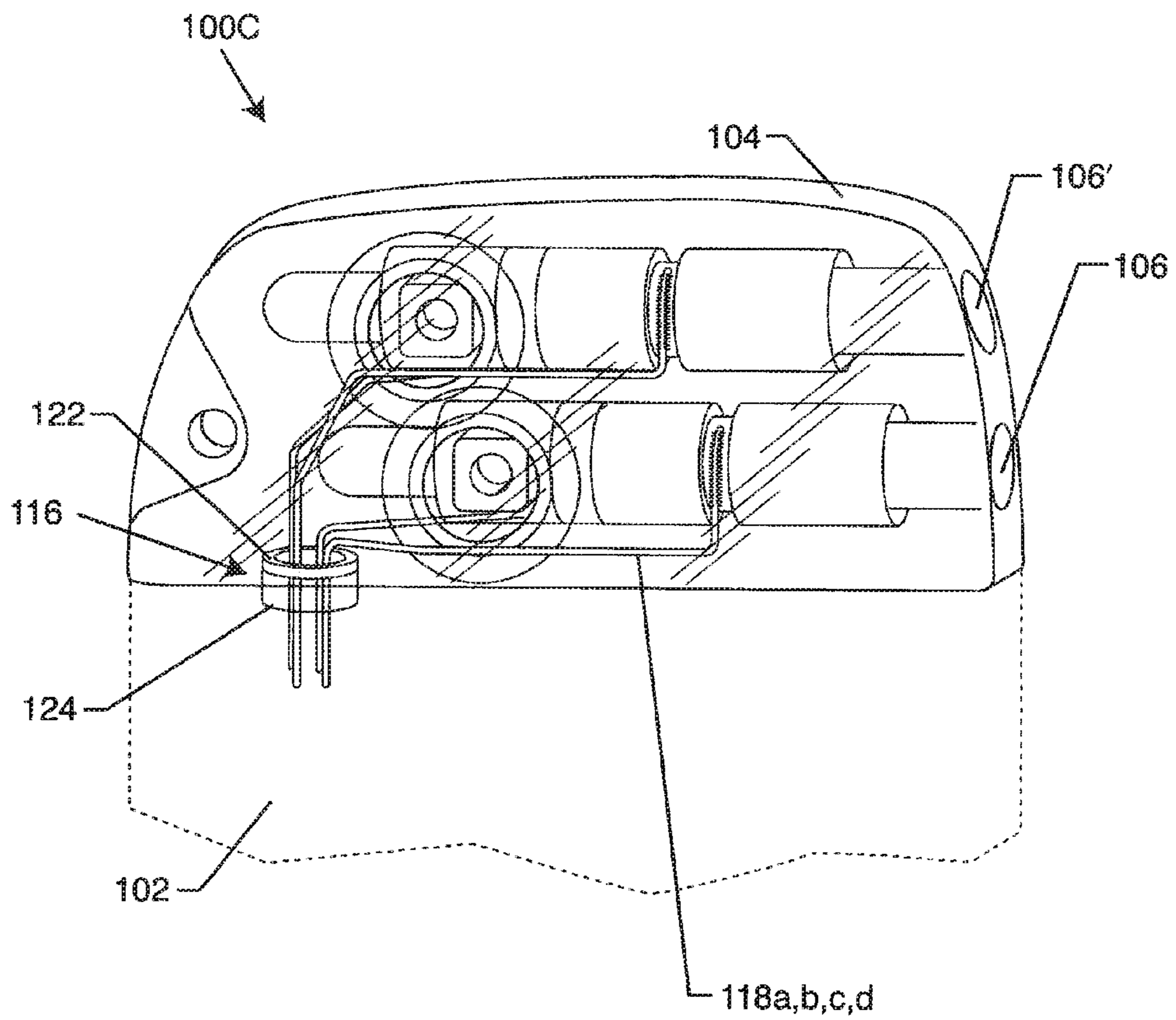
FIG. 27 PRIOR ART
