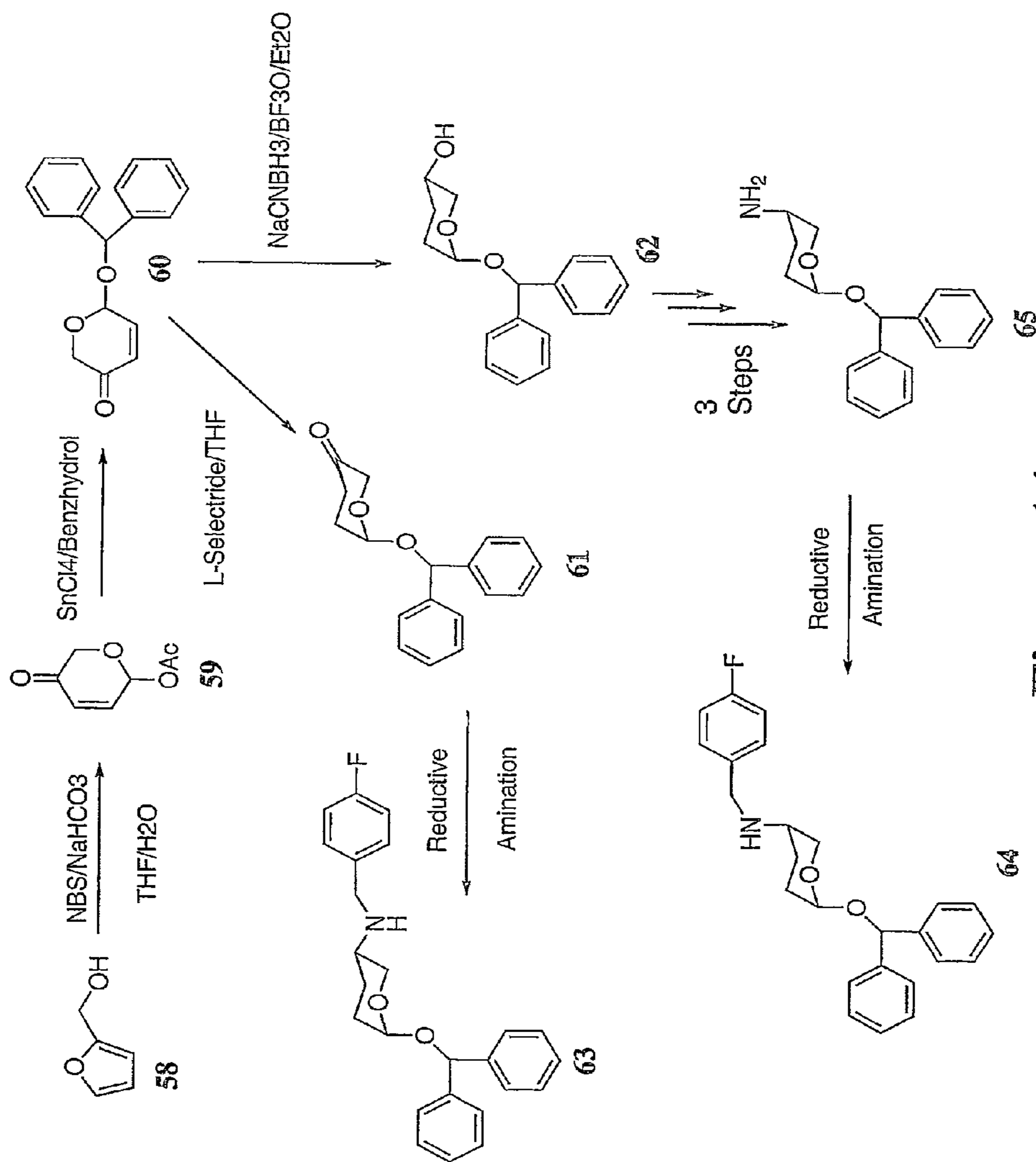
Scheme 9
