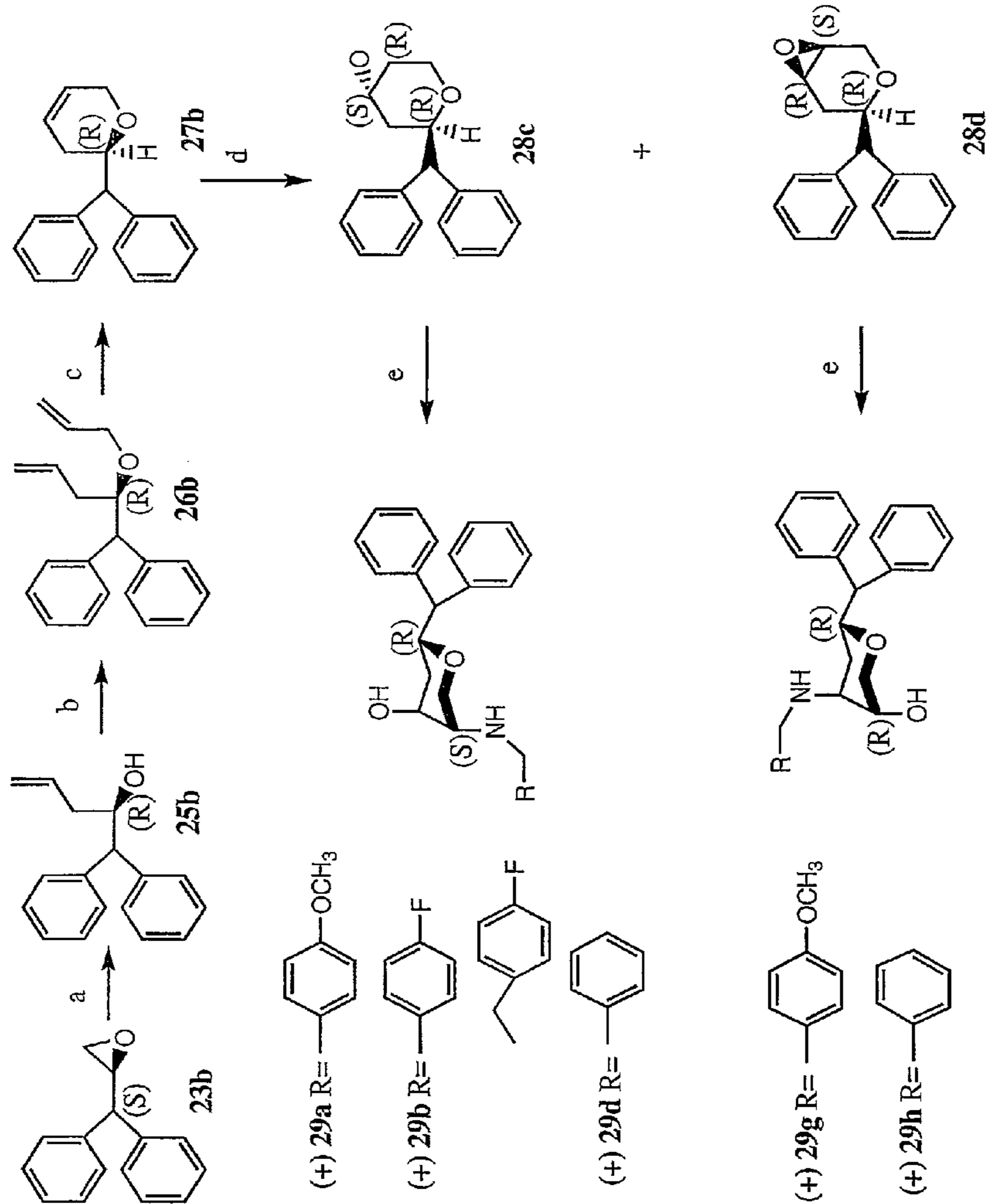
Scheme 3
