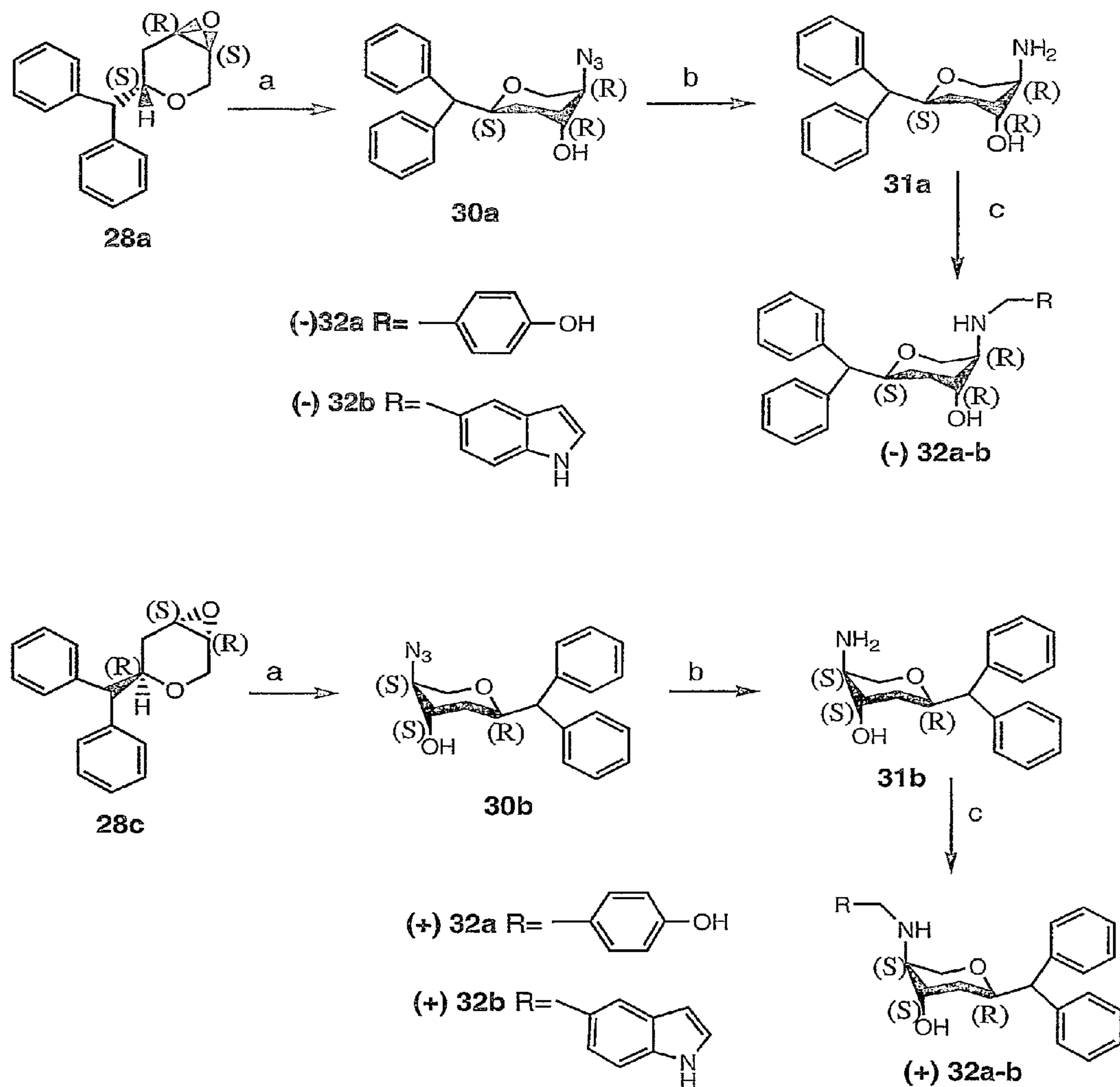
Scheme 4
