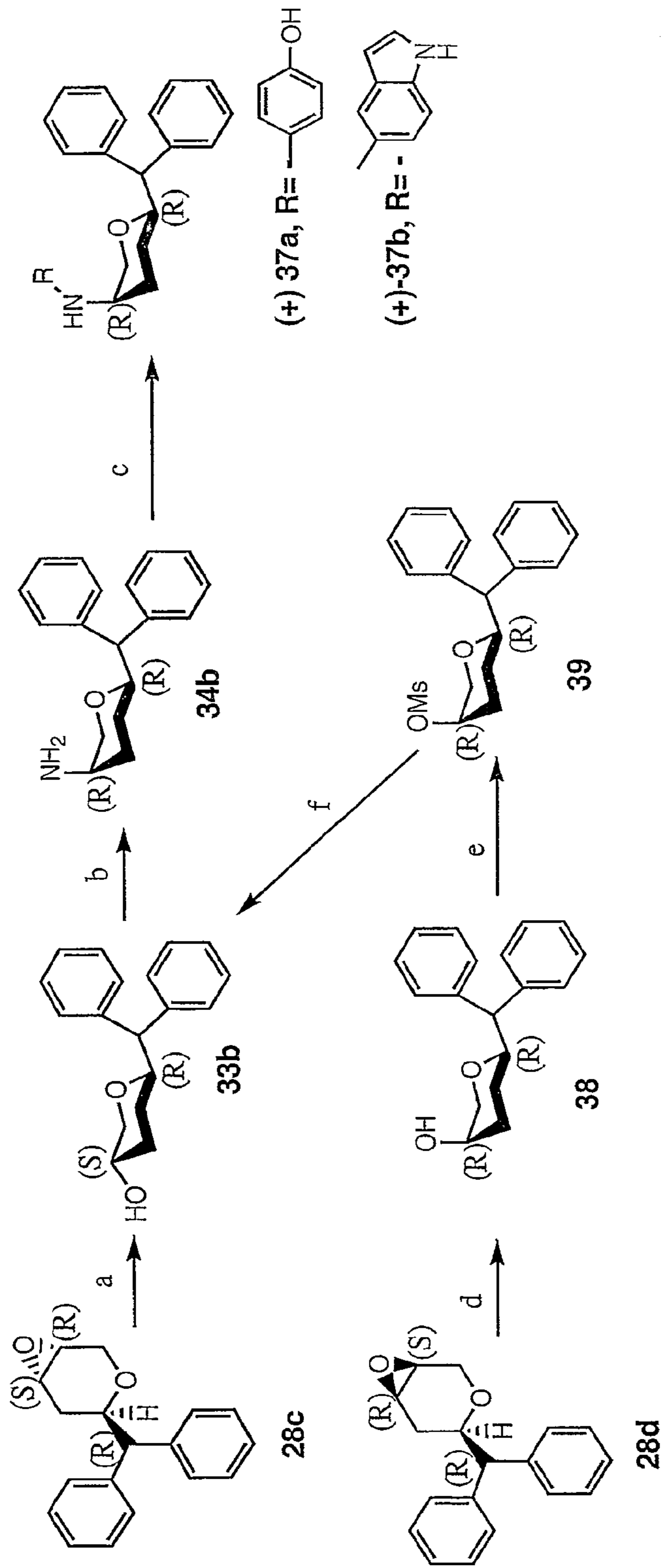
Scheme 6
