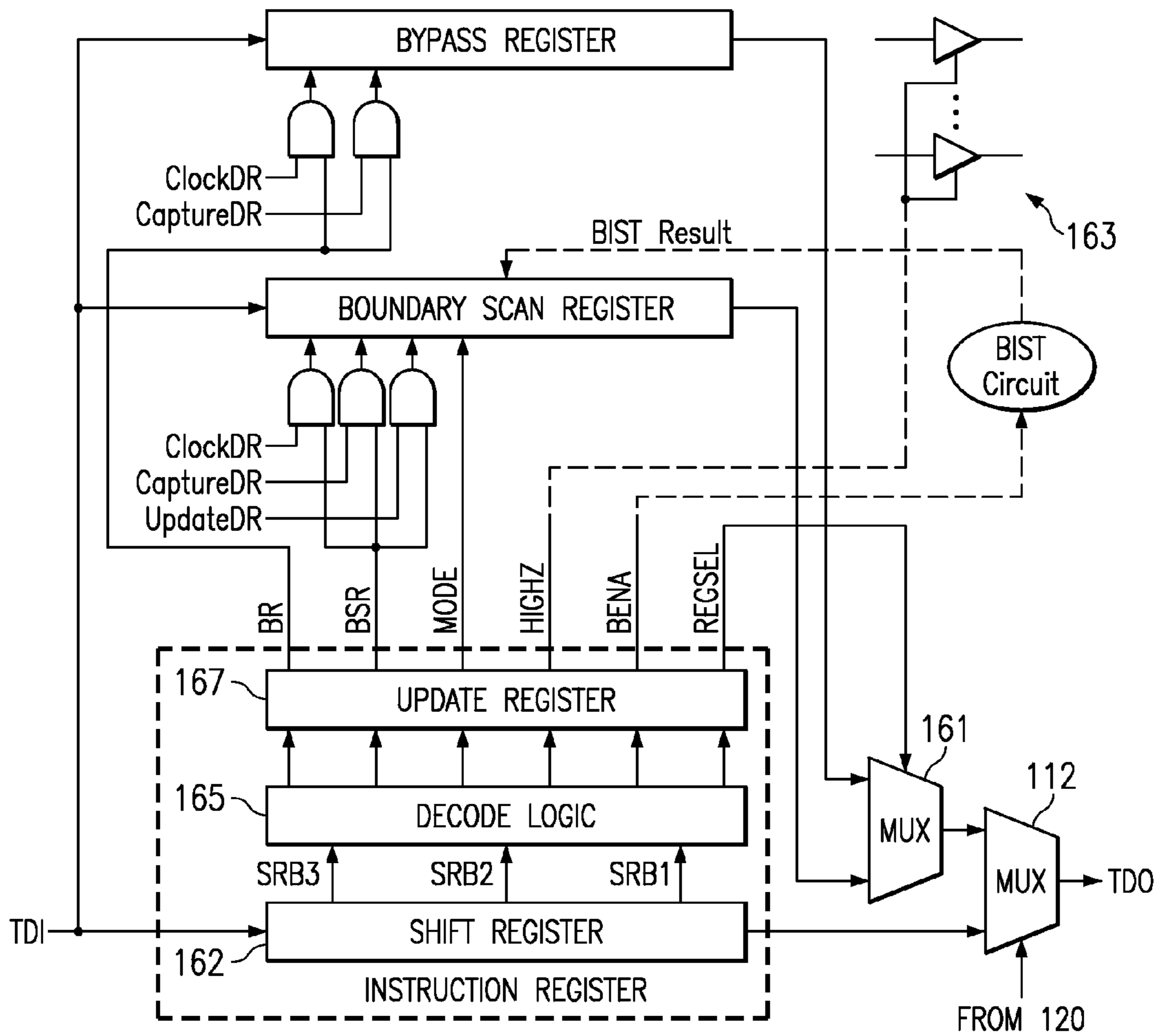
FIG. 16 (PRIOR ART)
