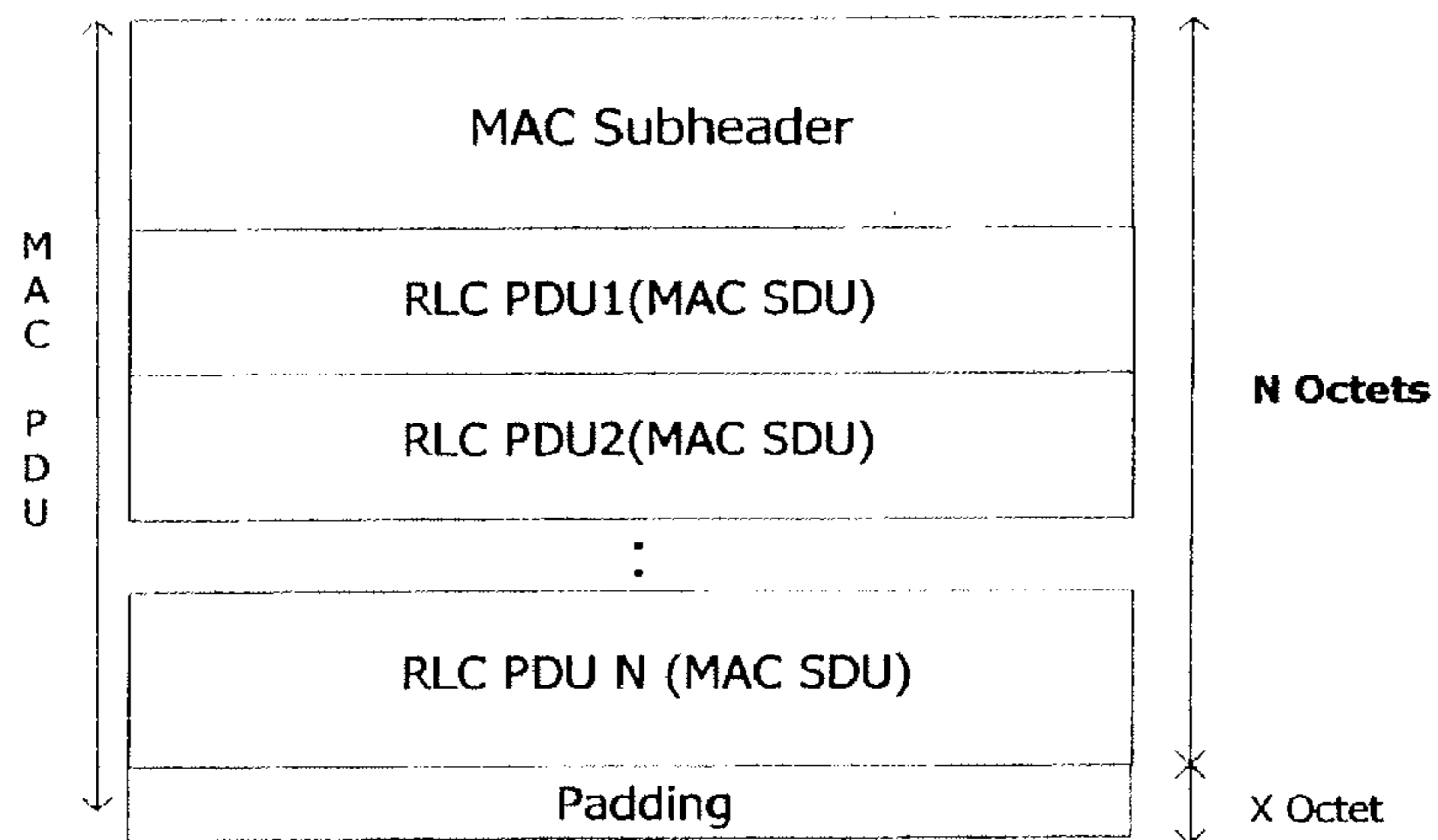
(a) MAC PDU with data and padding
