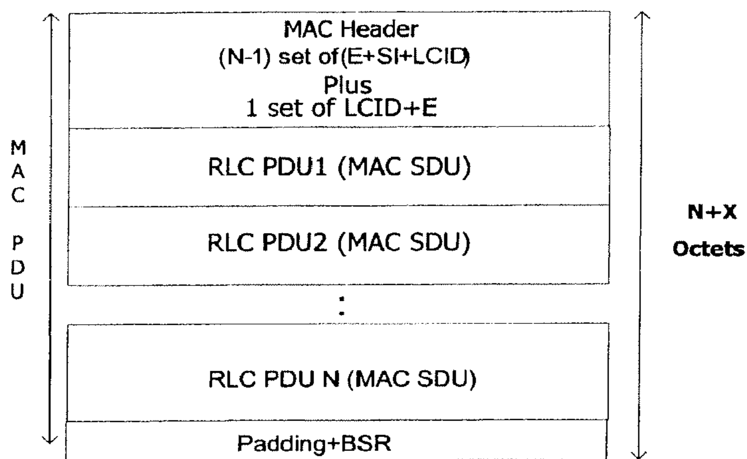
(b) MAC PDU with data and BSR and padding
