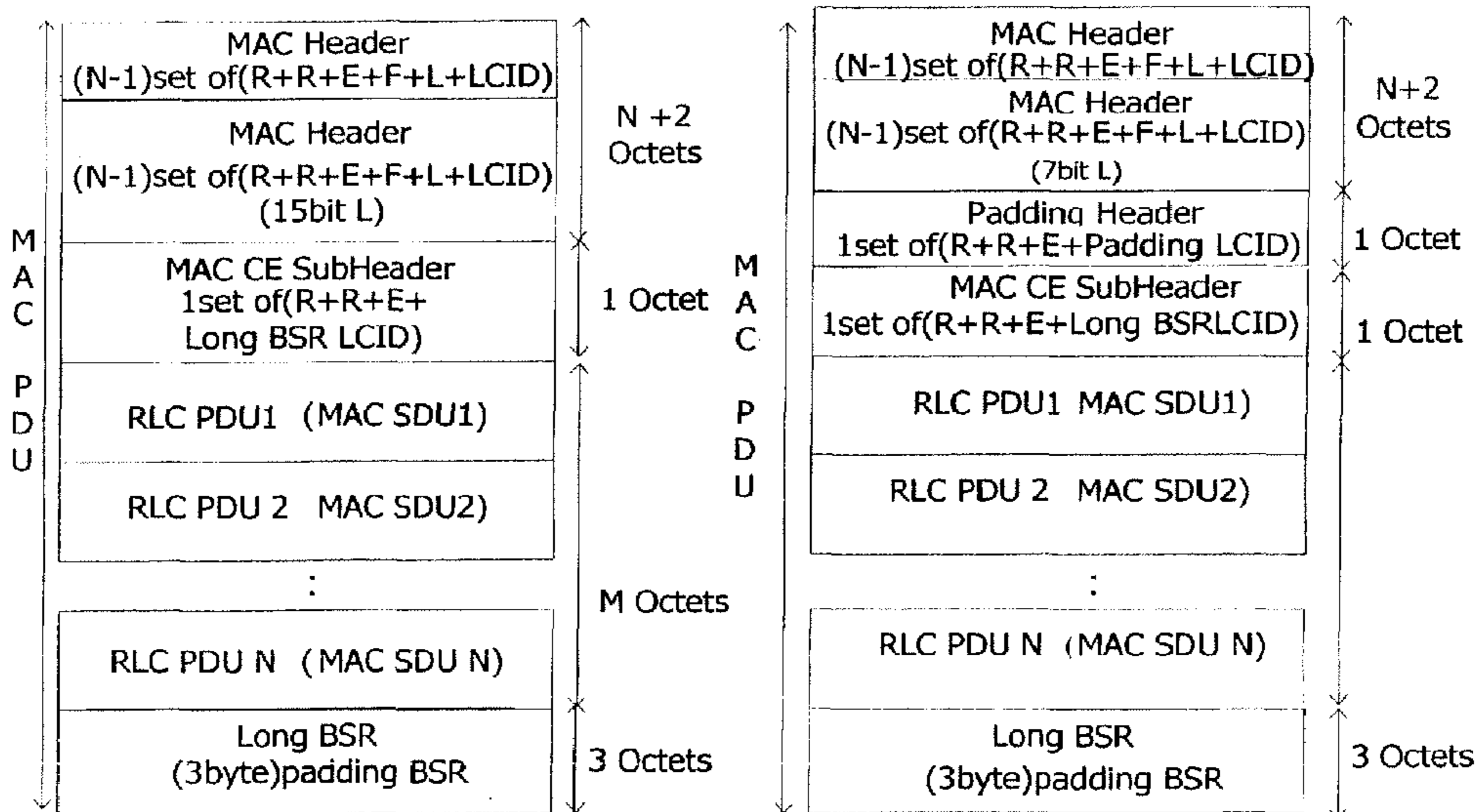
(b)case2, explicit padding BSR
