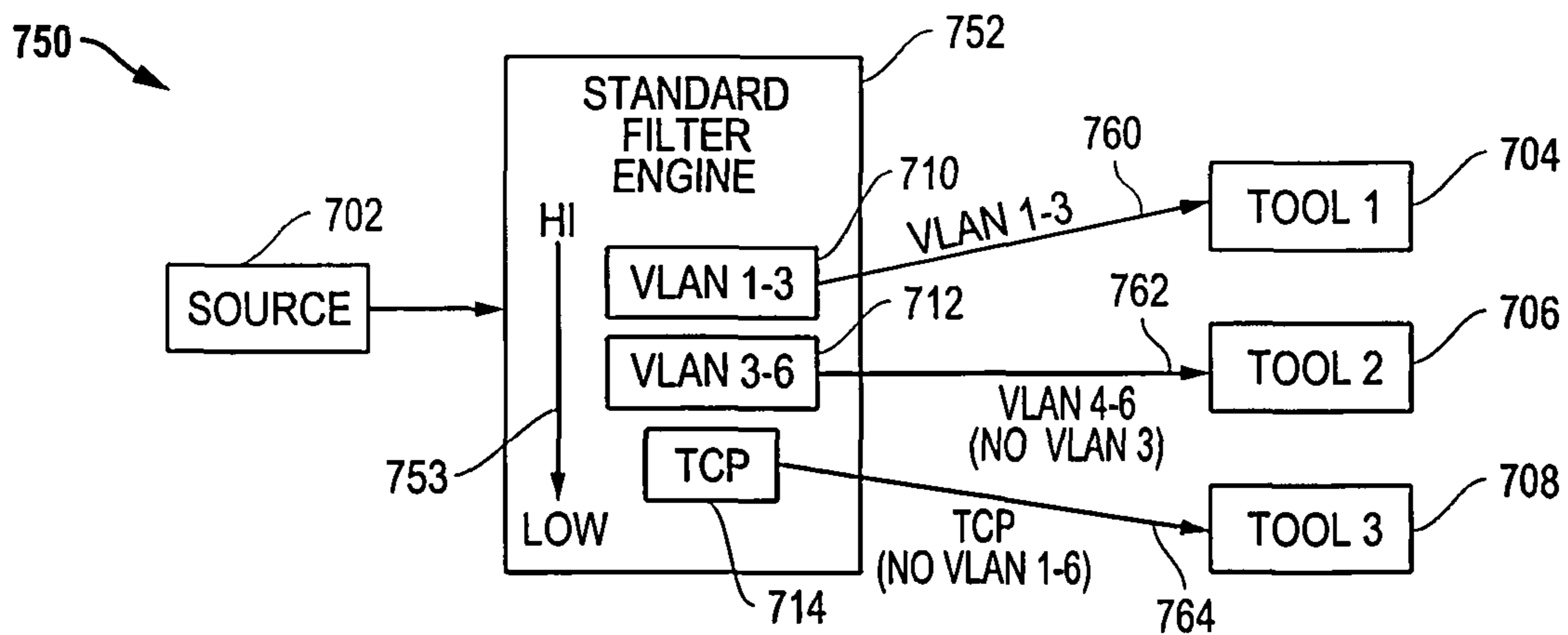
FIG. 7C (Prior Art)
