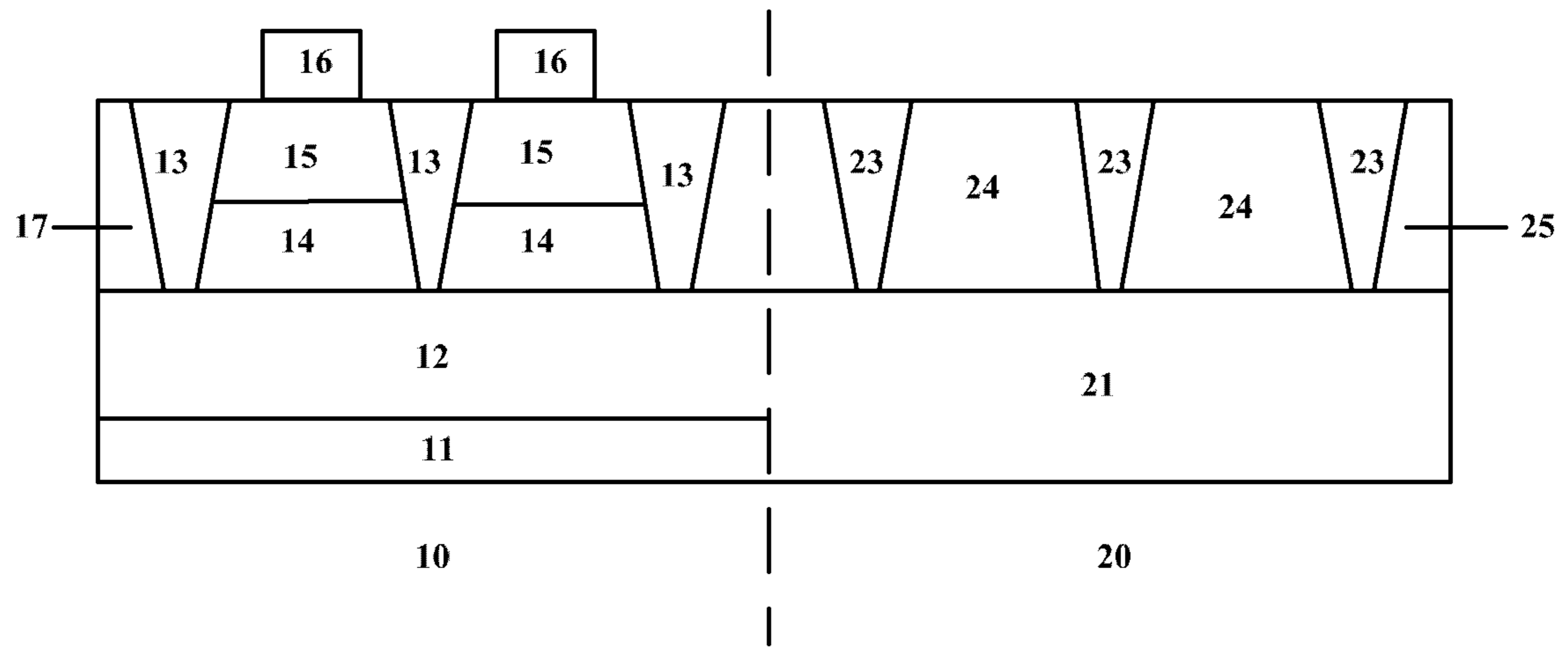
Fig. 7 (prior art)
