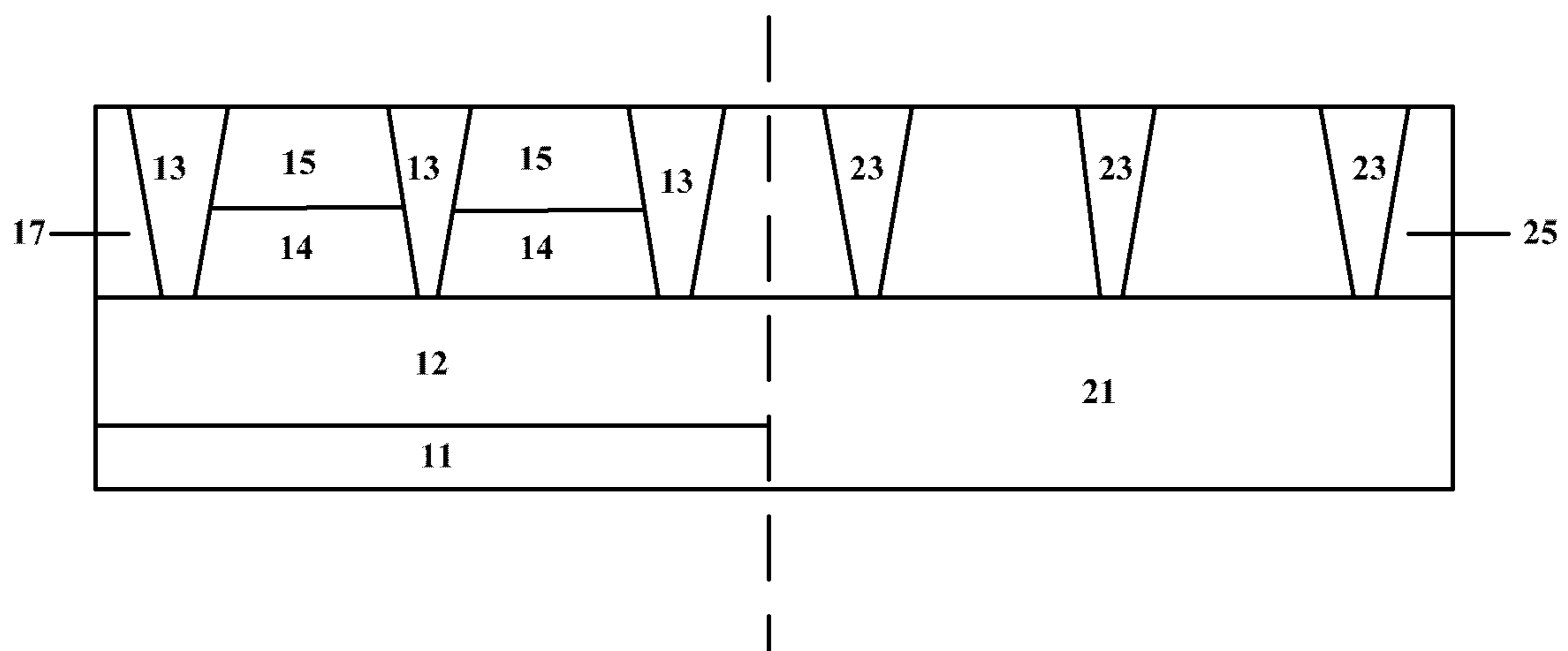
Fig. 5 (prior art)
