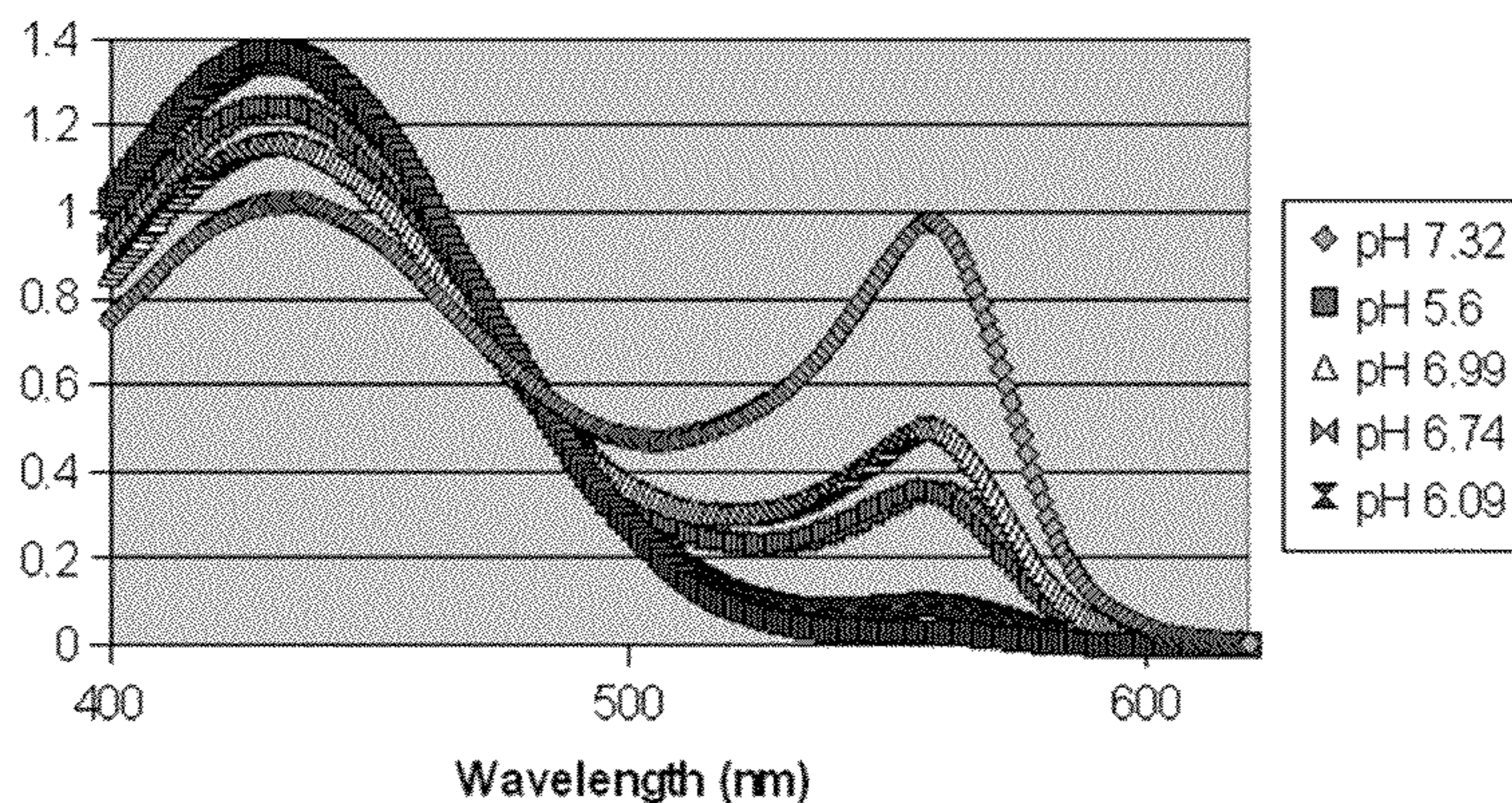
Phenol Red Absorbance in Different pH buffer Solution
