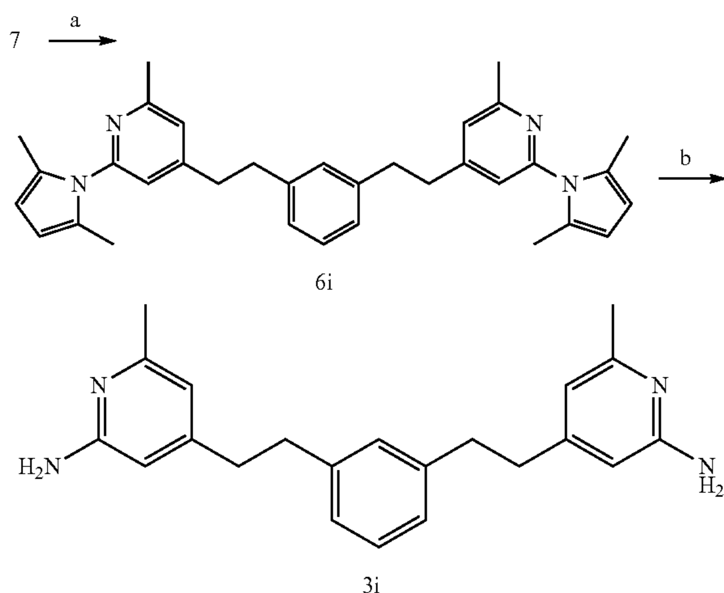
Scheme 4. Synthesis of 3i.
