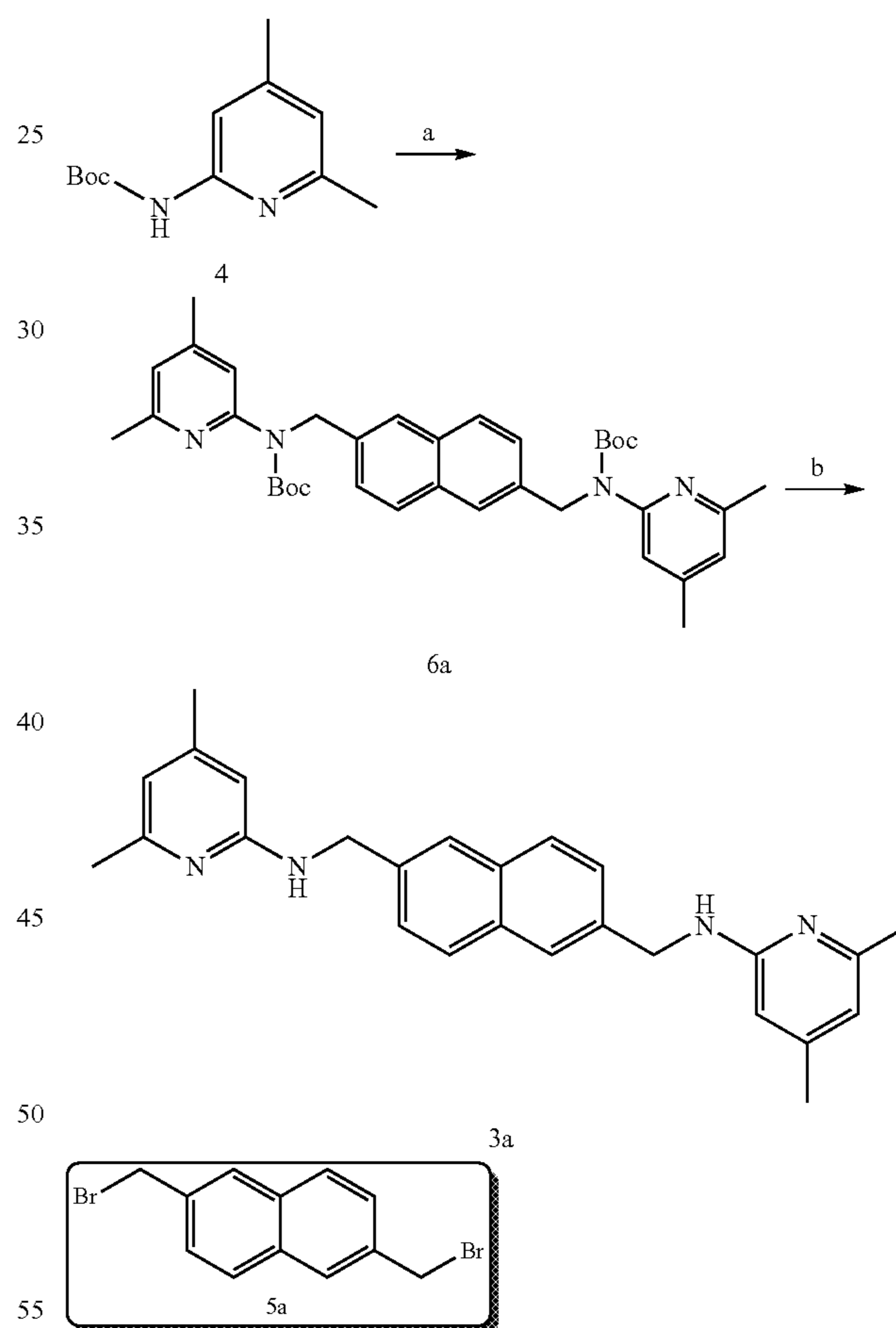
Scheme 1. Synthesis of 3a. α
