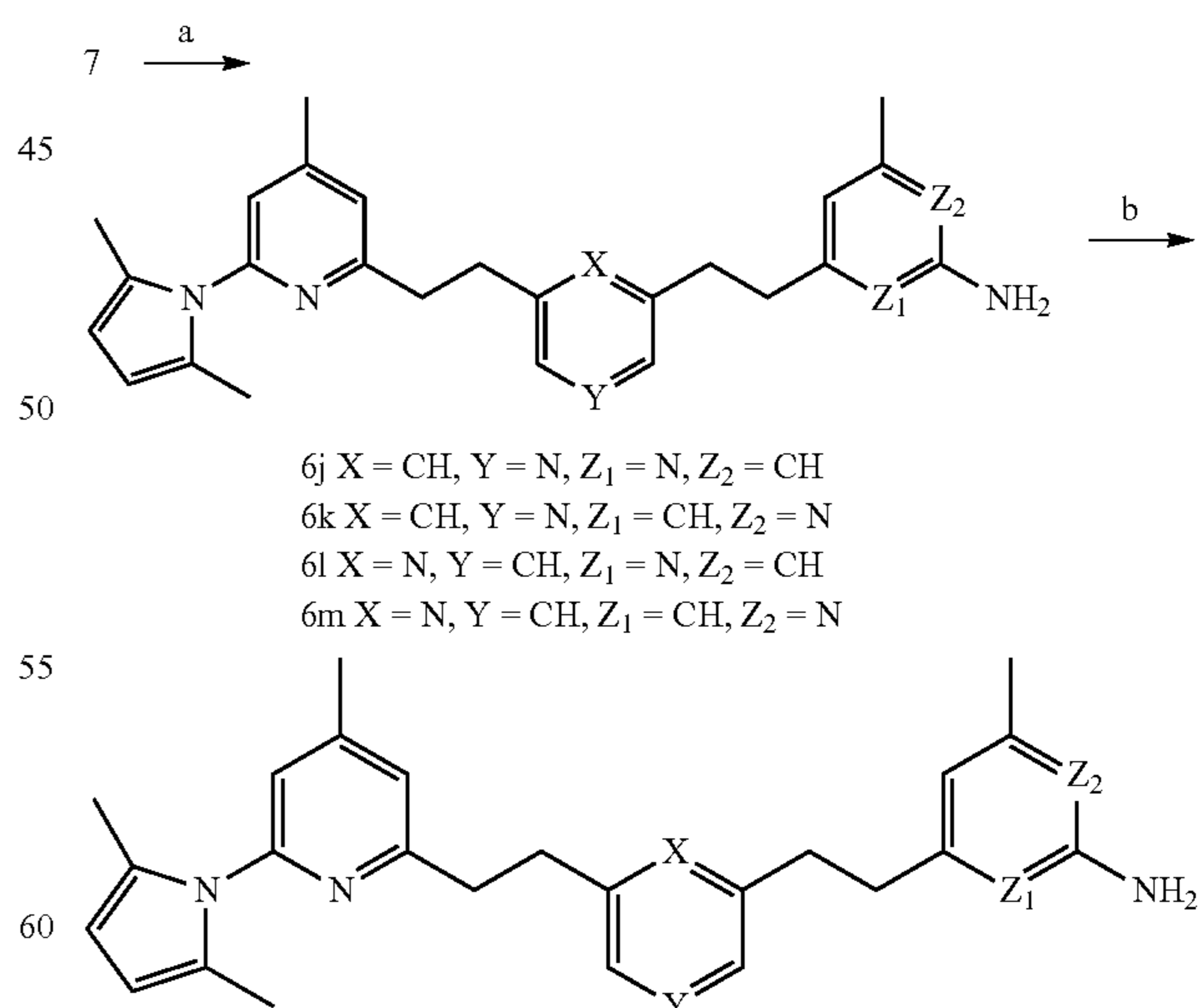
Scheme 5. Synthesis of 3j-m.
