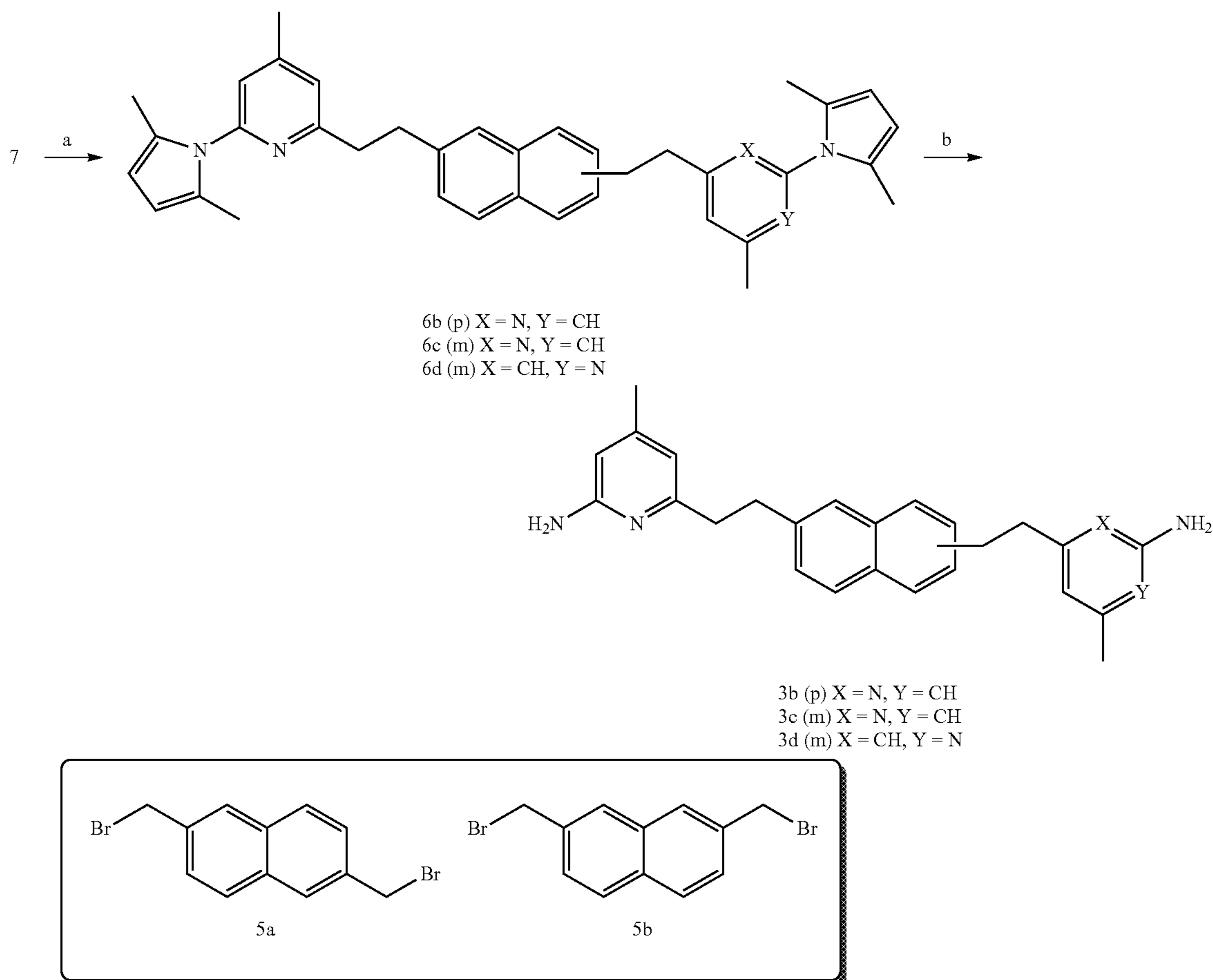
Scheme 2. Synthesis of 3b-d.
