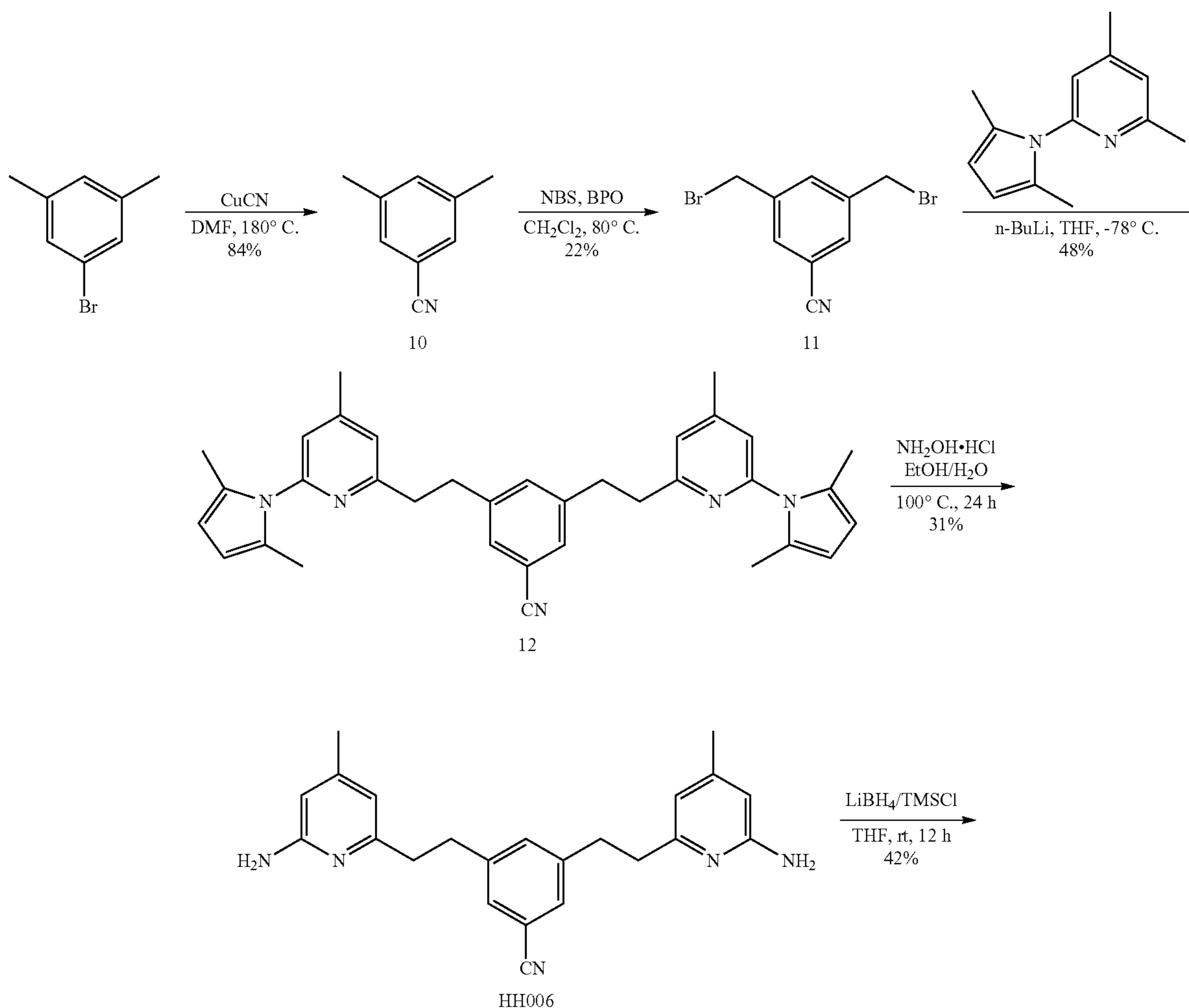
Scheme 9.
