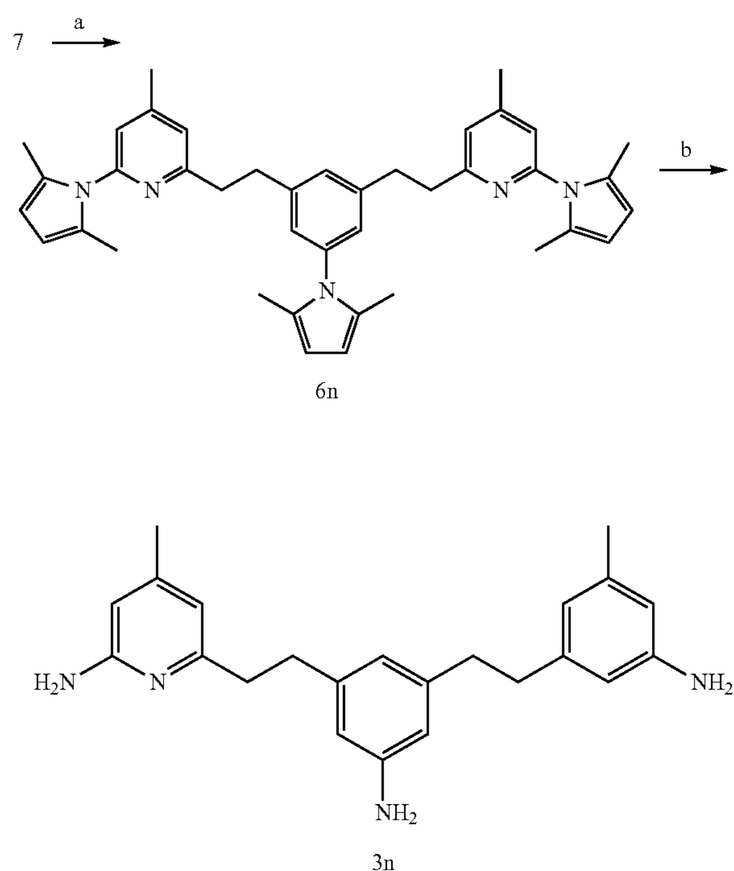
Scheme 7. Synthesis of amino-substituted inhibitor 3n.
