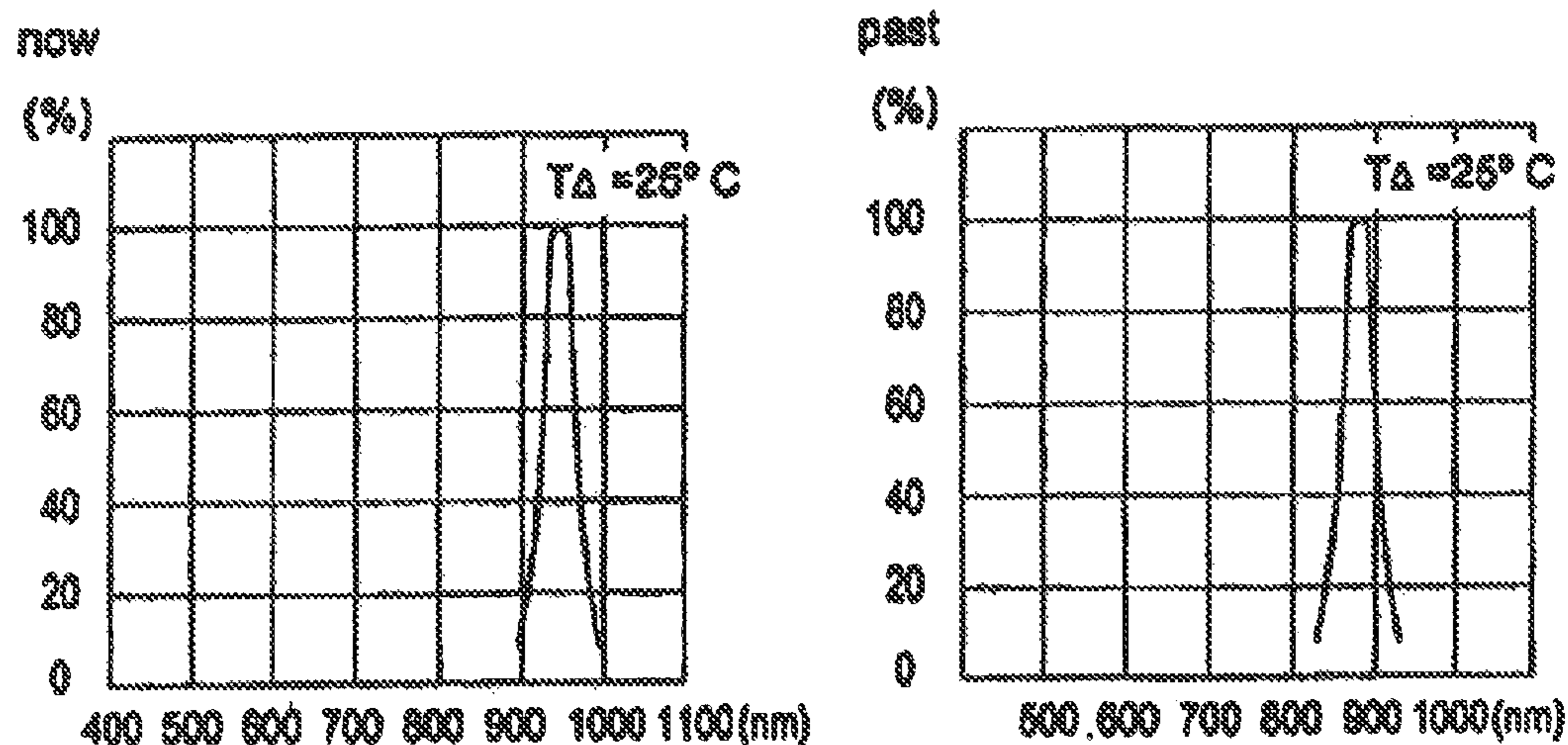
The spectral curve of the LED
